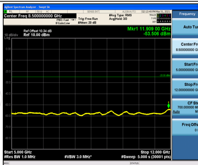
Band7-10MHz-16QAM-20800-1RB#0-Range6:12000~26500MHz
