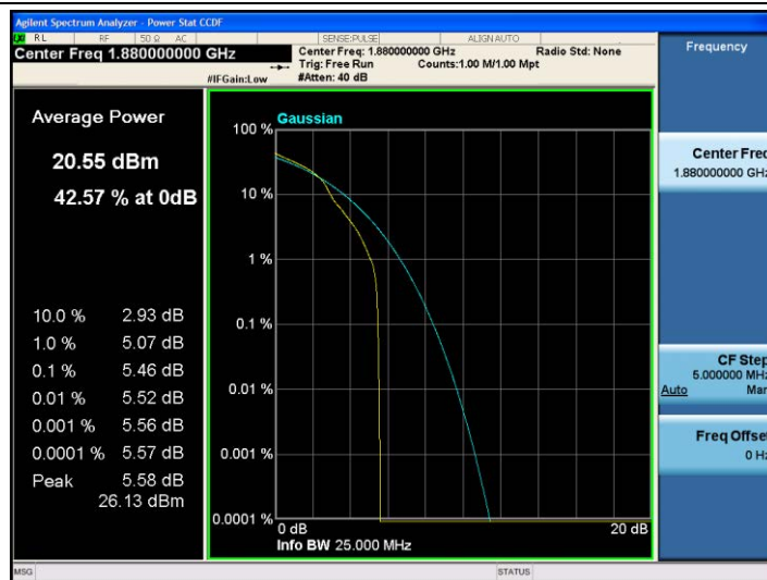
Band2-1.4MHz-16QAM-18900-1RB#0
