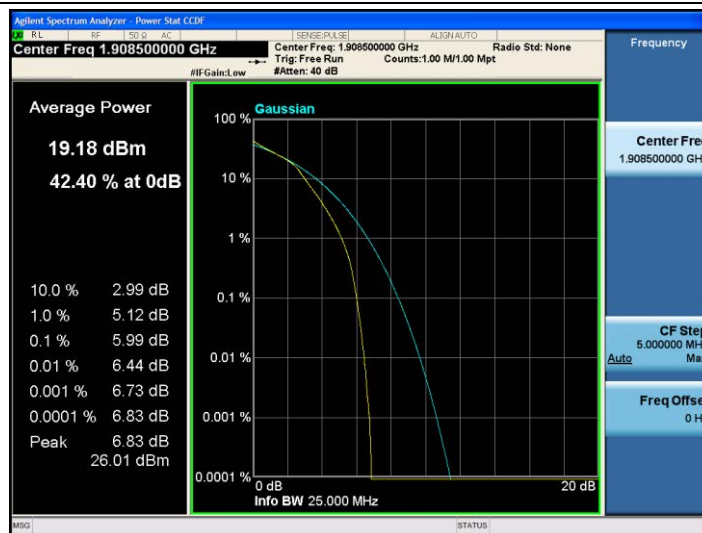
Band2-3MHz-16QAM-19185-15RB#0
