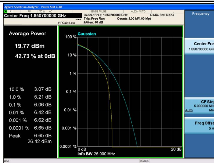
Band2-1.4MHz-16QAM-18607-6RB#0
