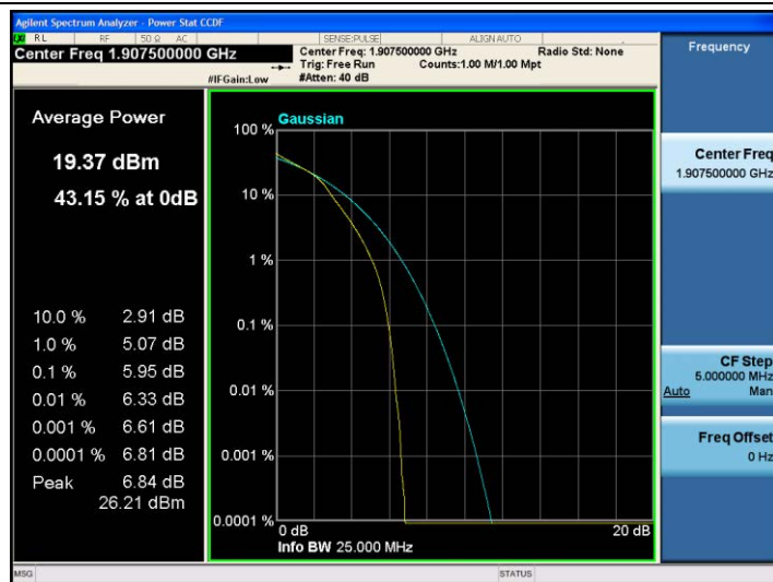
Band2-5MHz-16QAM-19175-25RB#0
