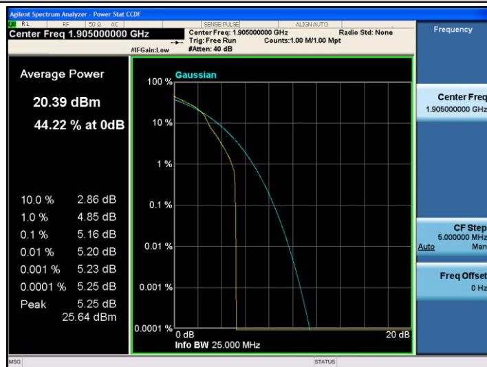
Band2-10MHz-16QAM-19150-1RB#0
