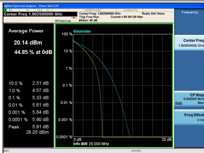
Band2-15MHz-QPSK-19125-75RB#0
