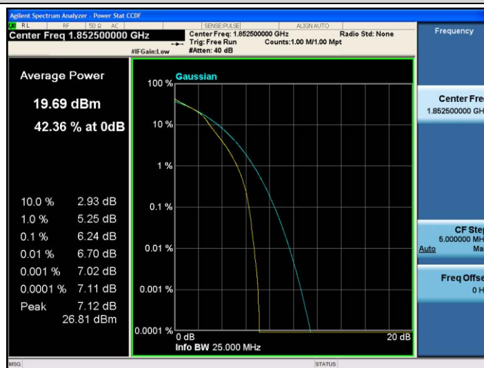
Band2-5MHz-16QAM-18625-25RB#0
