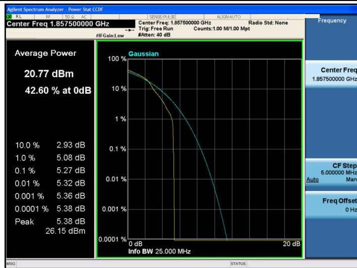
Band2-15MHz-16QAM-18675-1RB#0
