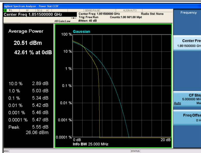
Band2-3MHz-16QAM-18615-1RB#0
