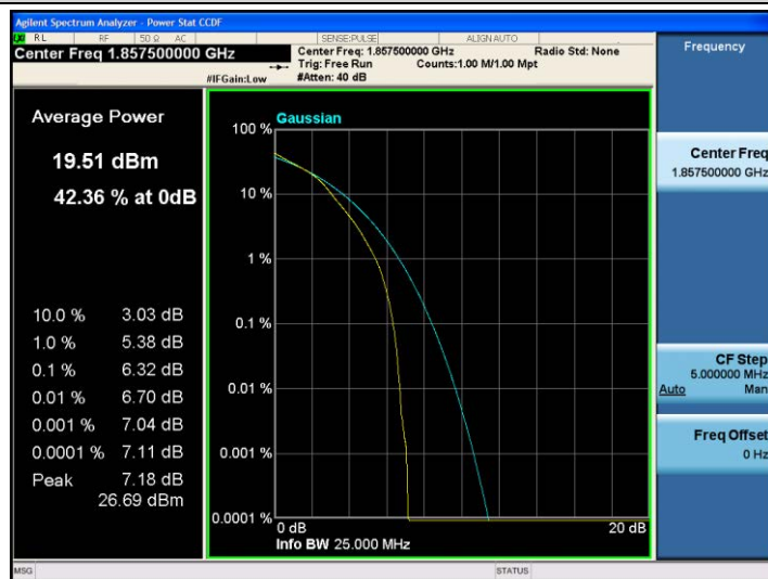
Band2-15MHz-16QAM-18675-75RB#0
