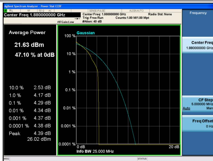
Band2-15MHz-QPSK-18900-1RB#0
