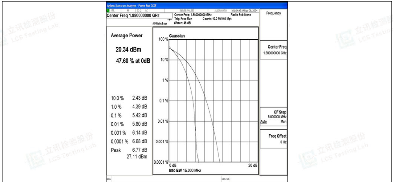
Band2-15MHz-QPSK-18900-75RB#0-PASS
