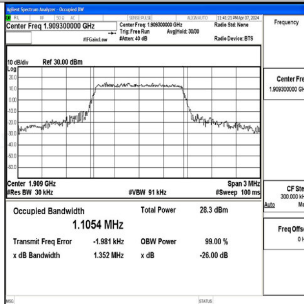
Band2-1.4MHz-64QAM-19193-6RB#0-PASS
