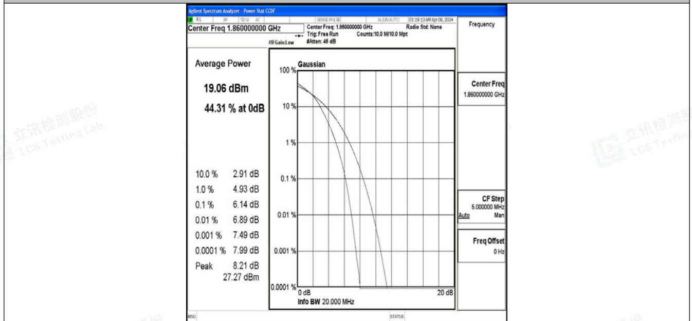
Band2-20MHz-64QAM-18700-100RB#0-PASS
