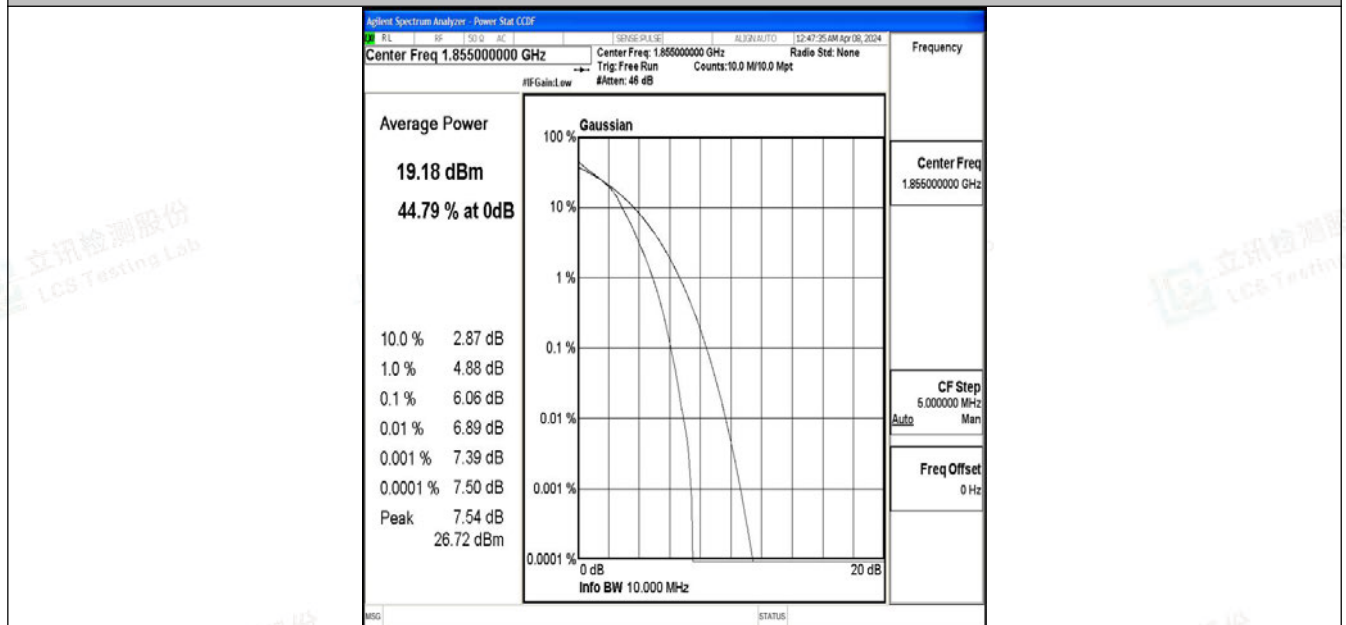
Band2-10MHz-64QAM-18650-50RB#0-PASS
