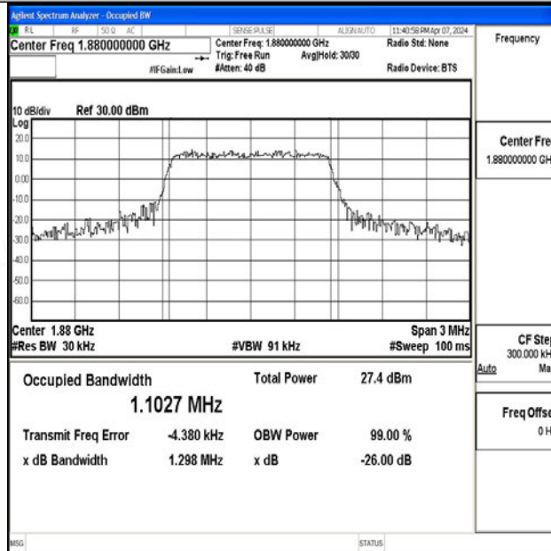
Band2-1.4MHz-64QAM-18900-6RB#0-PASS
