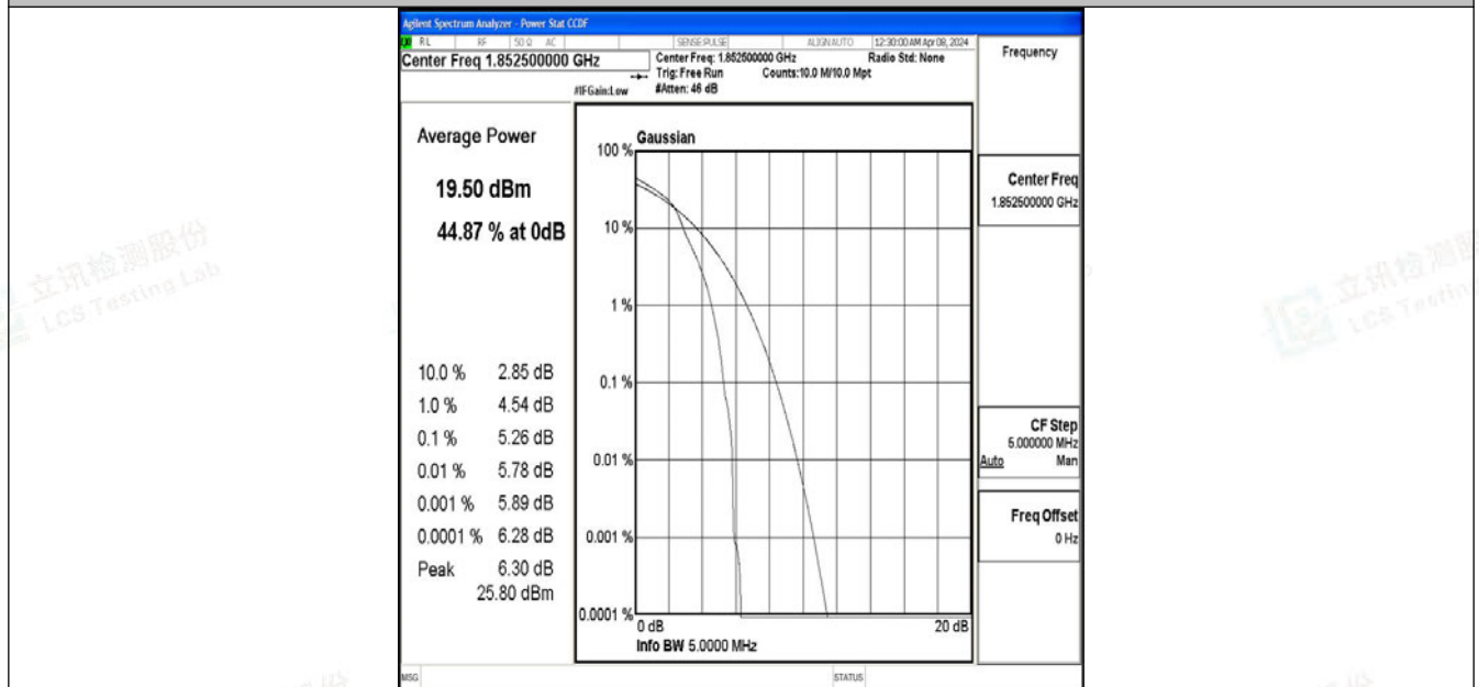
Band2-5MHz-64QAM-18625-1RB#0-PASS
