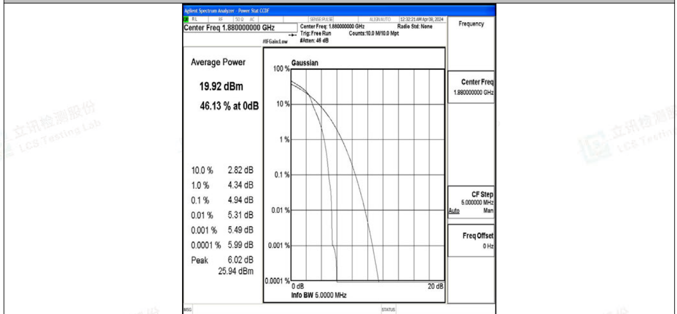
Band2-5MHz-64QAM-18900-1RB#0-PASS
