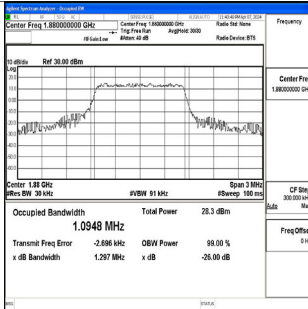
Band2-1.4MHz-QPSK-18900-6RB#0-PASS
