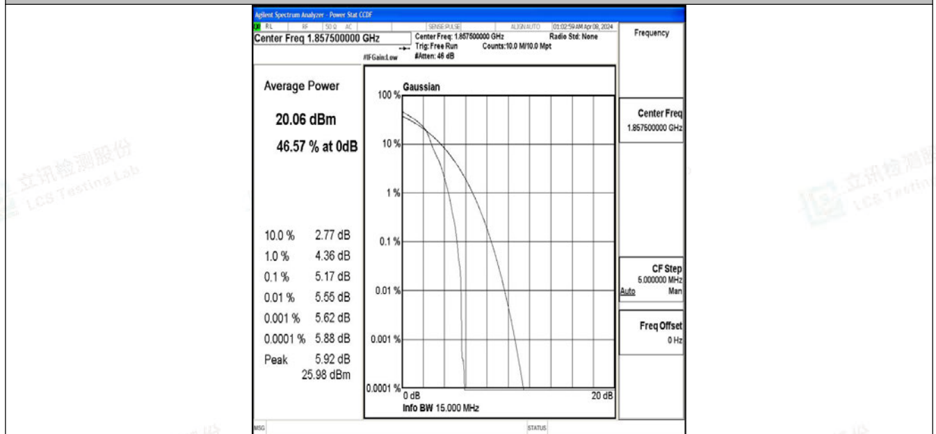
Band2-15MHz-64QAM-18675-1RB#0-PASS
