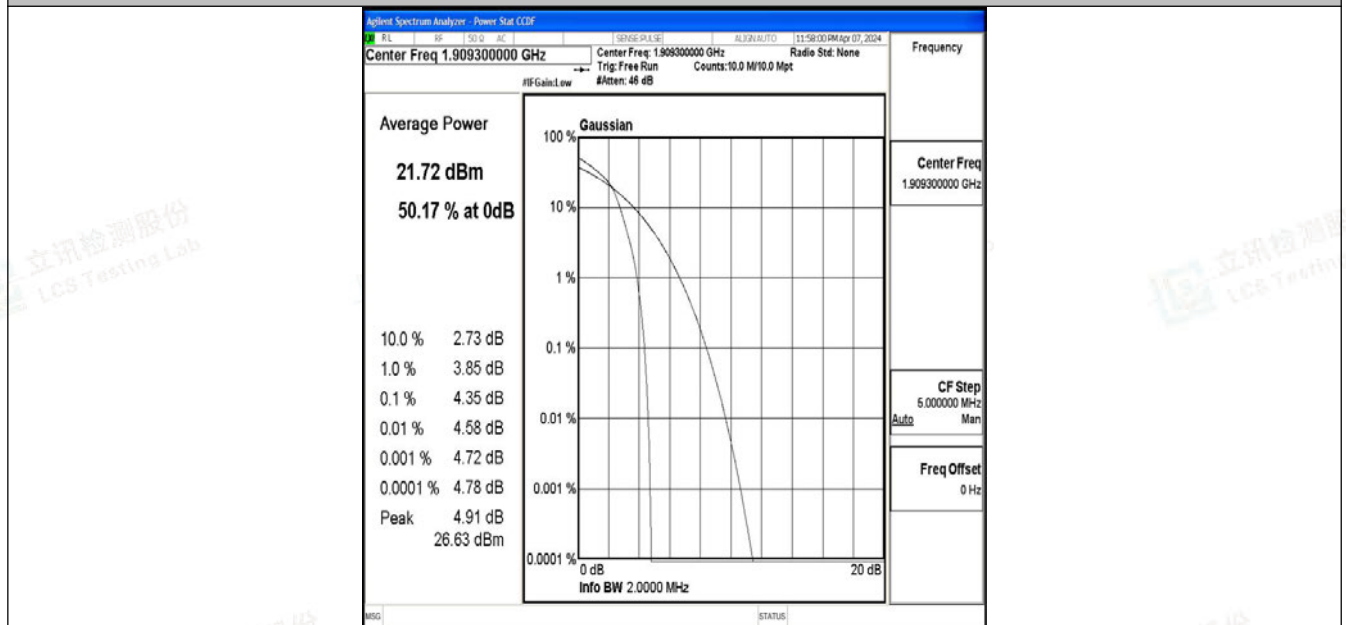
Band2-1.4MHz-64QAM-19193-1RB#0-PASS
