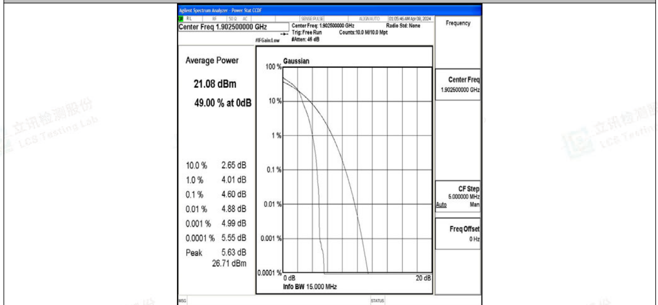
Band2-15MHz-64QAM-19125-1RB#0-PASS
