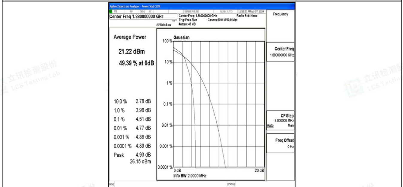
Band2-1.4MHz-64QAM-18900-1RB#0-PASS
