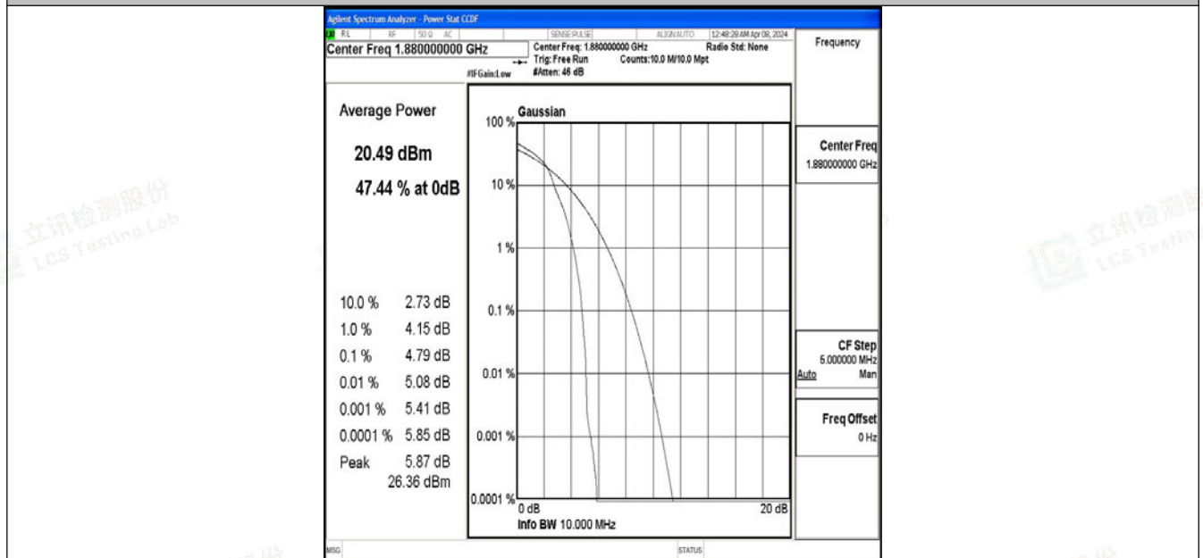
Band2-10MHz-64QAM-18900-1RB#0-PASS
