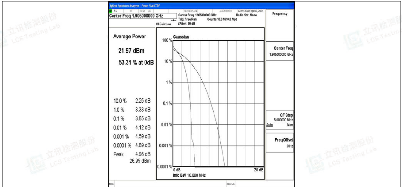
Band2-10MHz-QPSK-19150-1RB#0-PASS
