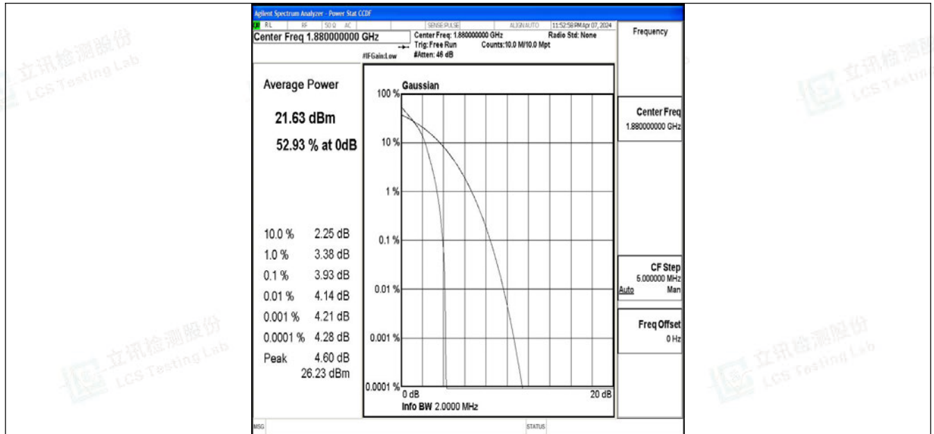
Band2-1.4MHz-QPSK-18900-1RB#0-PASS
