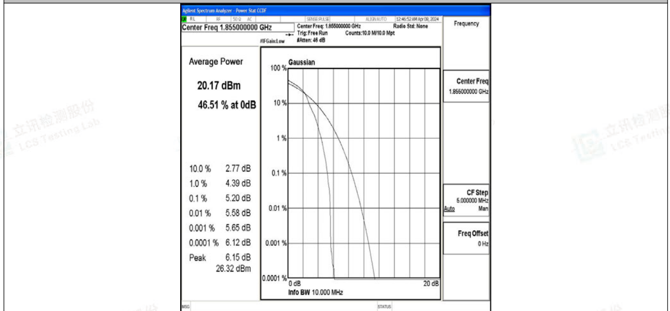
Band2-10MHz-64QAM-18650-1RB#0-PASS
