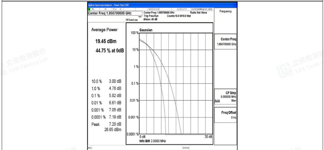
Band2-1.4MHz-64QAM-18607-6RB#0-PASS
