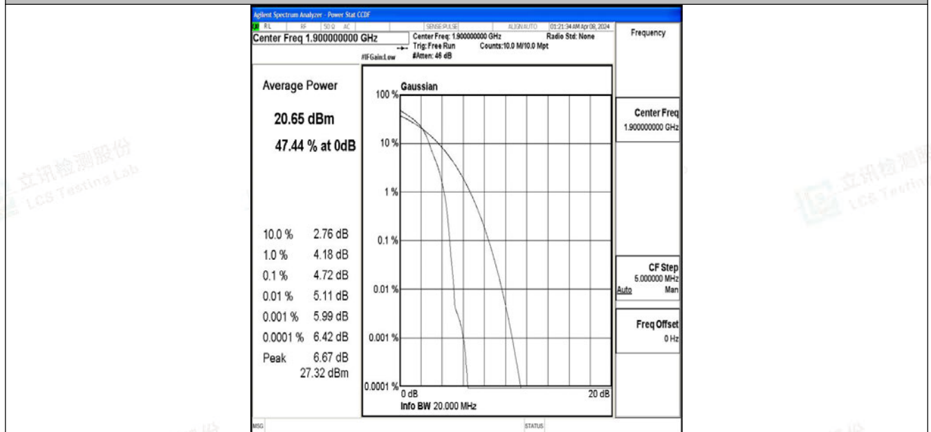
Band2-20MHz-64QAM-19100-1RB#0-PASS
