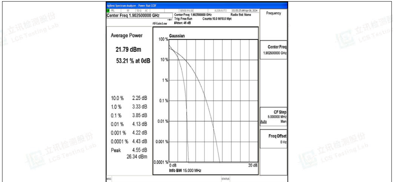
Band2-15MHz-QPSK-19125-1RB#0-PASS
