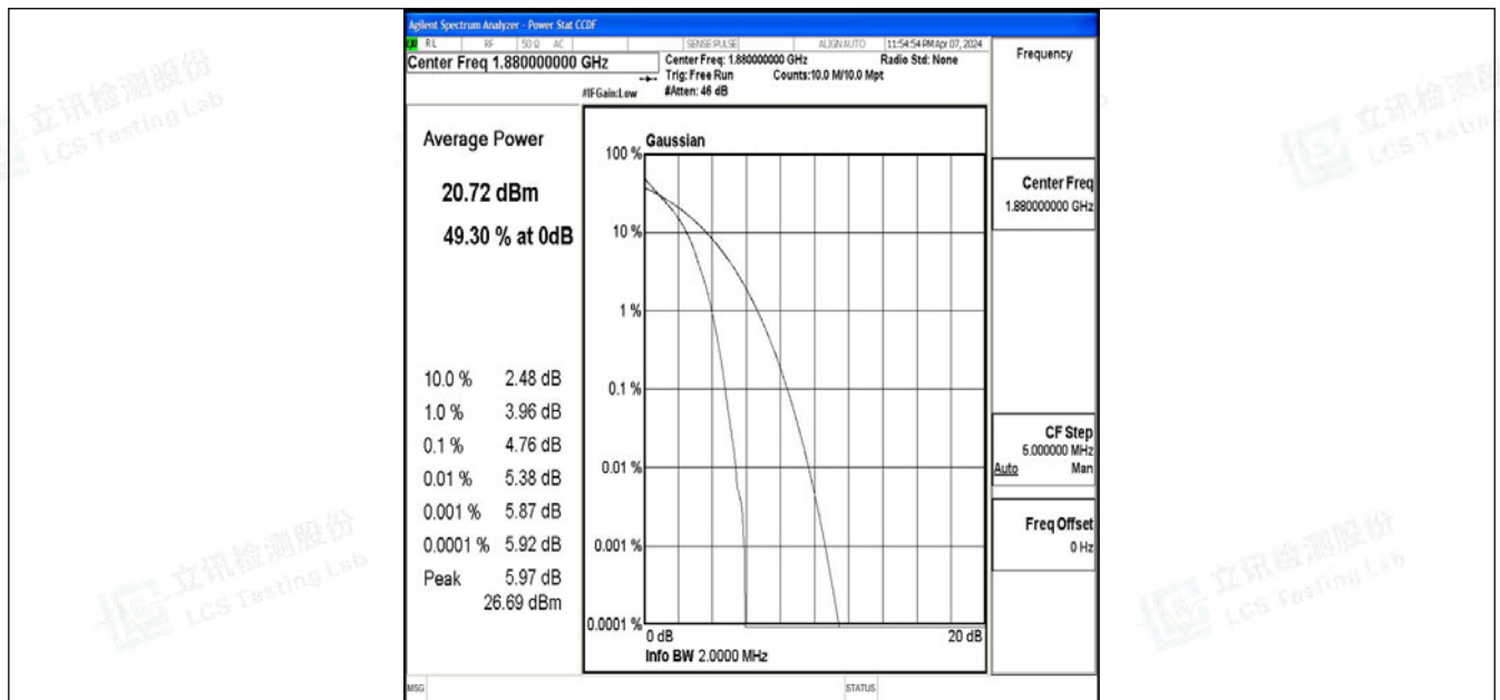
Band2-1.4MHz-QPSK-18900-6RB#0-PASS
