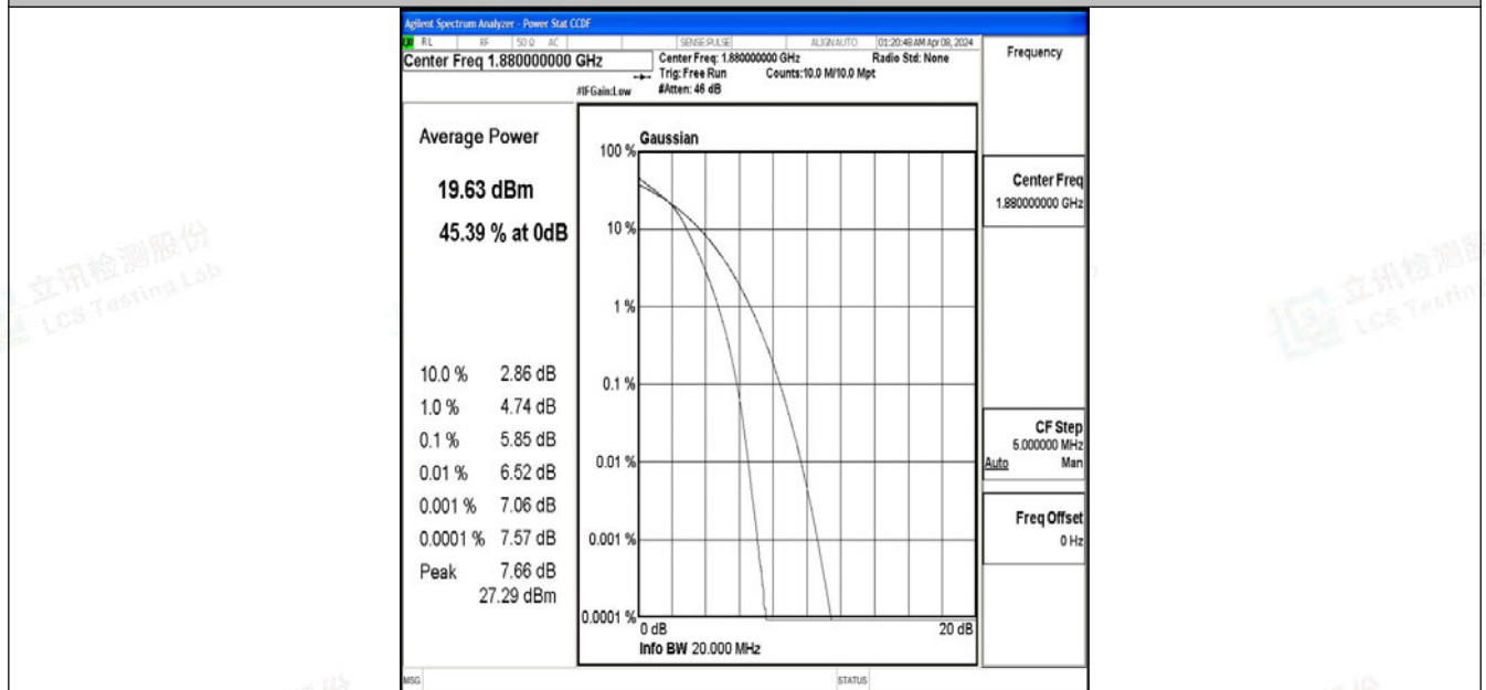
Band2-20MHz-64QAM-18900-100RB#0-PASS
