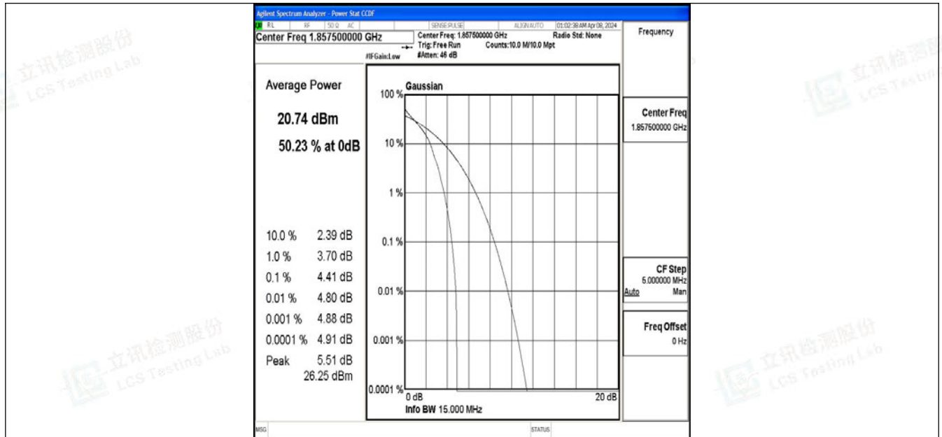
Band2-15MHz-QPSK-18675-1RB#0-PASS
