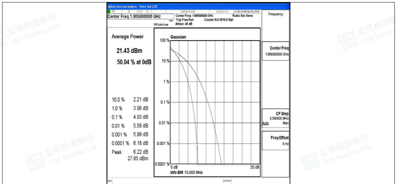
Band2-10MHz-QPSK-19150-50RB#0-PASS
