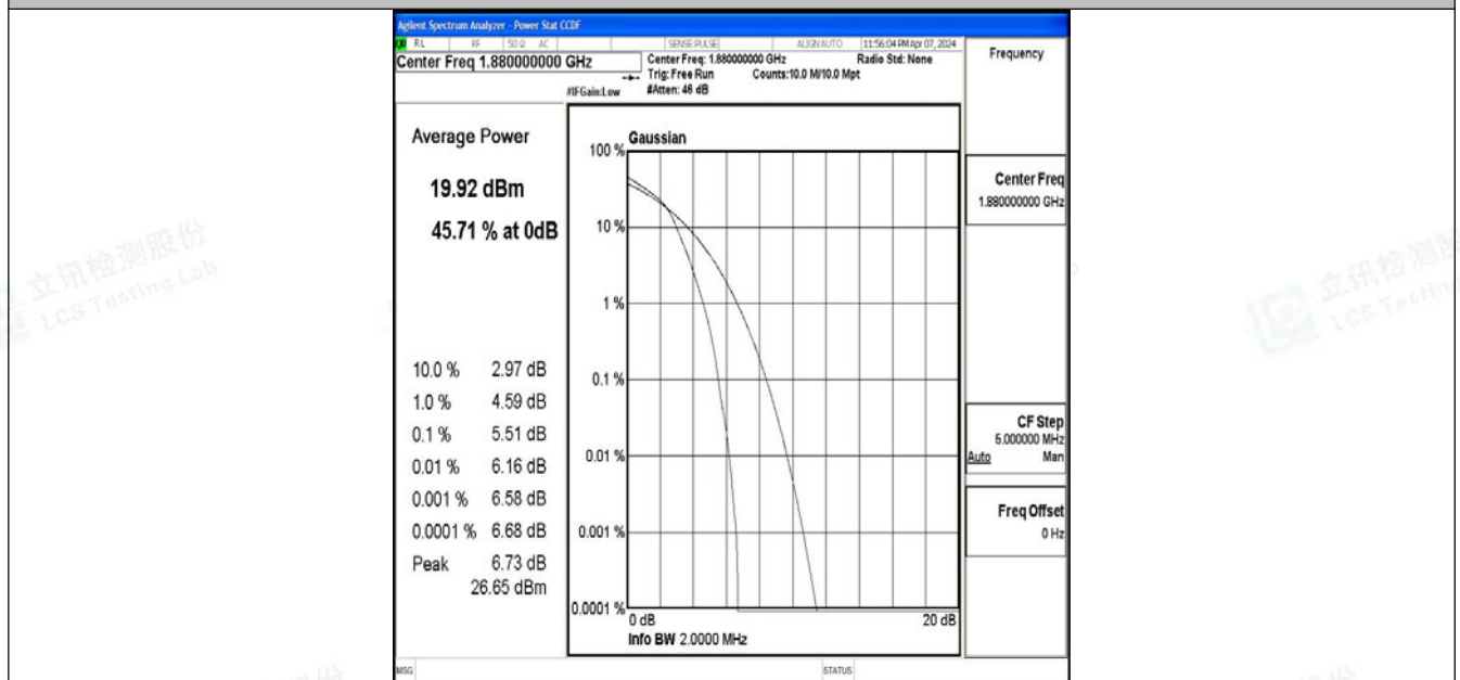
Band2-1.4MHz-64QAM-18900-6RB#0-PASS
