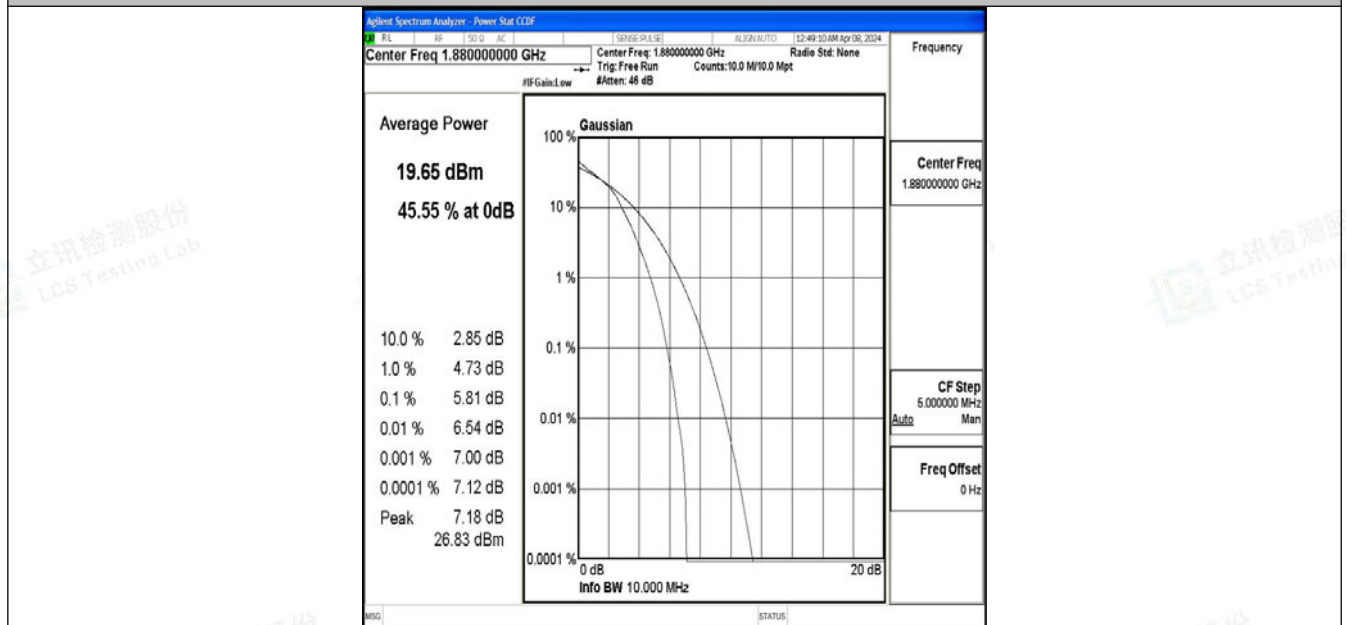
Band2-10MHz-64QAM-18900-50RB#0-PASS
