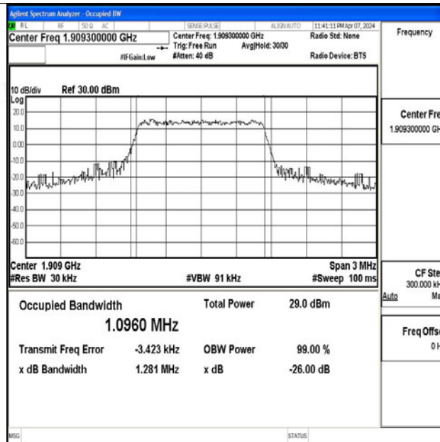
Band2-1.4MHz-QPSK-19193-6RB#0-PASS
