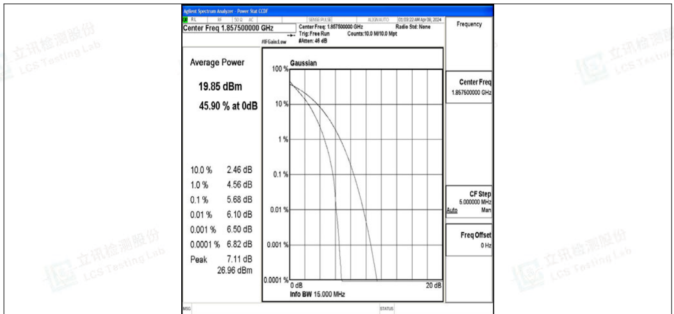
Band2-15MHz-QPSK-18675-75RB#0-PASS
