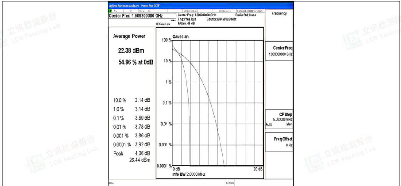
Band2-1.4MHz-QPSK-19193-1RB#0-PASS
