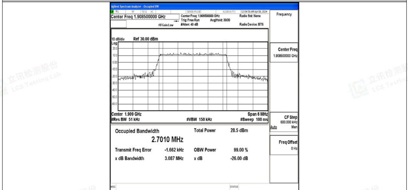
Band2-3MHz-64QAM-19185-15RB#0-PASS
