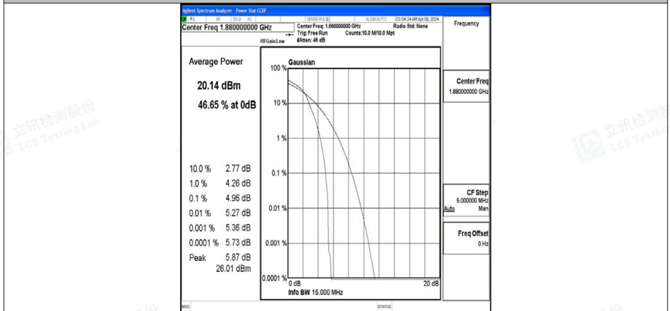
Band2-15MHz-64QAM-18900-1RB#0-PASS
