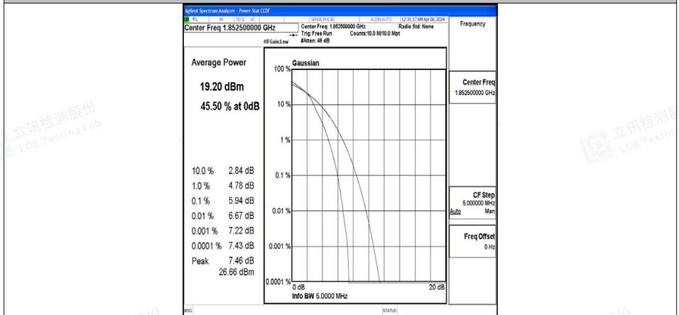
Band2-5MHz-64QAM-18625-25RB#0-PASS
