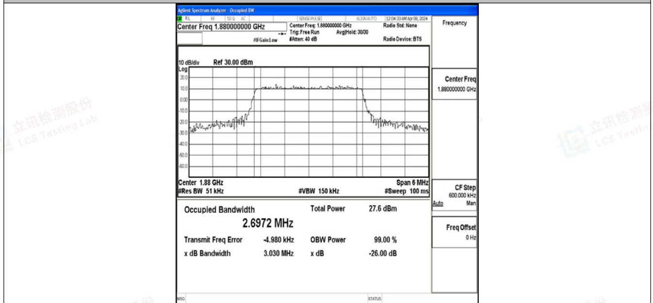
Band2-3MHz-64QAM-18900-15RB#0-PASS
