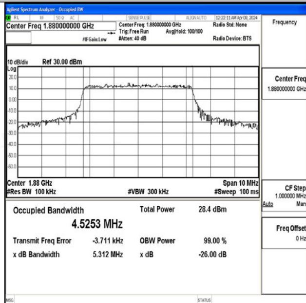
Band2-5MHz-64QAM-18900-25RB#0-PASS
