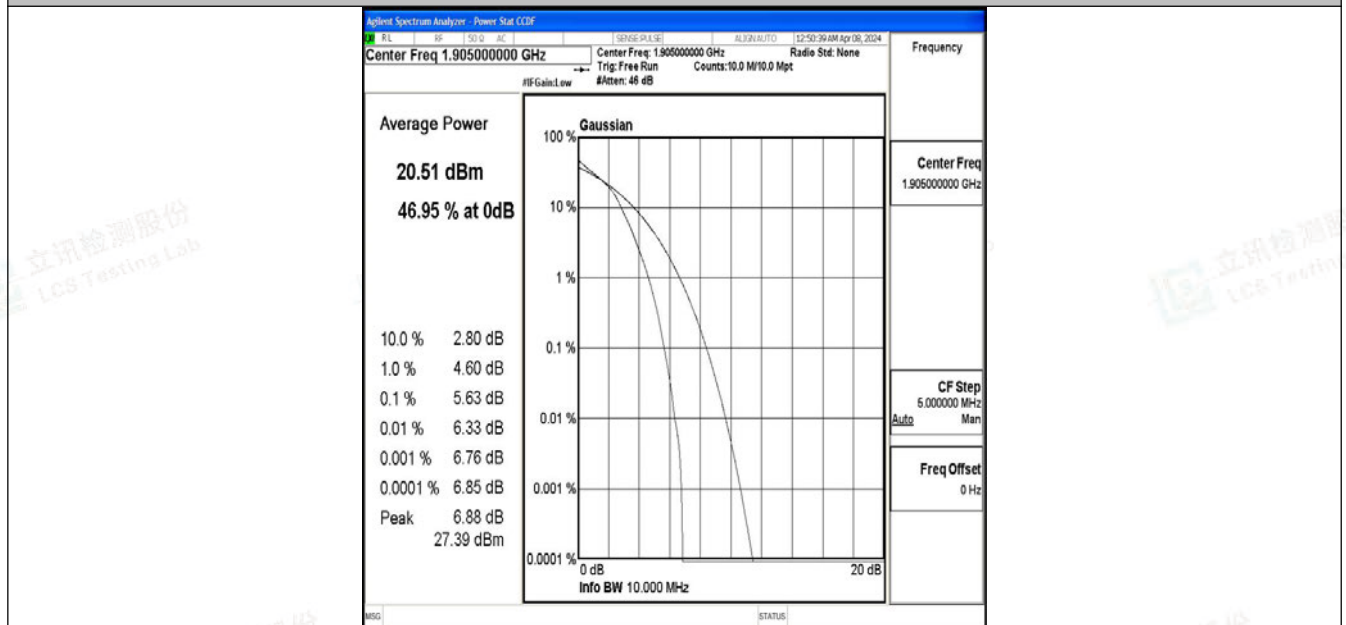
Band2-10MHz-64QAM-19150-50RB#0-PASS
