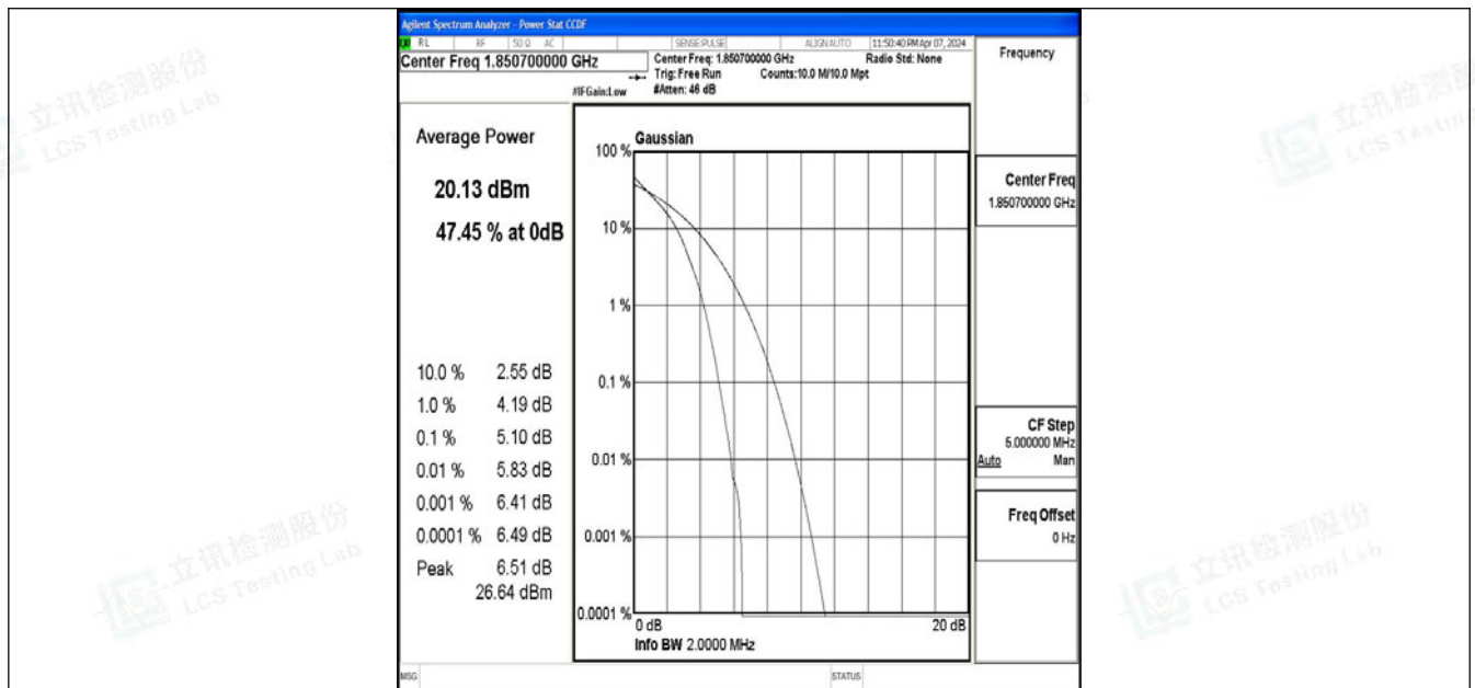
Band2-1.4MHz-QPSK-18607-6RB#0-PASS
