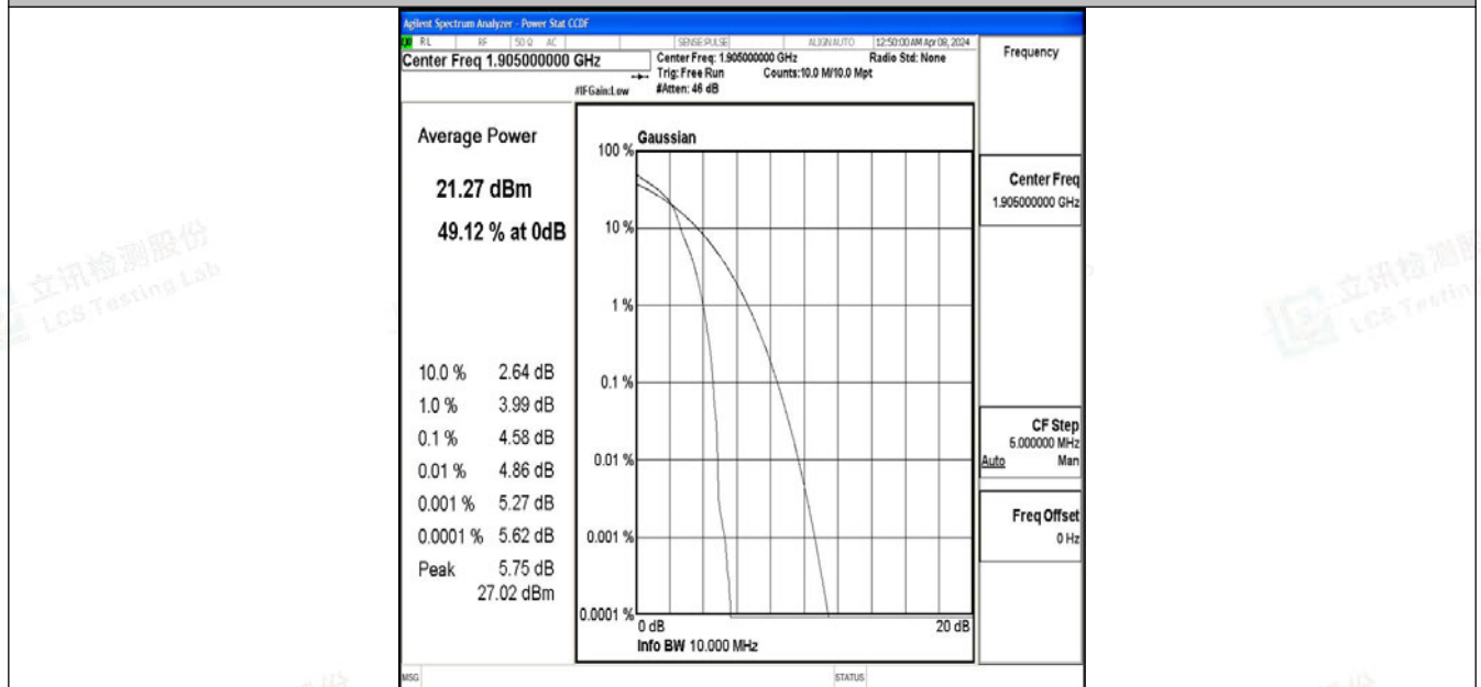
Band2-10MHz-64QAM-19150-1RB#0-PASS
