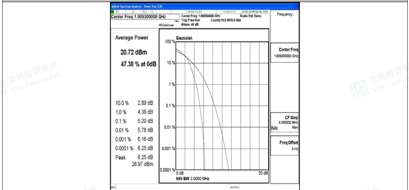
Band2-1.4MHz-64QAM-19193-6RB#0-PASS
