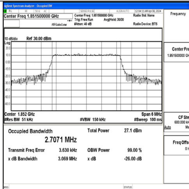
Band2-3MHz-64QAM-18615-15RB#0-PASS
