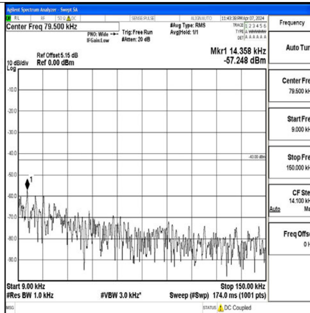
Band2_1.4MHz_64QAM_18900_1RB#0_0.009~0.15_0.009~0.15
