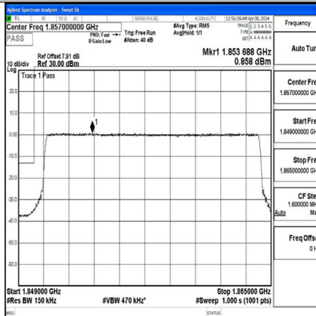
Band2_15MHz_64QAM_18675_75RB#0
