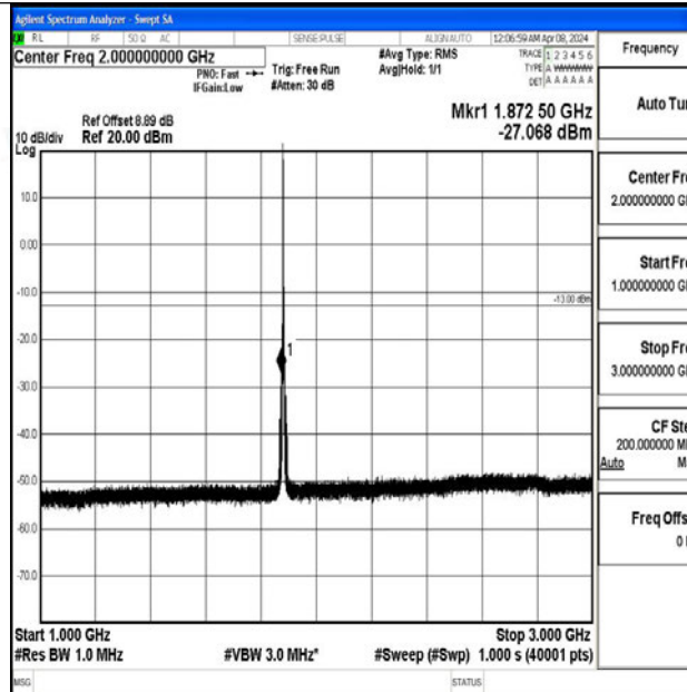
Band2_3MHz_QPSK_18900_1RB#0_1000~3000_1000~3000
