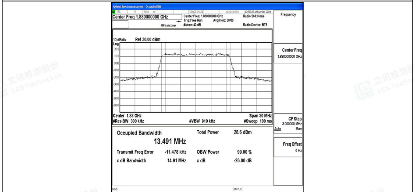
Band2-15MHz-64QAM-18900-75RB#0-PASS
