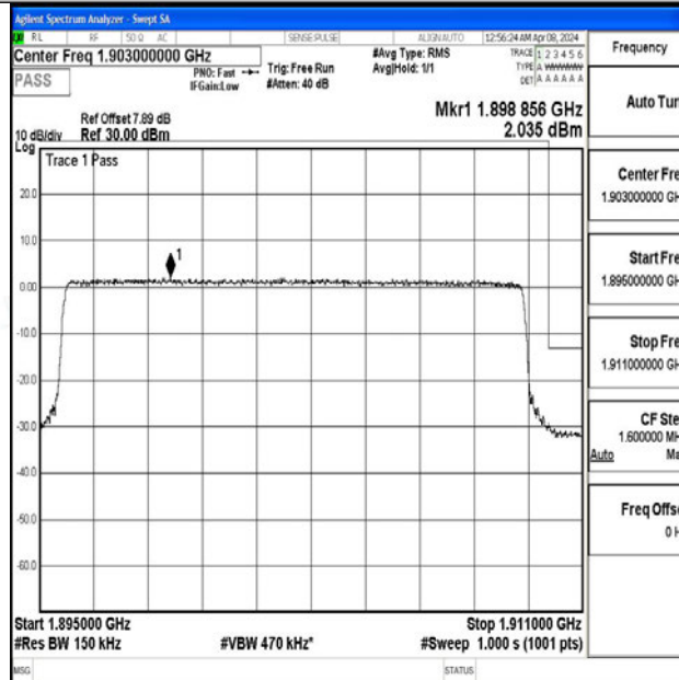
Band2_15MHz_64QAM_19125_75RB#0
