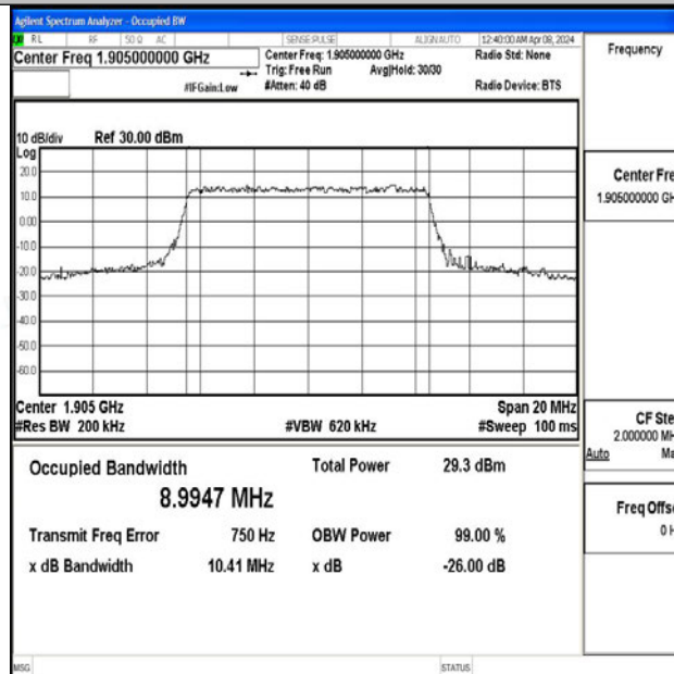
Band2-10MHz-64QAM-19150-50RB#0-PASS
