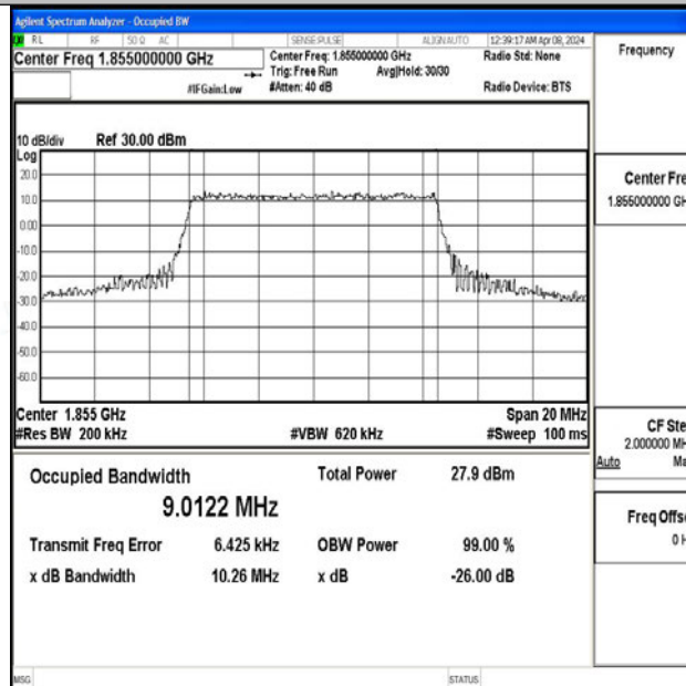
Band2-10MHz-64QAM-18650-50RB#0-PASS
