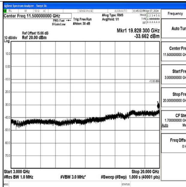
Band2_1.4MHz_64QAM_19193_1RB#0_3000~20000_3000~20000
