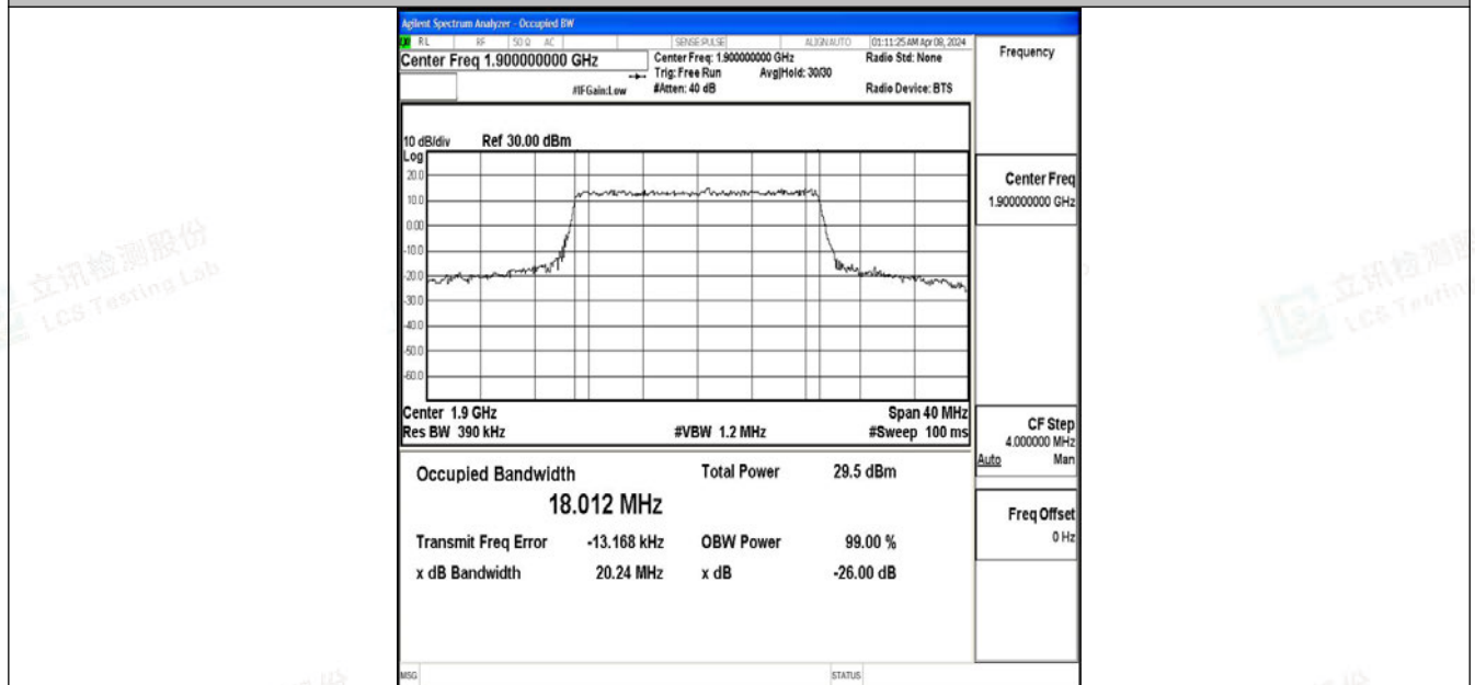
Band2-20MHz-64QAM-19100-100RB#0-PASS
