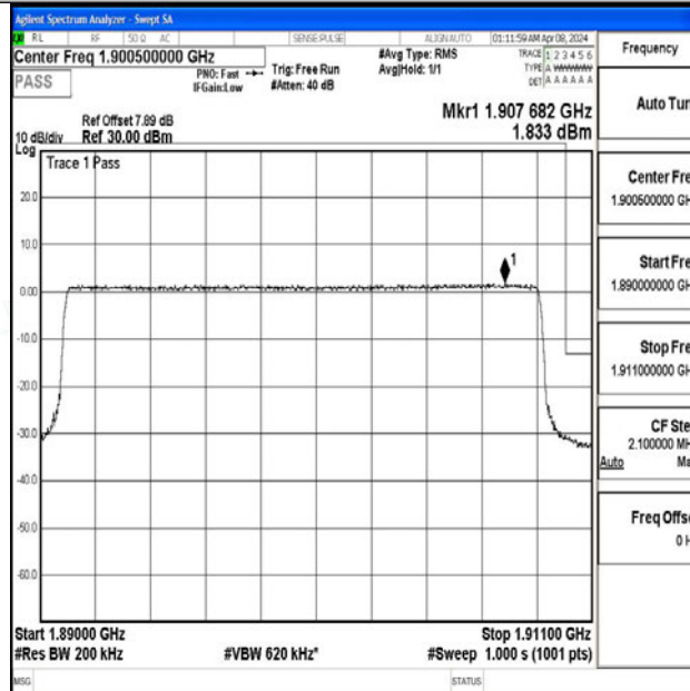
Band2_20MHz_64QAM_19100_100RB#0
