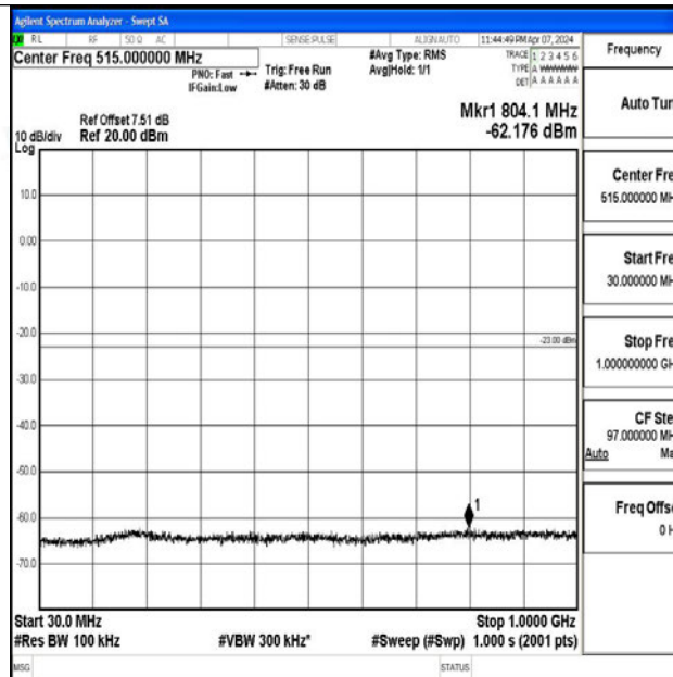
Band2_1.4MHz_64QAM_19193_1RB#0_30~1000_30~1000
