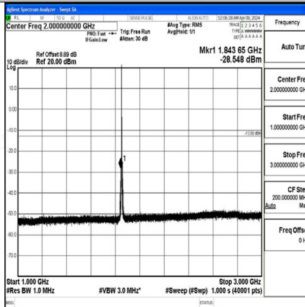
Band2_3MHz_64QAM_18615_1RB#0_1000~3000_1000~3000
