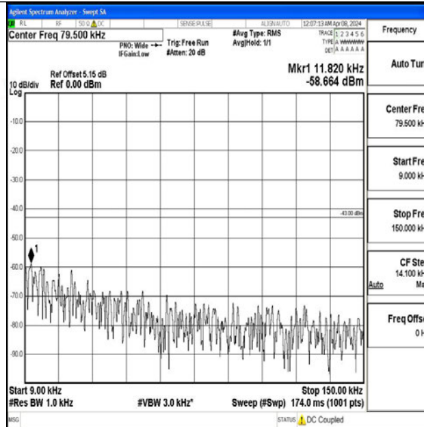
Band2_3MHz_64QAM_18900_1RB#0_0.009~0.15_0.009~0.15
