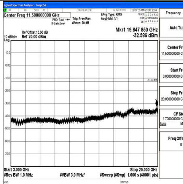
Band2_3MHz_QPSK_18900_1RB#0_3000~20000_3000~20000
