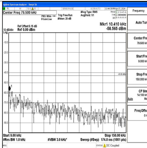
Band2_1.4MHz_64QAM_19193_1RB#0_0.009~0.15_0.009~0.15
