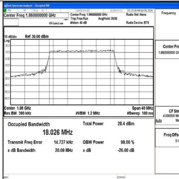
Band2-20MHz-64QAM-18700-100RB#0-PASS
