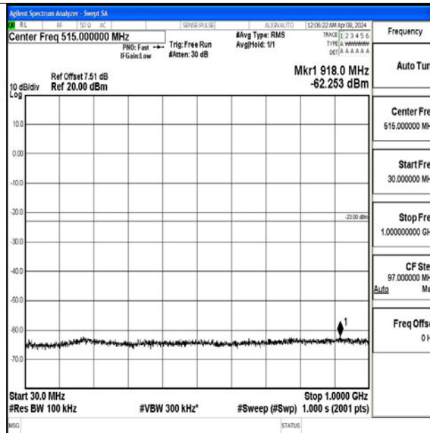
Band2_3MHz_64QAM_18615_1RB#0_30~1000_30~1000
