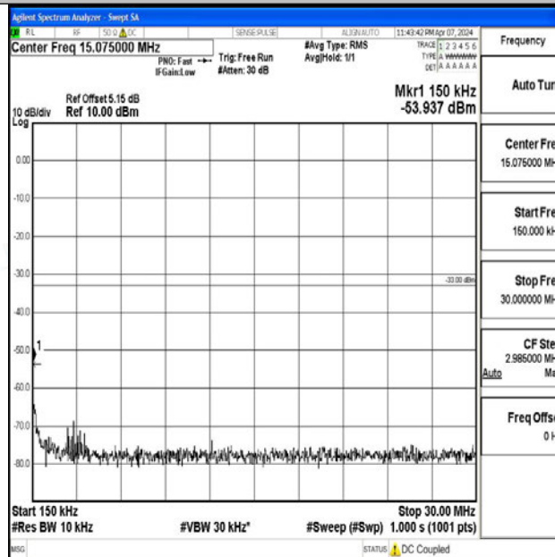
Band2_1.4MHz_64QAM_18900_1RB#0_0.15~30_0.15~30
