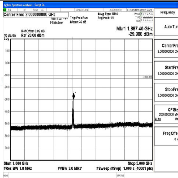
Band2_1.4MHz_64QAM_18900_1RB#0_1000~3000_1000~3000
