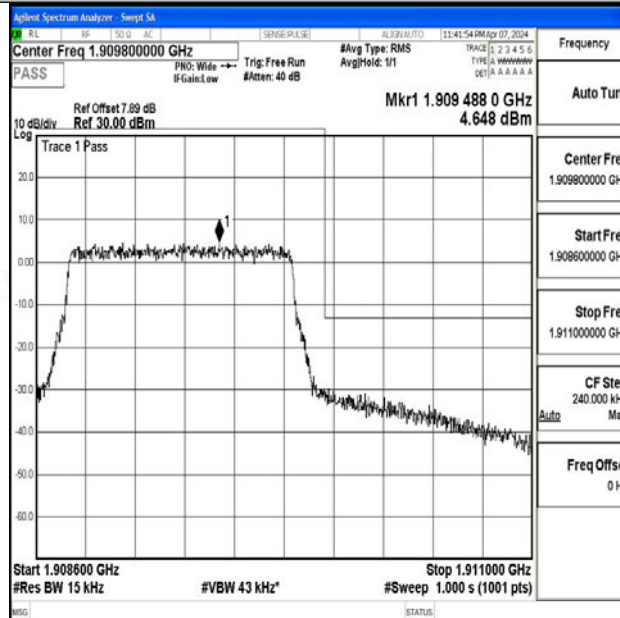
Band2_1.4MHz_64QAM_19193_6RB#0
