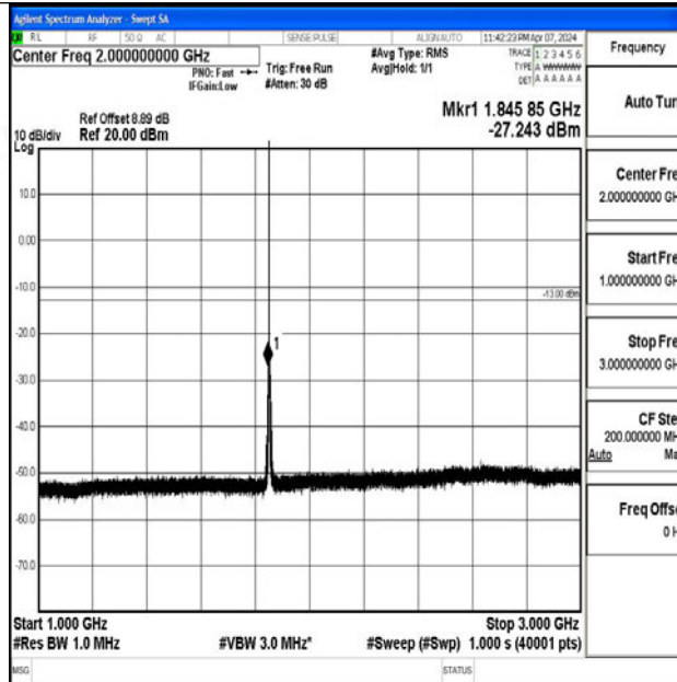
Band2_1.4MHz_QPSK_18607_1RB#0_1000~3000_1000~3000
