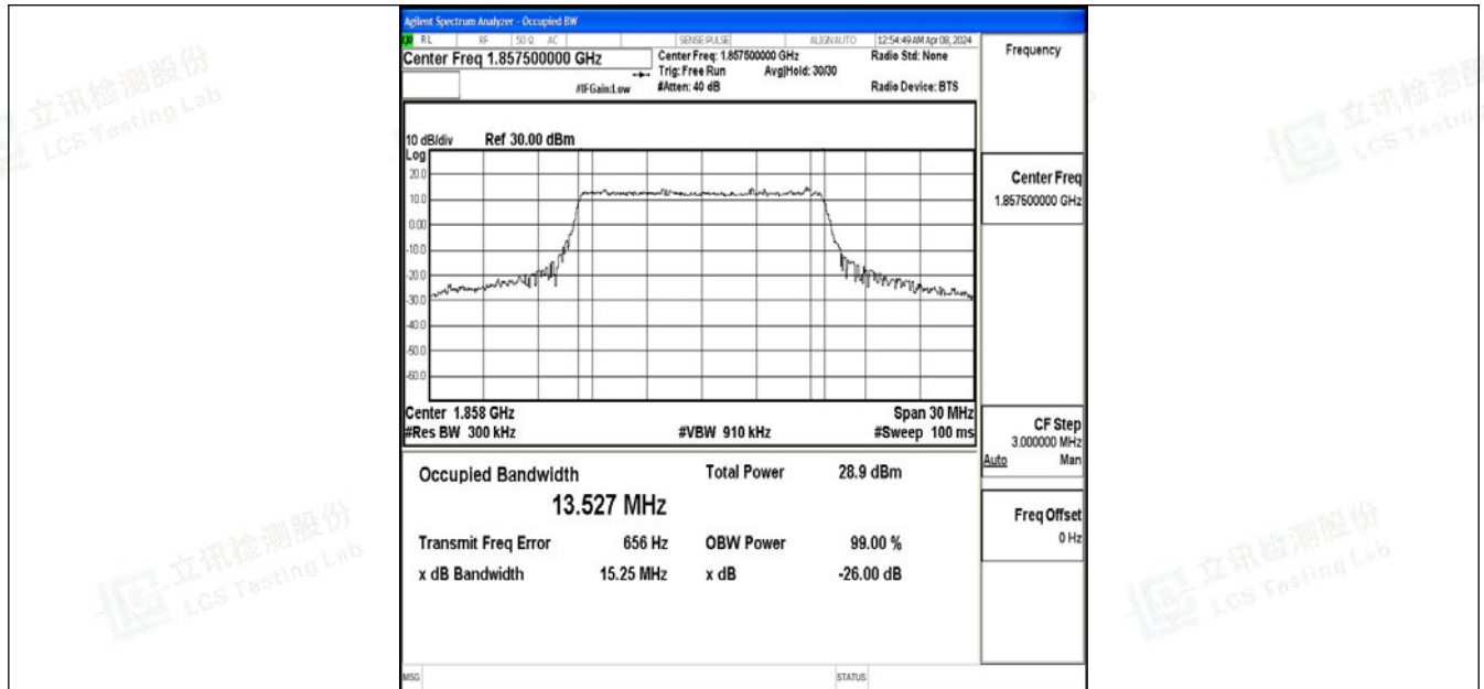
Band2-15MHz-QPSK-18675-75RB#0-PASS
