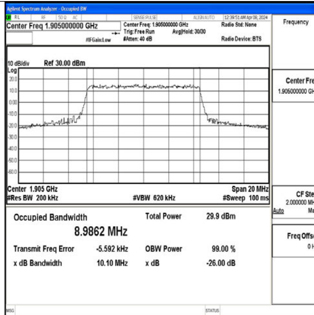
Band2-10MHz-QPSK-19150-50RB#0-PASS
