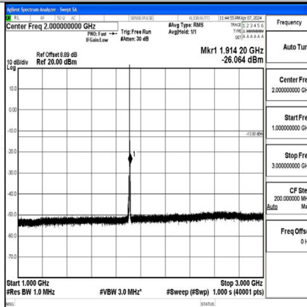
Band2_1.4MHz_64QAM_19193_1RB#0_1000~3000_1000~3000
