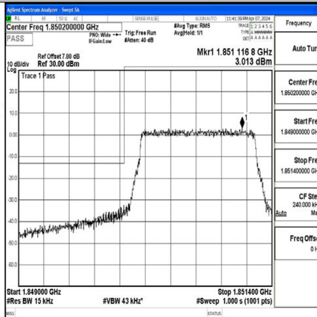
Band2_1.4MHz_64QAM_18607_6RB#0
