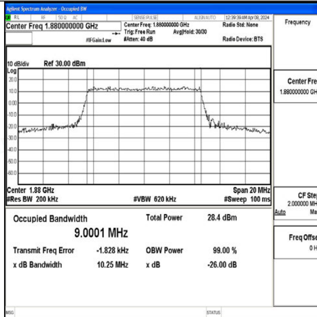
Band2-10MHz-64QAM-18900-50RB#0-PASS
