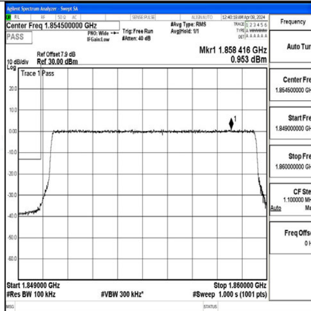
Band2_10MHz_64QAM_18650_50RB#0
