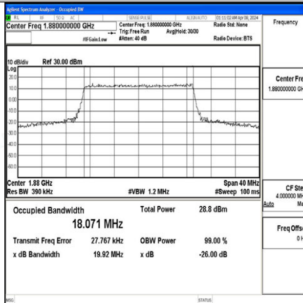
Band2-20MHz-64QAM-18900-100RB#0-PASS
