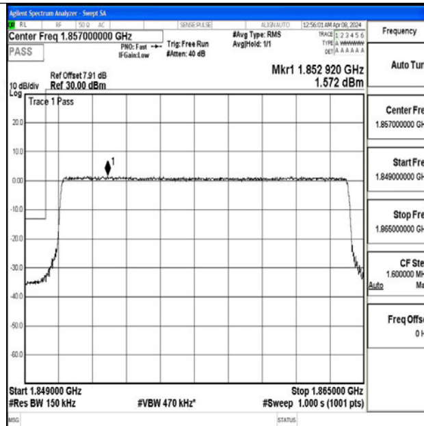
Band2_15MHz_QPSK_18675_75RB#0
