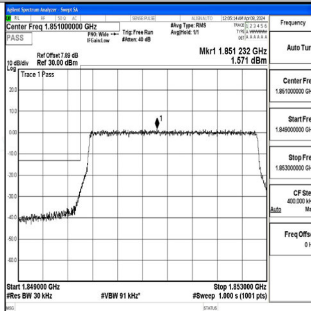
Band2_3MHz_64QAM_18615_15RB#0
