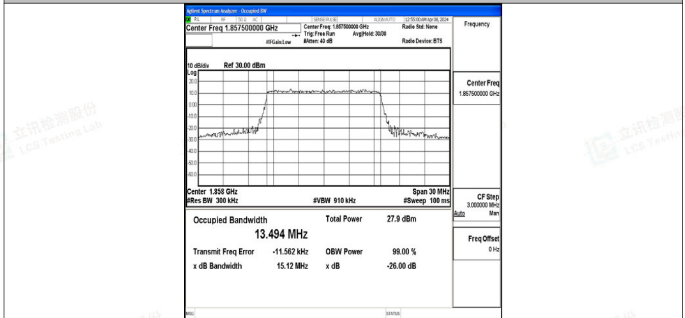
Band2-15MHz-64QAM-18675-75RB#0-PASS
