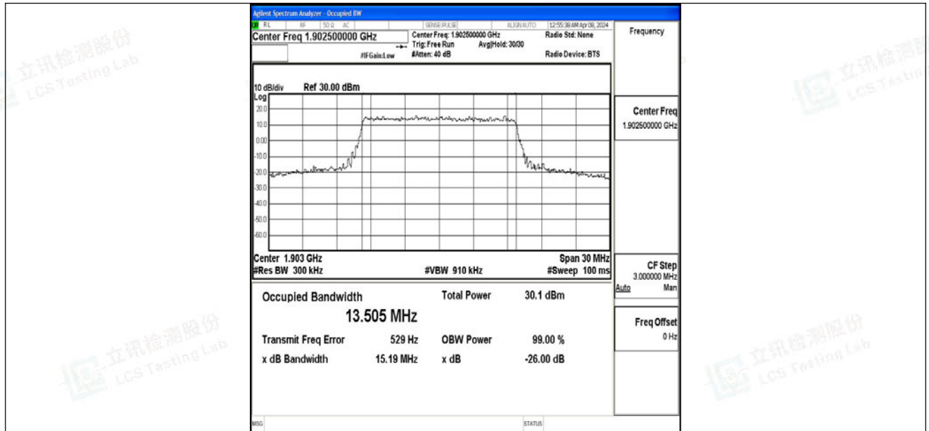
Band2-15MHz-QPSK-19125-75RB#0-PASS
