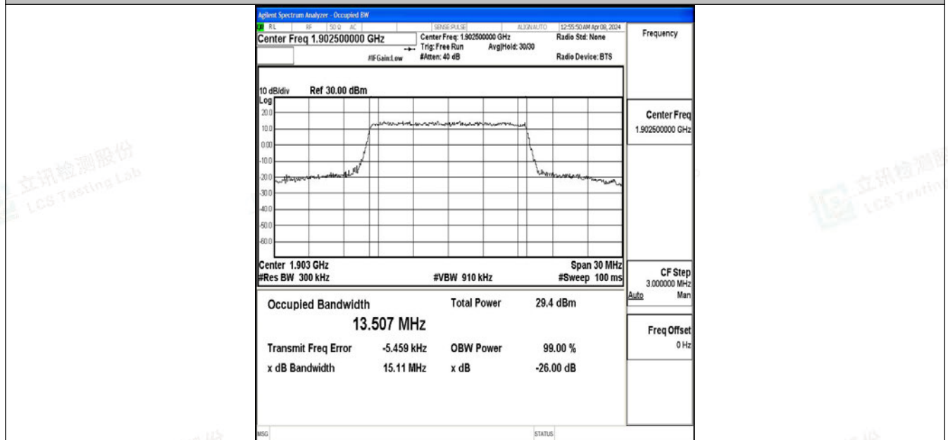
Band2-15MHz-64QAM-19125-75RB#0-PASS
