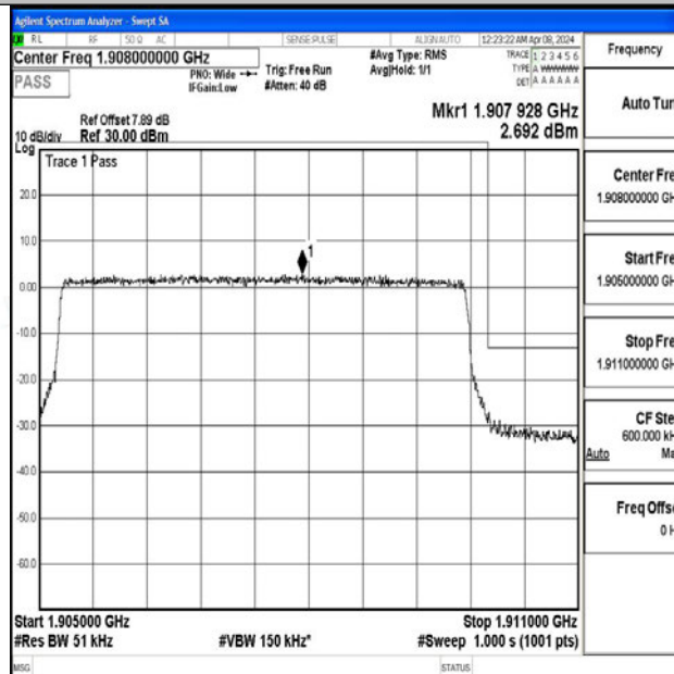
Band2_5MHz_64QAM_19175_25RB#0
