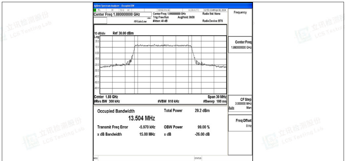
Band2-15MHz-QPSK-18900-75RB#0-PASS
