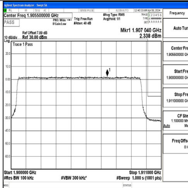
Band2_10MHz_64QAM_19150_50RB#0
