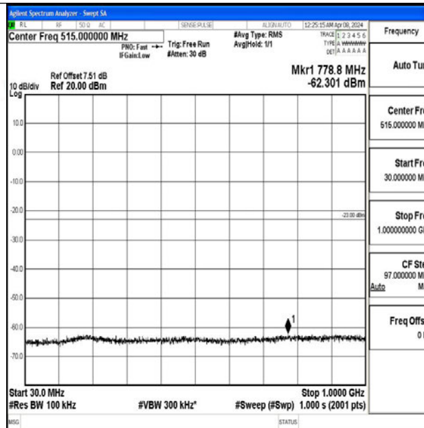
Band2_5MHz_64QAM_18900_1RB#0_30~1000_30~1000
