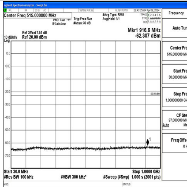
Band2_10MHz_64QAM_19150_1RB#0_30~1000_30~1000
