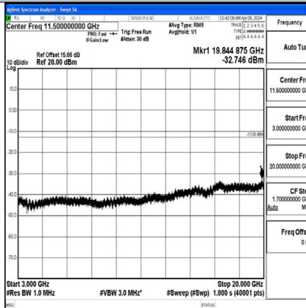
Band2_10MHz_QPSK_18900_1RB#0_3000~20000_3000~20000
