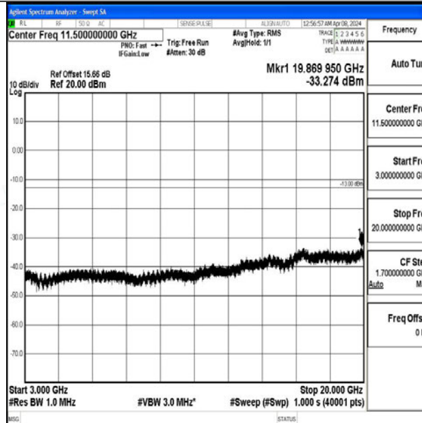
Band2_15MHz_QPSK_18675_1RB#0_3000~20000_3000~20000
