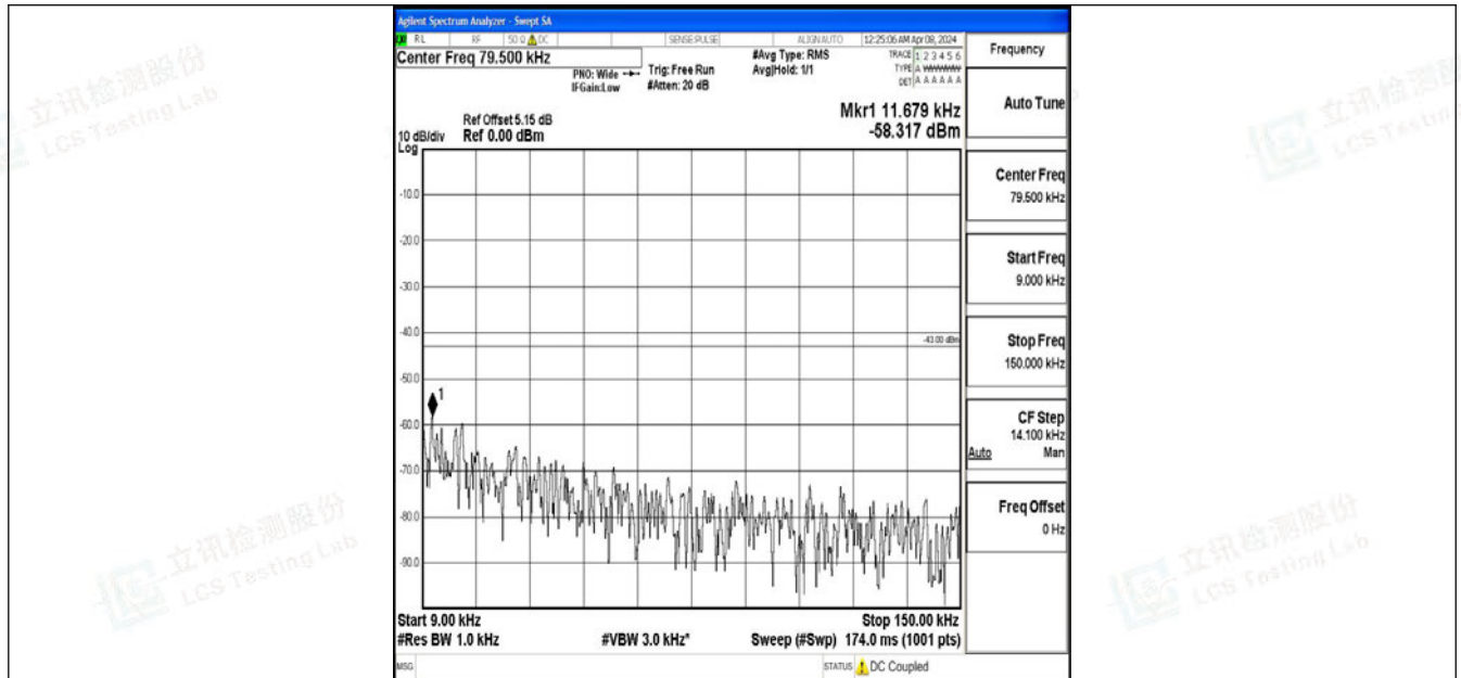
Band2_5MHz_64QAM_18900_1RB#0_0.009~0.15_0.009~0.15
