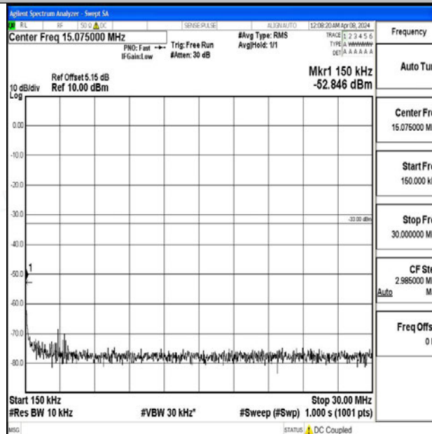
Band2_3MHz_64QAM_19185_1RB#0_0.15~30_0.15~30
