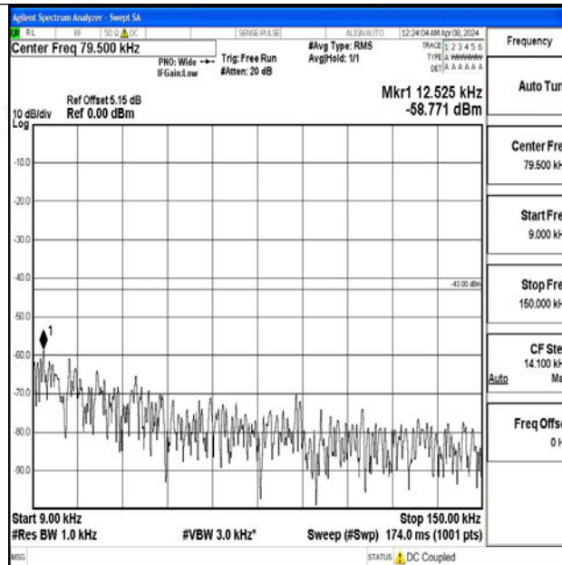
Band2_5MHz_64QAM_18625_1RB#0_0.009~0.15_0.009~0.15
