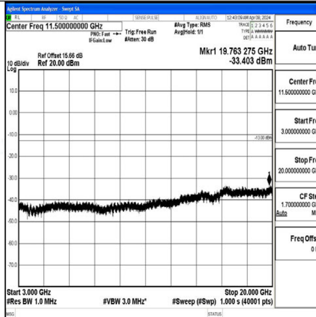
Band2_10MHz_QPSK_19150_1RB#0_3000~20000_3000~20000
