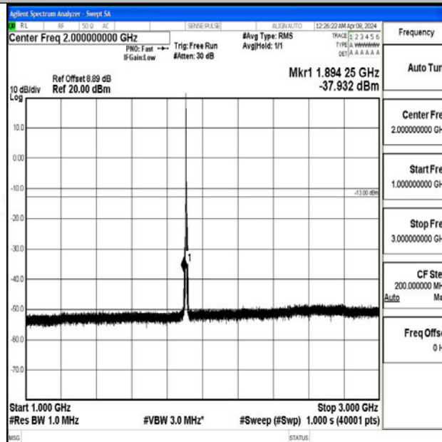
Band2_5MHz_64QAM_19175_1RB#0_1000~3000_1000~3000
