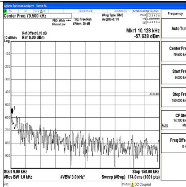
Band2_15MHz_64QAM_18900_1RB#0_0.009~0.15_0.009~0.15
