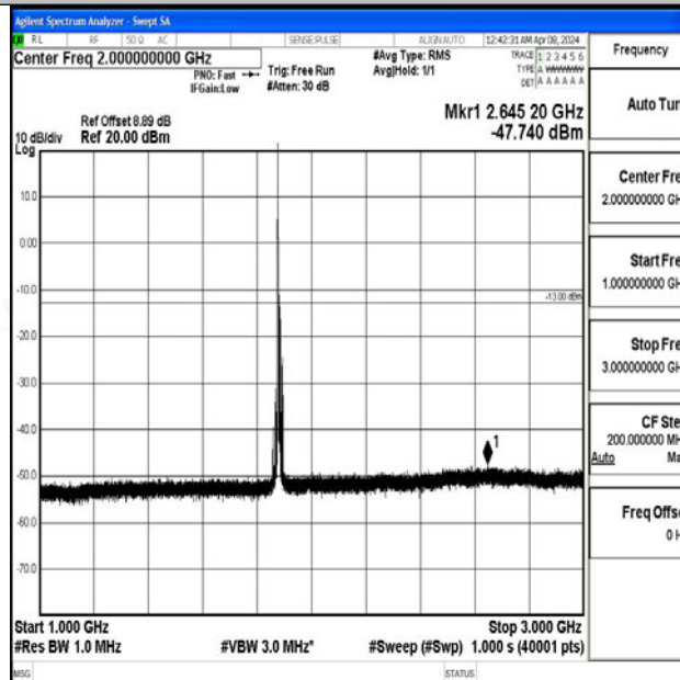
Band2_10MHz_64QAM_18900_1RB#0_1000~3000_1000~3000
