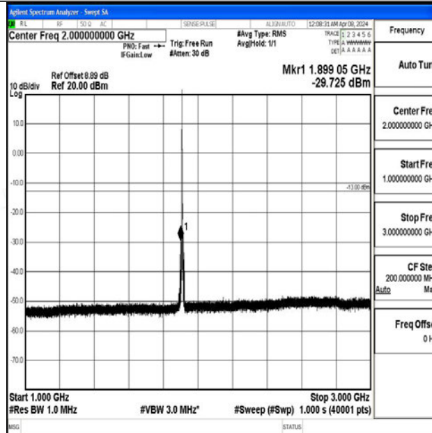
Band2_3MHz_64QAM_19185_1RB#0_1000~3000_1000~3000
