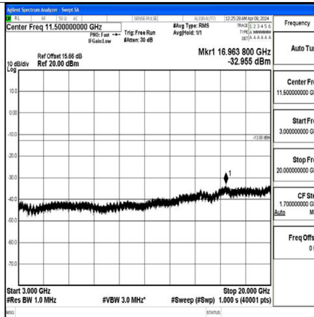
Band2_5MHz_64QAM_18900_1RB#0_3000~20000_3000~20000
