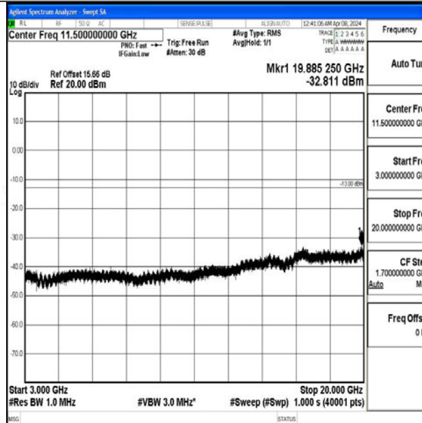
Band2_10MHz_QPSK_18650_1RB#0_3000~20000_3000~20000
