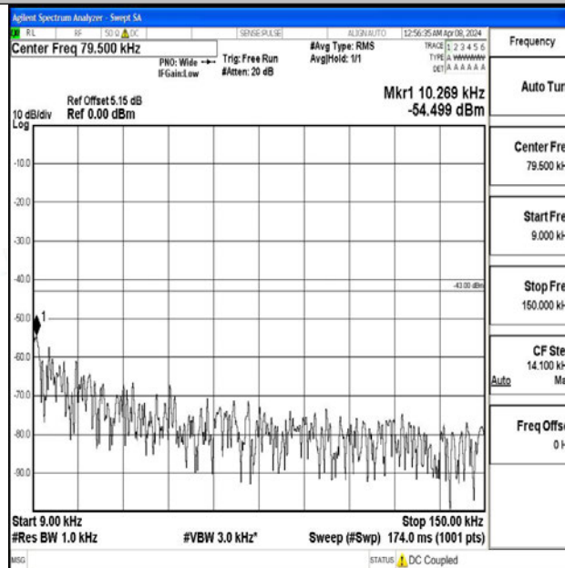
Band2_15MHz_QPSK_18675_1RB#0_0.009~0.15_0.009~0.15
