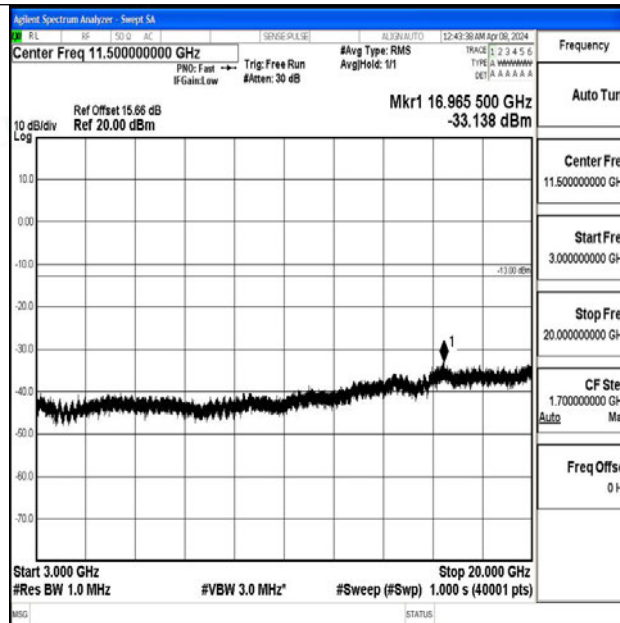
Band2_10MHz_64QAM_19150_1RB#0_3000~20000_3000~20000
