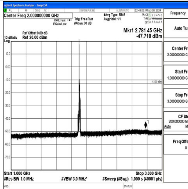
Band2_10MHz_QPSK_19150_1RB#0_1000~3000_1000~3000
