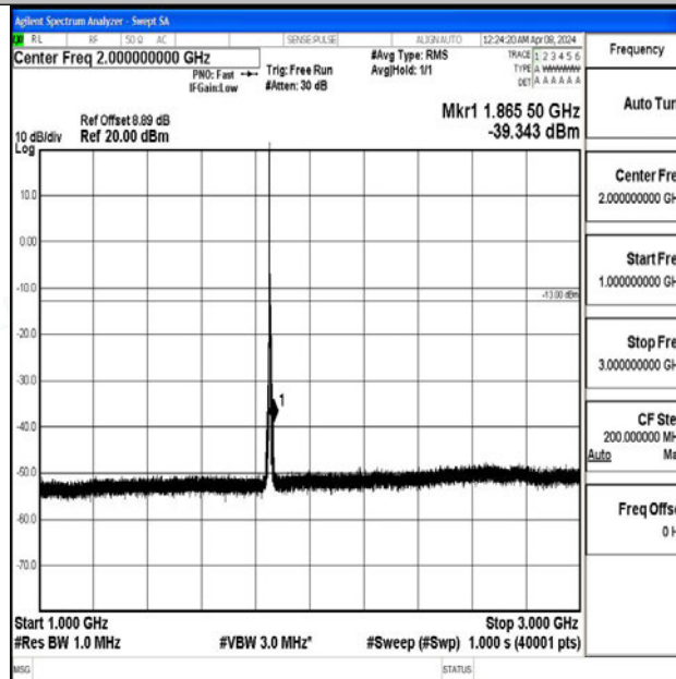
Band2_5MHz_64QAM_18625_1RB#0_1000~3000_1000~3000
