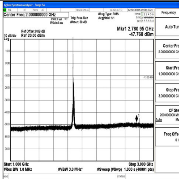
Band2_15MHz_64QAM_18900_1RB#0_1000~3000_1000~3000
