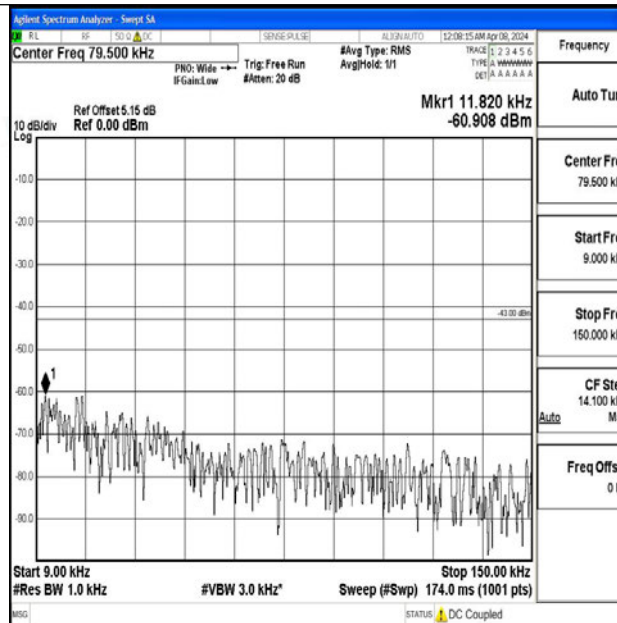
Band2_3MHz_64QAM_19185_1RB#0_0.009~0.15_0.009~0.15
