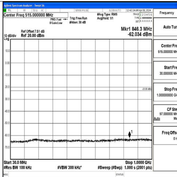
Band2_10MHz_64QAM_18900_1RB#0_30~1000_30~1000
