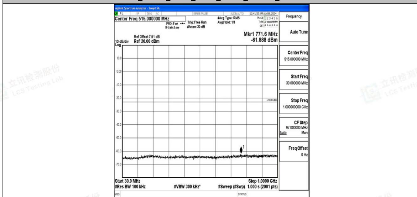
Band2 10MHz QPSK 18900 1RB#0 30~1000 30~1000
