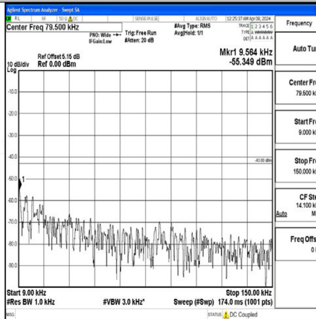
Band2_5MHz_QPSK_19175_1RB#0_0.009~0.15_0.009~0.15
