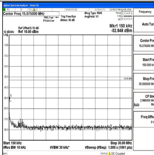
Band2_15MHz_64QAM_18900_1RB#0_0.15~30_0.15~30
