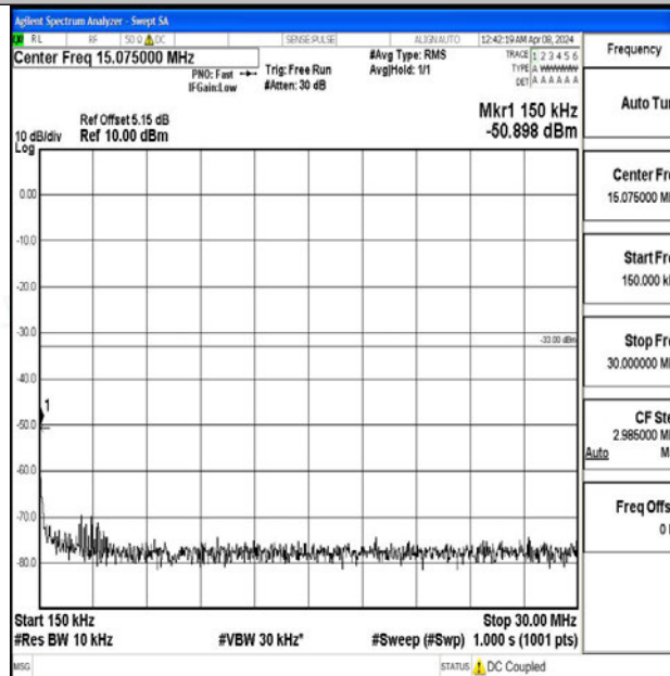
Band2_10MHz_64QAM_18900_1RB#0_0.15~30_0.15~30
