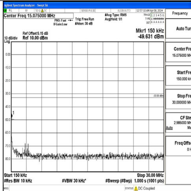
Band2_15MHz_64QAM_18675_1RB#0_0.15~30_0.15~30
