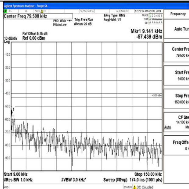
Band2_5MHz_QPSK_18625_1RB#0_0.009~0.15_0.009~0.15
