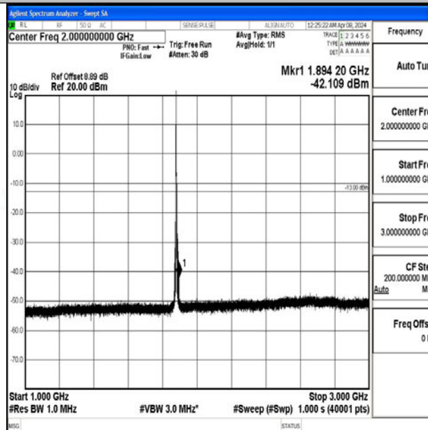
Band2_5MHz_64QAM_18900_1RB#0_1000~3000_1000~3000
