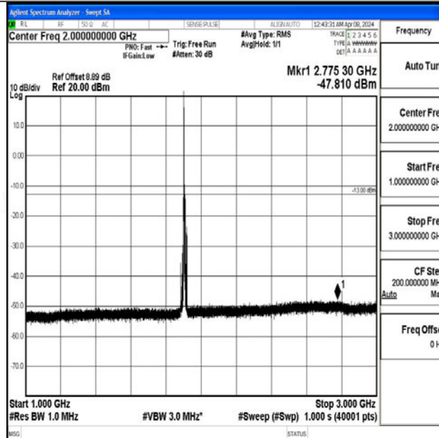
Band2_10MHz_64QAM_19150_1RB#0_1000~3000_1000~3000
