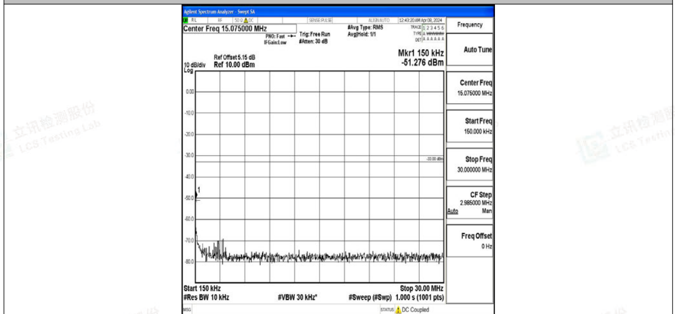
Band2_10MHz_64QAM_19150_1RB#0_0.15~30_0.15~30
