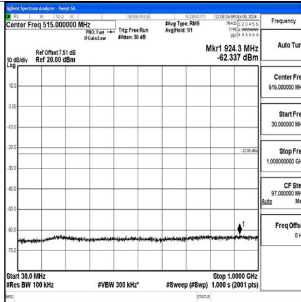
Band2_3MHz_64QAM_19185_1RB#0_30~1000_30~1000
