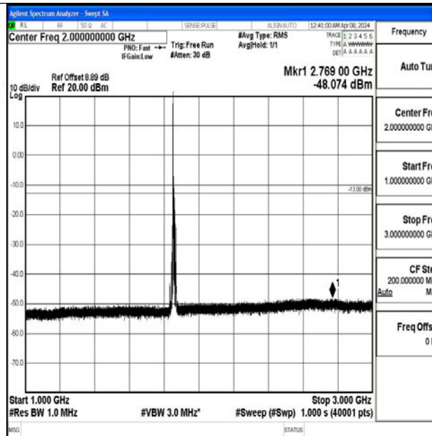
Band2_10MHz_QPSK_18650_1RB#0_1000~3000_1000~3000
