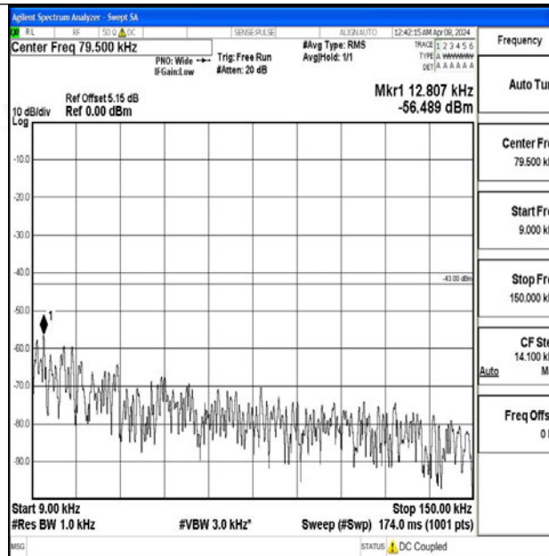
Band2_10MHz_64QAM_18900_1RB#0_0.009~0.15_0.009~0.15
