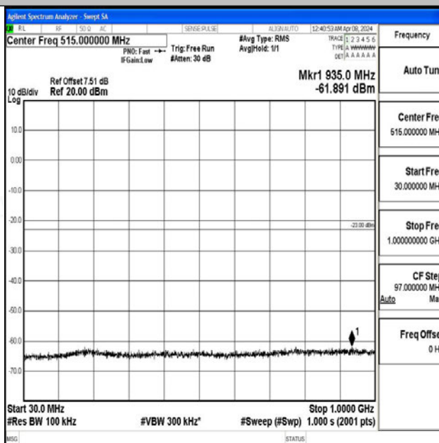
Band2 10MHz QPSK 18650 1RB#0 30~1000 30~1000
