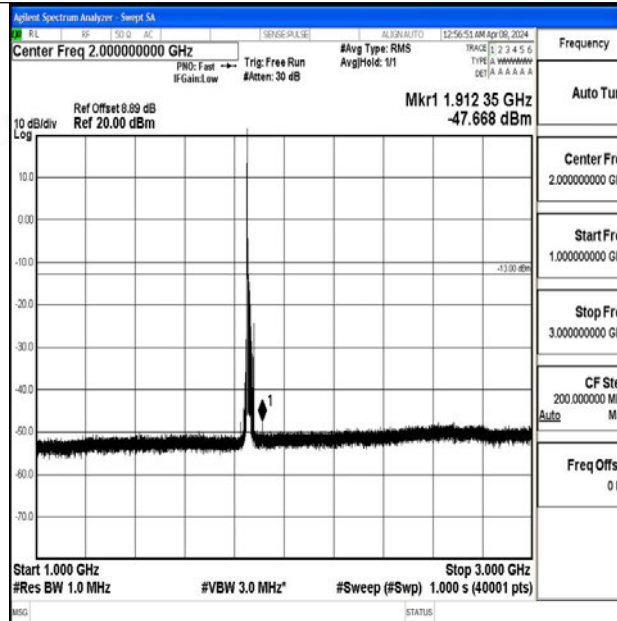
Band2_15MHz_QPSK_18675_1RB#0_1000~3000_1000~3000
