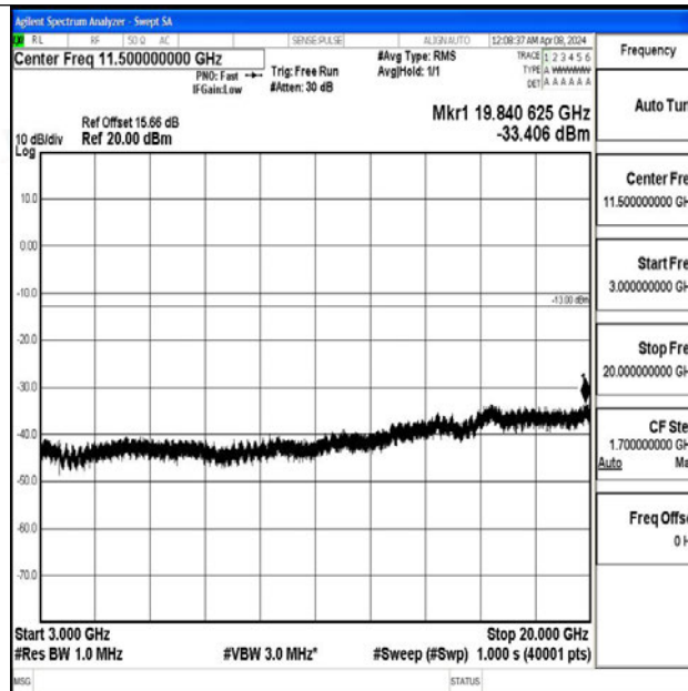
Band2_3MHz_64QAM_19185_1RB#0_3000~20000_3000~20000
