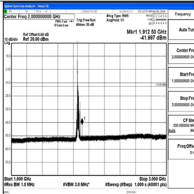
Band2_20MHz_64QAM_18700_1RB#0_1000~3000_1000~3000
