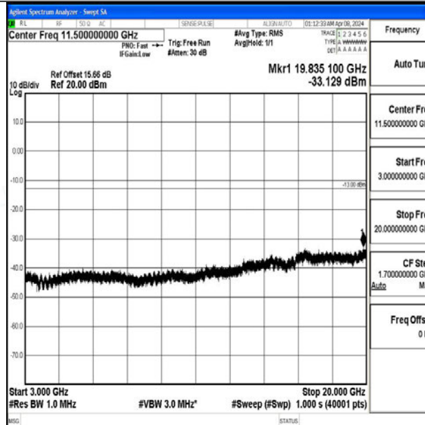
Band2_20MHz_QPSK_18700_1RB#0_3000~20000_3000~20000
