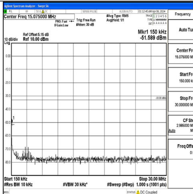
Band2_20MHz_64QAM_18700_1RB#0_0.15~30_0.15~30
