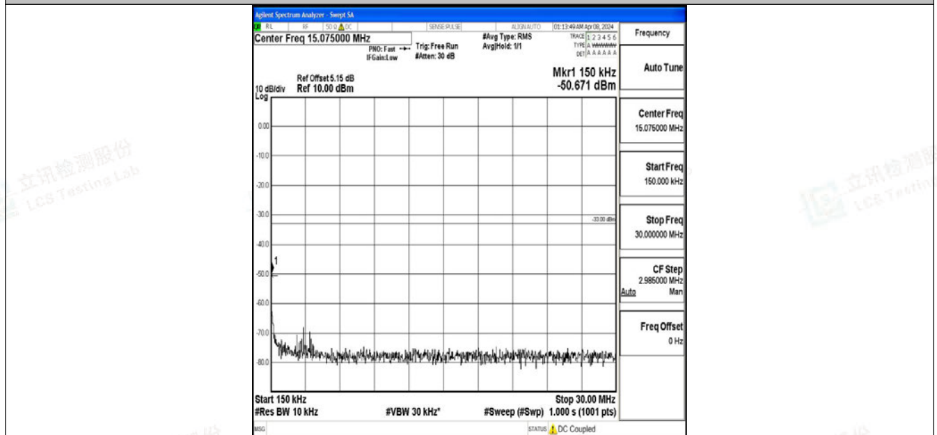
Band2_20MHz_64QAM_18900_1RB#0_0.15~30_0.15~30
