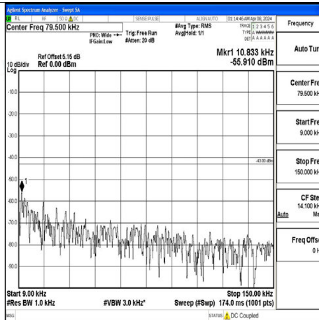
Band2_20MHz_64QAM_19100_1RB#0_0.009~0.15_0.009~0.15
