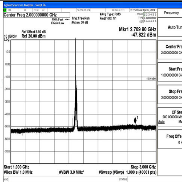
Band2_20MHz_64QAM_19100_1RB#0_1000~3000_1000~3000
