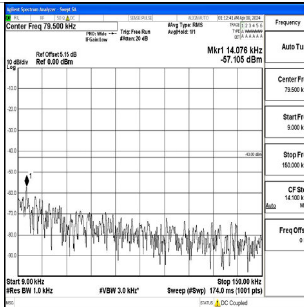
Band2_20MHz_64QAM_18700_1RB#0_0.009~0.15_0.009~0.15
