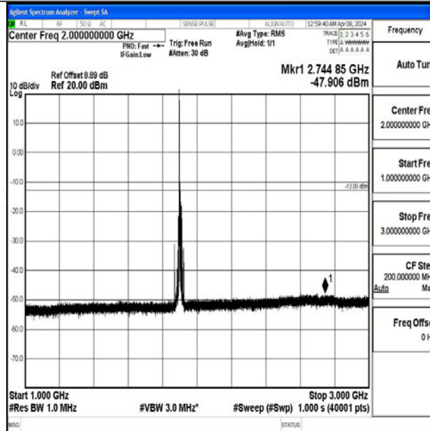
Band2_15MHz_64QAM_19125_1RB#0_1000~3000_1000~3000
