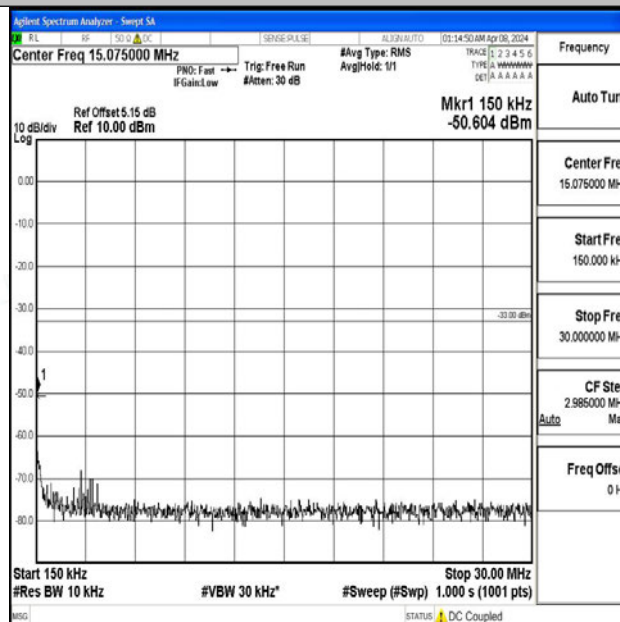
Band2_20MHz_64QAM_19100_1RB#0_0.15~30_0.15~30
