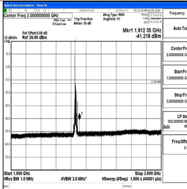
Band2_20MHz_QPSK_18700_1RB#0_1000~3000_1000~3000
