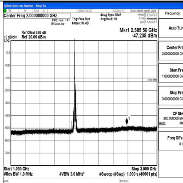
Band2_20MHz_64QAM_18900_1RB#0_1000~3000_1000~3000
