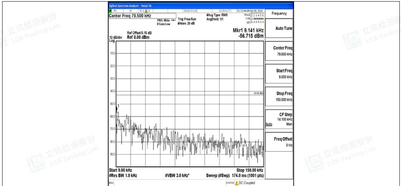
Band2_20MHz_64QAM_18900_1RB#0_0.009~0.15_0.009~0.15
