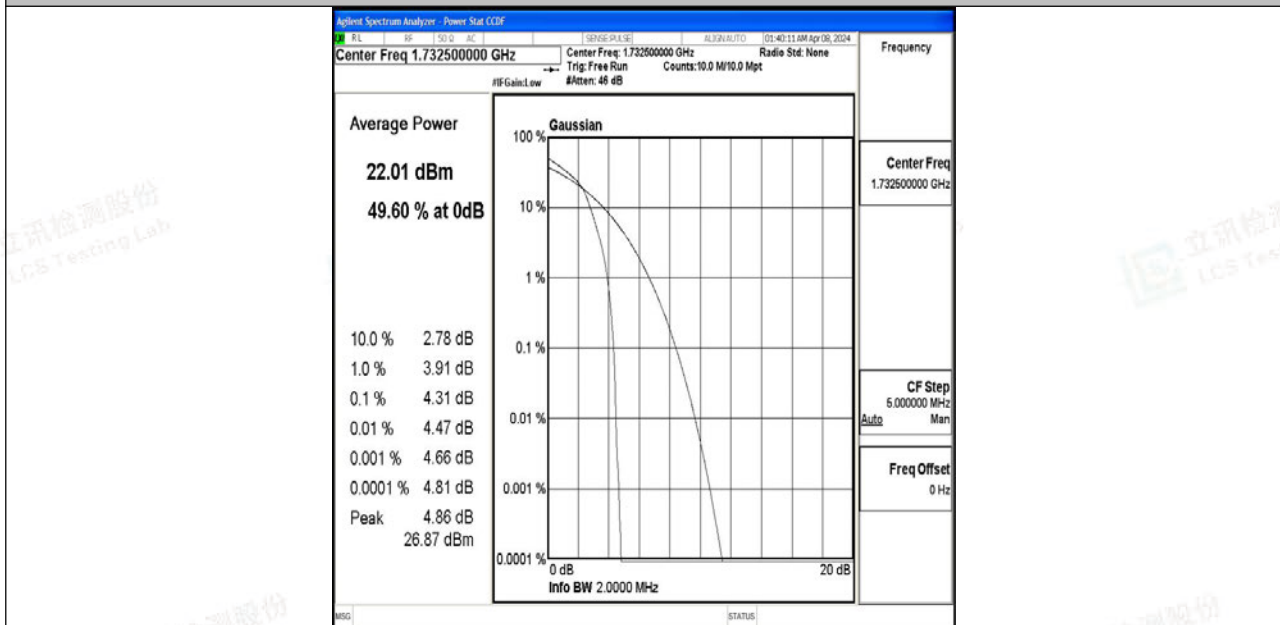
Band4-1.4MHz-64QAM-20175-1RB#0-PASS
