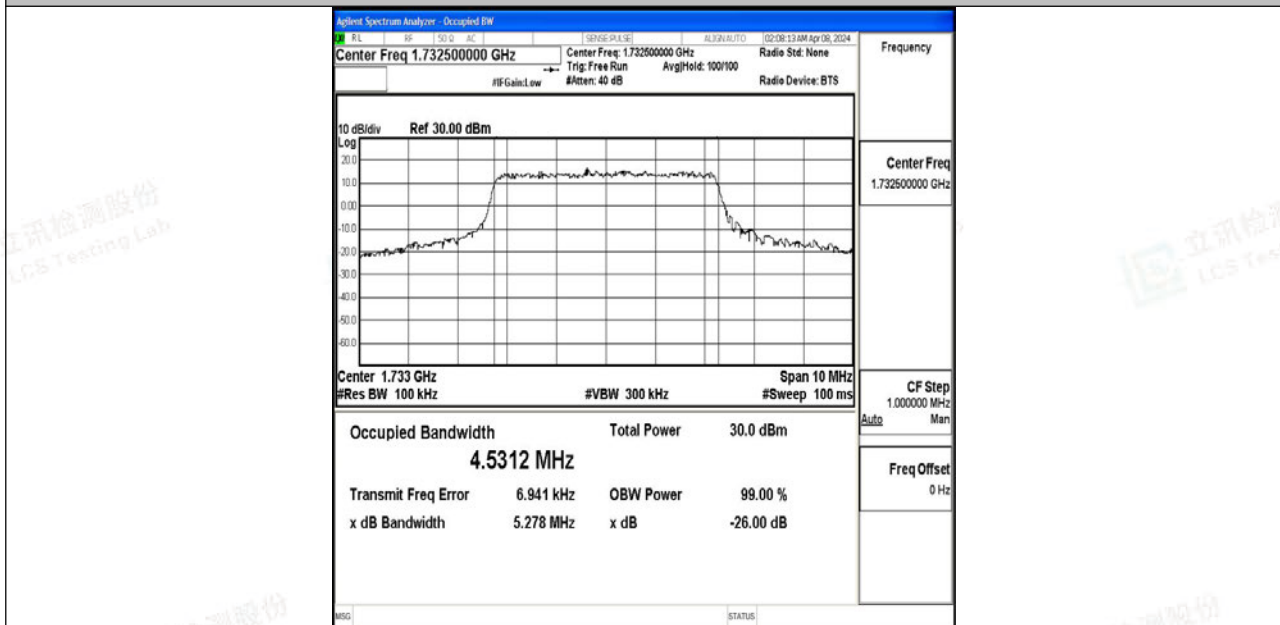
Band4-5MHz-64QAM-20175-25RB#0-PASS
