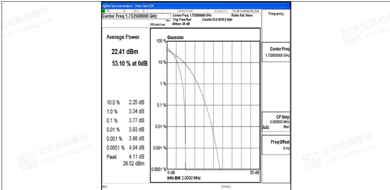
Band4-1.4MHz-QPSK-20175-1RB#0-PASS
