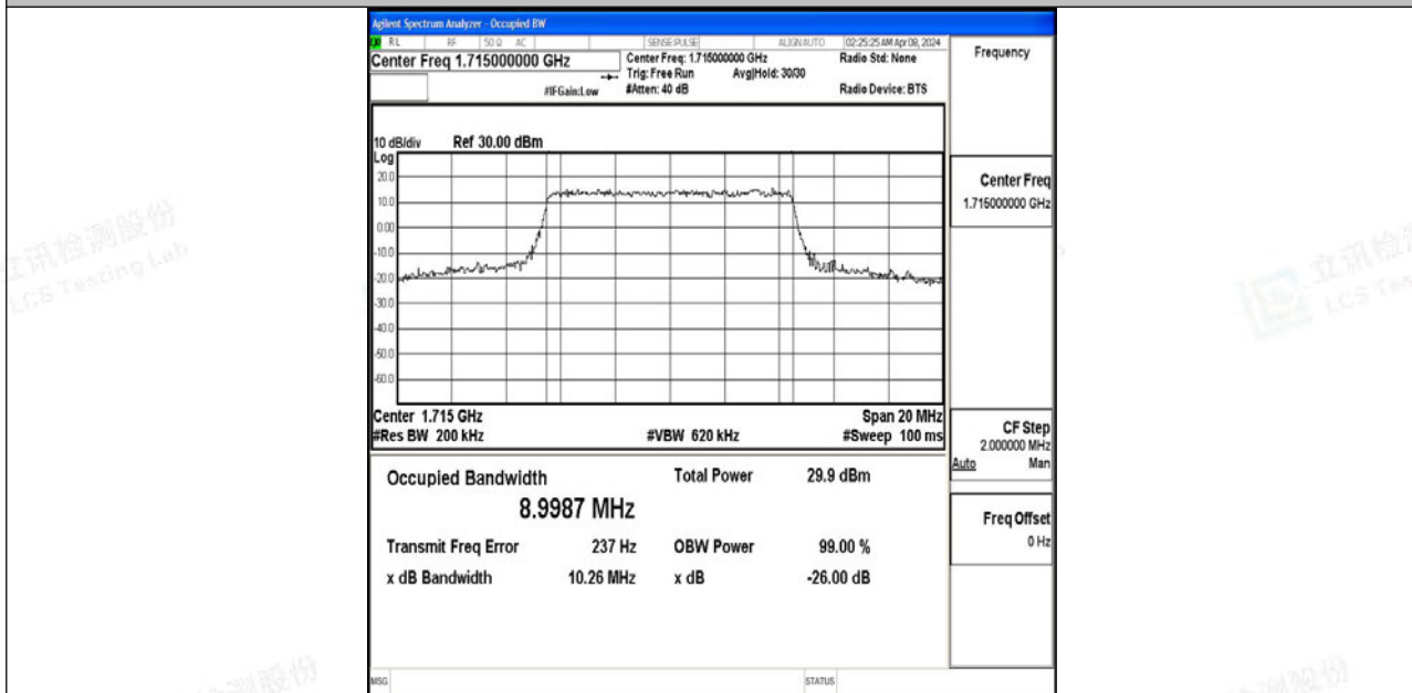
Band4-10MHz-64QAM-20000-50RB#0-PASS
