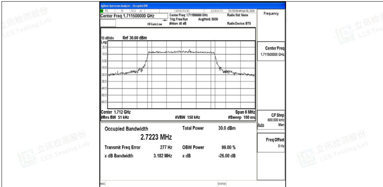
Band4-3MHz-QPSK-19965-15RB#0-PASS
