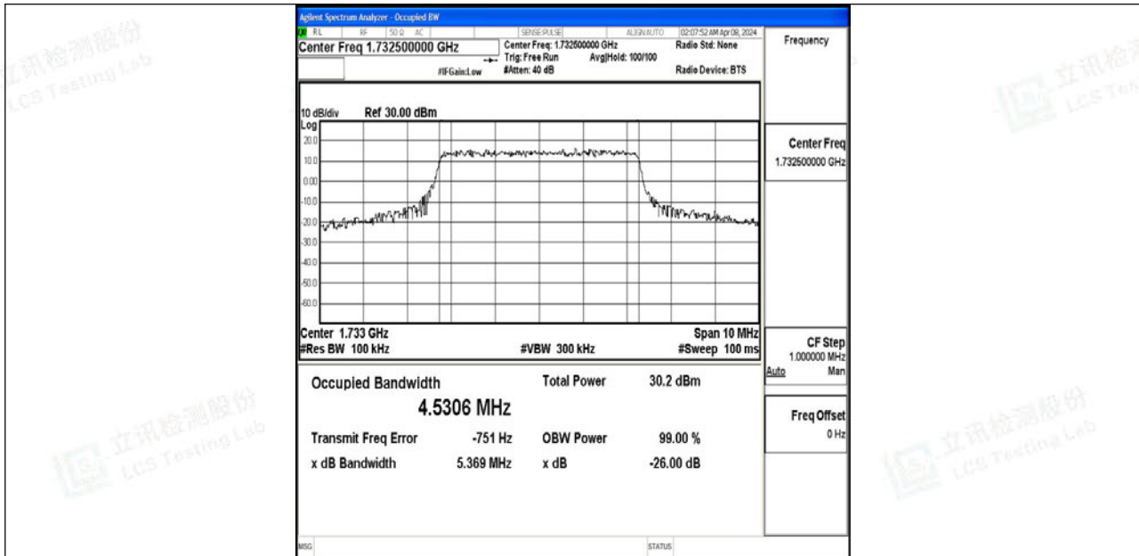
Band4-5MHz-QPSK-20175-25RB#0-PASS
