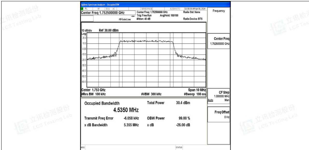
Band4-5MHz-QPSK-20375-25RB#0-PASS
