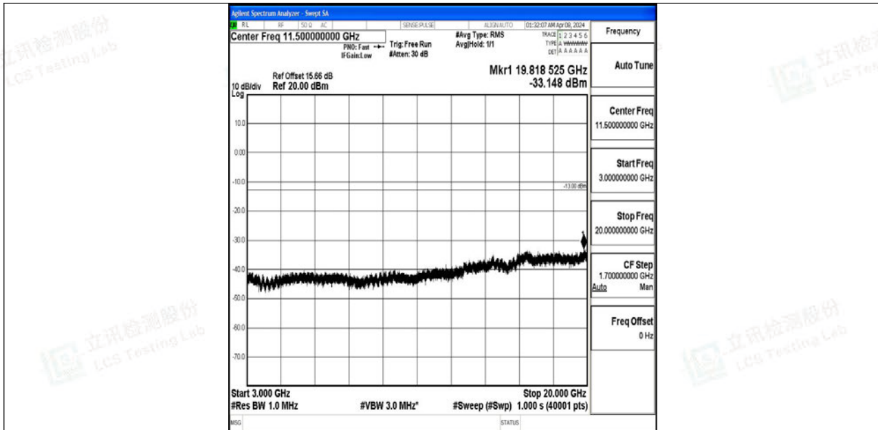
Band4_1.4MHz_64QAM_20393_1RB#0_3000~20000_3000~20000
