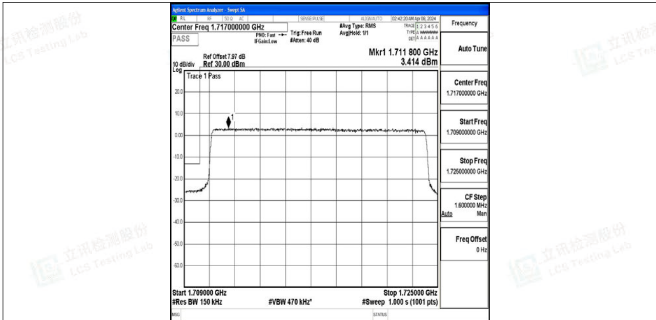
Band4_15MHz_QPSK_20025_75RB#0
