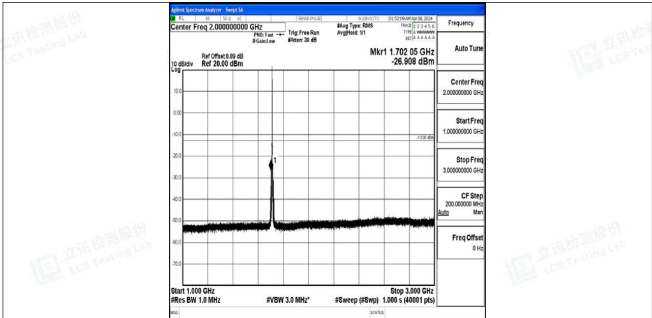
Band4_3MHz_QPSK_19965_1RB#0_1000~3000_1000~3000
