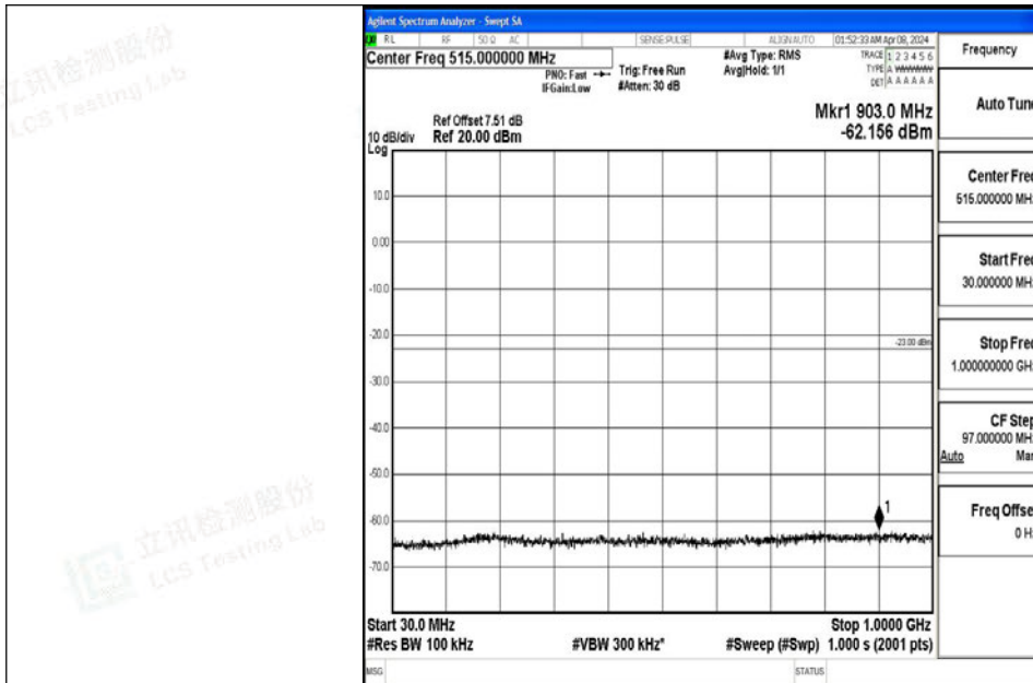
Band4_3MHz_64QAM_19965_1RB#0_30~1000_30~1000
