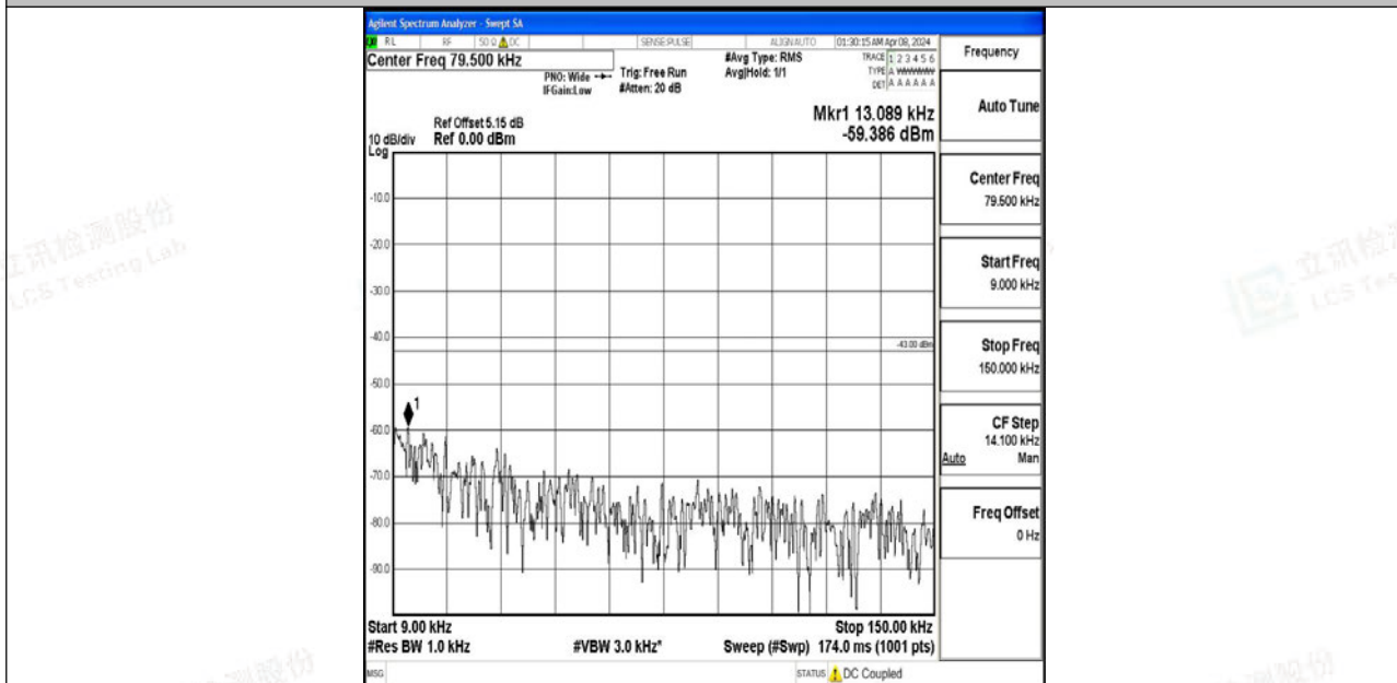
Band4_1.4MHz_QPSK_20175_1RB#0_0.009~0.15_0.009~0.15
