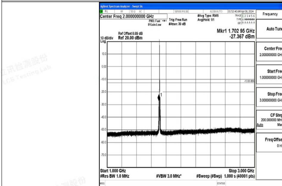
Band4_3MHz_64QAM_19965_1RB#0_1000~3000_1000~3000
