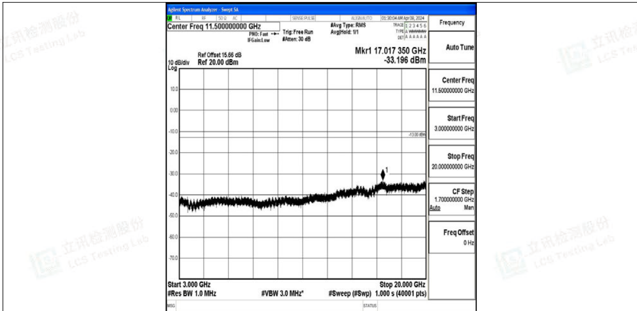
Band4_1.4MHz_64QAM_19957_1RB#0_3000~20000_3000~20000
