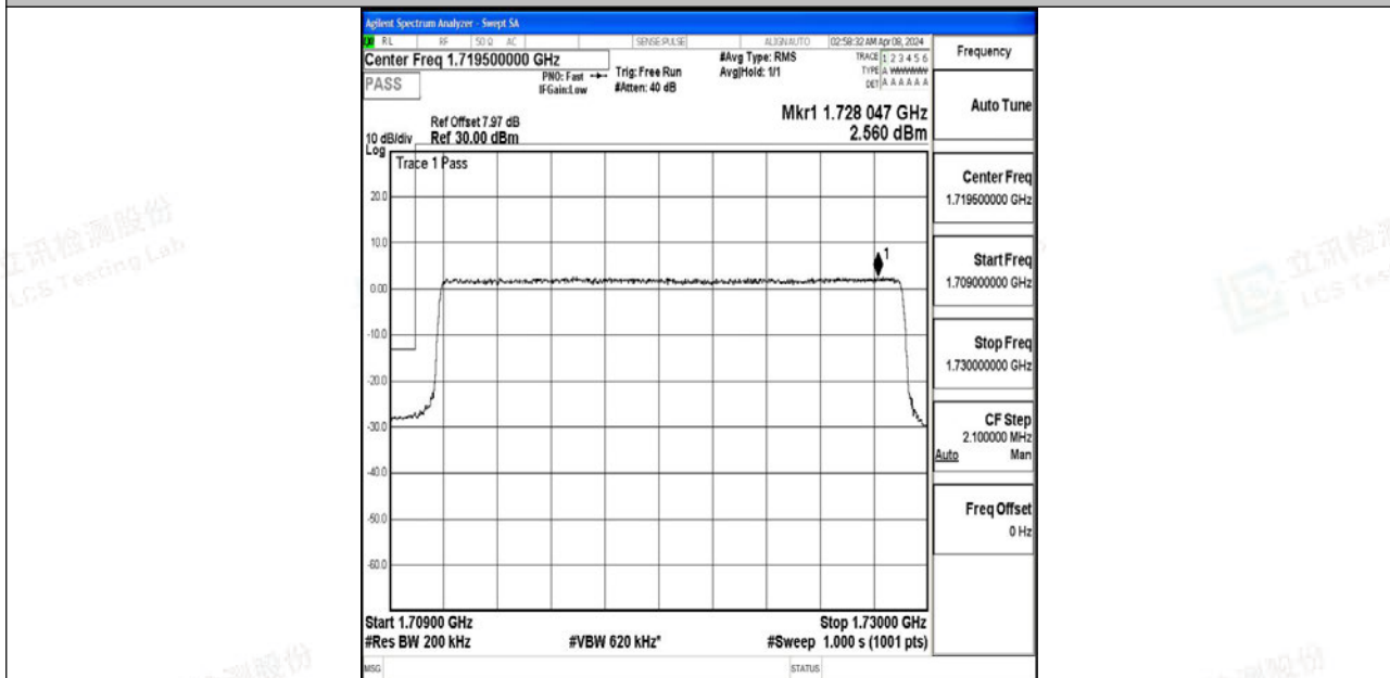
Band4_20MHz_64QAM_20050_100RB#0
