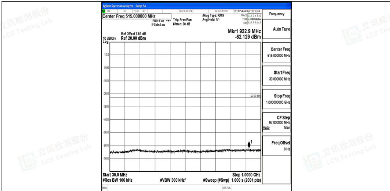
Band4_1.4MHz_64QAM_20175_1RB#0_30~1000_30~1000
