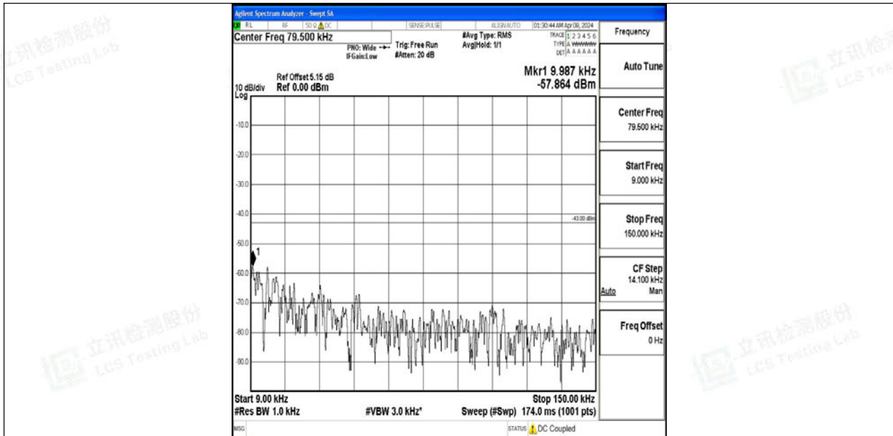
Band4_1.4MHz_64QAM_20175_1RB#0_0.009~0.15_0.009~0.15
