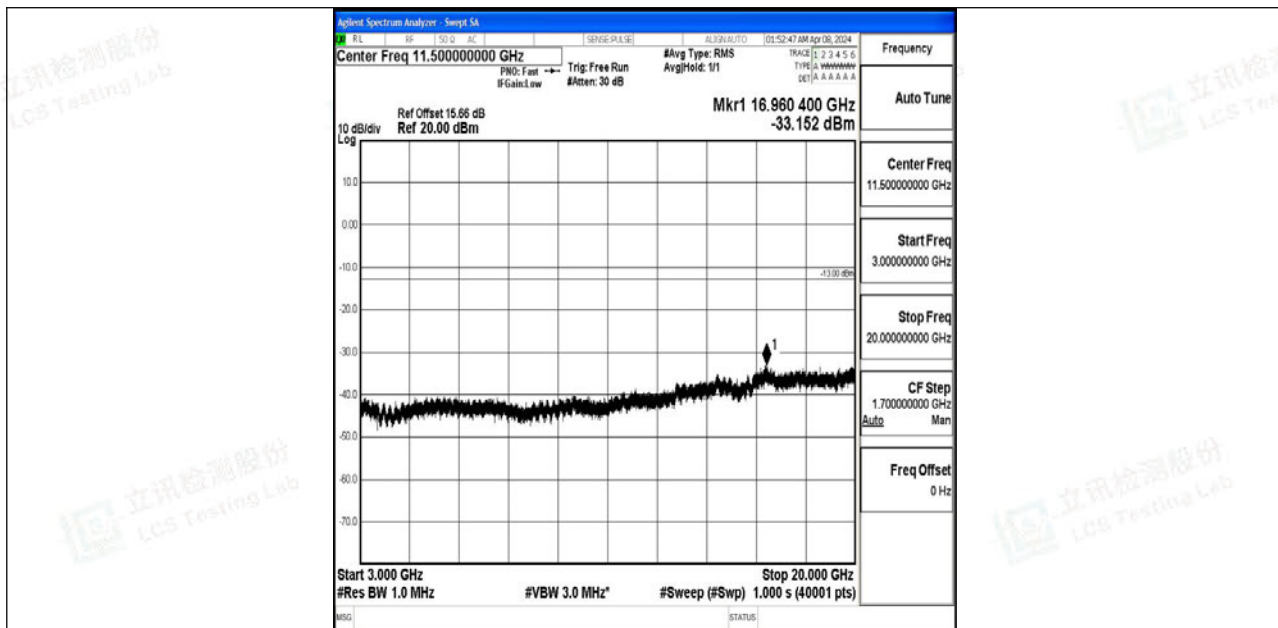
Band4_3MHz_64QAM_19965_1RB#0_3000~20000_3000~20000
