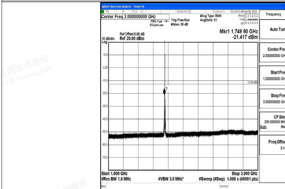
Band4_1.4MHz_64QAM_20393_1RB#0_1000~3000_1000~3000
