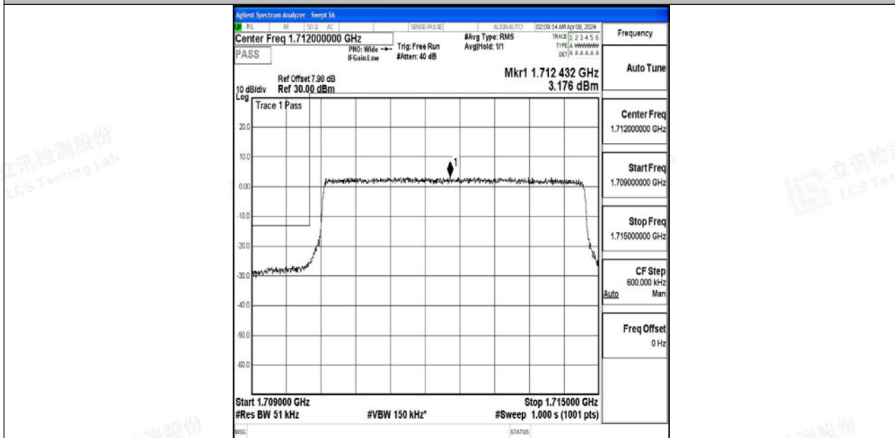
Band4_5MHz_64QAM_19975_25RB#0
