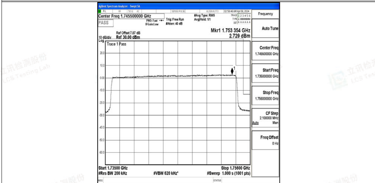
Band4_20MHz_64QAM_20300_100RB#0
