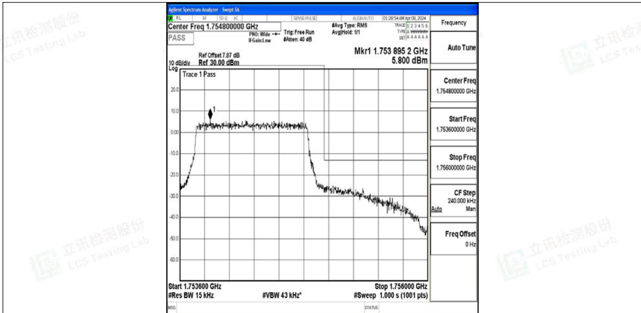
Band4_1.4MHz_QPSK_20393_6RB#0
