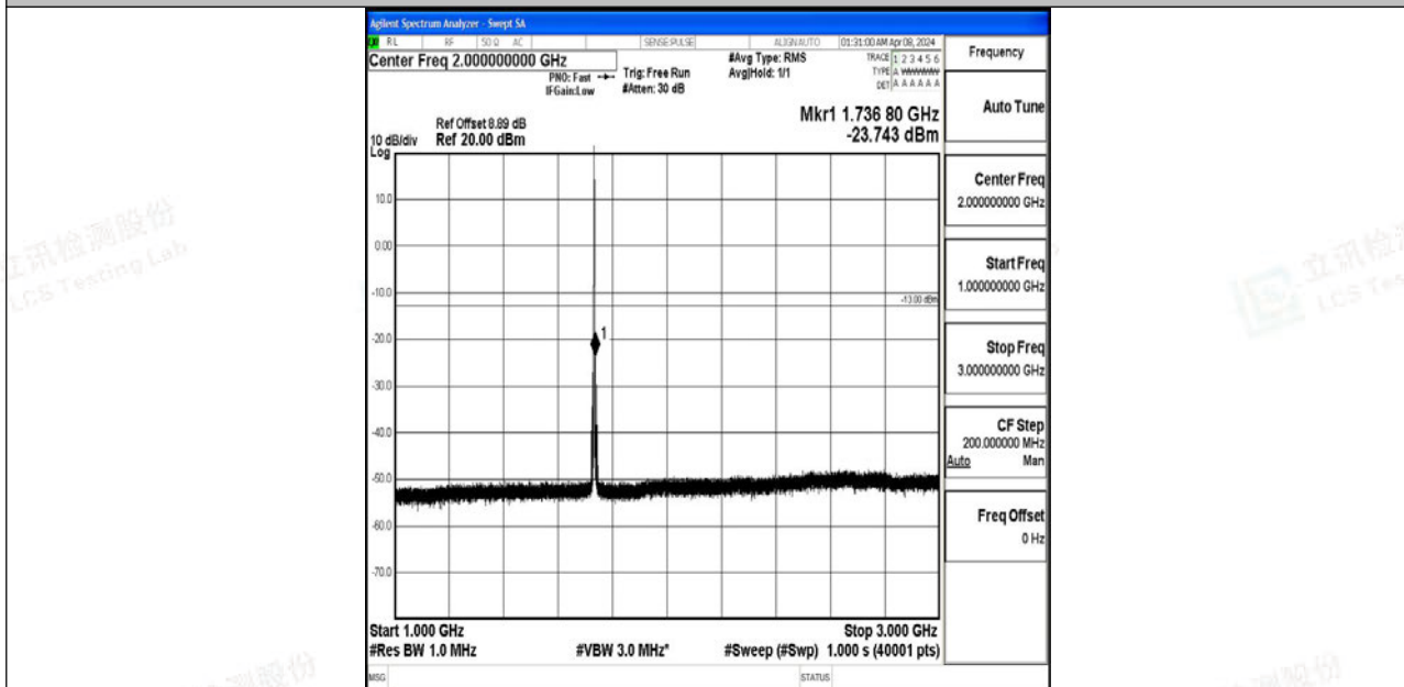
Band4_1.4MHz_64QAM_20175_1RB#0_1000~3000_1000~3000
