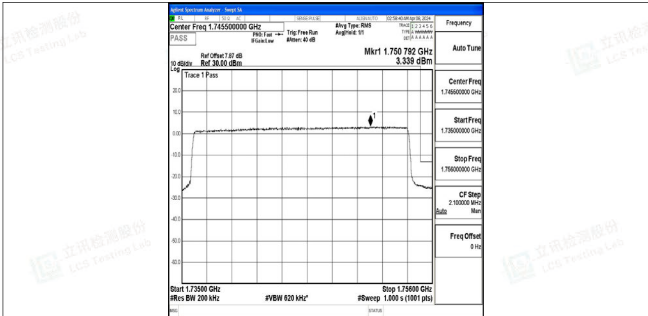
Band4_20MHz_QPSK_20300_100RB#0
