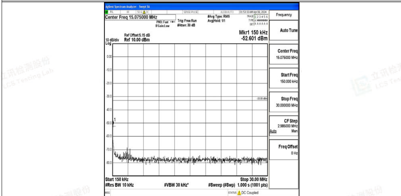
Band4_3MHz_64QAM_20175_1RB#0_0.15~30_0.15~30
