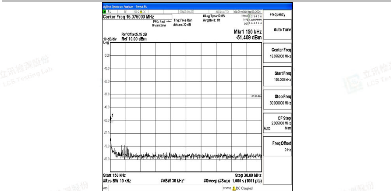
Band4_1.4MHz_64QAM_19957_1RB#0_0.15~30_0.15~30
