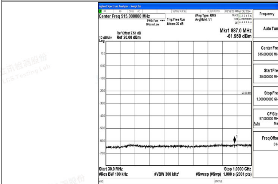
Band4_3MHz_QPSK_19965_1RB#0_30~1000_30~1000
