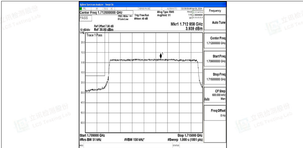
Band4_5MHz_QPSK_19975_25RB#0
