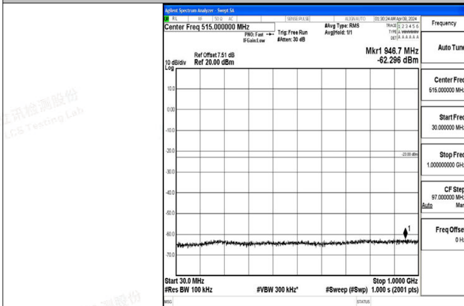
Band4_1.4MHz_QPSK_20175_1RB#0_30~1000_30~1000
