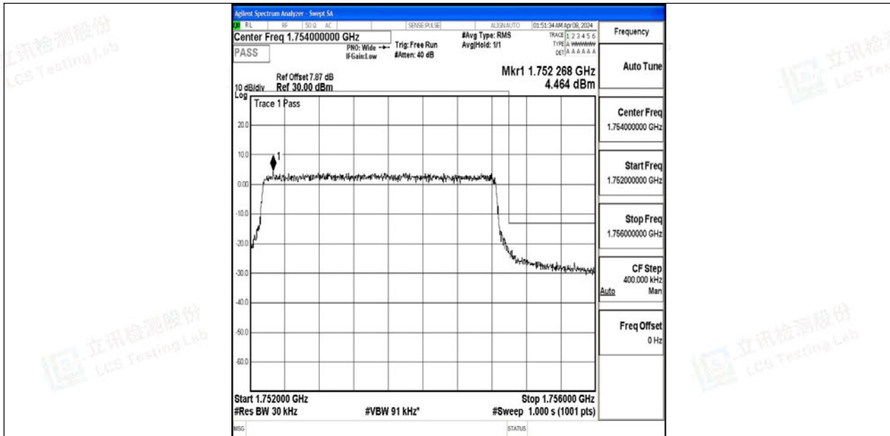
Band4_3MHz_QPSK_20385_15RB#0
