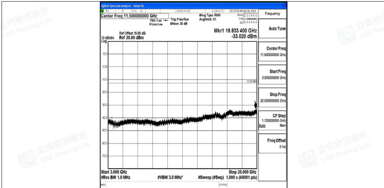
Band4_3MHz_64QAM_20175_1RB#0_3000~20000_3000~20000
