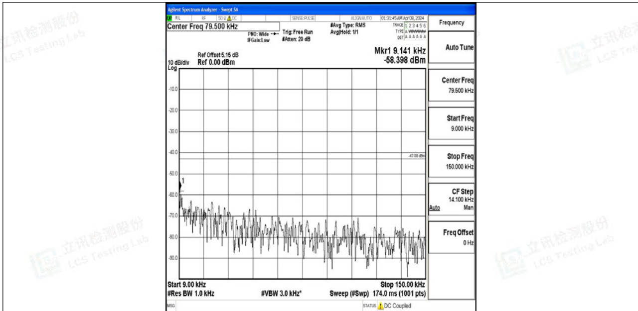
Band4_1.4MHz_64QAM_20393_1RB#0_0.009~0.15_0.009~0.15
