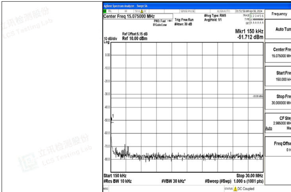
Band4_3MHz_QPSK_19965_1RB#0_0.15~30_0.15~30
