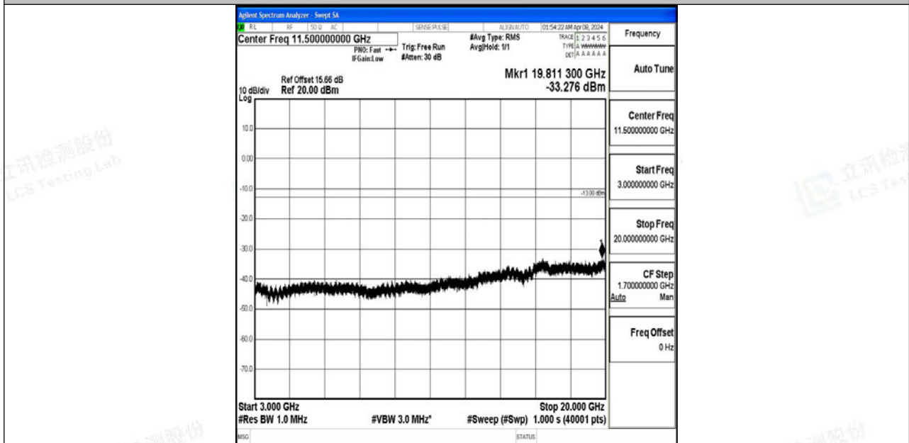
Band4_3MHz_QPSK_20385_1RB#0_3000~20000_3000~20000
