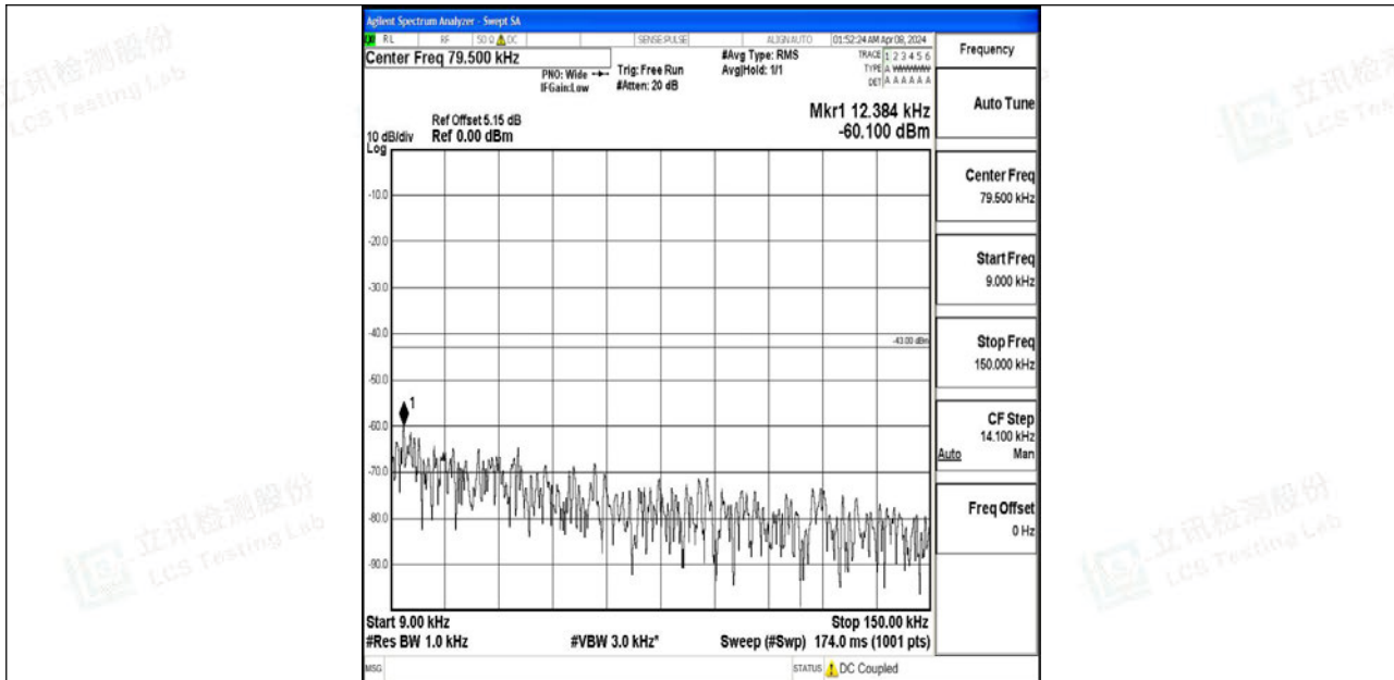
Band4_3MHz_64QAM_19965_1RB#0_0.009~0.15_0.009~0.15
