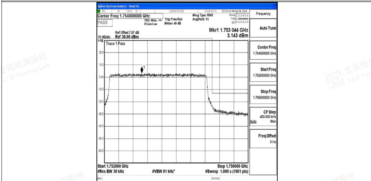
Band4_3MHz_64QAM_20385_15RB#0
