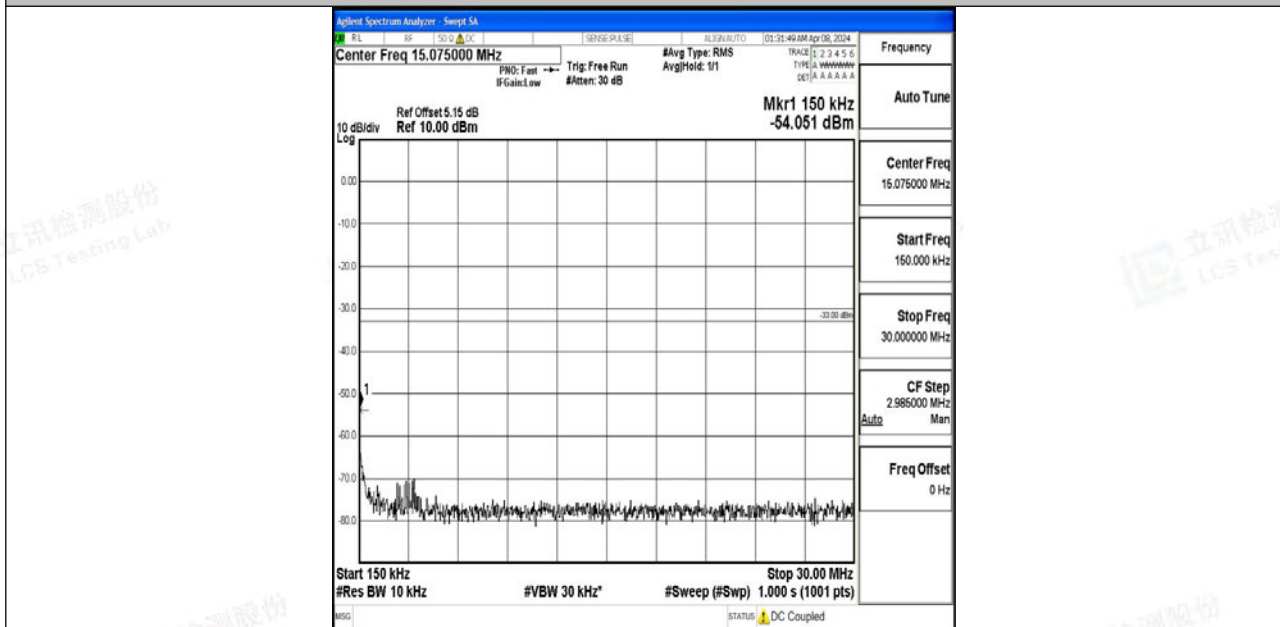
Band4_1.4MHz_64QAM_20393_1RB#0_0.15~30_0.15~30
