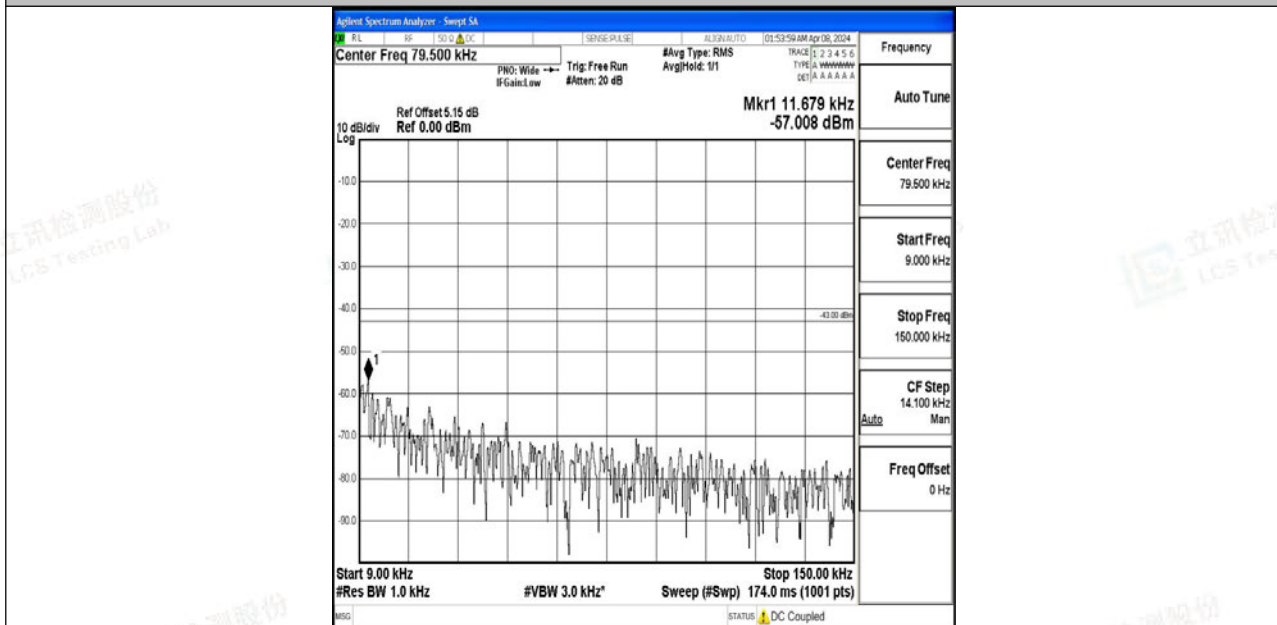
Band4_3MHz_QPSK_20385_1RB#0_0.009~0.15_0.009~0.15
