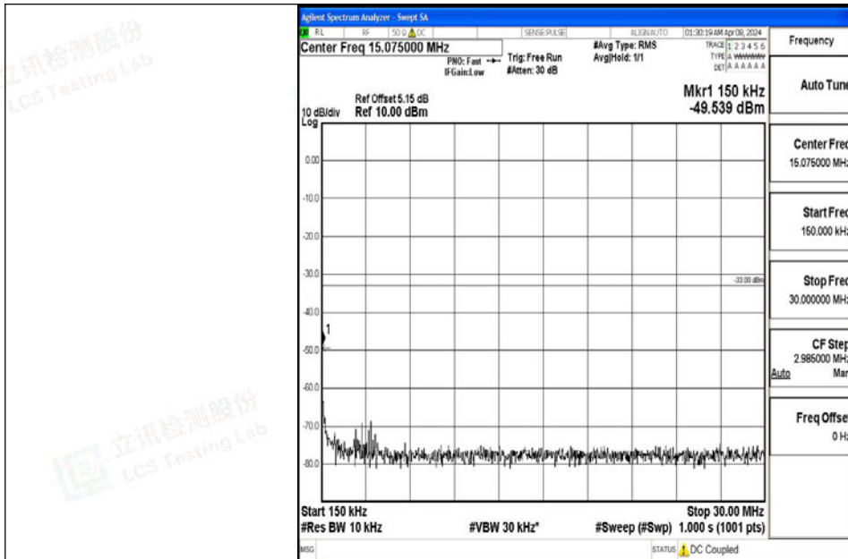
Band4_1.4MHz_QPSK_20175_1RB#0_0.15~30_0.15~30
