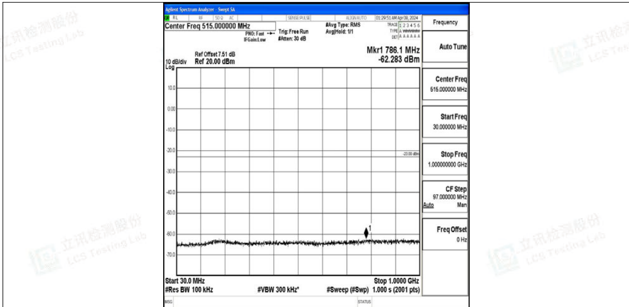
Band4_1.4MHz_64QAM_19957_1RB#0_30~1000_30~1000
