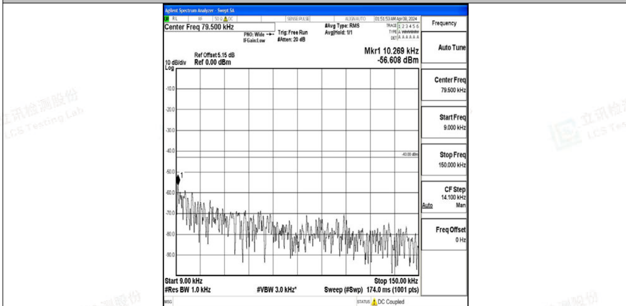
Band4_3MHz_QPSK_19965_1RB#0_0.009~0.15_0.009~0.15
