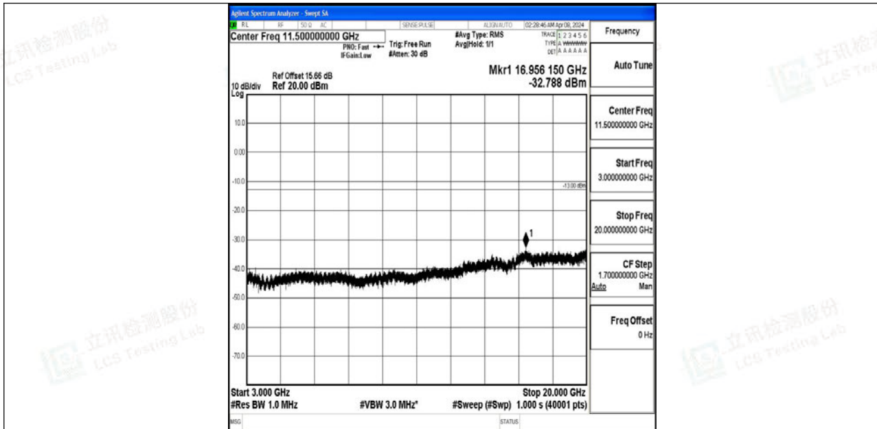
Band4_10MHz_64QAM_20175_1RB#0_3000~20000_3000~20000
