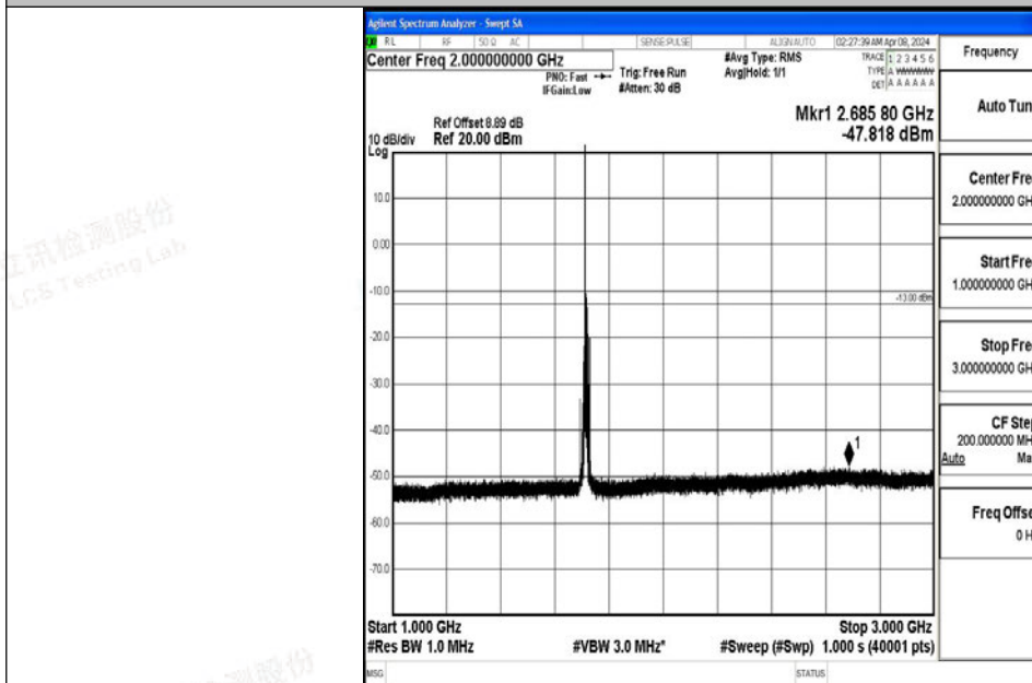
Band4_10MHz_64QAM_20000_1RB#0_1000~3000_1000~3000
