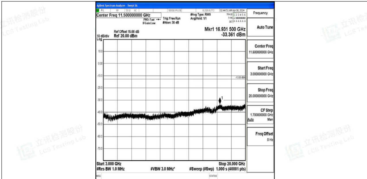
Band4_15MHz_64QAM_20175_1RB#0_3000~20000_3000~20000
