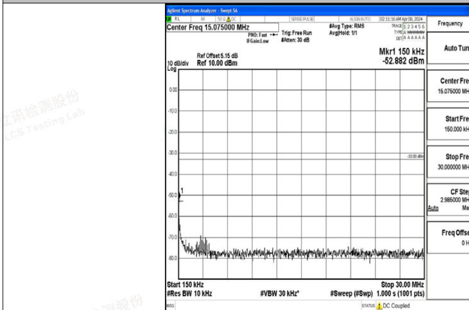
Band4_5MHz_64QAM_20175_1RB#0_0.15~30_0.15~30
