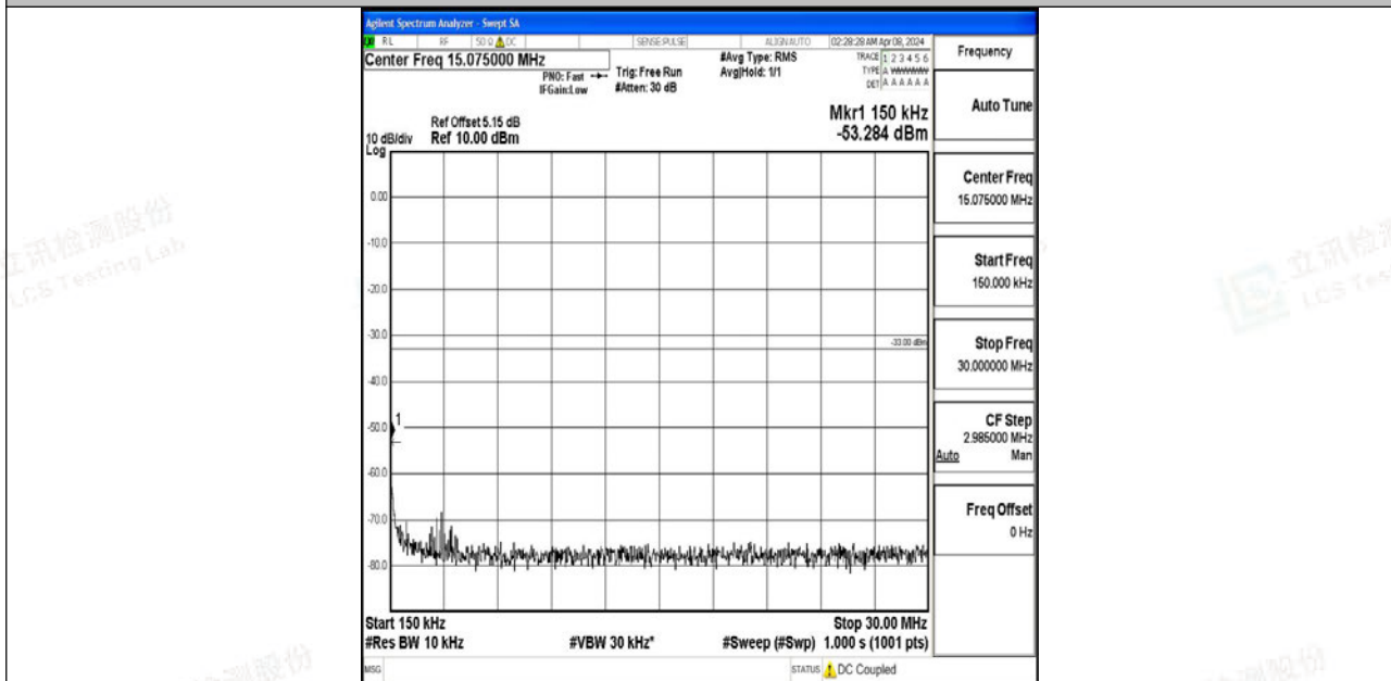
Band4_10MHz_64QAM_20175_1RB#0_0.15~30_0.15~30
