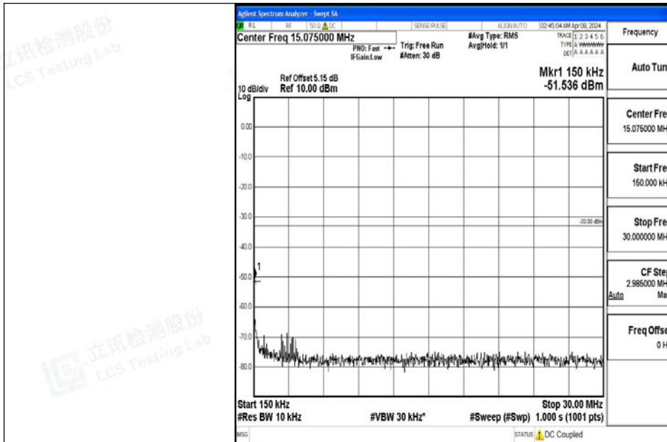
Band4_15MHz_QPSK_20325_1RB#0_0.15~30_0.15~30
