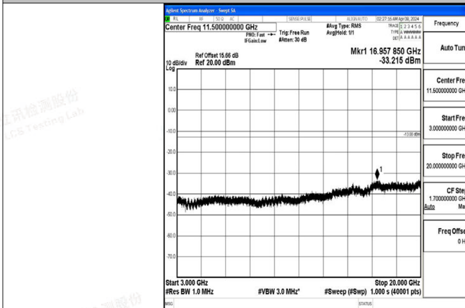
Band4_10MHz_QPSK_20000_1RB#0_3000~20000_3000~20000
