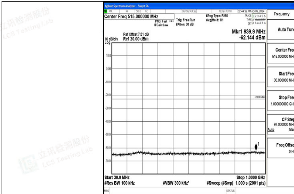
Band4_15MHz_64QAM_20175_1RB#0_30~1000_30~1000
