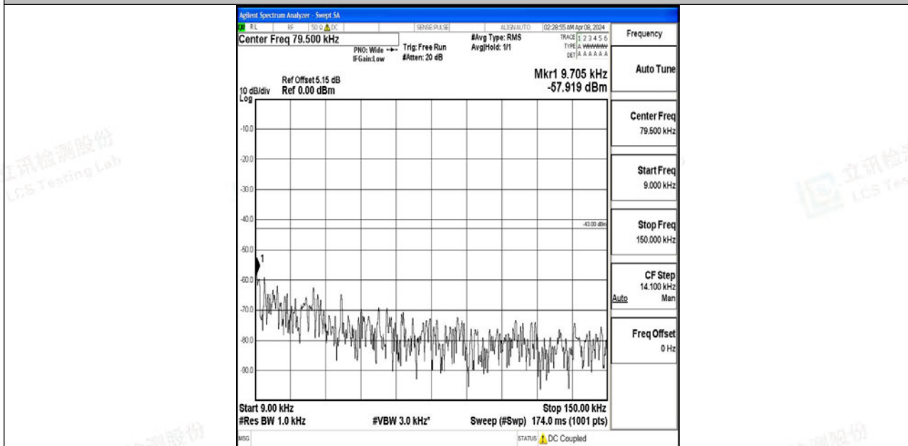
Band4_10MHz_QPSK_20350_1RB#0_0.009~0.15_0.009~0.15
