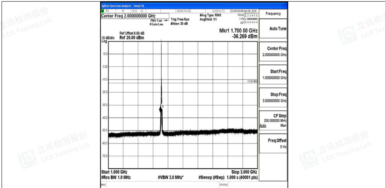
Band4_5MHz_QPSK_19975_1RB#0_1000~3000_1000~3000
