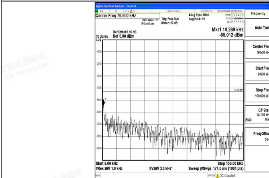
Band4_15MHz_QPSK_20025_1RB#0_0.009~0.15_0.009~0.15
