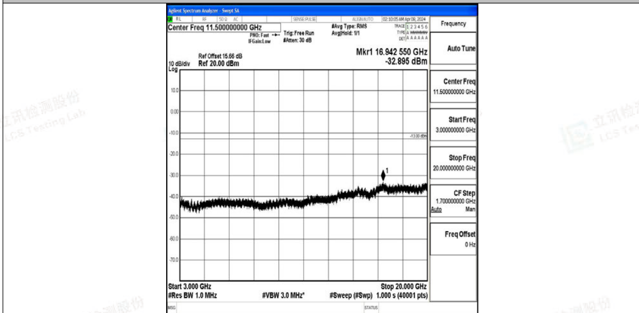
Band4_5MHz_QPSK_19975_1RB#0_3000~20000_3000~20000
