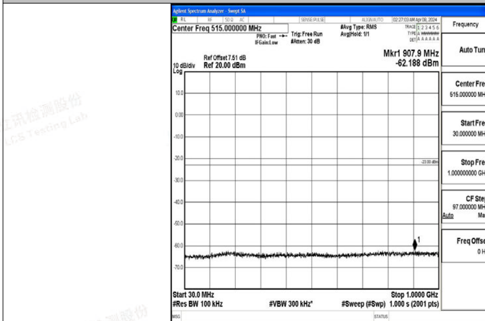
Band4_10MHz_QPSK_20000_1RB#0_30~1000_30~1000
