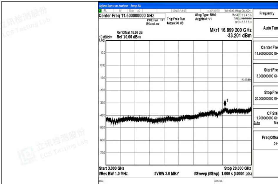
Band4_15MHz_64QAM_20025_1RB#0_3000~20000_3000~20000
