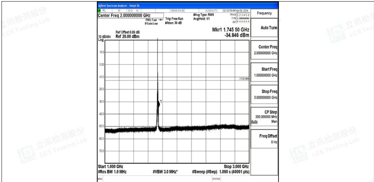
Band4_5MHz_QPSK_20175_1RB#0_1000~3000_1000~3000
