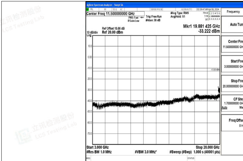
Band4_10MHz_64QAM_20350_1RB#0_3000~20000_3000~20000
