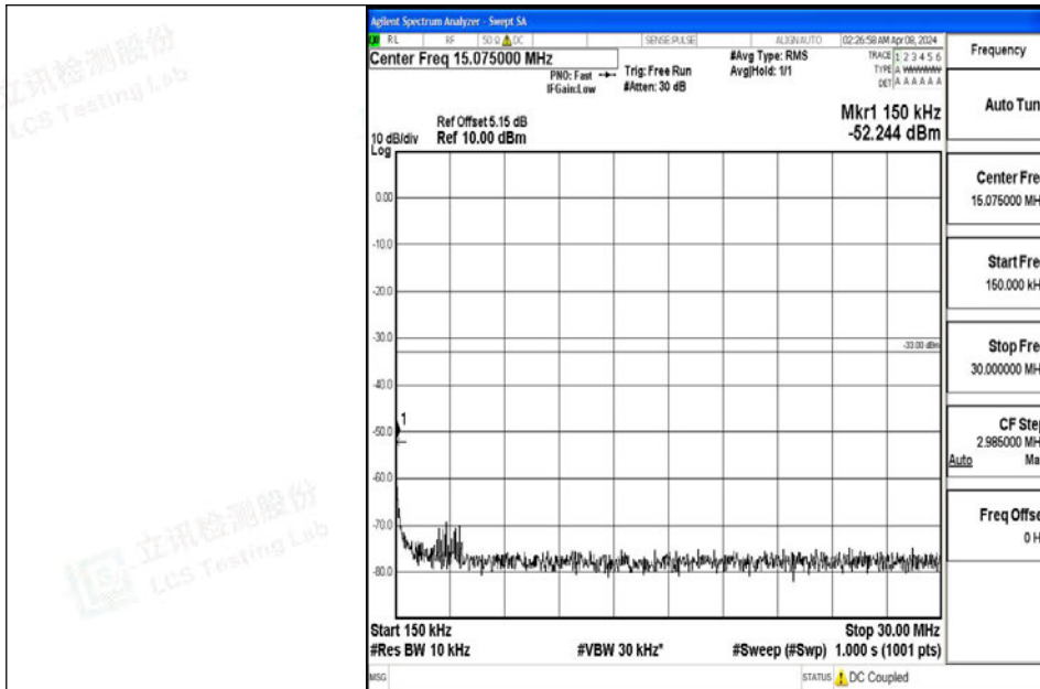
Band4_10MHz_QPSK_20000_1RB#0_0.15~30_0.15~30
