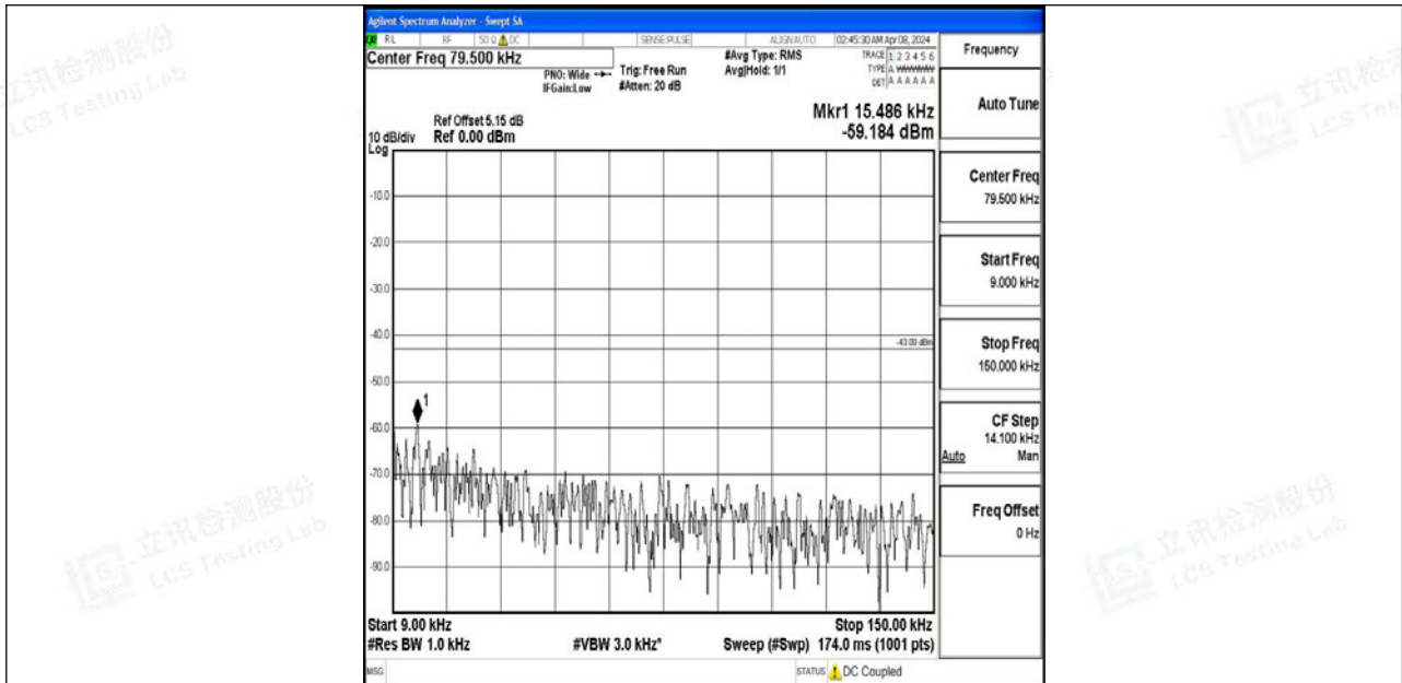
Band4_15MHz_64QAM_20325_1RB#0_0.009~0.15_0.009~0.15
