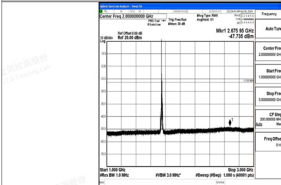
Band4_10MHz_64QAM_20350_1RB#0_1000~3000_1000~3000
