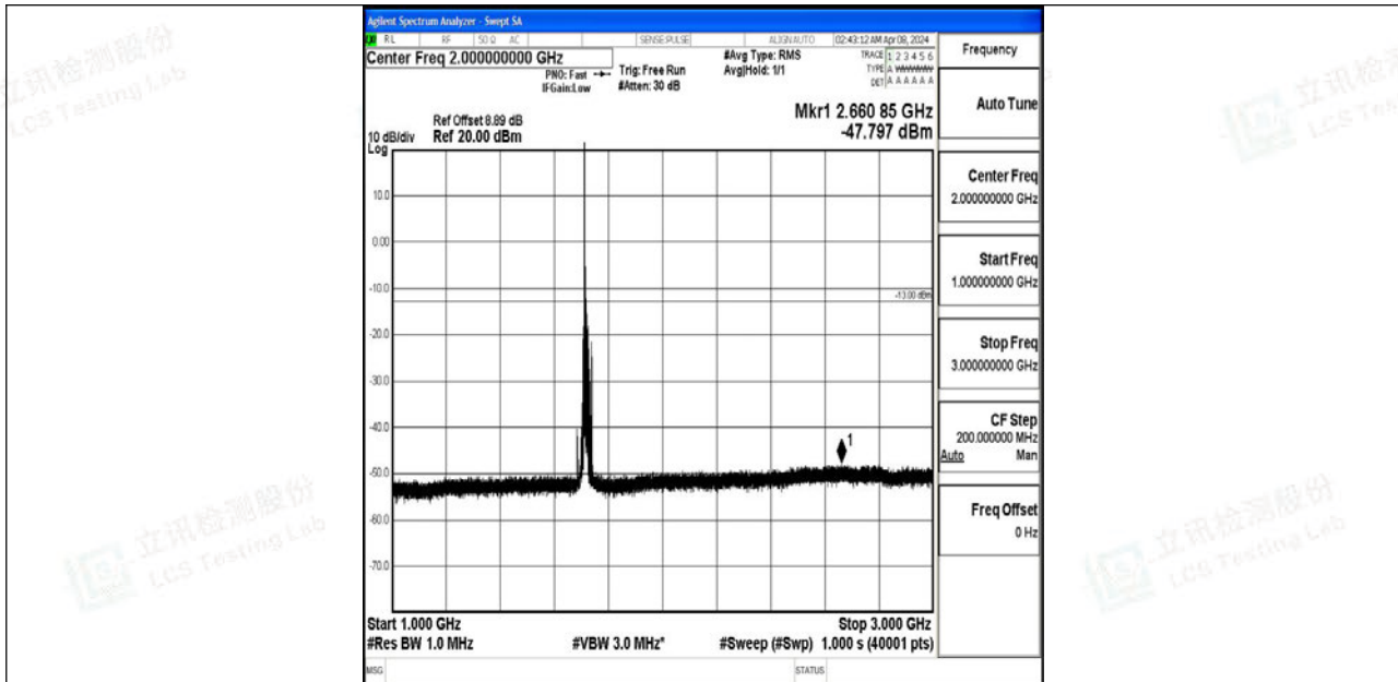
Band4_15MHz_QPSK_20025_1RB#0_1000~3000_1000~3000
