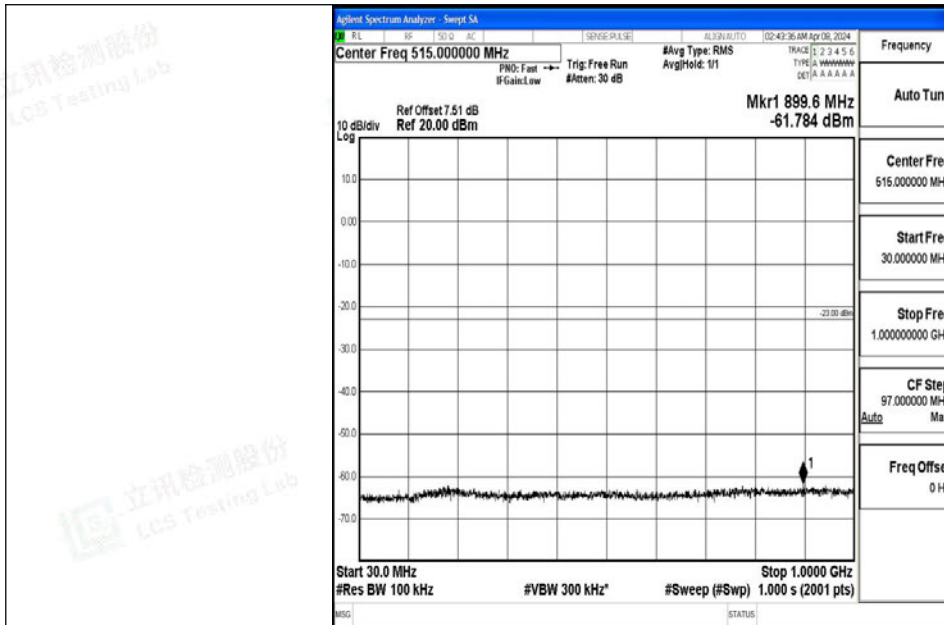
Band4_15MHz_64QAM_20025_1RB#0_30~1000_30~1000
