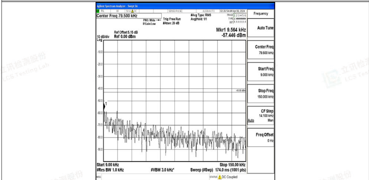
Band4_10MHz_QPSK_20000_1RB#0_0.009~0.15_0.009~0.15
