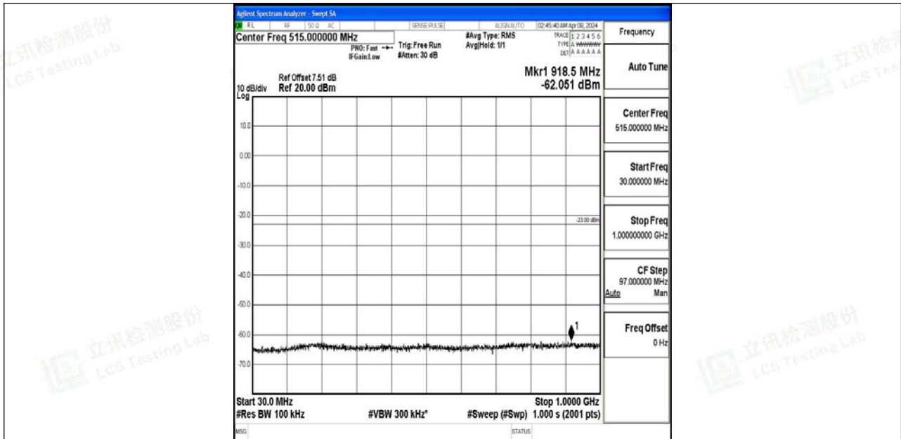
Band4_15MHz_64QAM_20325_1RB#0_30~1000_30~1000
