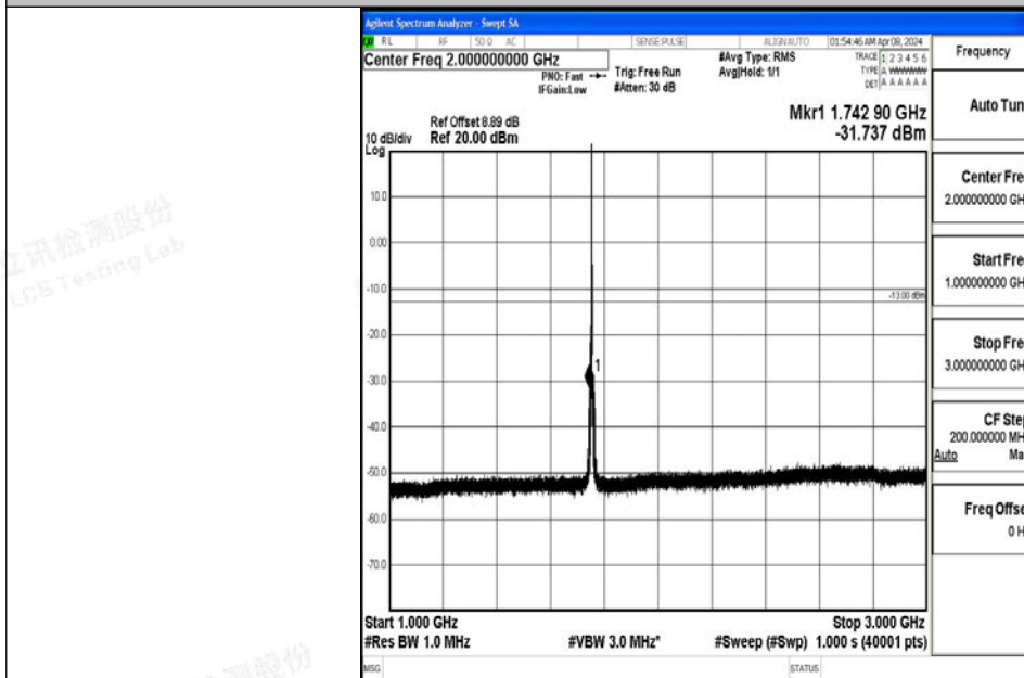
Band4_3MHz_64QAM_20385_1RB#0_1000~3000_1000~3000
