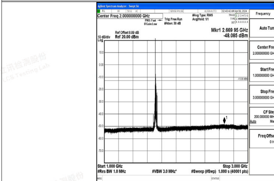
Band4_15MHz_64QAM_20025_1RB#0_1000~3000_1000~3000
