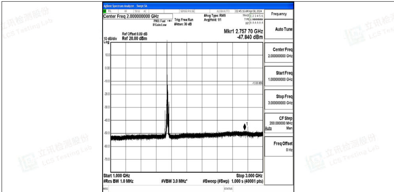
Band4_15MHz_QPSK_20325_1RB#0_1000~3000_1000~3000
