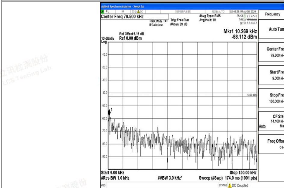
Band4_15MHz_QPSK_20175_1RB#0_0.009~0.15_0.009~0.15
