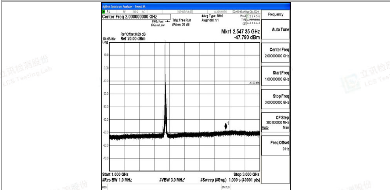
Band4_15MHz_64QAM_20325_1RB#0_1000~3000_1000~3000
