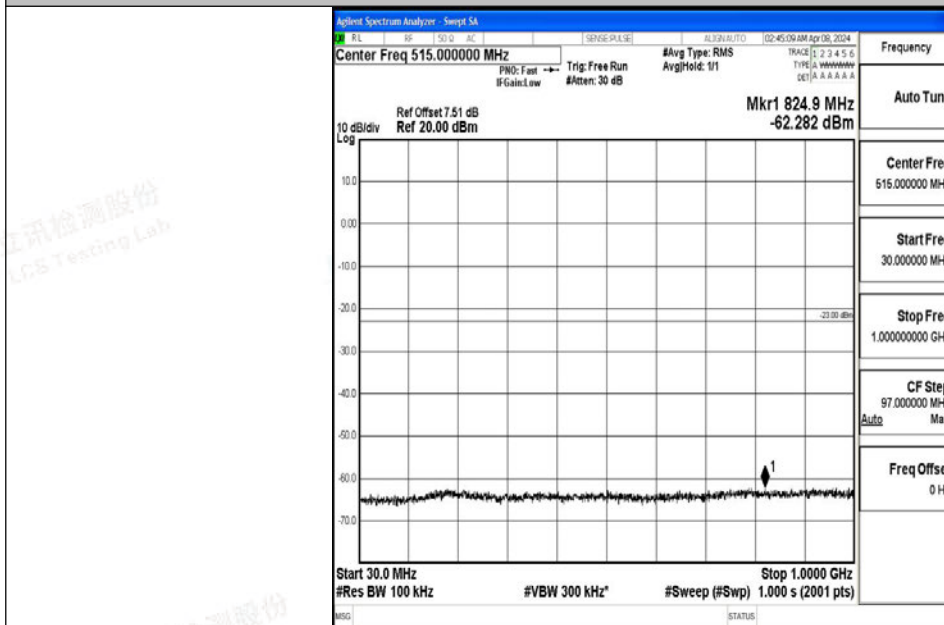
Band4_15MHz_QPSK_20325_1RB#0_30~1000_30~1000
