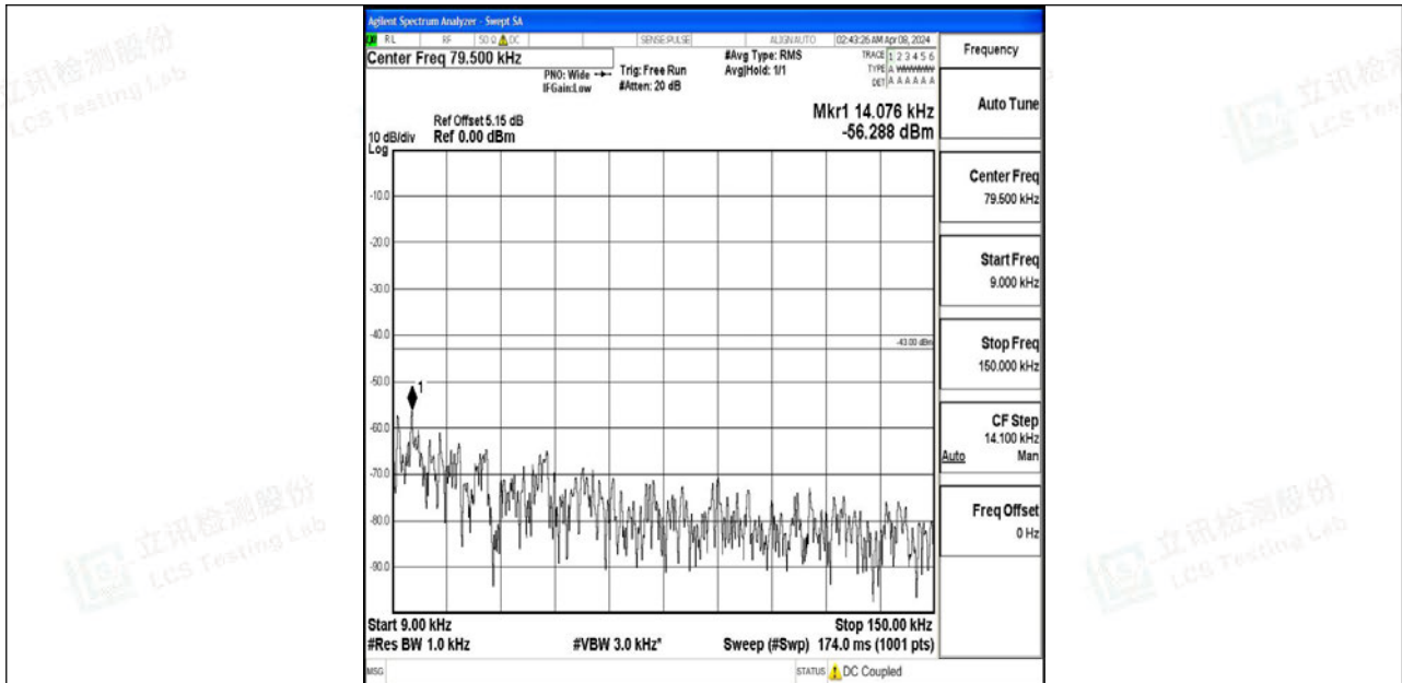
Band4_15MHz_64QAM_20025_1RB#0_0.009~0.15_0.009~0.15
