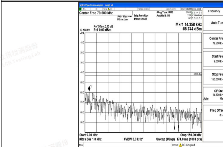
Band4_10MHz_QPSK_20175_1RB#0_0.009~0.15_0.009~0.15
