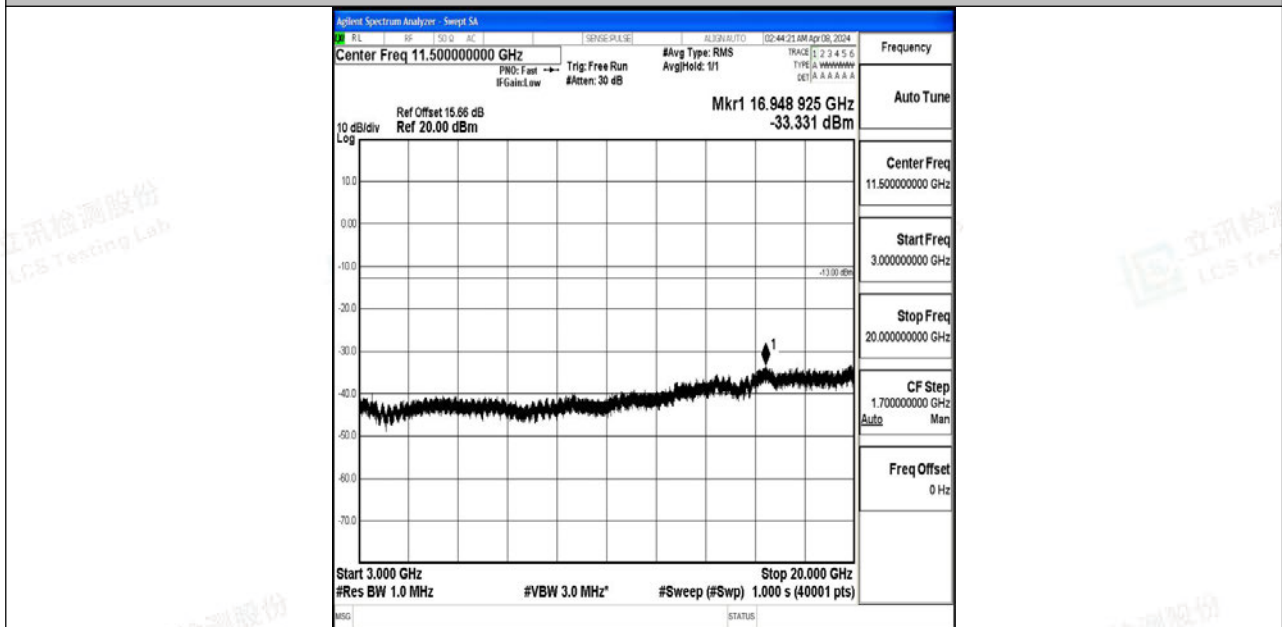
Band4_15MHz_QPSK_20175_1RB#0_3000~20000_3000~20000
