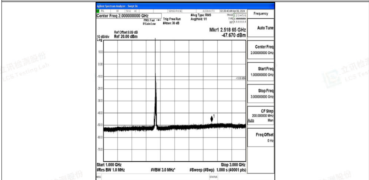
Band4_10MHz_64QAM_20175_1RB#0_1000~3000_1000~3000
