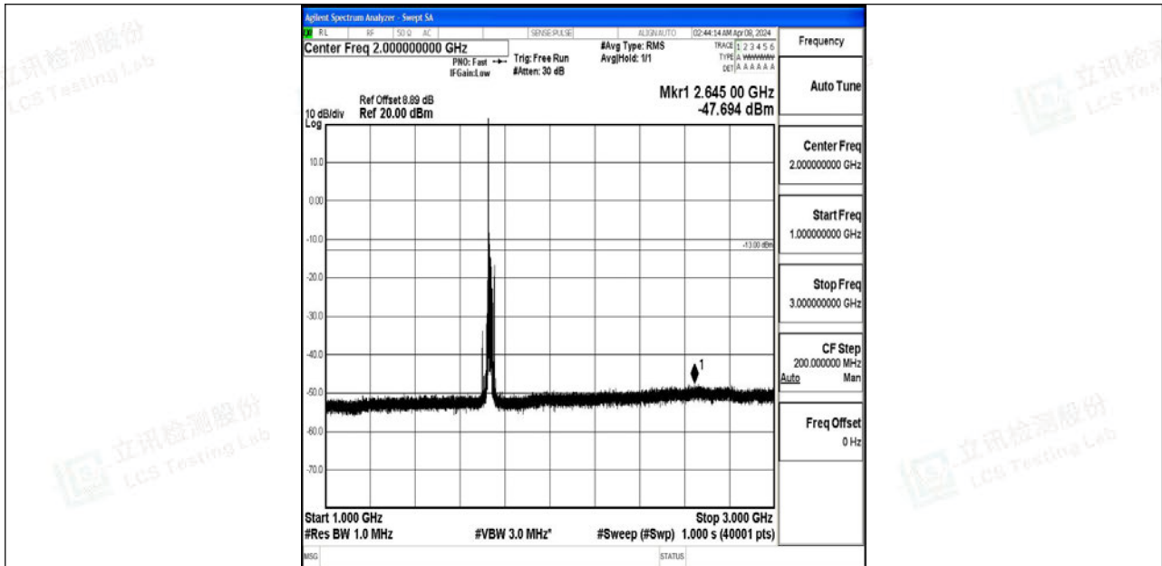
Band4_15MHz_QPSK_20175_1RB#0_1000~3000_1000~3000
