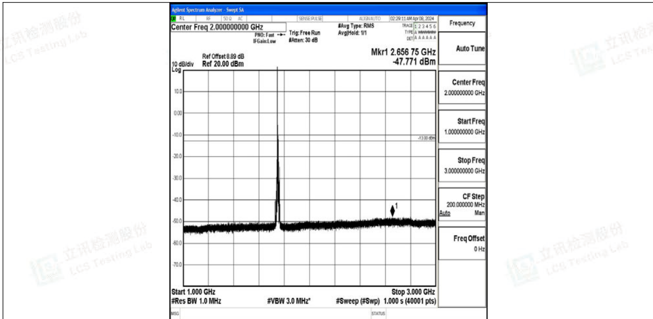
Band4_10MHz_QPSK_20350_1RB#0_1000~3000_1000~3000
