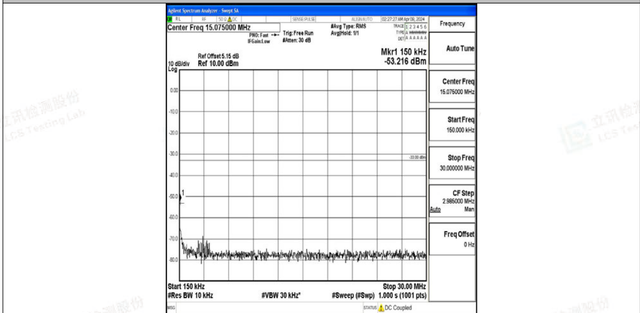
Band4_10MHz_64QAM_20000_1RB#0_0.15~30_0.15~30
