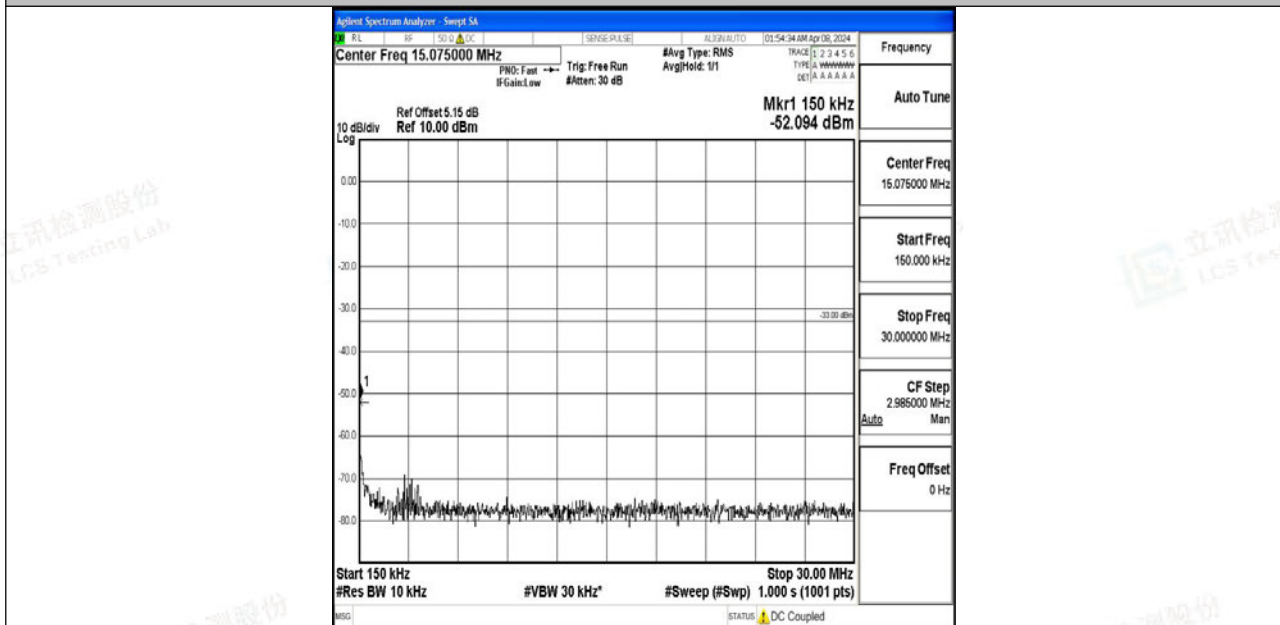
Band4_3MHz_64QAM_20385_1RB#0_0.15~30_0.15~30
