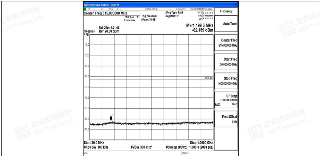
Band4_10MHz_64QAM_20175_1RB#0_30~1000_30~1000
