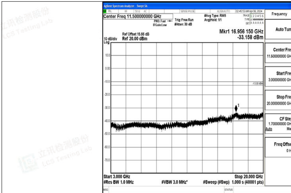
Band4_15MHz_64QAM_20325_1RB#0_3000~20000_3000~20000
