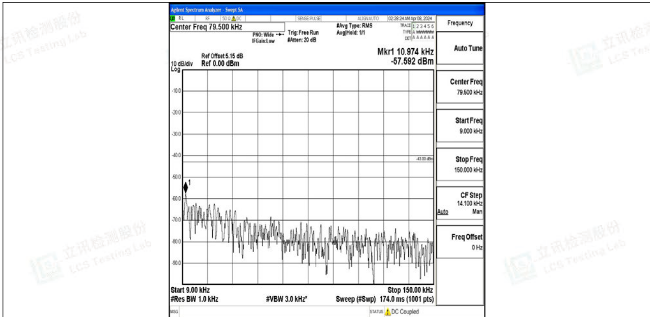
Band4_10MHz_64QAM_20175_1RB#0_0.009~0.15_0.009~0.15
