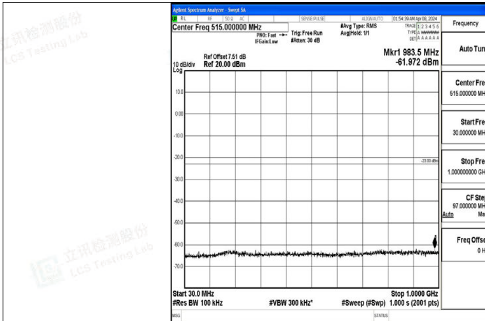
Band4_3MHz_64QAM_20385_1RB#0_30~1000_30~1000
