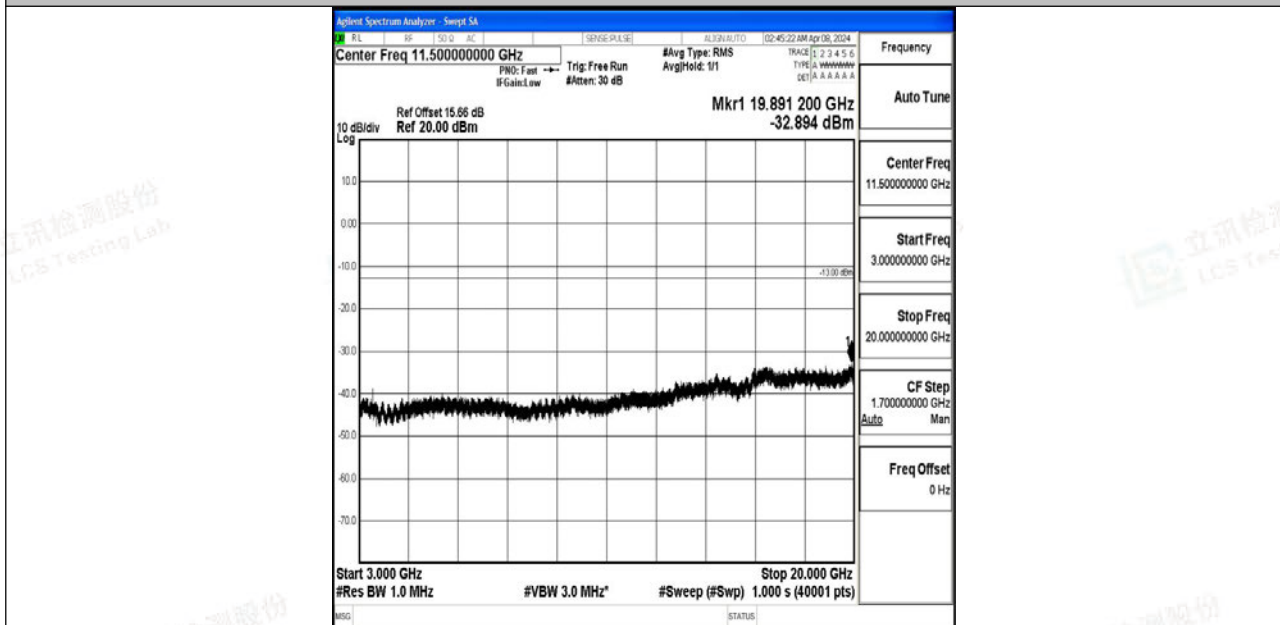
Band4_15MHz_QPSK_20325_1RB#0_3000~20000_3000~20000
