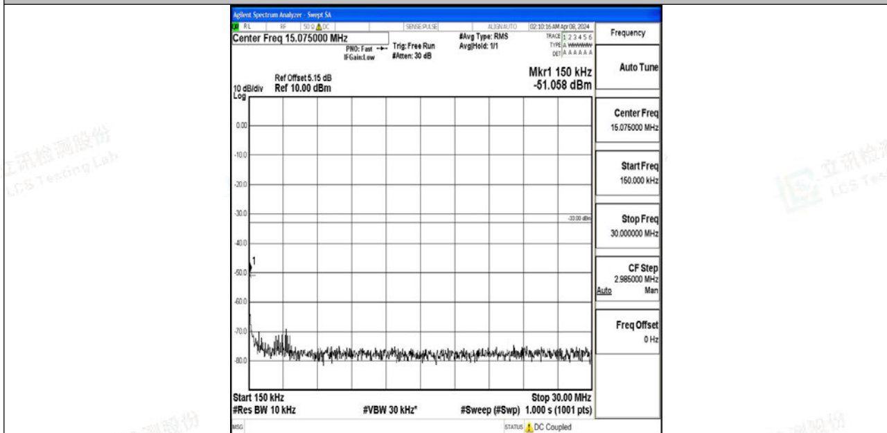
Band4_5MHz_64QAM_19975_1RB#0_0.15~30_0.15~30
