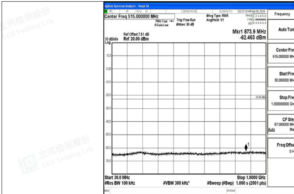
Band4_10MHz_64QAM_20000_1RB#0_30~1000_30~1000
