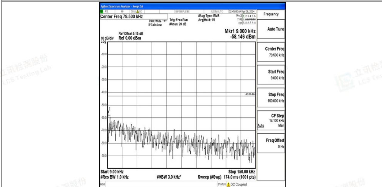
Band4_15MHz_QPSK_20325_1RB#0_0.009~0.15_0.009~0.15
