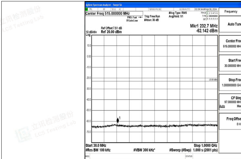
Band4_10MHz_64QAM_20350_1RB#0_30~1000_30~1000
