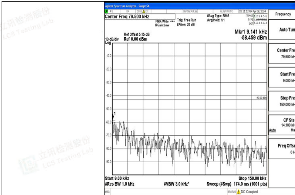
Band4_5MHz_64QAM_20175_1RB#0_0.009~0.15_0.009~0.15
