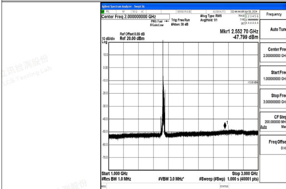
Band4_15MHz_64QAM_20175_1RB#0_1000~3000_1000~3000
