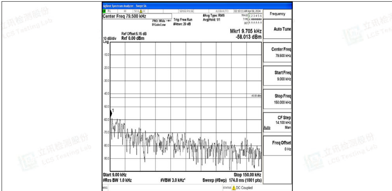
Band4_5MHz_64QAM_19975_1RB#0_0.009~0.15_0.009~0.15
