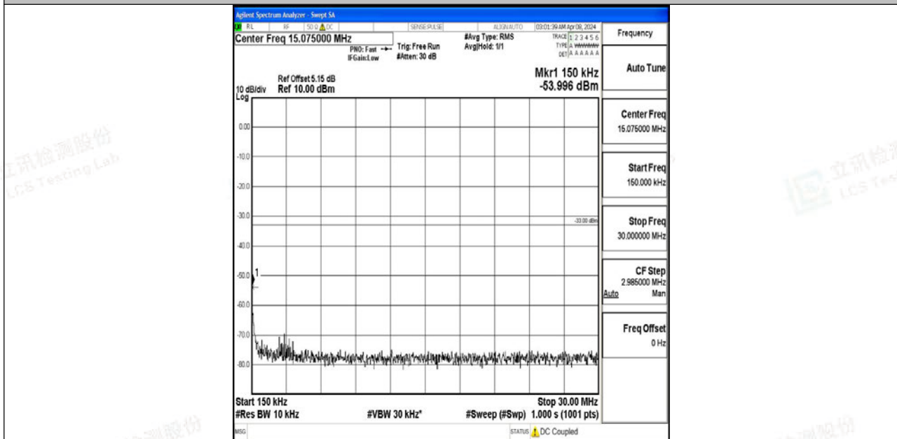
Band4_20MHz_64QAM_20300_1RB#0_0.15~30_0.15~30
