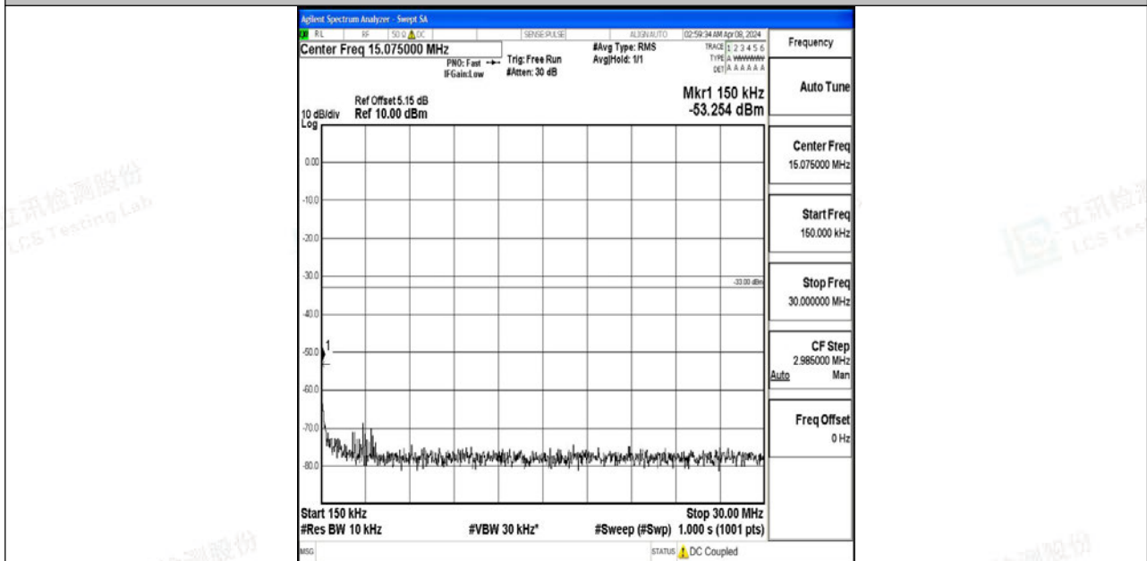
Band4_20MHz_64QAM_20050_1RB#0_0.15~30_0.15~30
