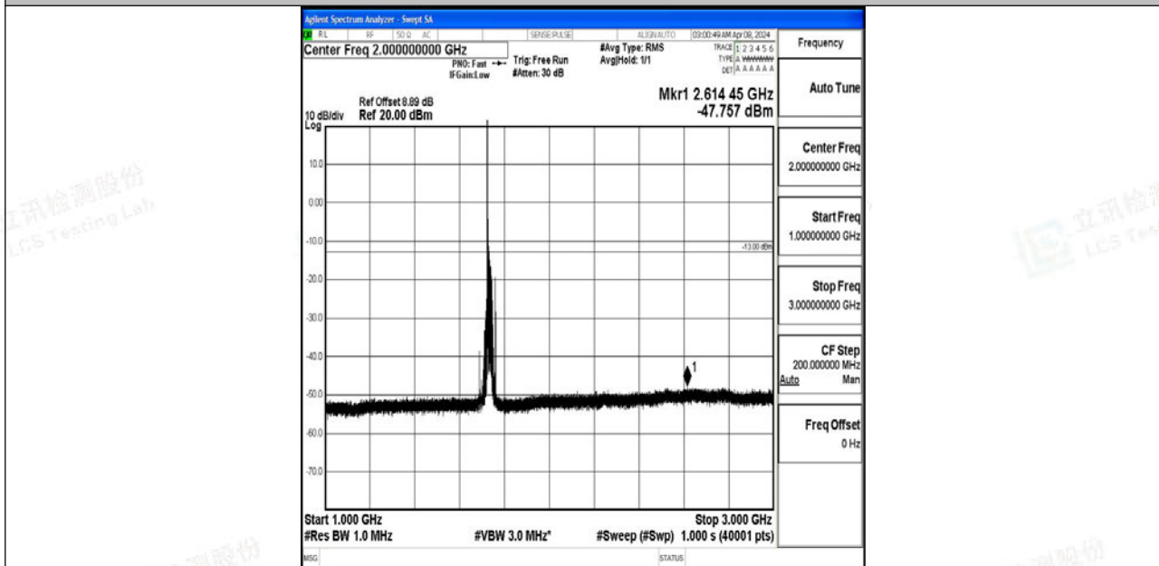
Band4_20MHz_64QAM_20175_1RB#0_1000~3000_1000~3000
