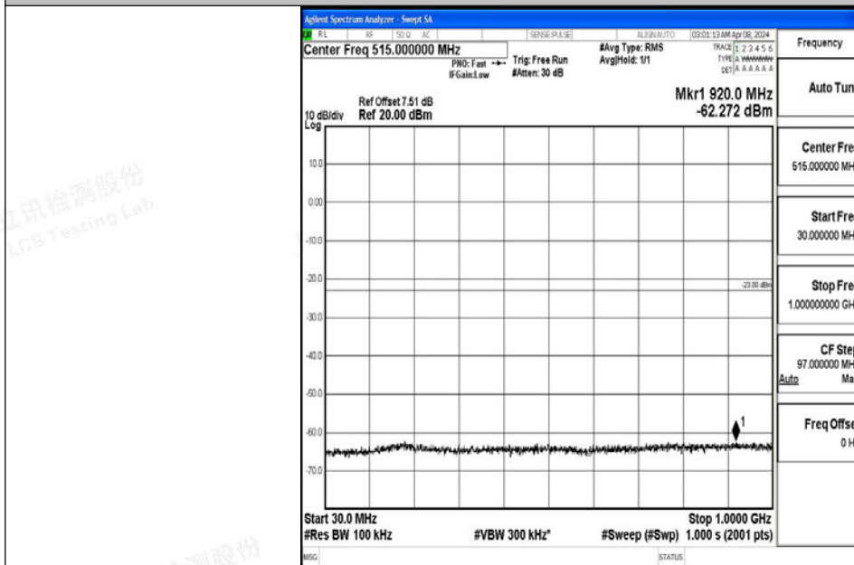
Band4_20MHz_QPSK_20300_1RB#0_30~1000_30~1000
