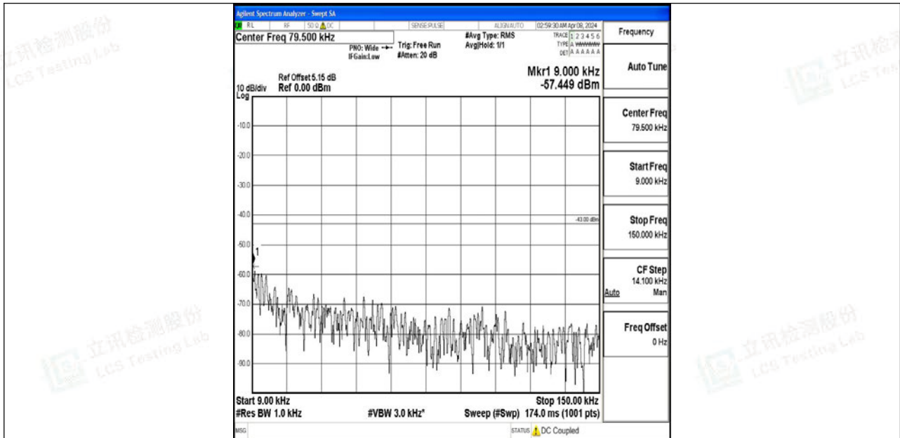
Band4_20MHz_64QAM_20050_1RB#0_0.009~0.15_0.009~0.15
