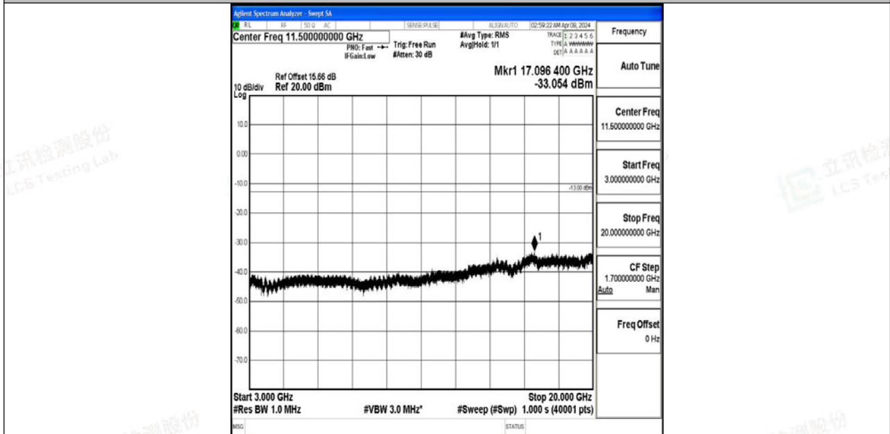
Band4_20MHz_QPSK_20050_1RB#0_3000~20000_3000~20000
