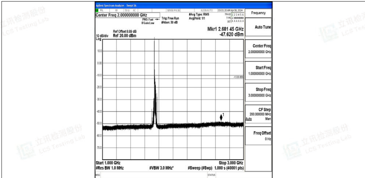
Band4_20MHz_QPSK_20300_1RB#0_1000~3000_1000~3000
