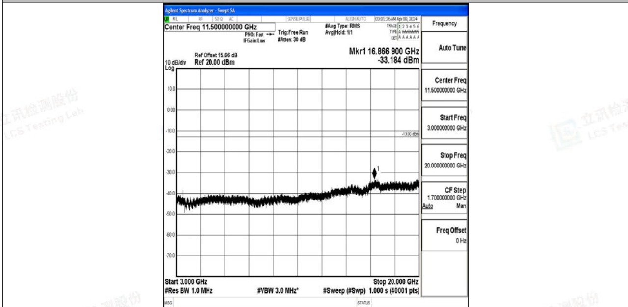
Band4_20MHz_QPSK_20300_1RB#0_3000~20000_3000~20000
