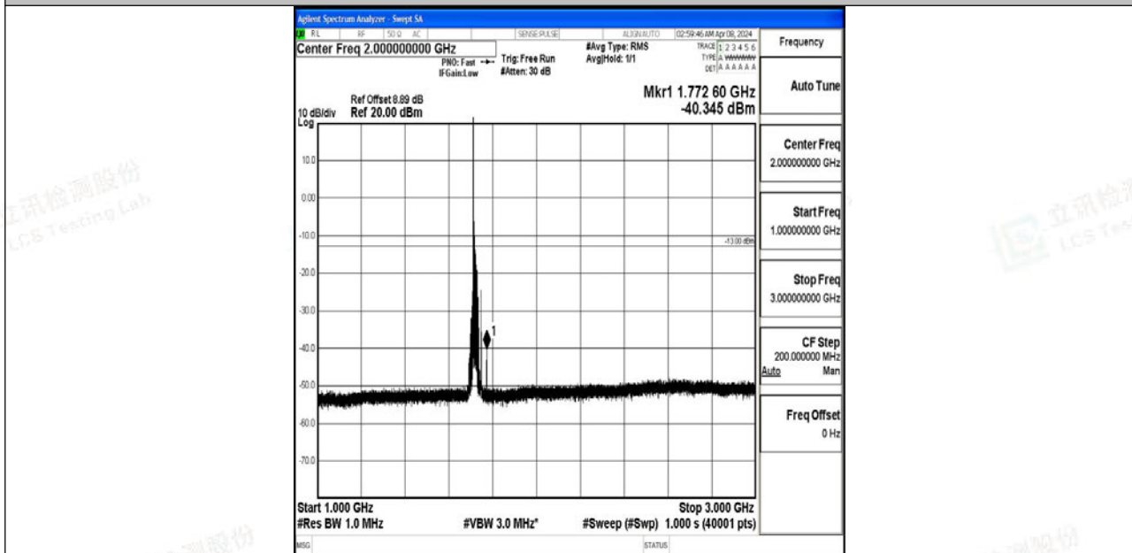
Band4_20MHz_64QAM_20050_1RB#0_1000~3000_1000~3000
