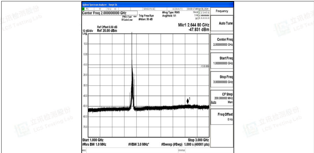
Band4_20MHz_QPSK_20175_1RB#0_1000~3000_1000~3000
