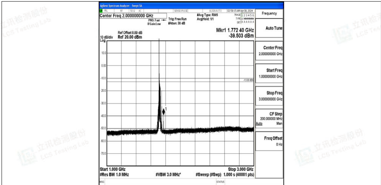
Band4_20MHz_QPSK_20050_1RB#0_1000~3000_1000~3000
