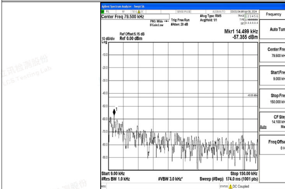
Band4_20MHz_QPSK_20300_1RB#0_0.009~0.15_0.009~0.15
