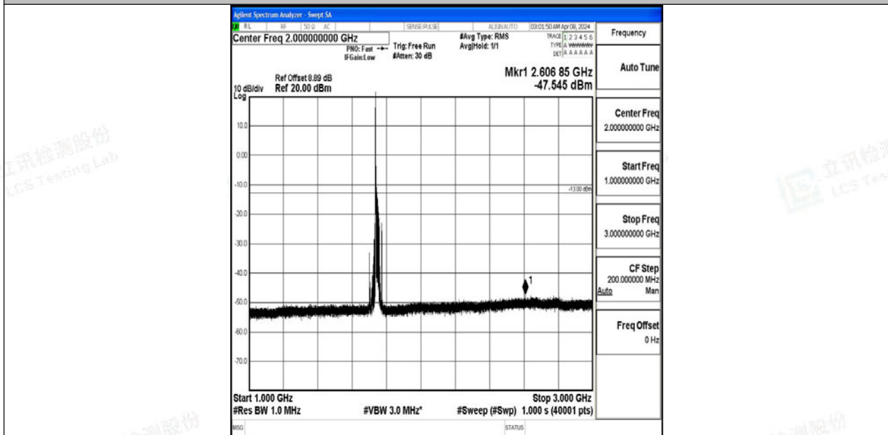
Band4_20MHz_64QAM_20300_1RB#0_1000~3000_1000~3000
