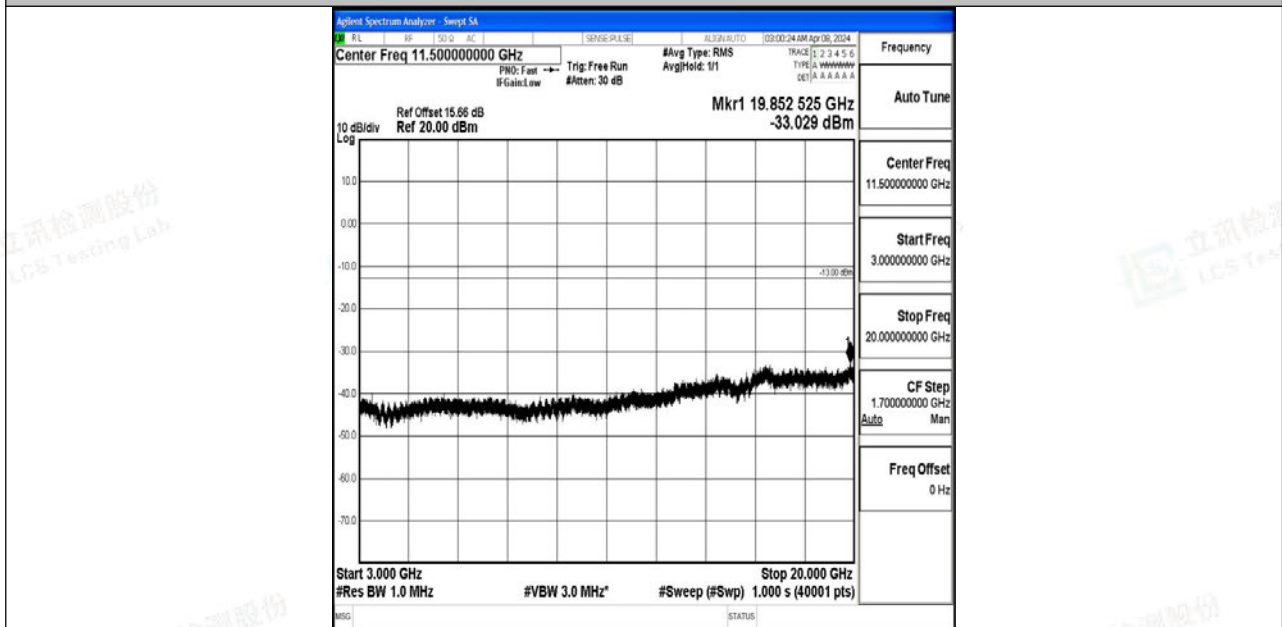
Band4_20MHz_QPSK_20175_1RB#0_3000~20000_3000~20000
