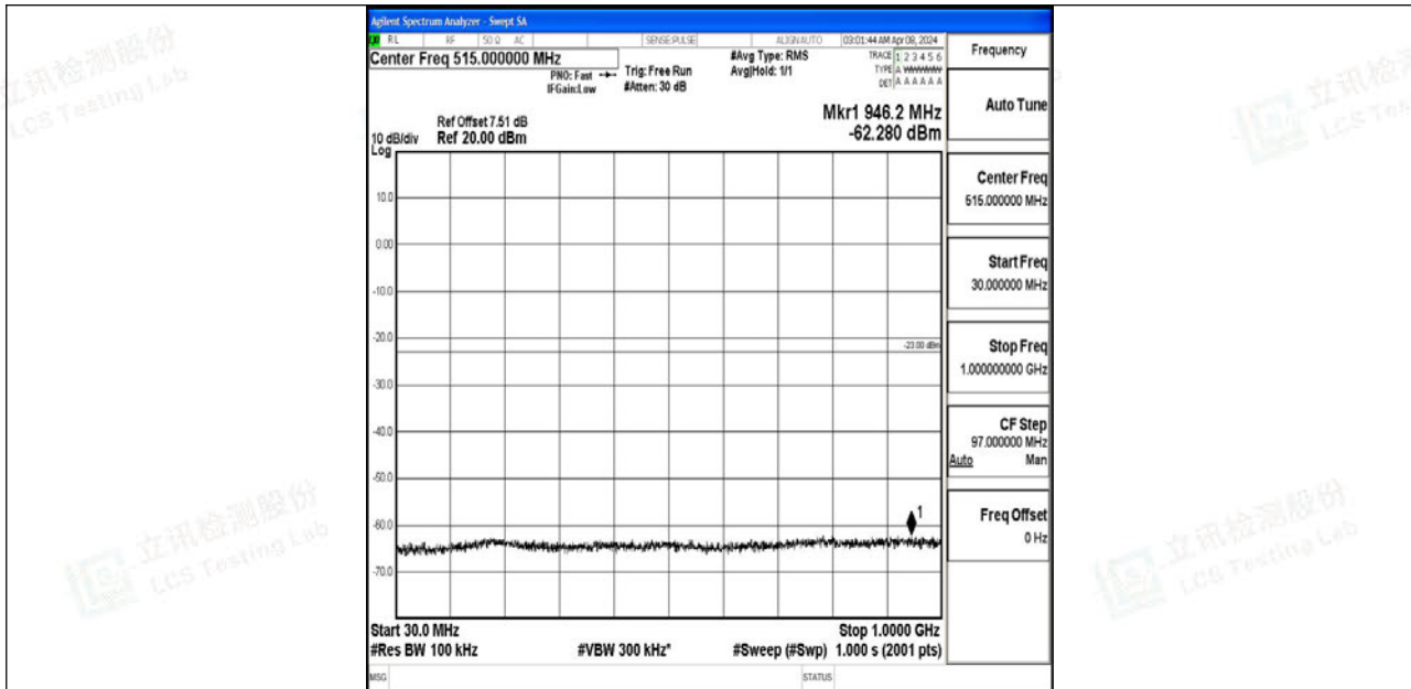
Band4_20MHz_64QAM_20300_1RB#0_30~1000_30~1000
