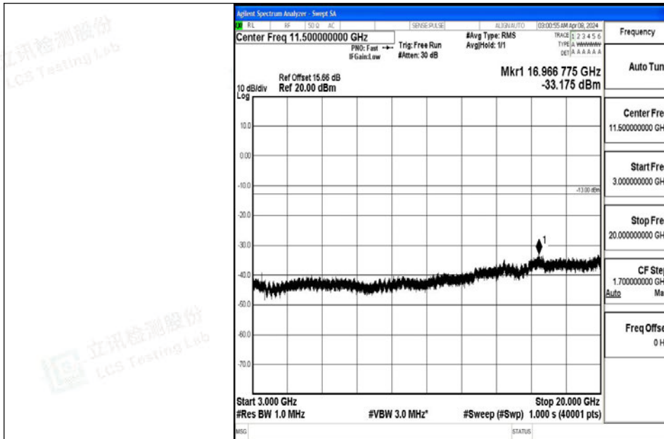
Band4_20MHz_64QAM_20175_1RB#0_3000~20000_3000~20000
