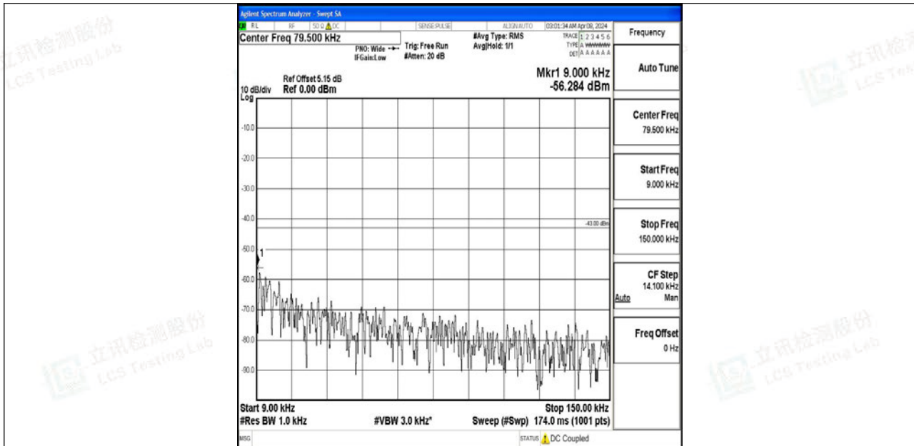
Band4_20MHz_64QAM_20300_1RB#0_0.009~0.15_0.009~0.15
