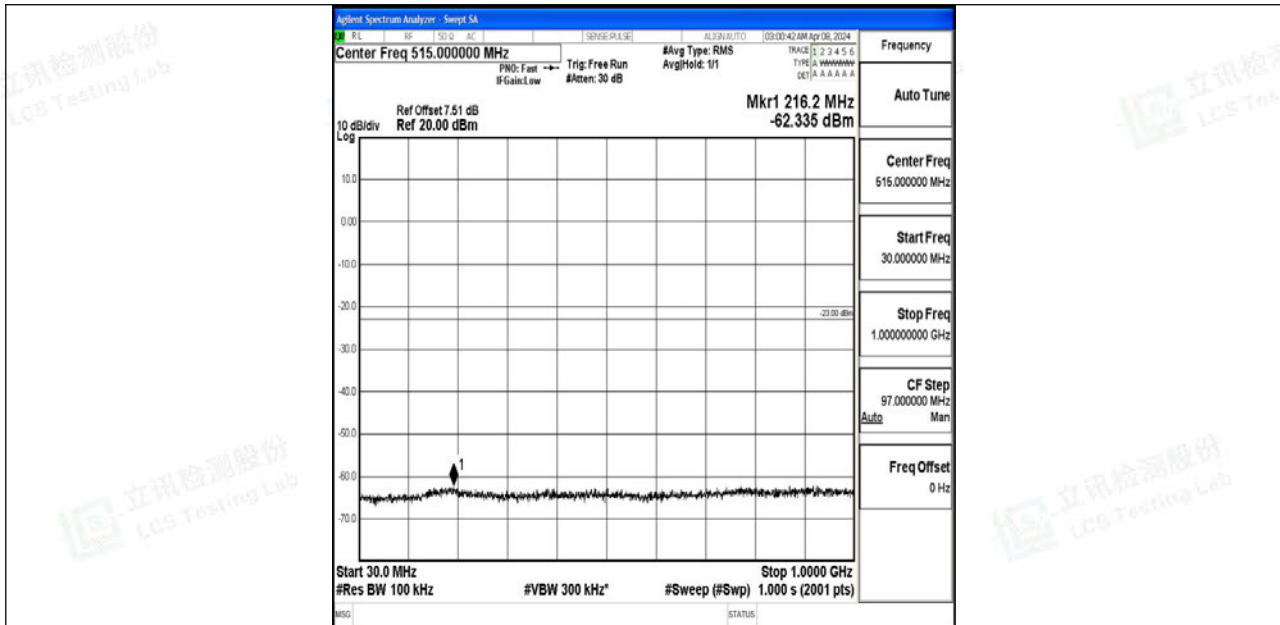
Band4_20MHz_64QAM_20175_1RB#0_30~1000_30~1000
