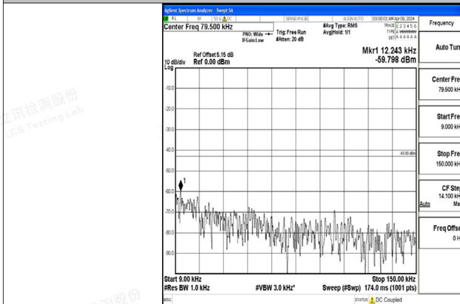
Band4_20MHz_QPSK_20175_1RB#0_0.009~0.15_0.009~0.15
