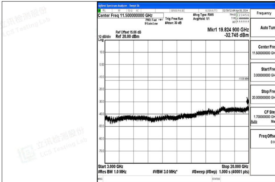
Band4_20MHz_64QAM_20050_1RB#0_3000~20000_3000~20000
