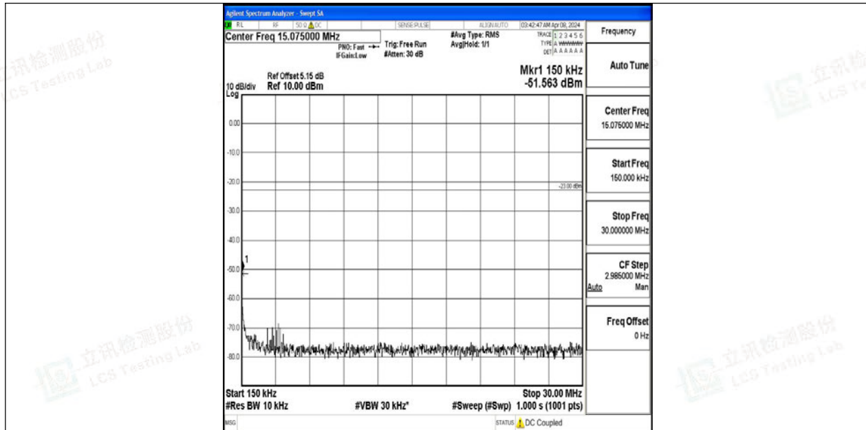
Band12_3MHz_64QAM_23165_1RB#0_0.15~30_0.15~30
