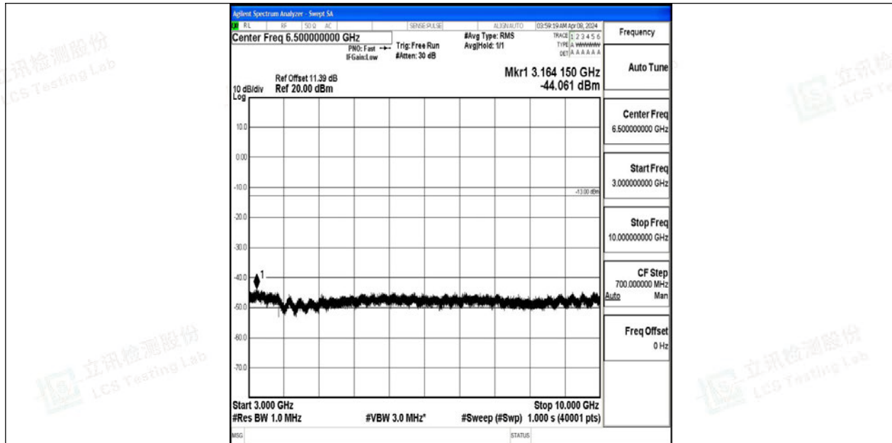
Band12_5MHz_QPSK_23035_1RB#0_3000~10000_3000~10000
