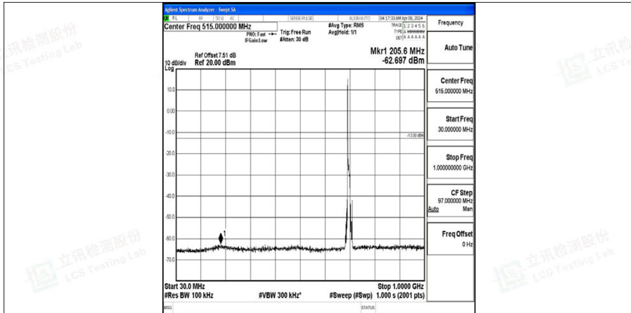
Band12_10MHz_QPSK_23060_1RB#0_30~1000_30~1000
