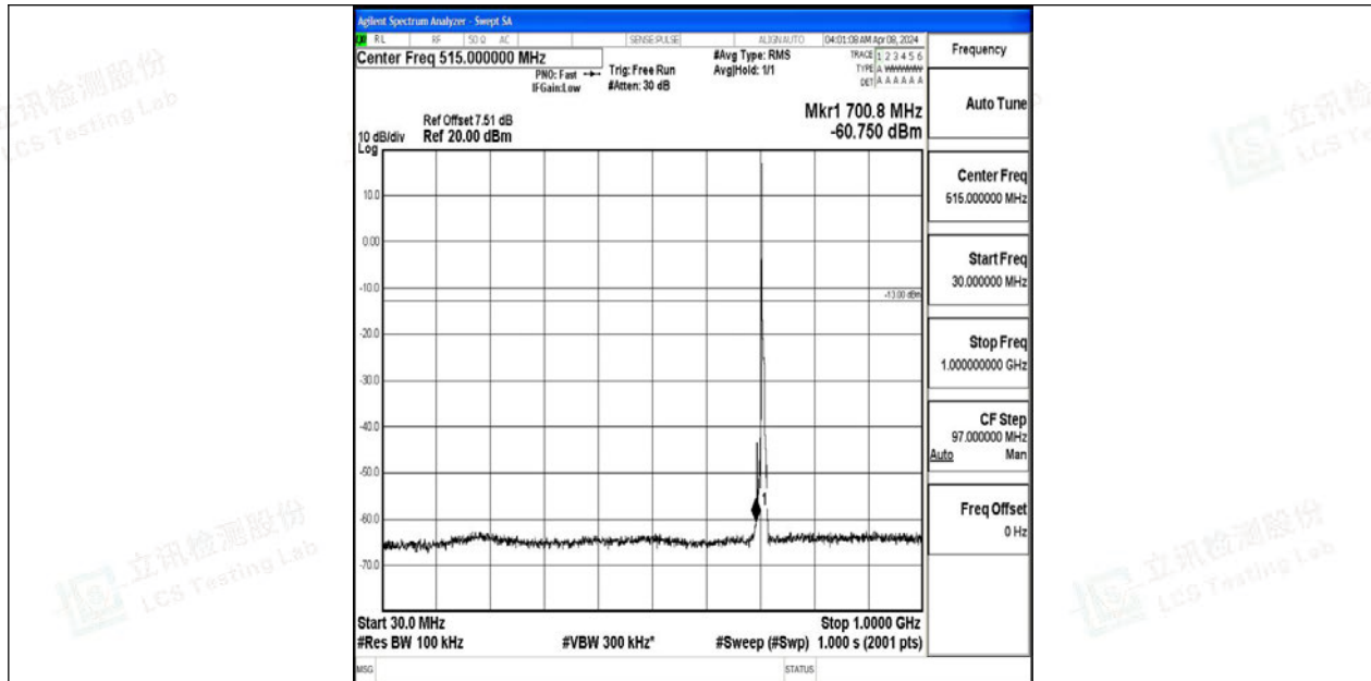
Band12_5MHz_QPSK_23155_1RB#0_30~1000_30~1000
