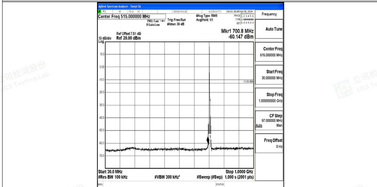
Band12_5MHz_64QAM_23155_1RB#0_30~1000_30~1000
