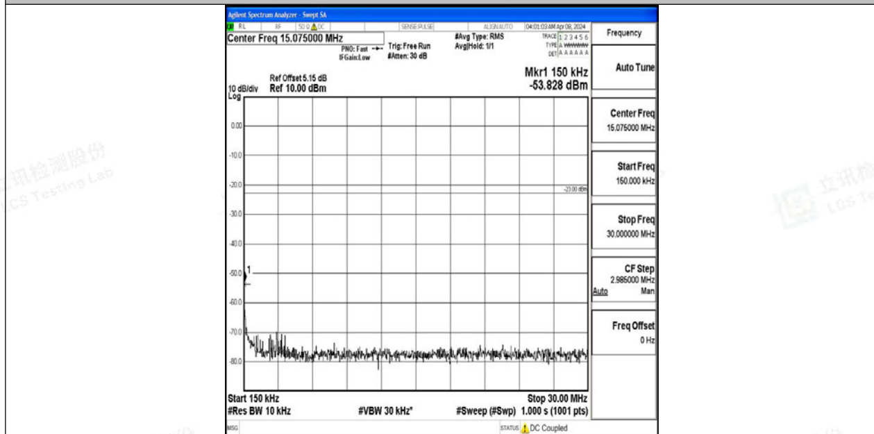
Band12_5MHz_QPSK_23155_1RB#0_0.15~30_0.15~30
