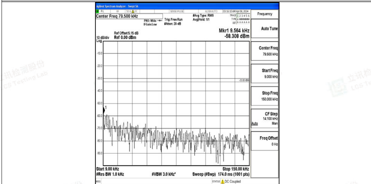
Band12_1.4MHz_64QAM_23095_1RB#0_0.009~0.15_0.009~0.15
