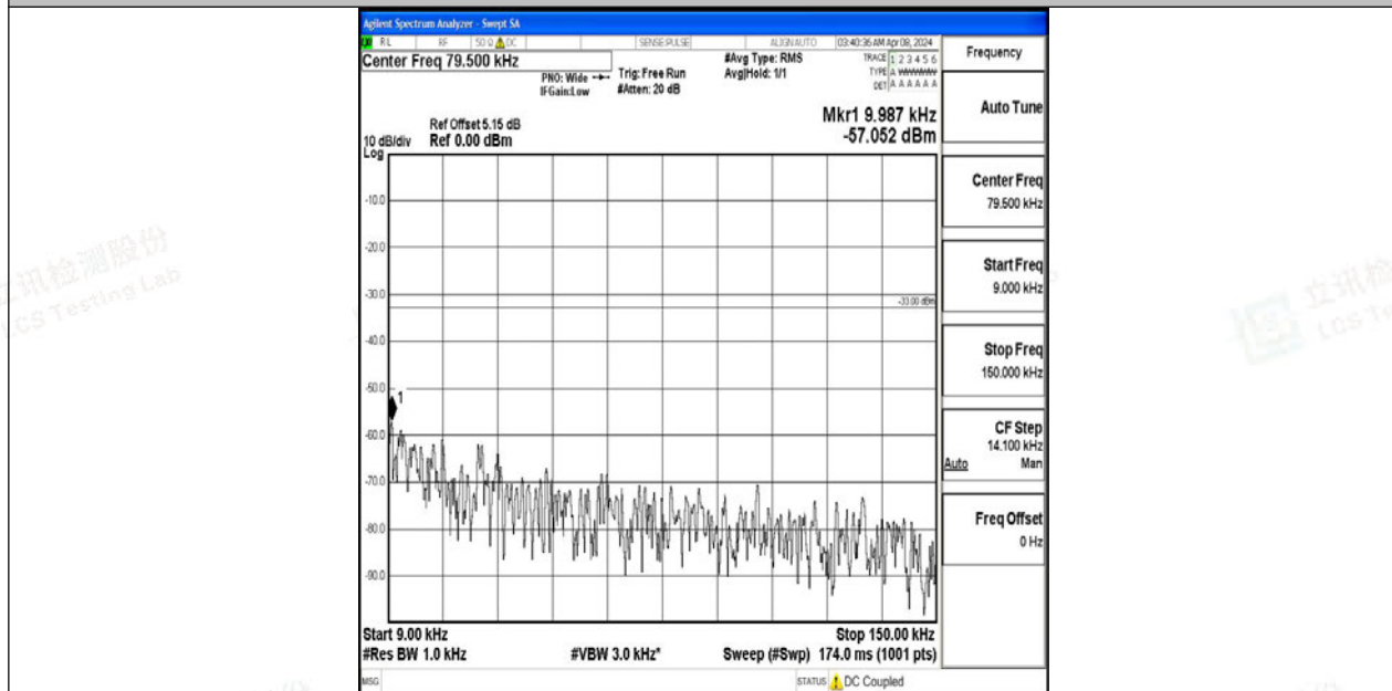
Band12_3MHz_64QAM_23025_1RB#0_0.009~0.15_0.009~0.15
