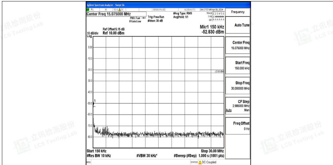
Band12_10MHz_64QAM_23060_1RB#0_0.15~30_0.15~30
