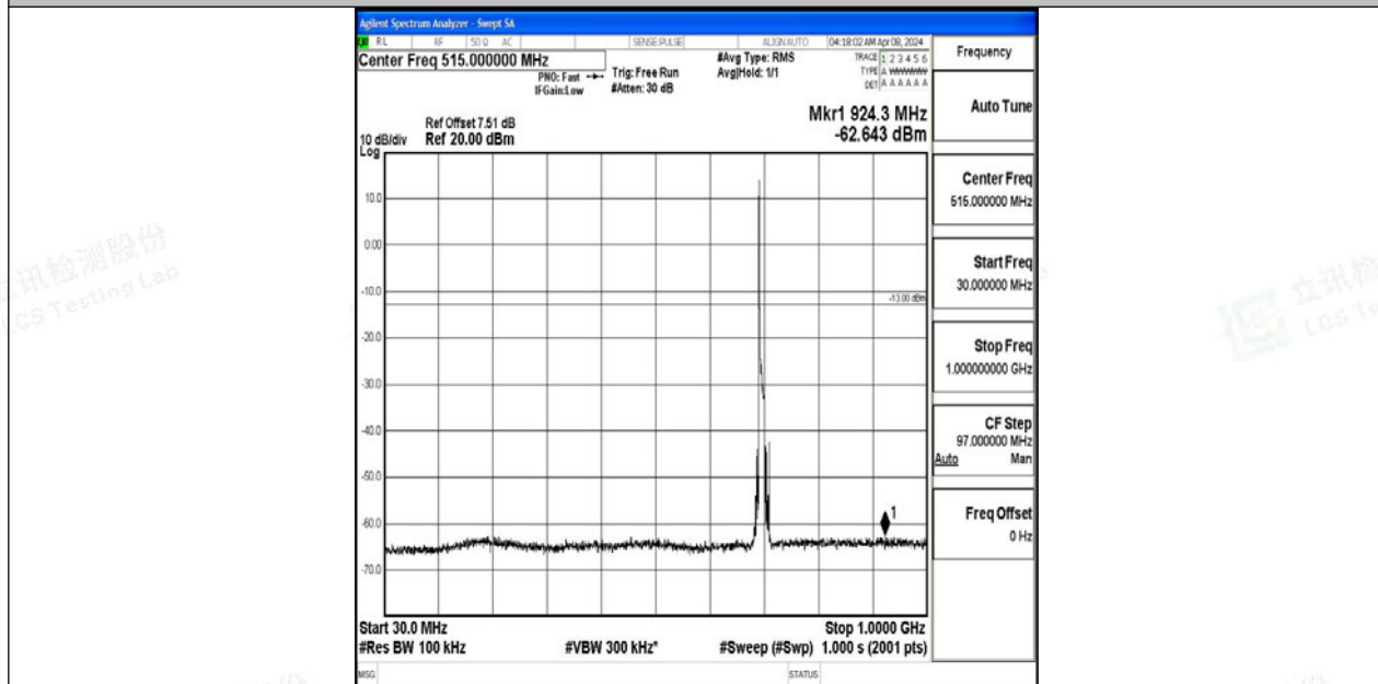
Band12_10MHz_64QAM_23060_1RB#0_30~1000_30~1000
