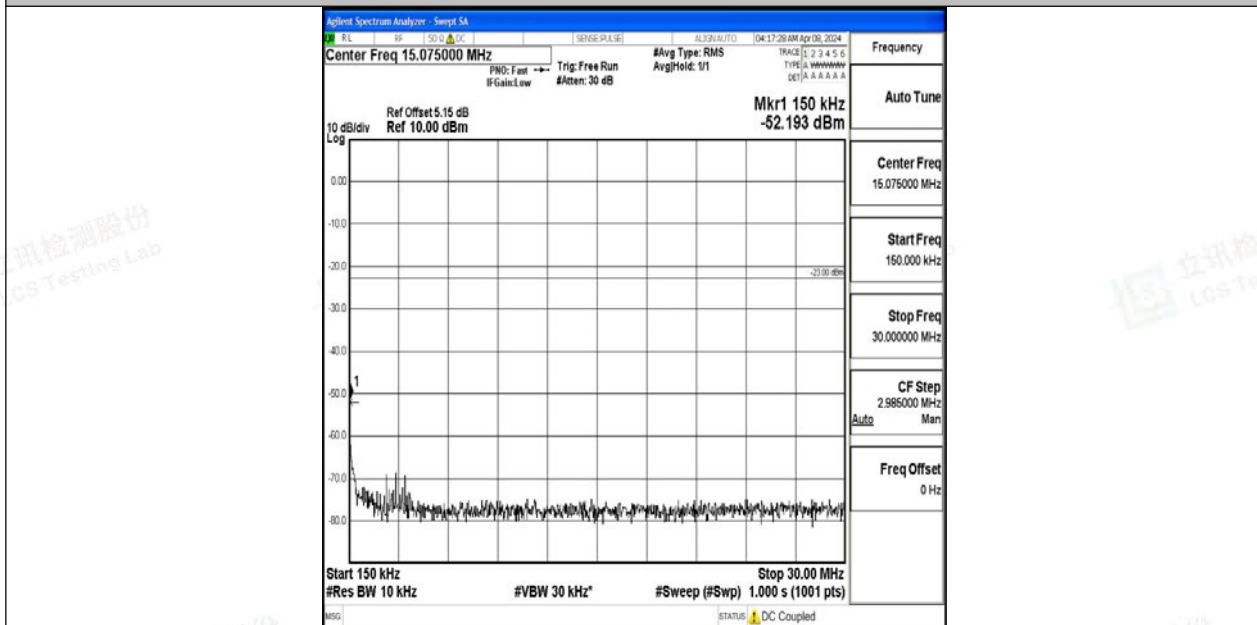
Band12_10MHz_QPSK_23060_1RB#0_0.15~30_0.15~30
