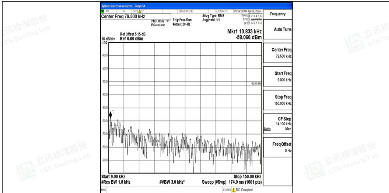
Band12_5MHz_QPSK_23095_1RB#0_0.009~0.15_0.009~0.15
