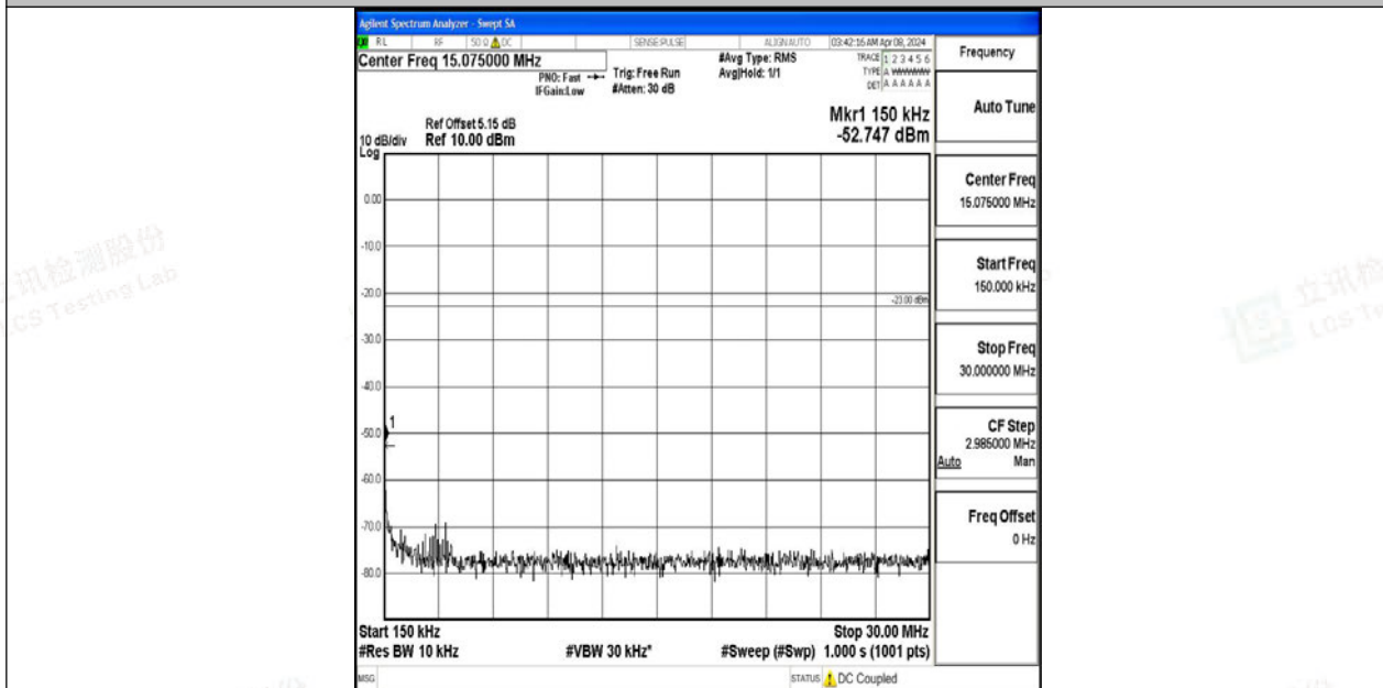
Band12_3MHz_QPSK_23165_1RB#0_0.15~30_0.15~30
