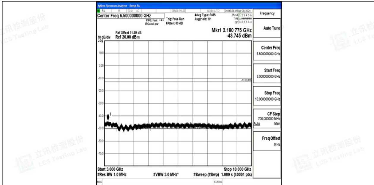
Band12_5MHz_QPSK_23095_1RB#0_3000~10000_3000~10000
