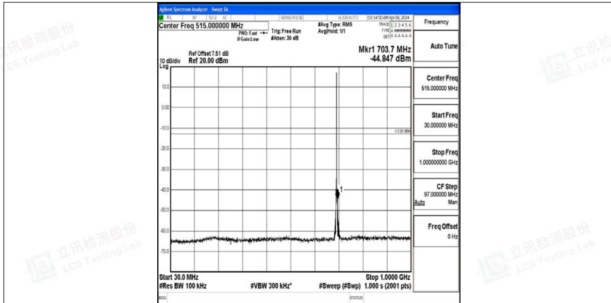
Band12_1.4MHz_QPSK_23017_1RB#0_30~1000_30~1000
