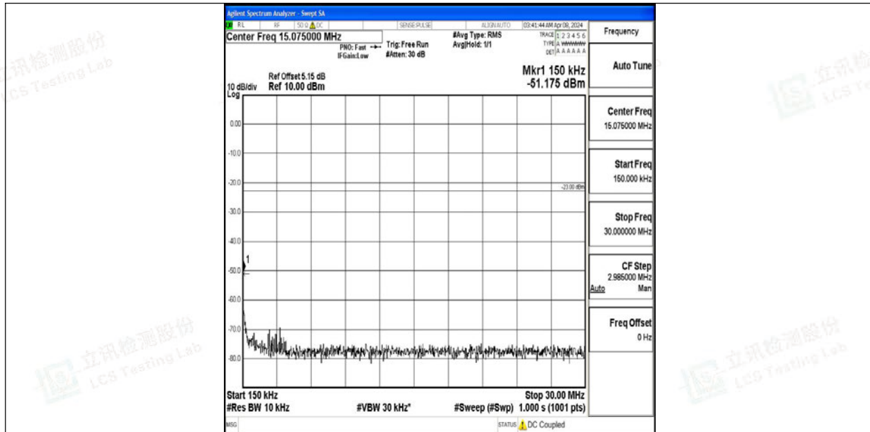
Band12_3MHz_64QAM_23095_1RB#0_0.15~30_0.15~30
