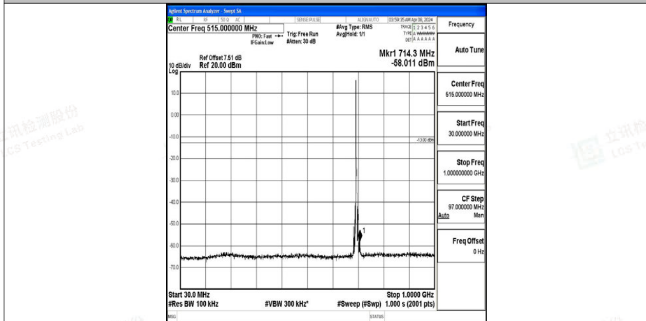
Band12_5MHz_64QAM_23035_1RB#0_30~1000_30~1000
