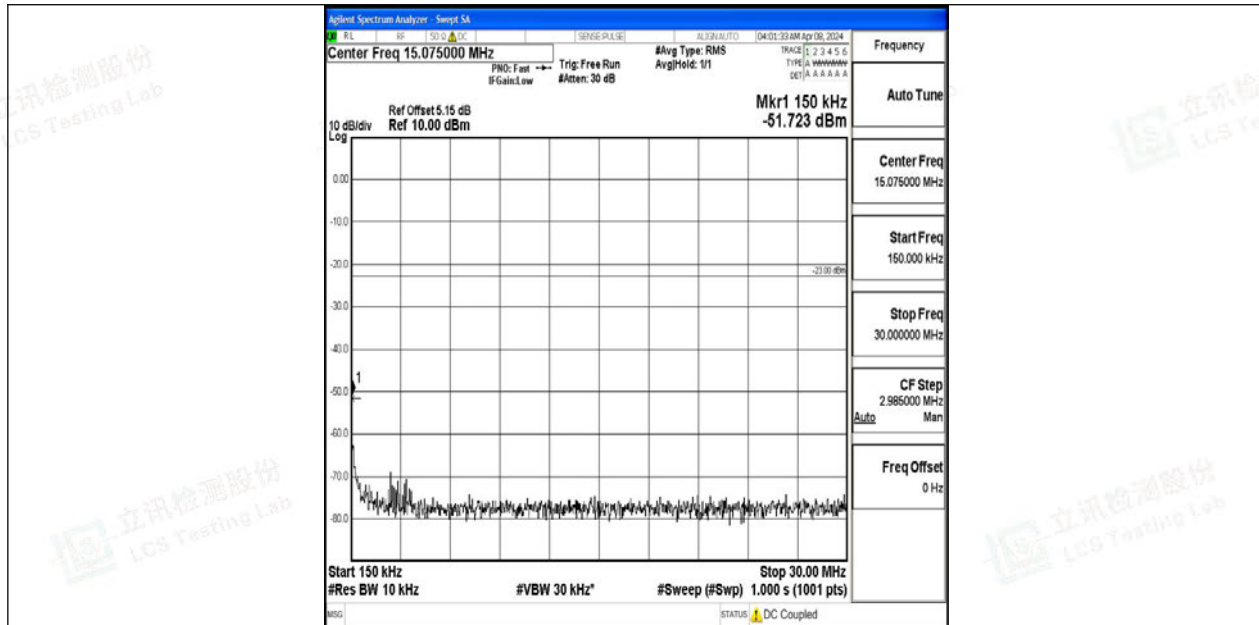
Band12_5MHz_64QAM_23155_1RB#0_0.15~30_0.15~30
