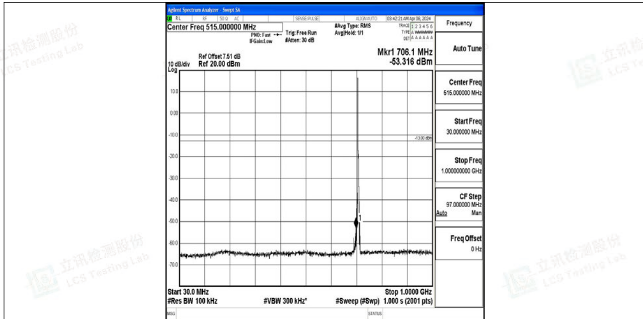
Band12_3MHz_QPSK_23165_1RB#0_30~1000_30~1000
