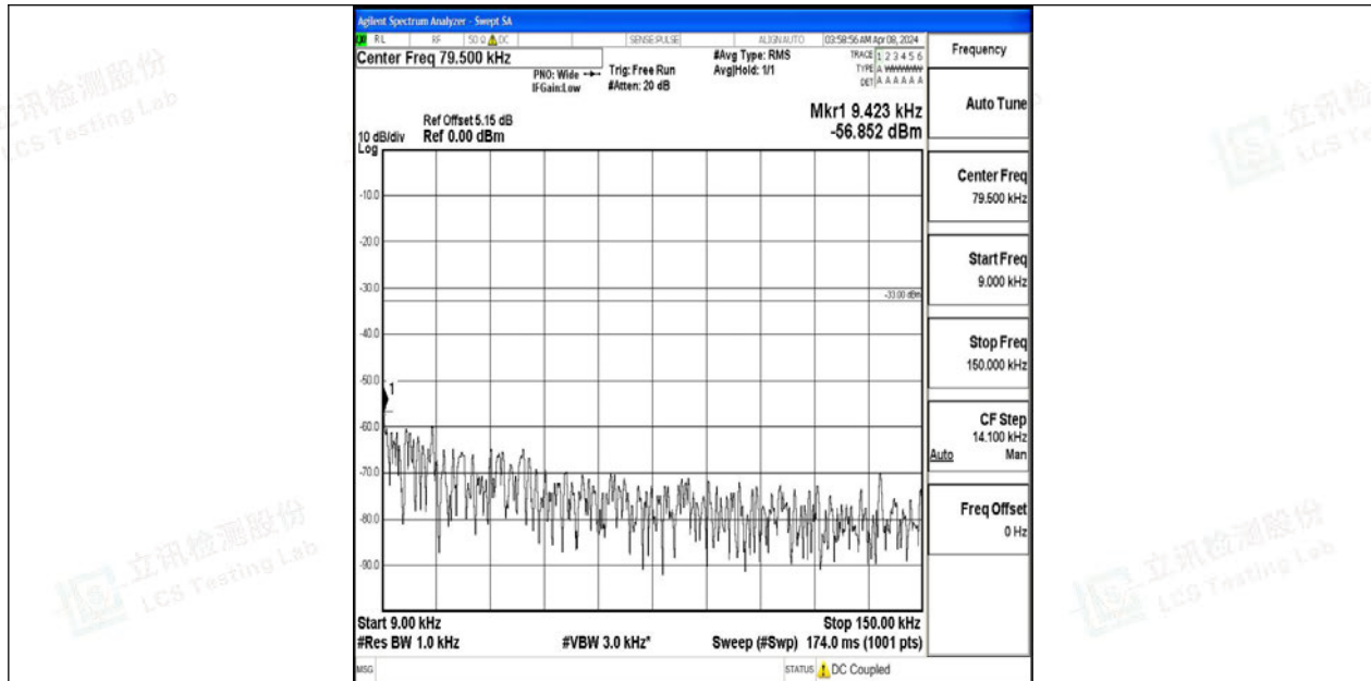
Band12_5MHz_QPSK_23035_1RB#0_0.009~0.15_0.009~0.15
