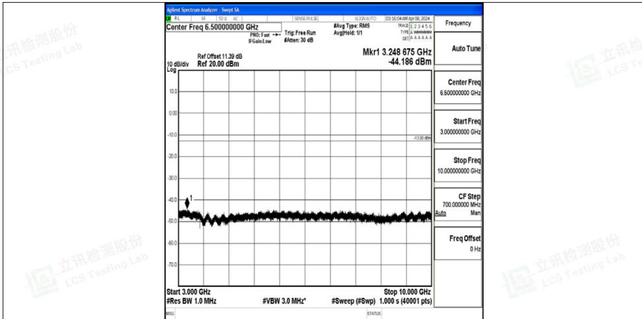
Band12_1.4MHz_QPSK_23095_1RB#0_3000~10000_3000~10000
