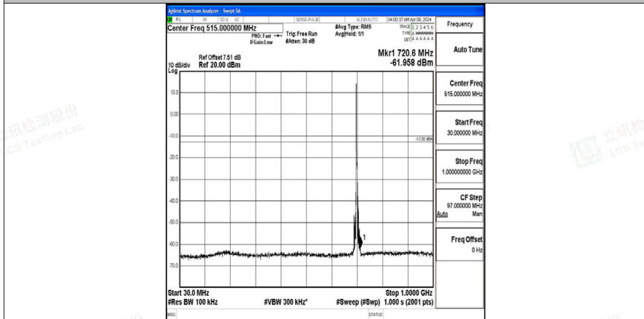
Band12_5MHz_64QAM_23095_1RB#0_30~1000_30~1000
