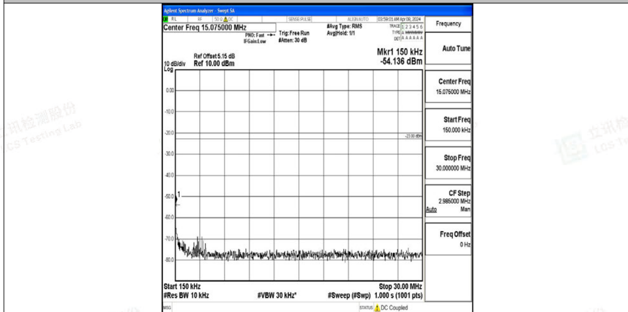
Band12_5MHz_QPSK_23035_1RB#0_0.15~30_0.15~30
