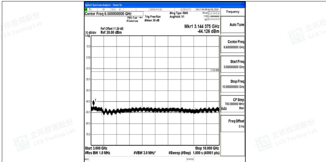
Band12_10MHz_QPSK_23060_1RB#0_3000~10000_3000~10000
