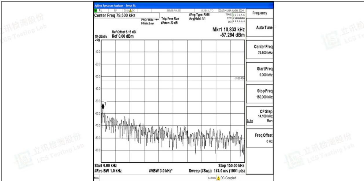
Band12_1.4MHz_QPSK_23095_1RB#0_0.009~0.15_0.009~0.15
