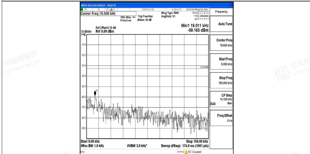
Band12_3MHz_64QAM_23165_1RB#0_0.009~0.15_0.009~0.15
