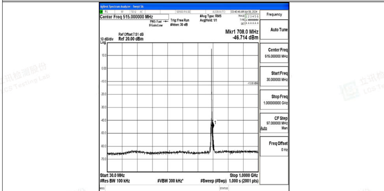
Band12_3MHz_64QAM_23025_1RB#0_30~1000_30~1000
