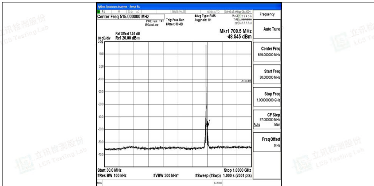
Band12_3MHz_QPSK_23025_1RB#0_30~1000_30~1000
