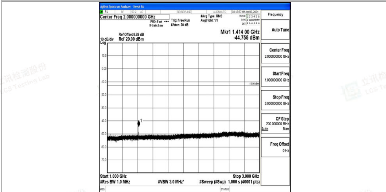
Band12_1.4MHz_QPSK_23095_1RB#0_1000~3000_1000~3000
