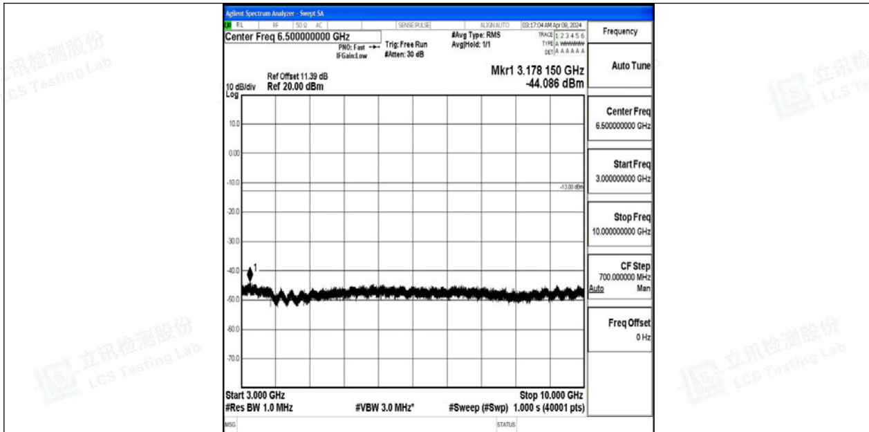
Band12_1.4MHz_QPSK_23173_1RB#0_3000~10000_3000~10000
