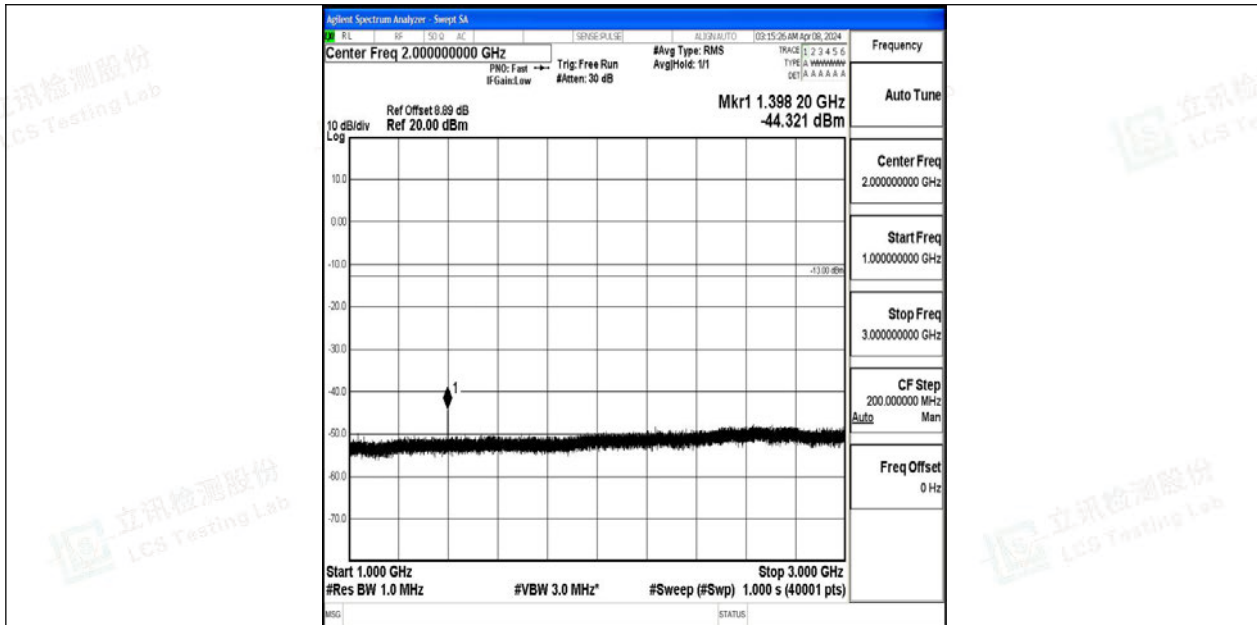
Band12_1.4MHz_64QAM_23017_1RB#0_1000~3000_1000~3000
