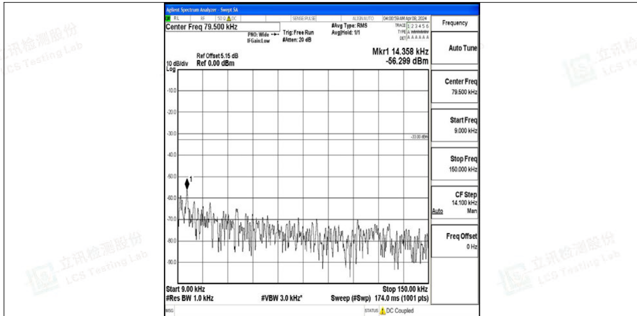
Band12_5MHz_QPSK_23155_1RB#0_0.009~0.15_0.009~0.15
