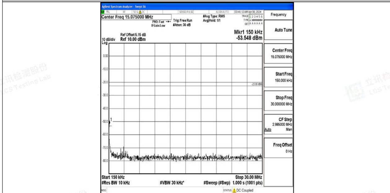
Band12_3MHz_QPSK_23095_1RB#0_0.15~30_0.15~30
