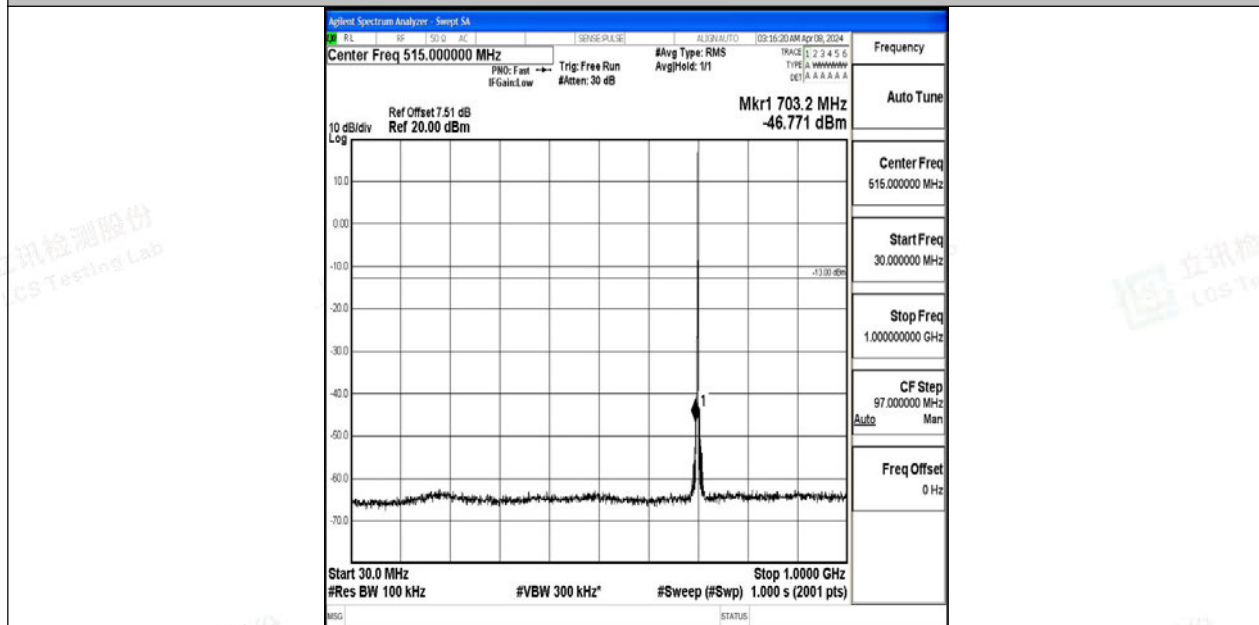
Band12_1.4MHz_64QAM_23095_1RB#0_30~1000_30~1000
