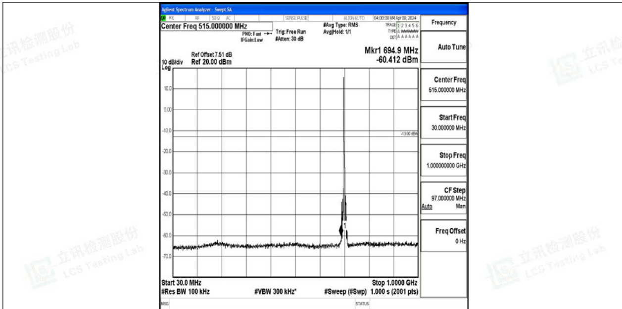
Band12_5MHz_QPSK_23095_1RB#0_30~1000_30~1000
