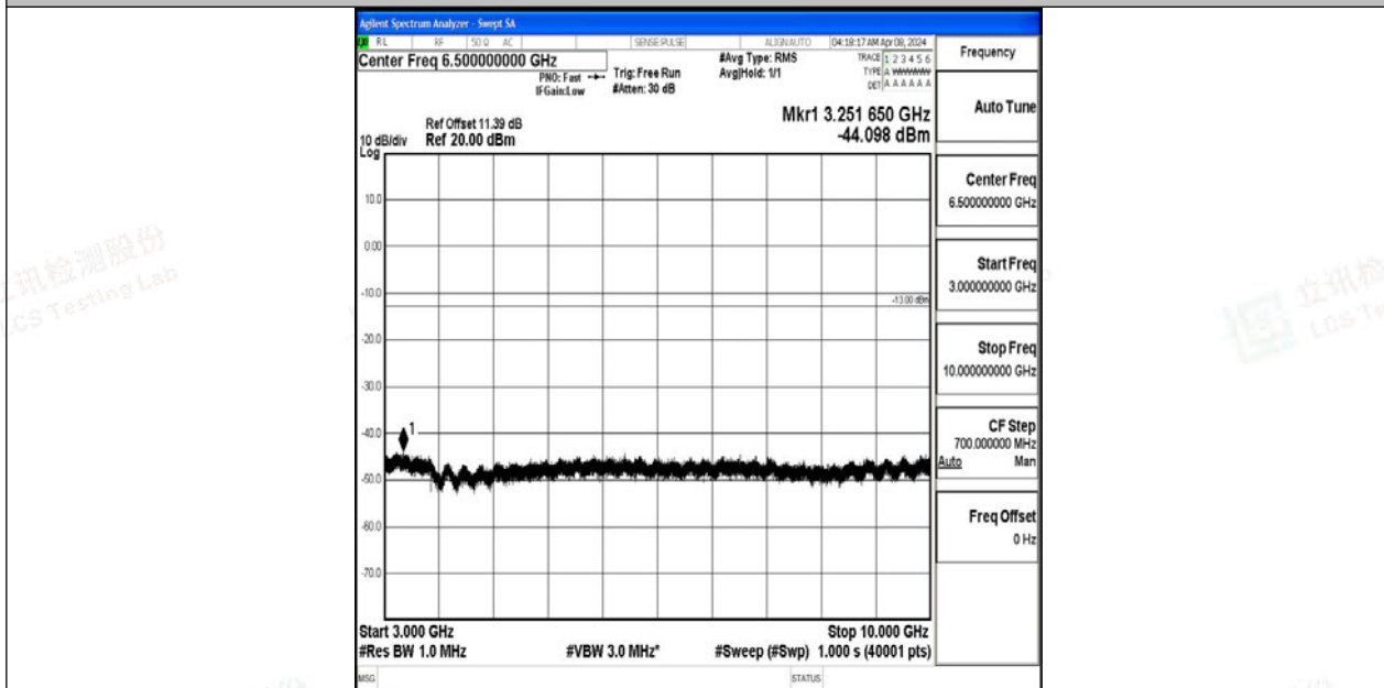
Band12_10MHz_64QAM_23060_1RB#0_3000~10000_3000~10000
