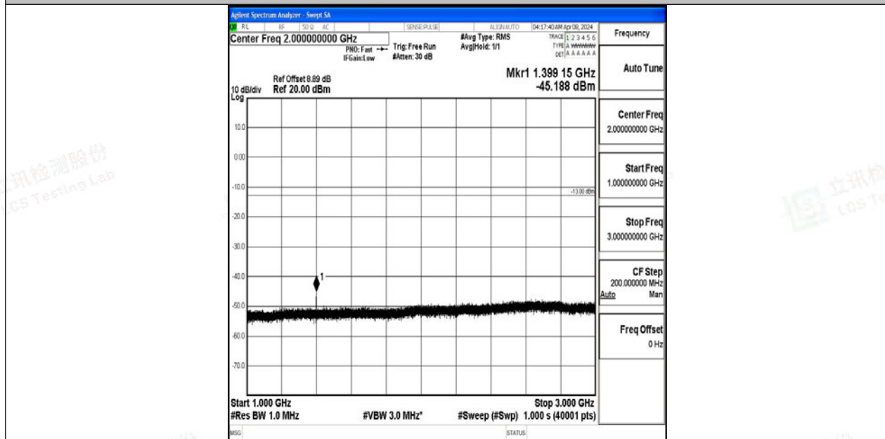
Band12_10MHz_QPSK_23060_1RB#0_1000~3000_1000~3000
