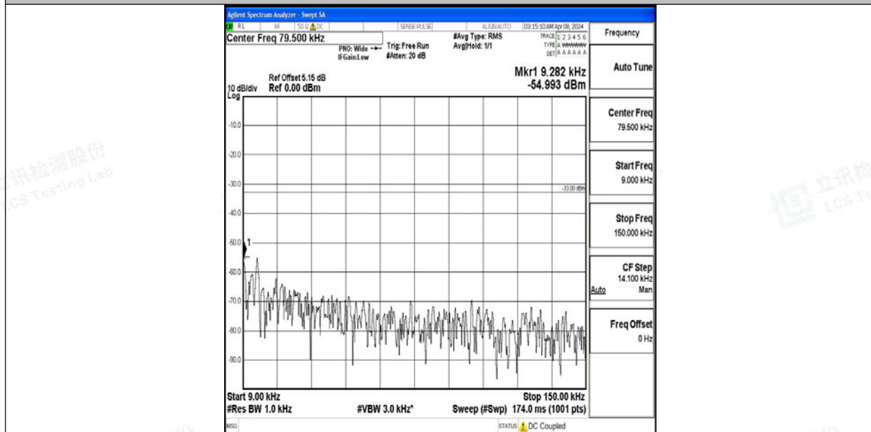
Band12_1.4MHz_64QAM_23017_1RB#0_0.009~0.15_0.009~0.15
