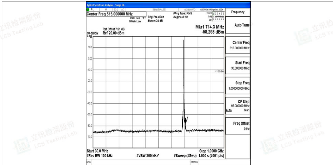
Band12_5MHz_QPSK_23035_1RB#0_30~1000_30~1000
