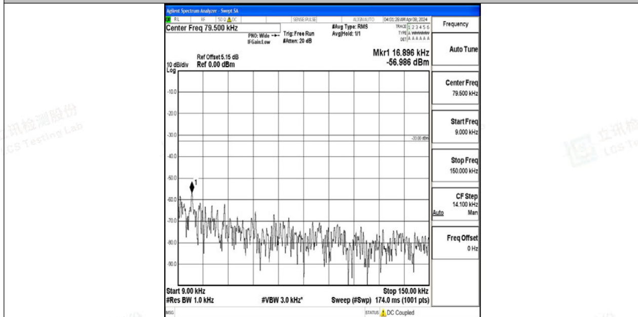
Band12_5MHz_64QAM_23155_1RB#0_0.009~0.15_0.009~0.15
