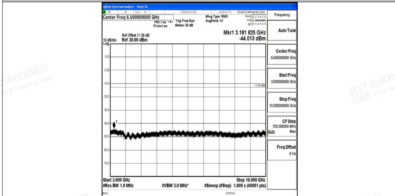
Band12_3MHz_64QAM_23095_1RB#0_3000~10000_3000~10000
