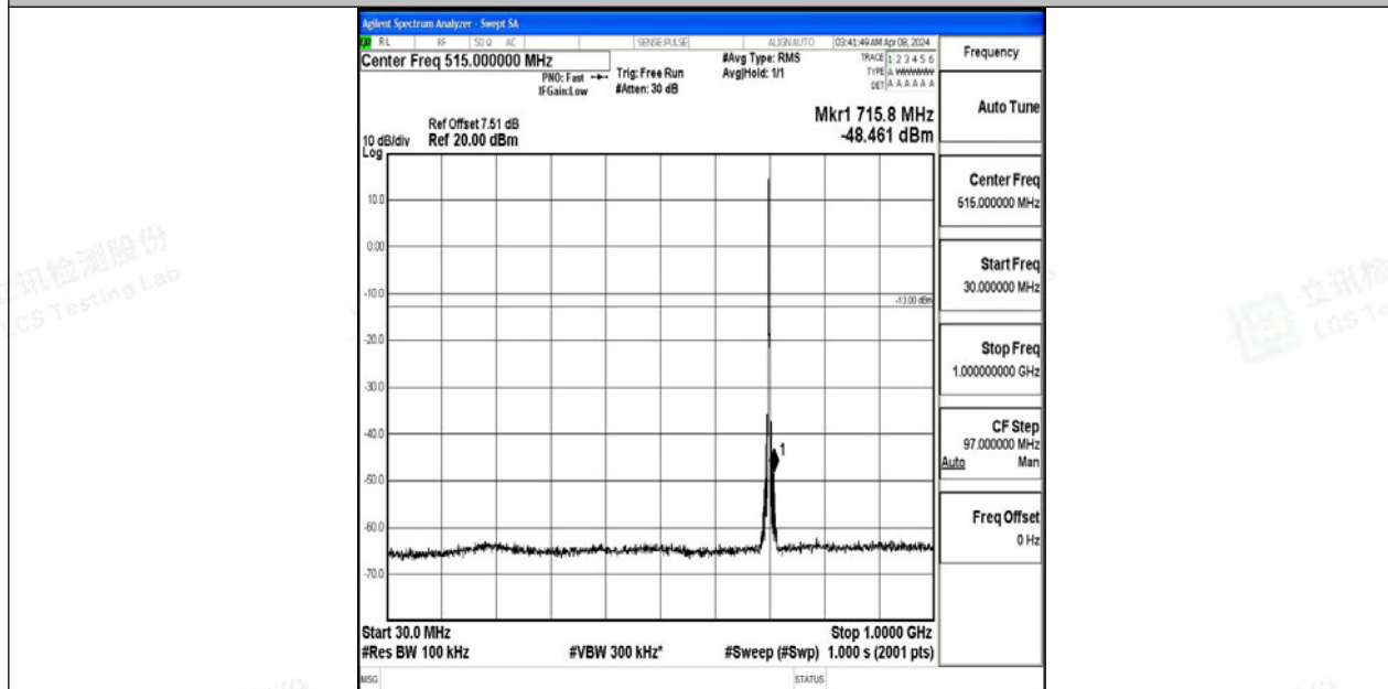
Band12_3MHz_64QAM_23095_1RB#0_30~1000_30~1000
