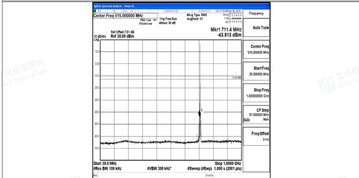
Band12_1.4MHz_64QAM_23173_1RB#0_30~1000_30~1000
