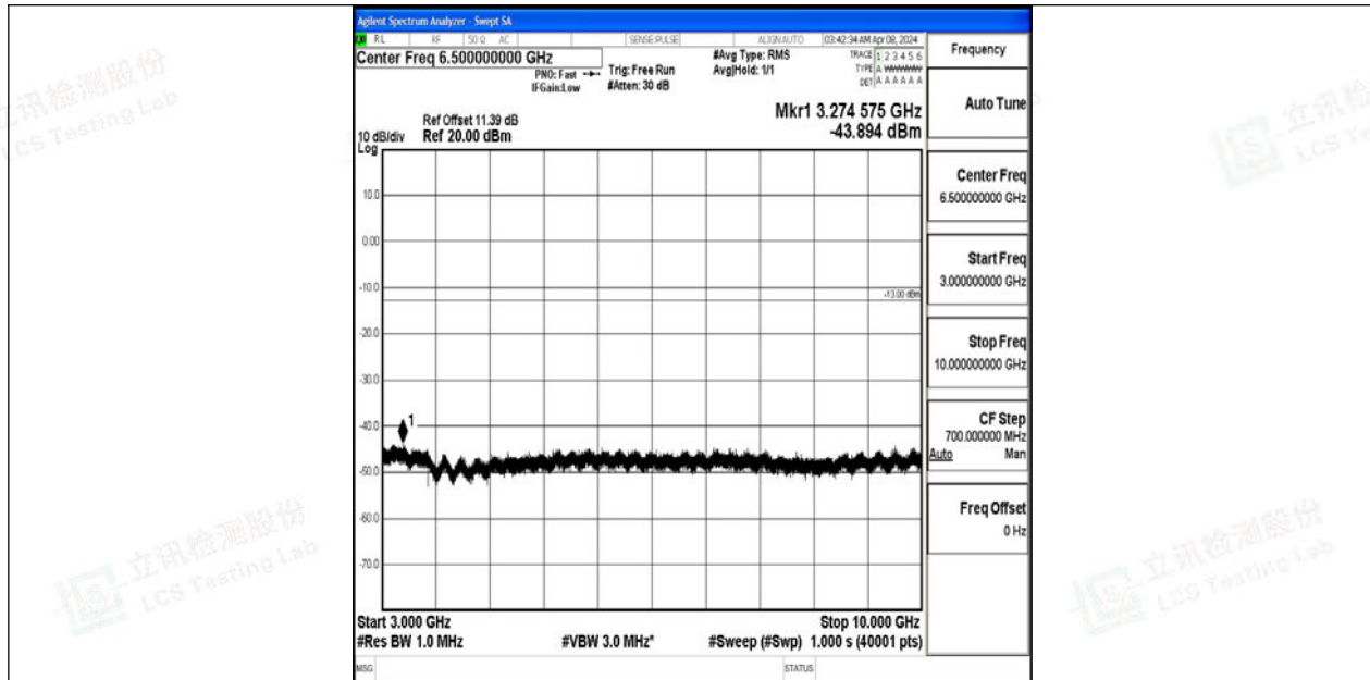
Band12_3MHz_QPSK_23165_1RB#0_3000~10000_3000~10000
