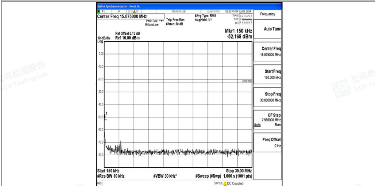
Band12_1.4MHz_QPSK_23095_1RB#0_0.15~30_0.15~30
