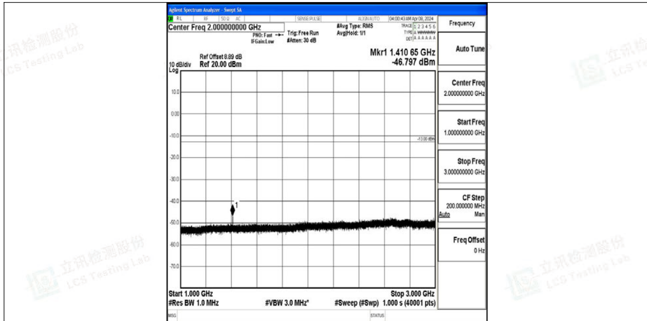
Band12_5MHz_64QAM_23095_1RB#0_1000~3000_1000~3000
