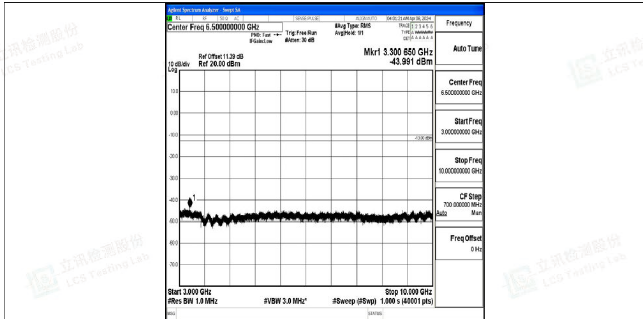
Band12_5MHz_QPSK_23155_1RB#0_3000~10000_3000~10000
