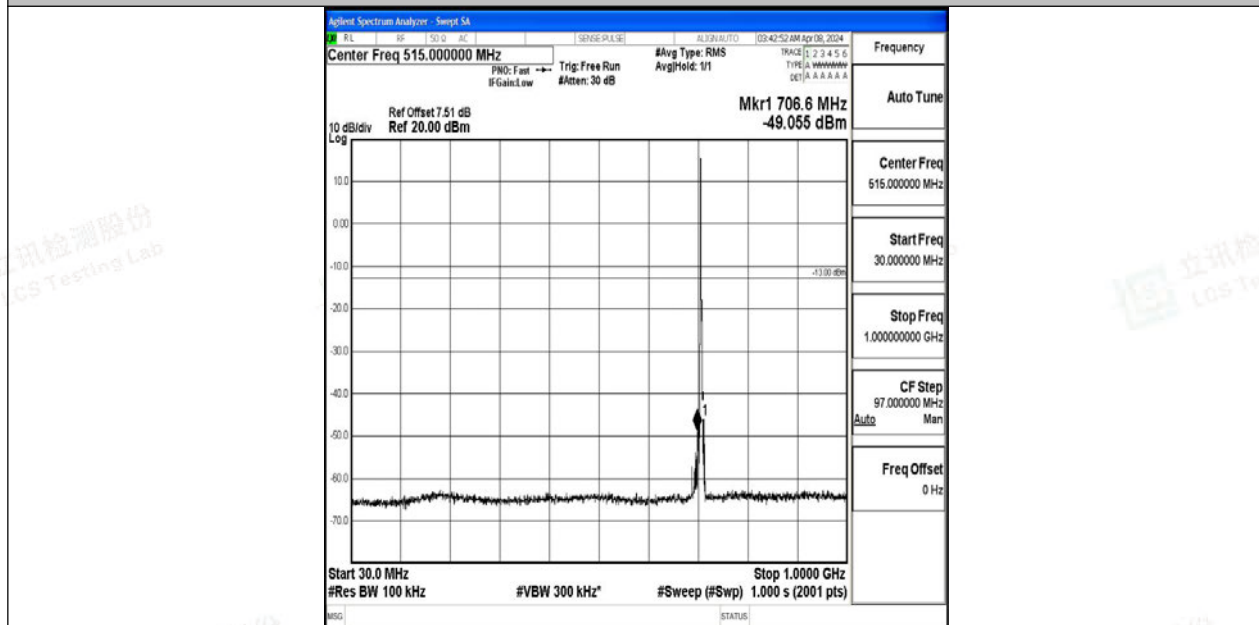
Band12_3MHz_64QAM_23165_1RB#0_30~1000_30~1000
