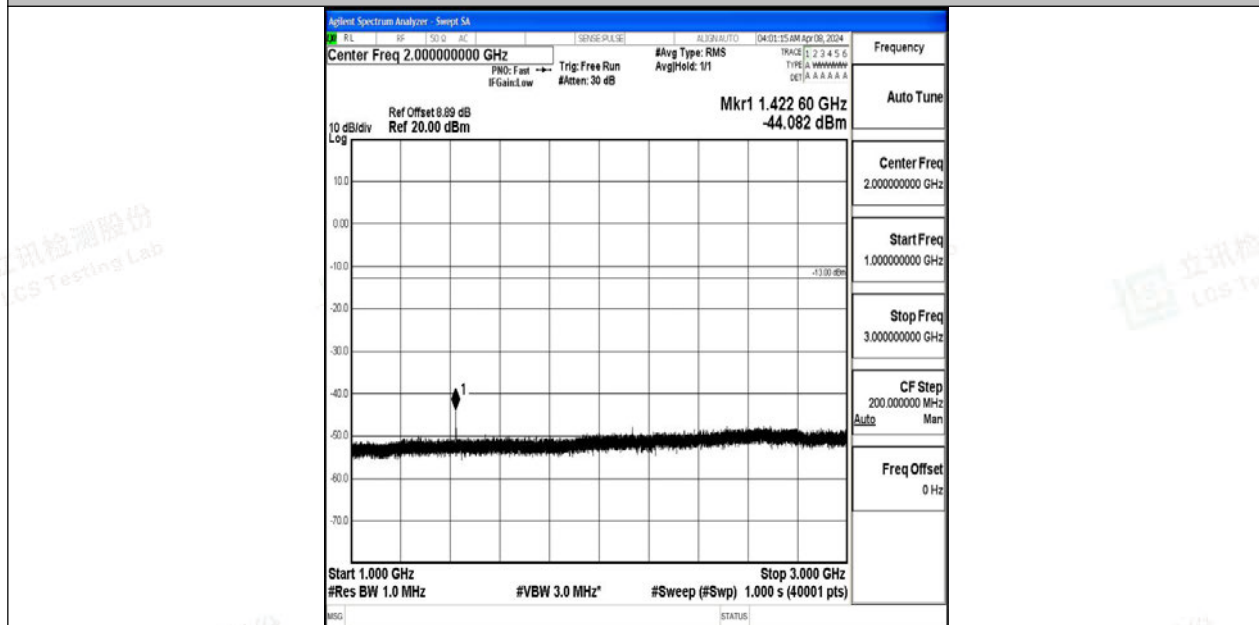
Band12_5MHz_QPSK_23155_1RB#0_1000~3000_1000~3000
