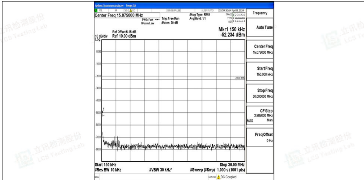
Band12_5MHz_64QAM_23035_1RB#0_0.15~30_0.15~30
