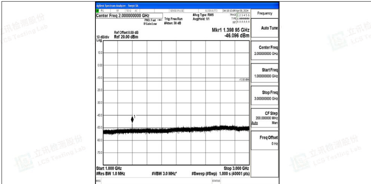
Band12_10MHz_64QAM_23060_1RB#0_1000~3000_1000~3000
