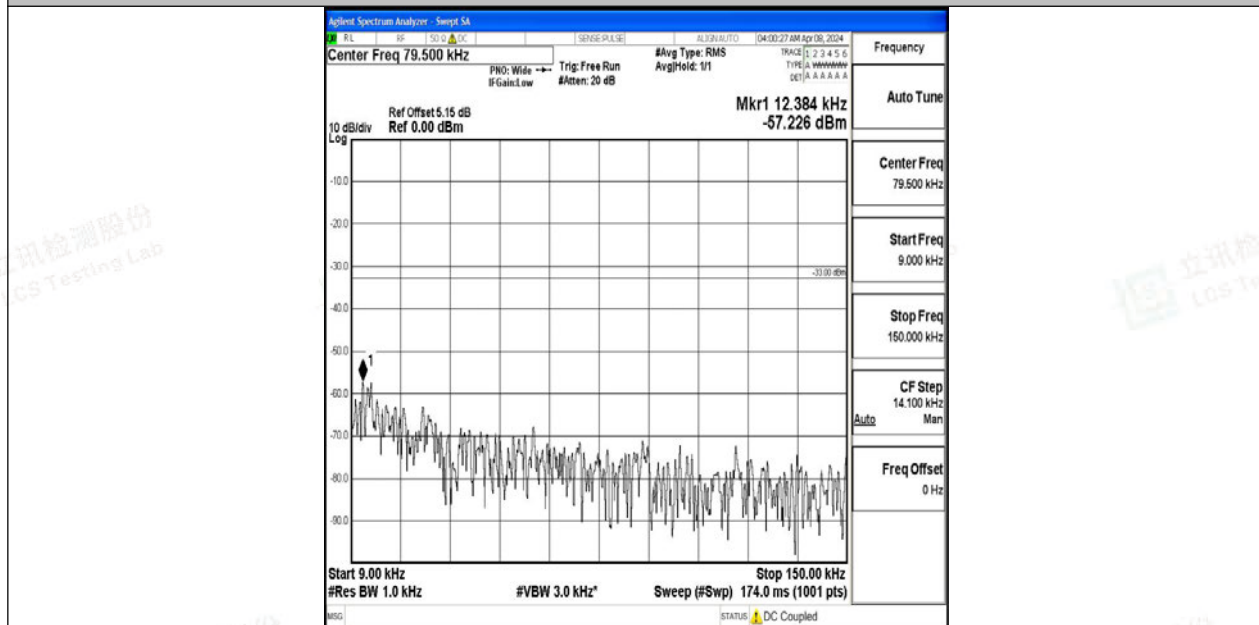
Band12_5MHz_64QAM_23095_1RB#0_0.009~0.15_0.009~0.15
