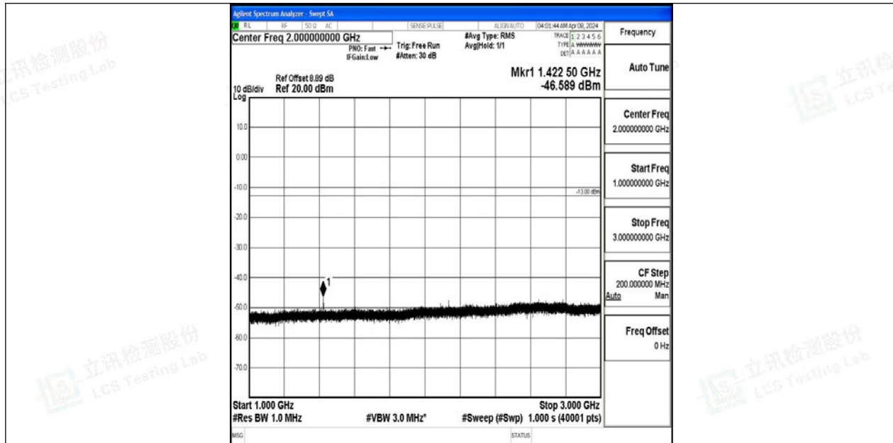
Band12_5MHz_64QAM_23155_1RB#0_1000~3000_1000~3000
