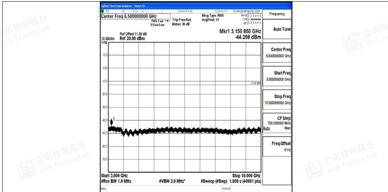
Band12_3MHz_QPSK_23025_1RB#0_3000~10000_3000~10000
