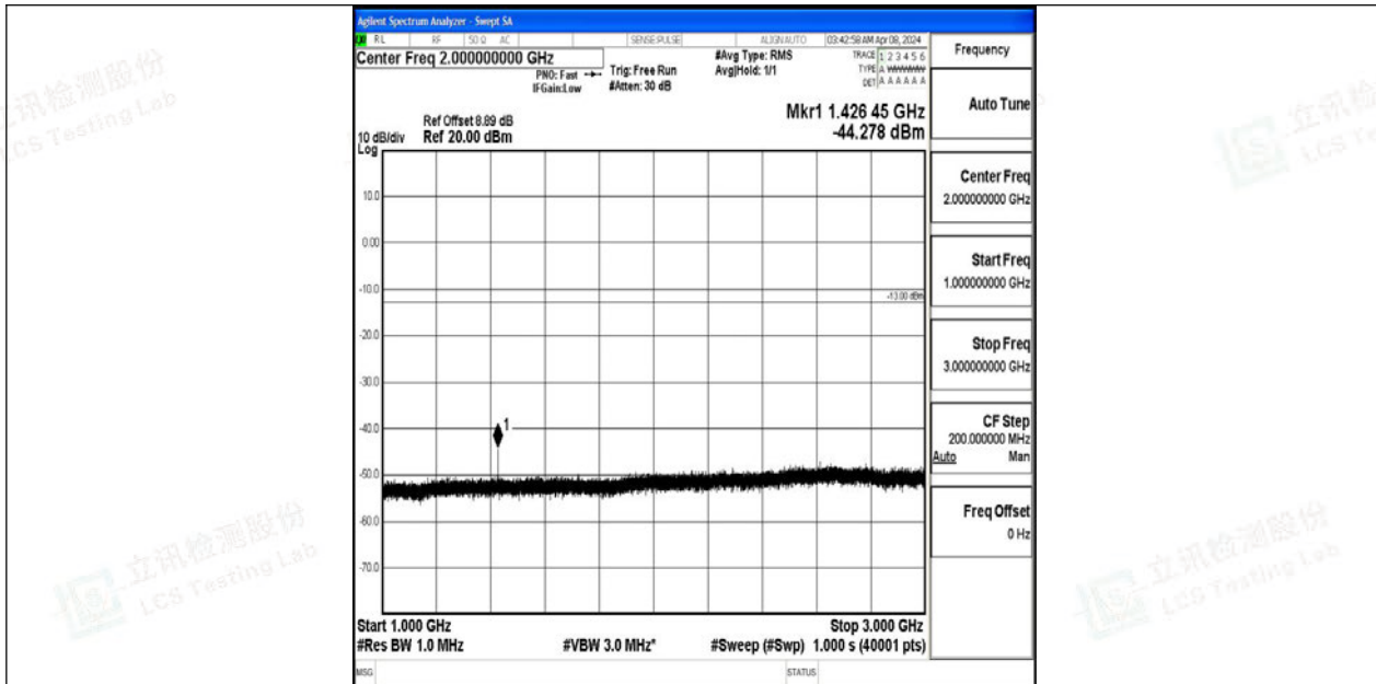
Band12_3MHz_64QAM_23165_1RB#0_1000~3000_1000~3000
