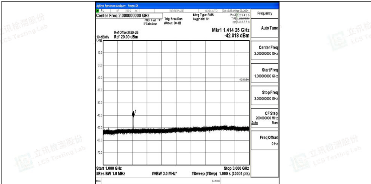
Band12_1.4MHz_64QAM_23095_1RB#0_1000~3000_1000~3000
