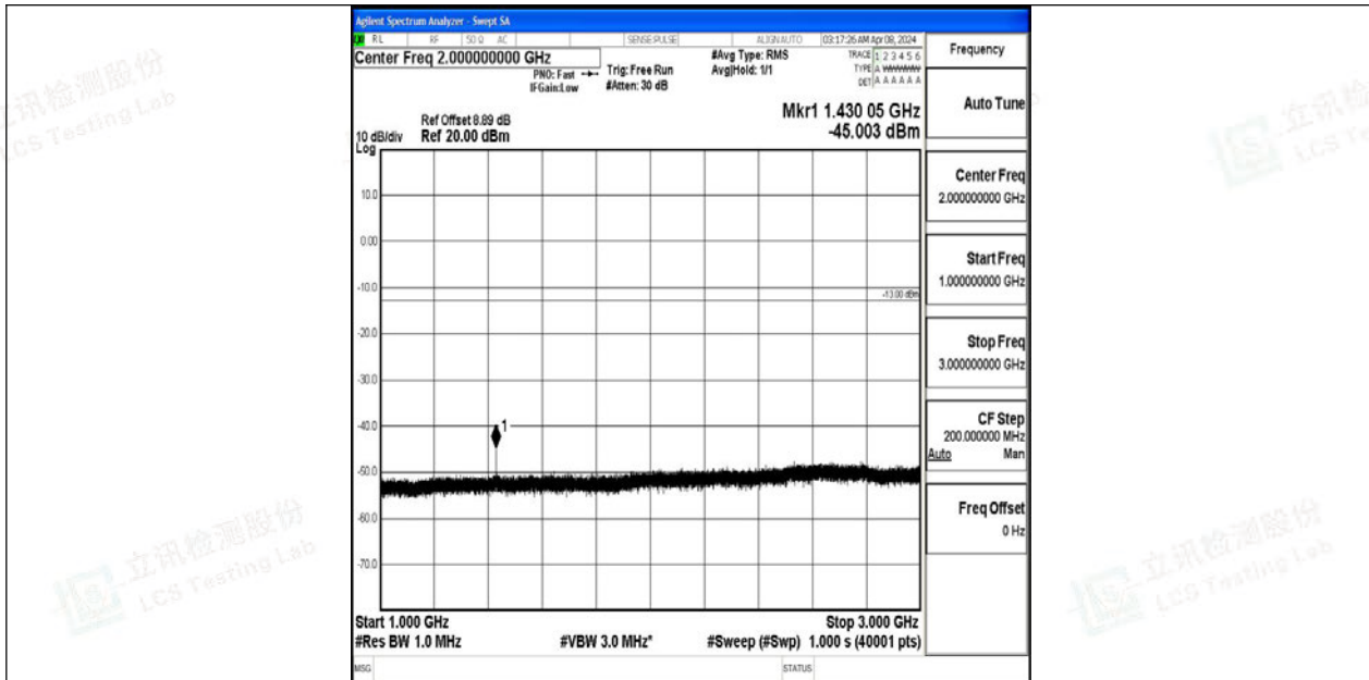
Band12_1.4MHz_64QAM_23173_1RB#0_1000~3000_1000~3000
