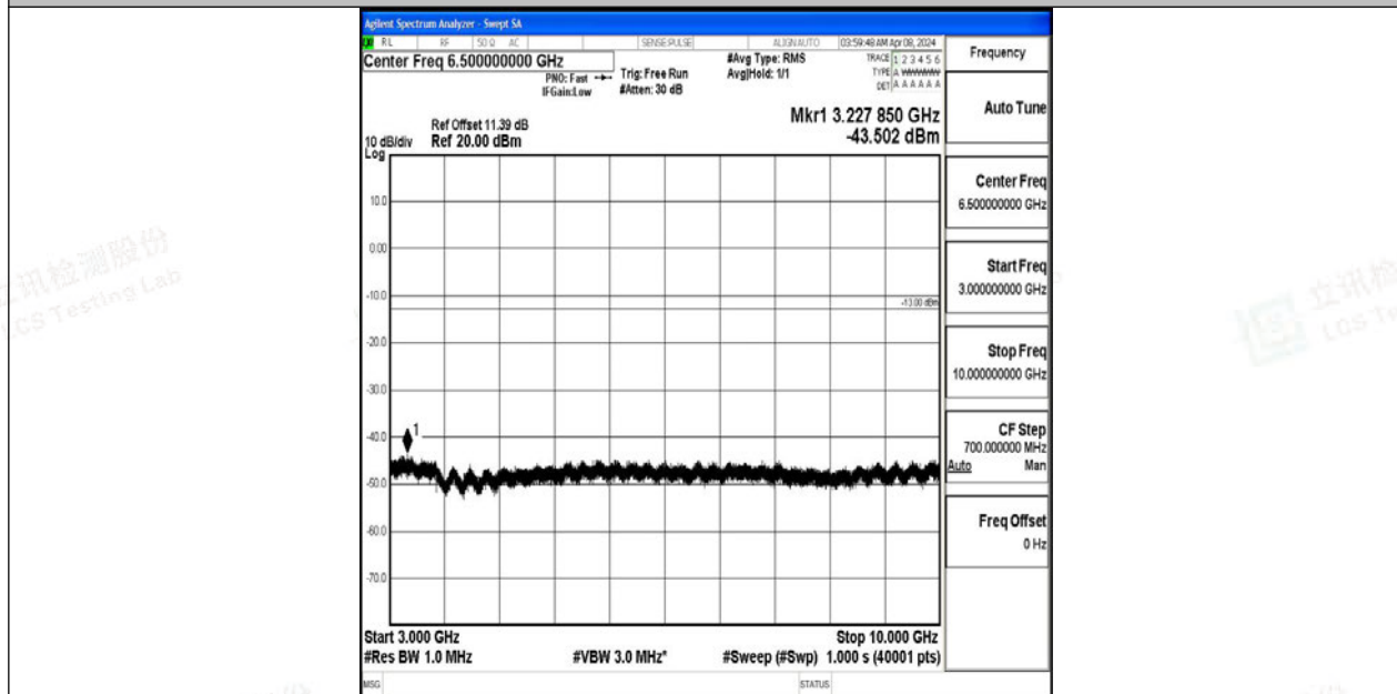
Band12_5MHz_64QAM_23035_1RB#0_3000~10000_3000~10000
