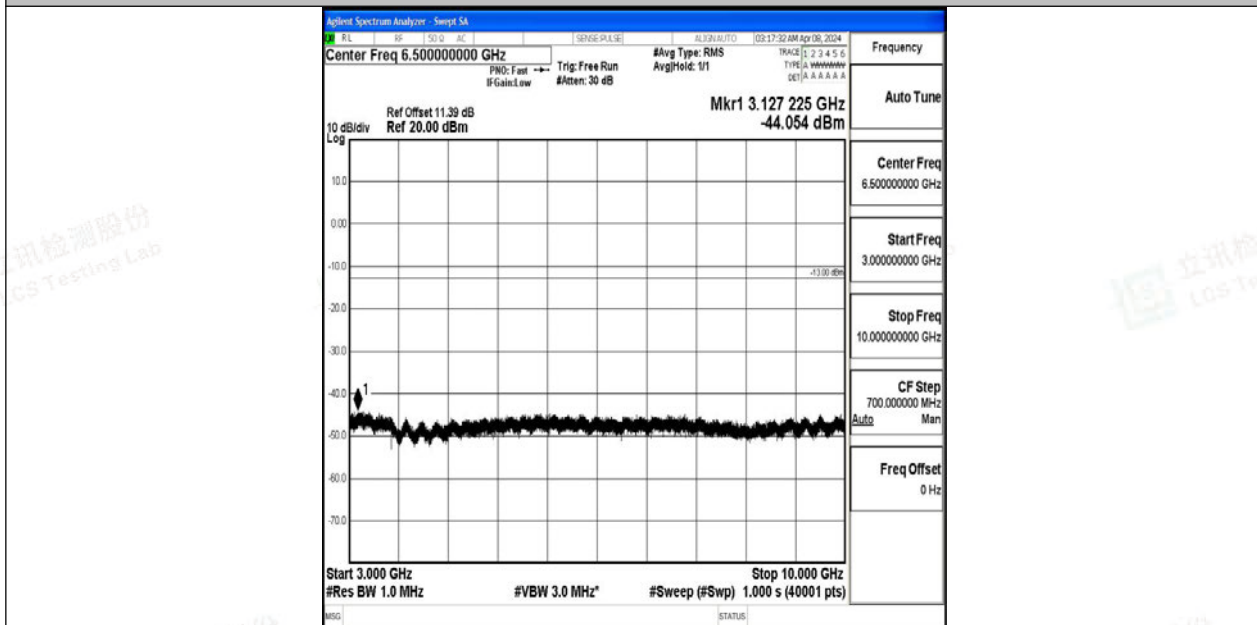
Band12_1.4MHz_64QAM_23173_1RB#0_3000~10000_3000~10000
