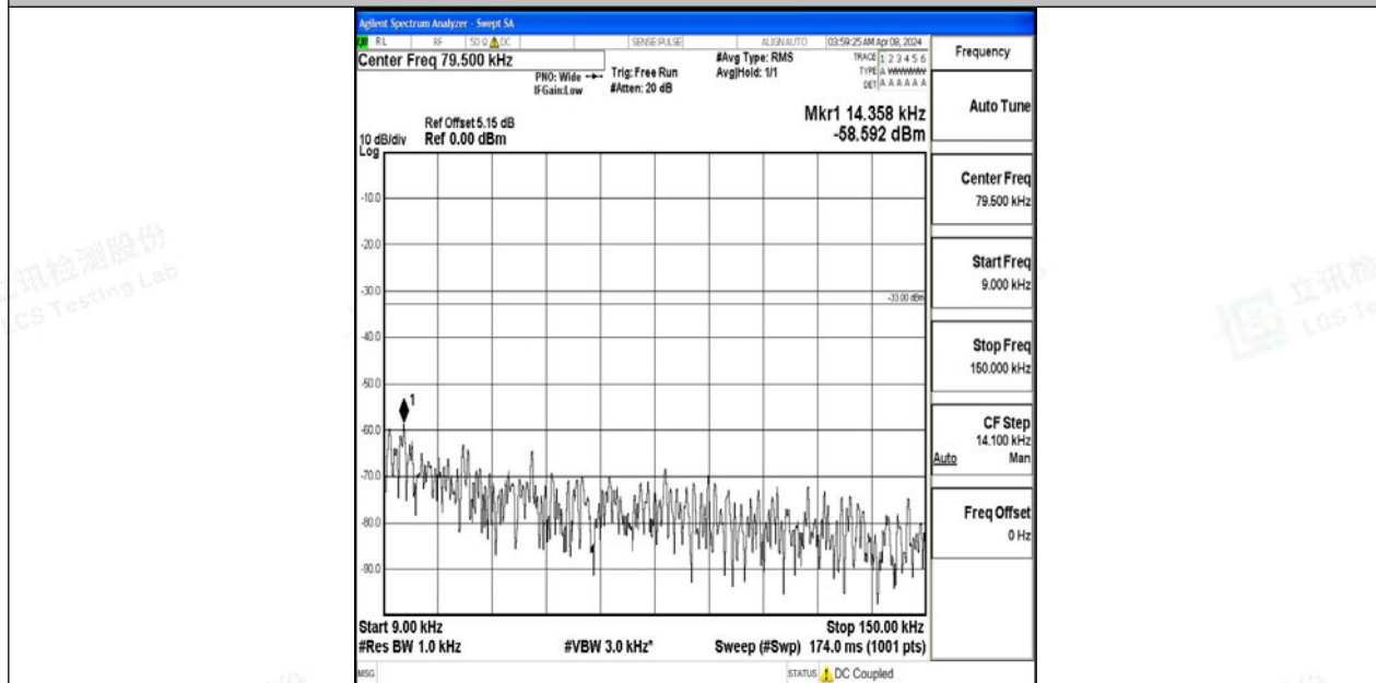
Band12_5MHz_64QAM_23035_1RB#0_0.009~0.15_0.009~0.15
