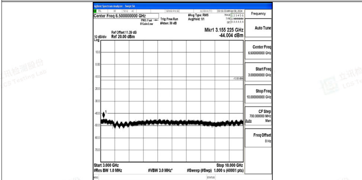
Band12_1.4MHz_64QAM_23095_1RB#0_3000~10000_3000~10000
