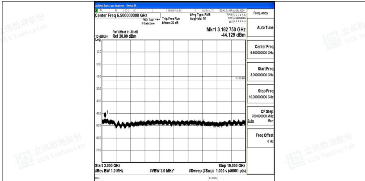
Band12_3MHz_QPSK_23095_1RB#0_3000~10000_3000~10000
