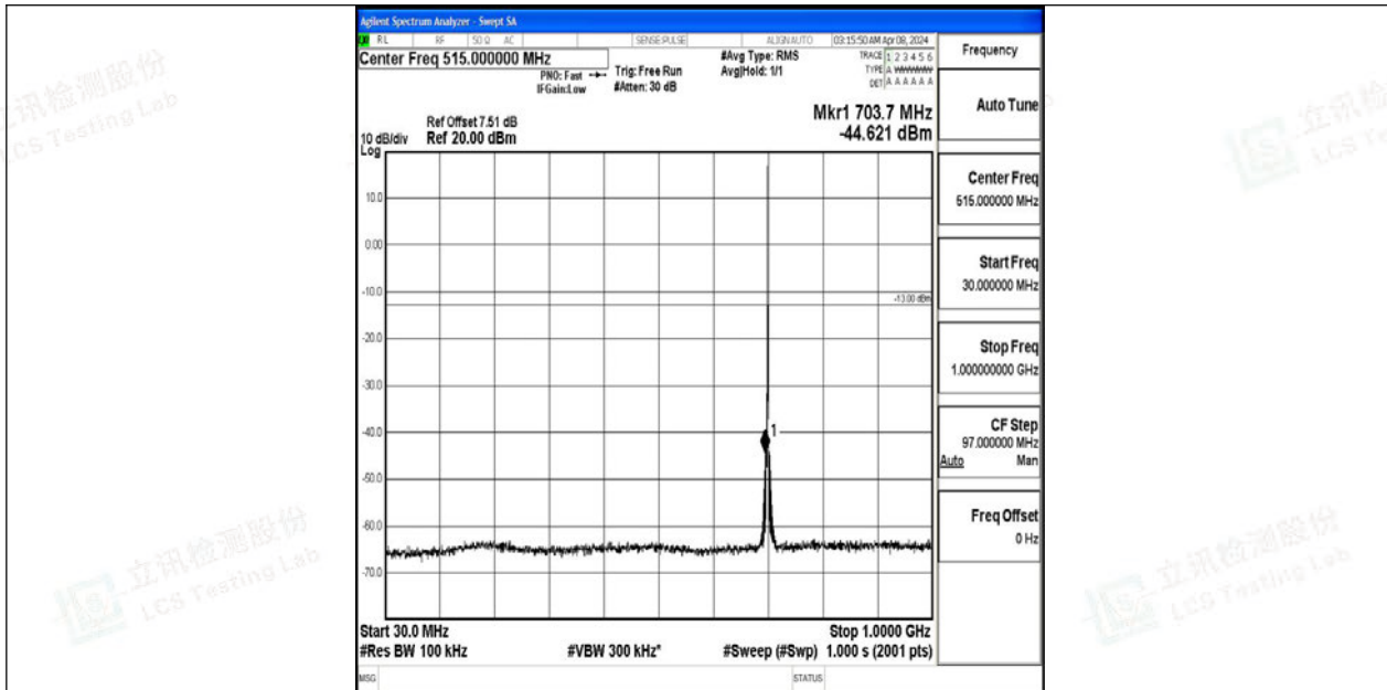
Band12_1.4MHz_QPSK_23095_1RB#0_30~1000_30~1000
