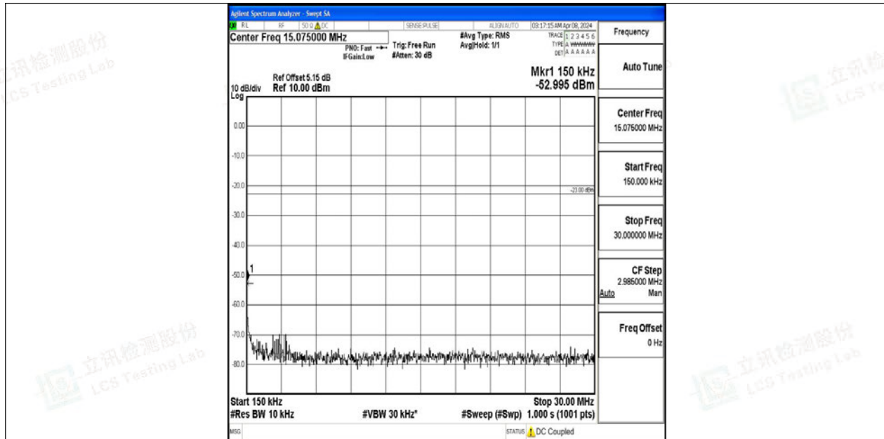
Band12_1.4MHz_64QAM_23173_1RB#0_0.15~30_0.15~30
