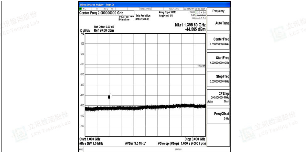
Band12_3MHz_64QAM_23025_1RB#0_1000~3000_1000~3000
