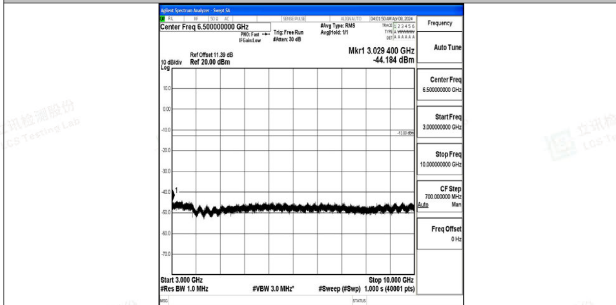
Band12_5MHz_64QAM_23155_1RB#0_3000~10000_3000~10000
