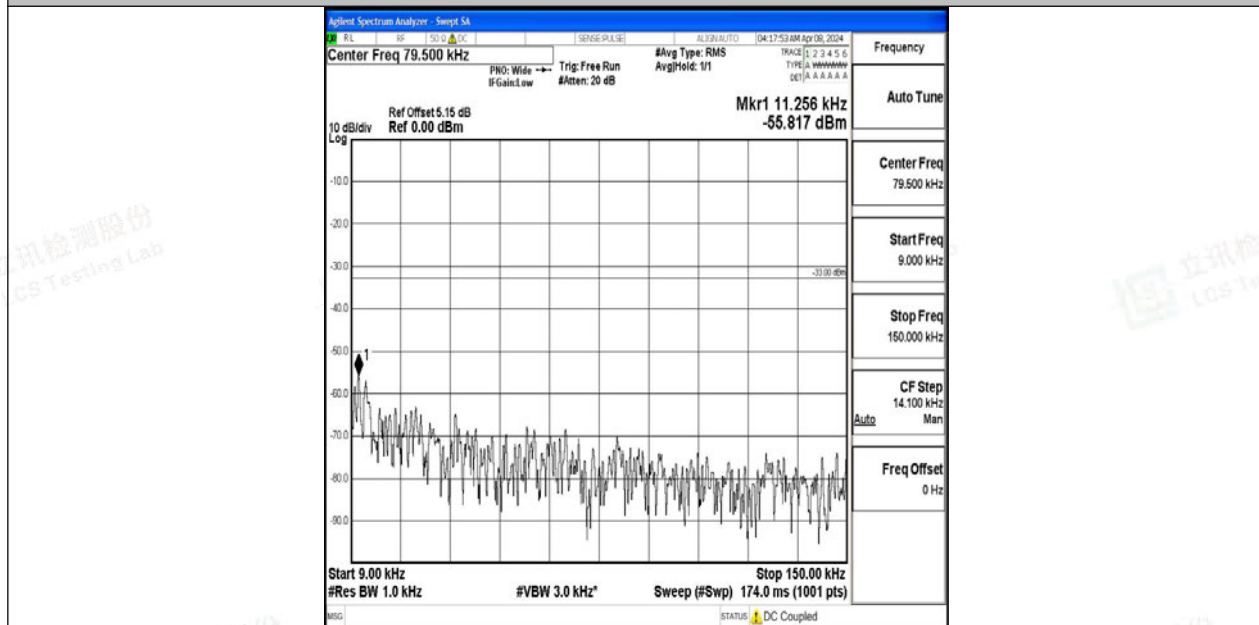
Band12_10MHz_64QAM_23060_1RB#0_0.009~0.15_0.009~0.15
