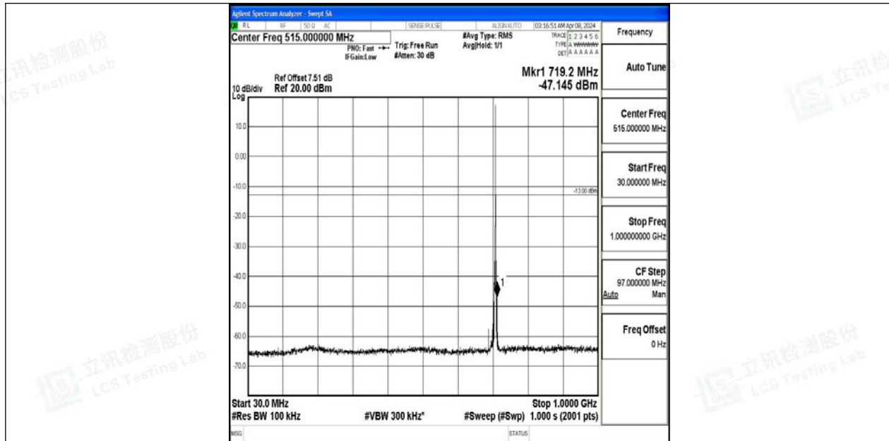
Band12_1.4MHz_QPSK_23173_1RB#0_30~1000_30~1000
