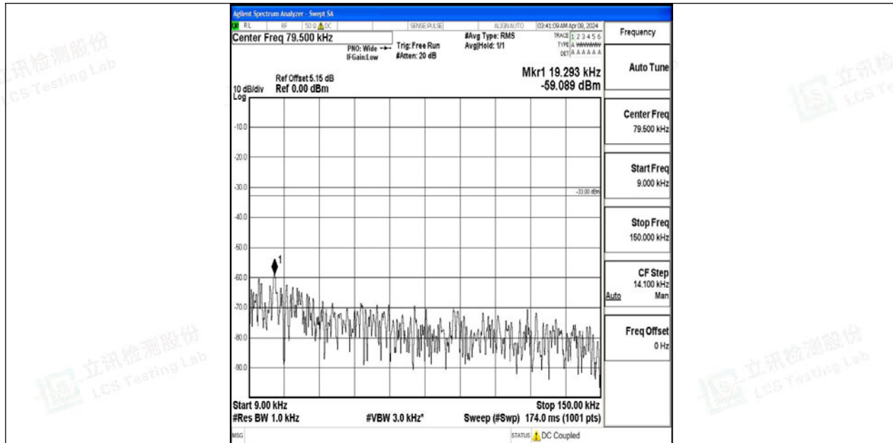
Band12_3MHz_QPSK_23095_1RB#0_0.009~0.15_0.009~0.15
