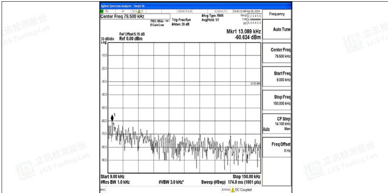
Band12_3MHz_QPSK_23165_1RB#0_0.009~0.15_0.009~0.15
