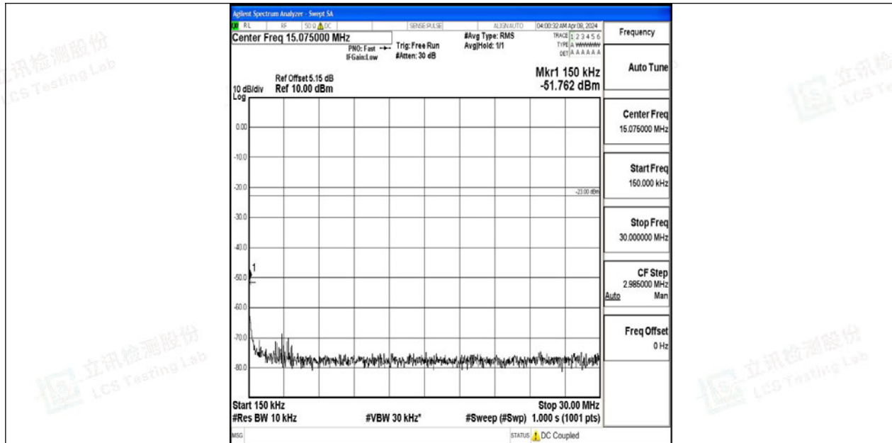
Band12_5MHz_64QAM_23095_1RB#0_0.15~30_0.15~30
