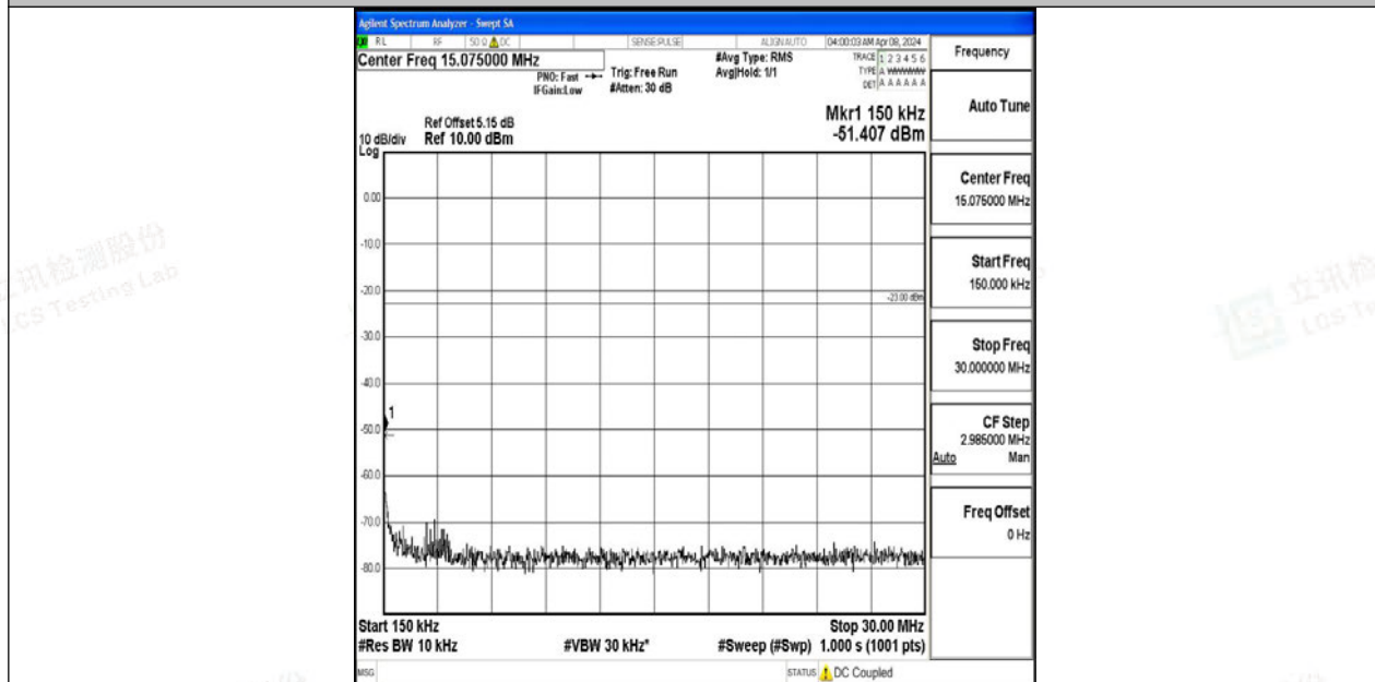
Band12_5MHz_QPSK_23095_1RB#0_0.15~30_0.15~30
