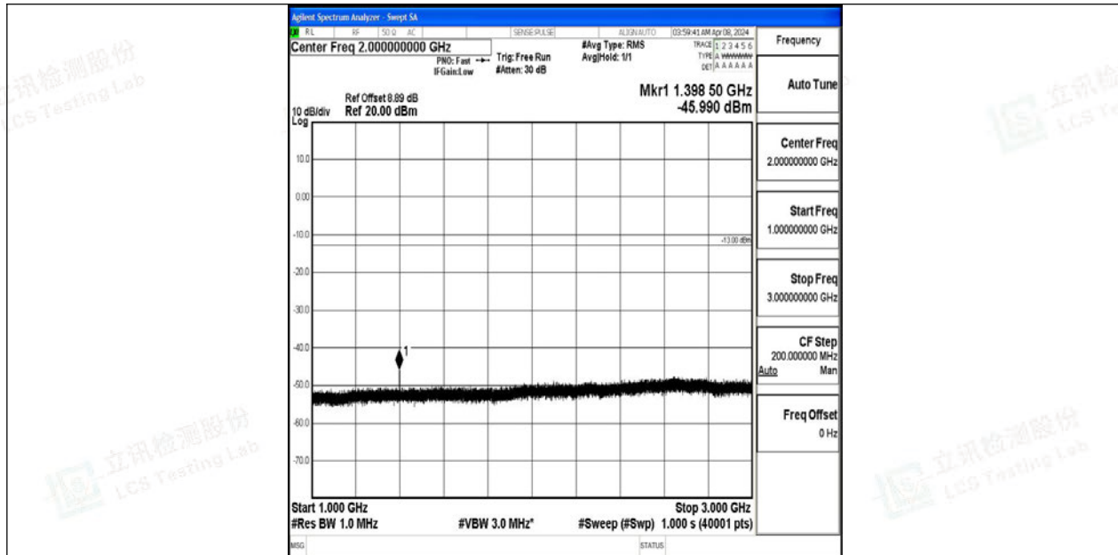
Band12_5MHz_64QAM_23035_1RB#0_1000~3000_1000~3000
