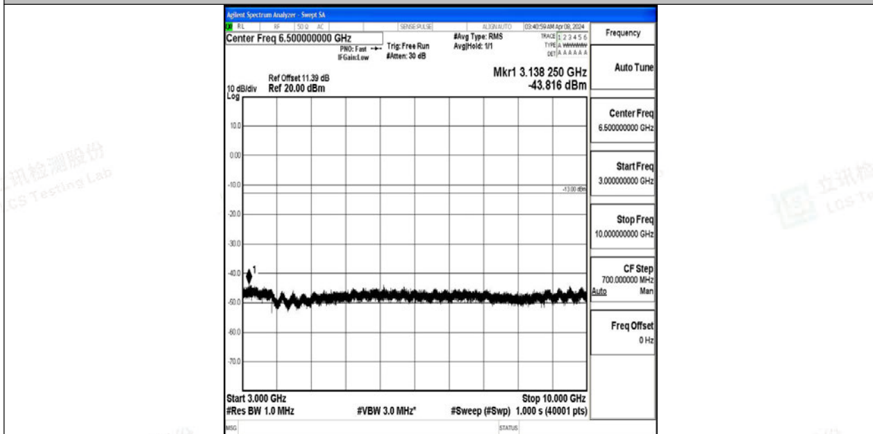
Band12_3MHz_64QAM_23025_1RB#0_3000~10000_3000~10000
