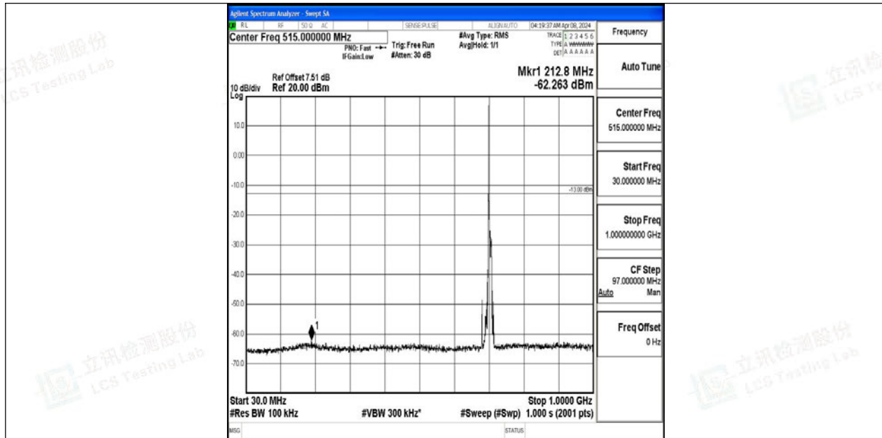
Band12_10MHz_QPSK_23130_1RB#0_30~1000_30~1000
