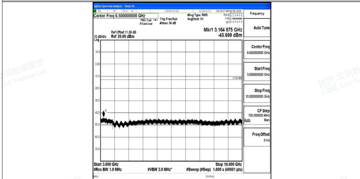
Band12_10MHz_64QAM_23095_1RB#0_3000~10000_3000~10000
