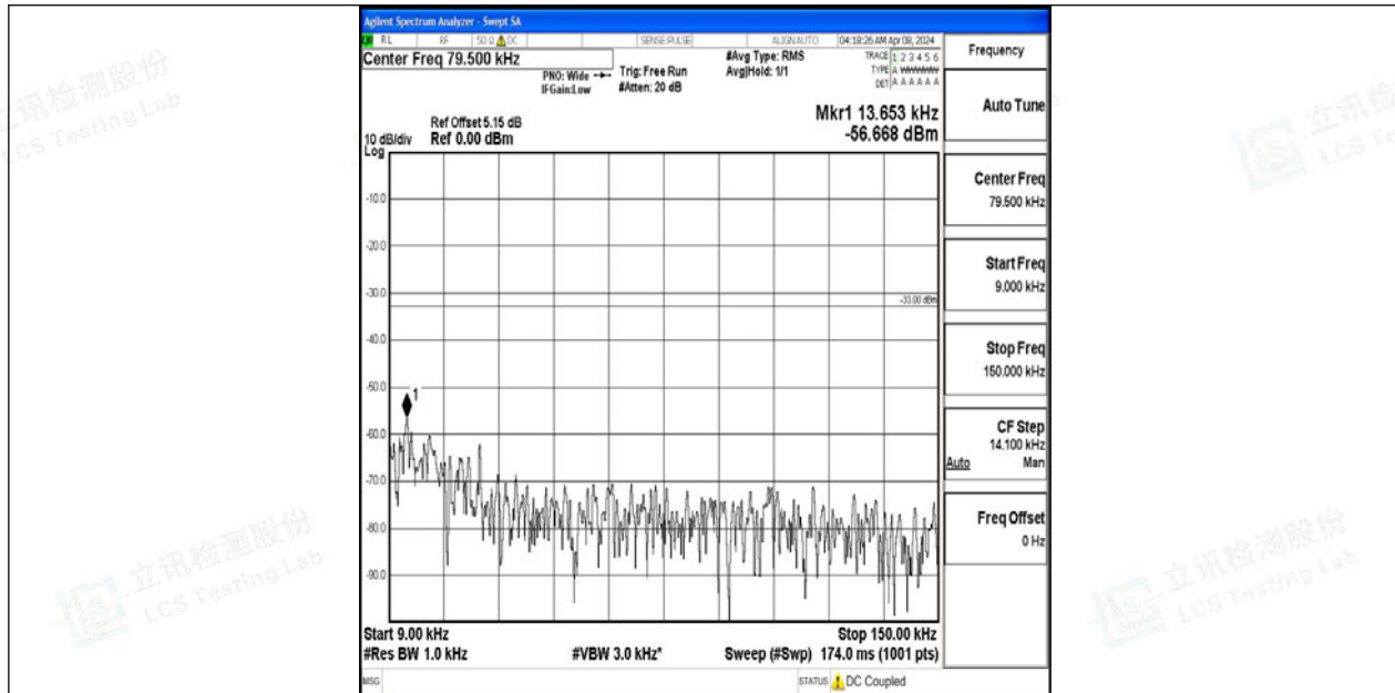
Band12_10MHz_QPSK_23095_1RB#0_0.009~0.15_0.009~0.15
