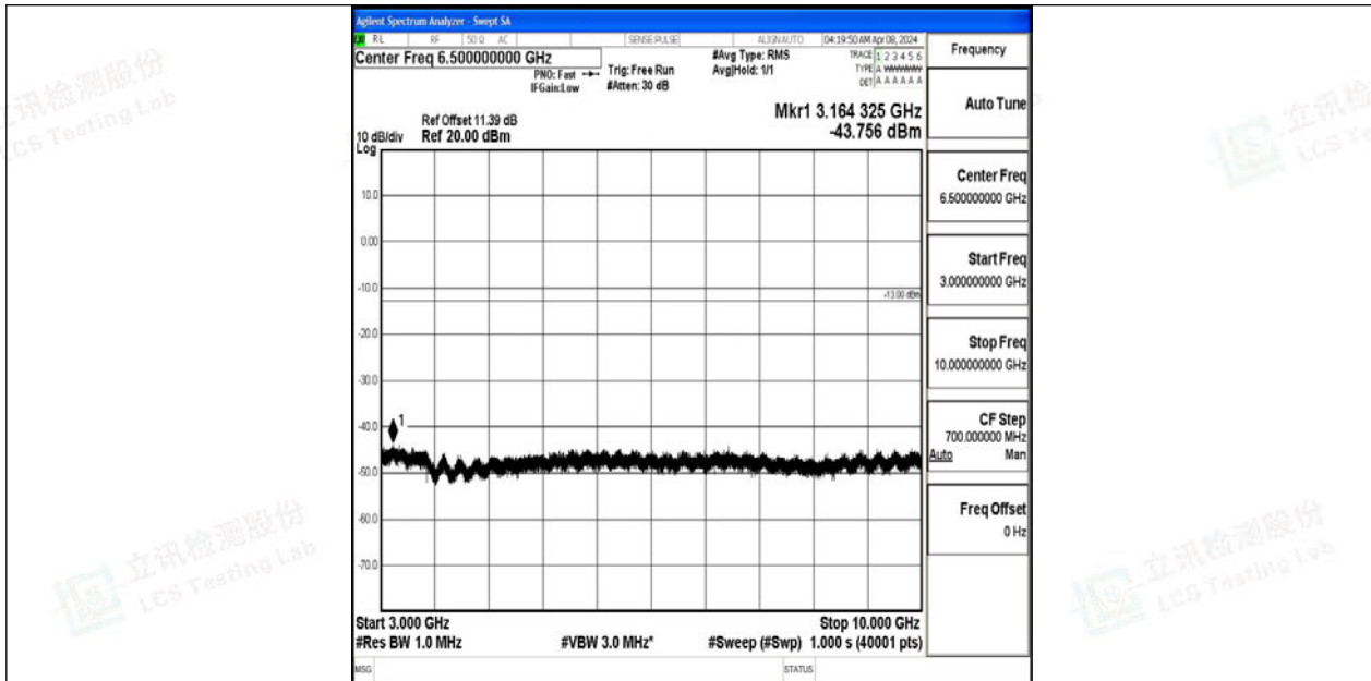
Band12_10MHz_QPSK_23130_1RB#0_3000~10000_3000~10000
