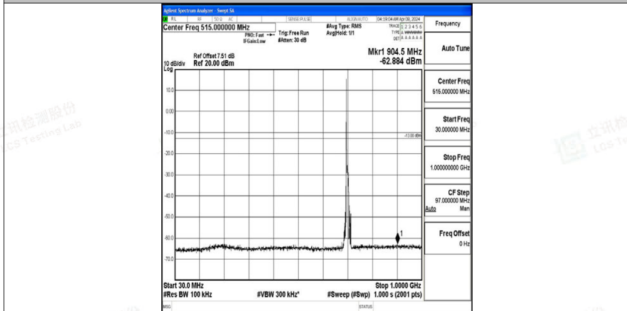
Band12_10MHz_64QAM_23095_1RB#0_30~1000_30~1000
