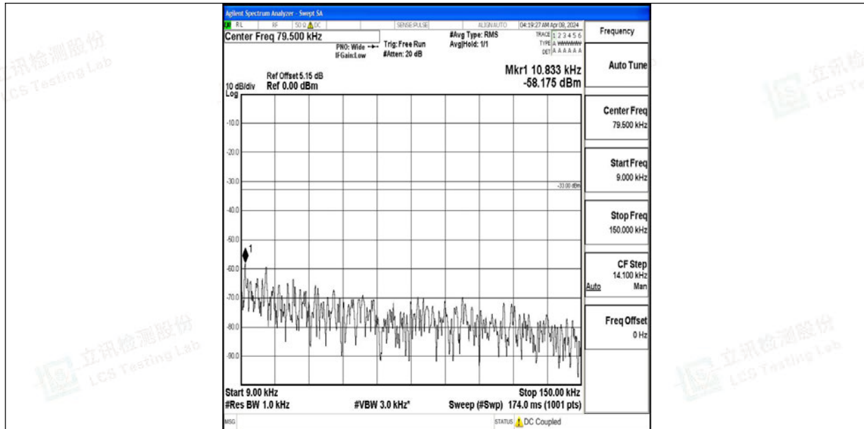
Band12_10MHz_QPSK_23130_1RB#0_0.009~0.15_0.009~0.15
