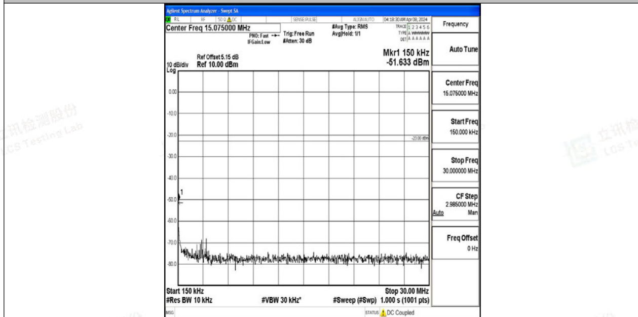
Band12_10MHz_QPSK_23095_1RB#0_0.15~30_0.15~30
