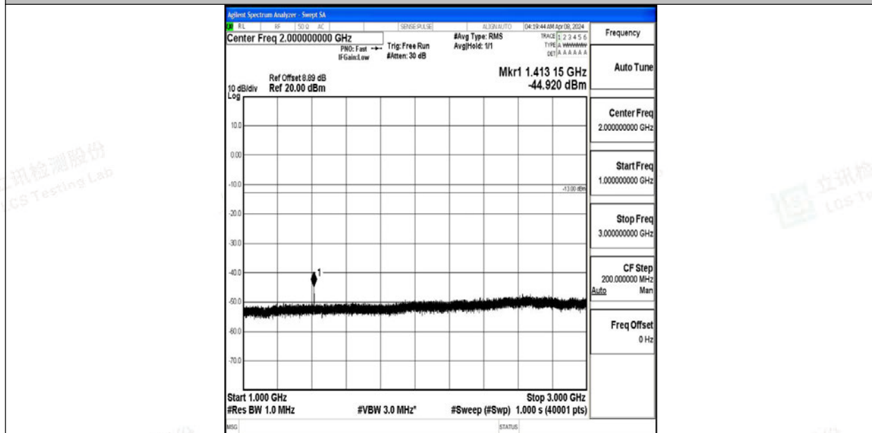
Band12_10MHz_QPSK_23130_1RB#0_1000~3000_1000~3000
