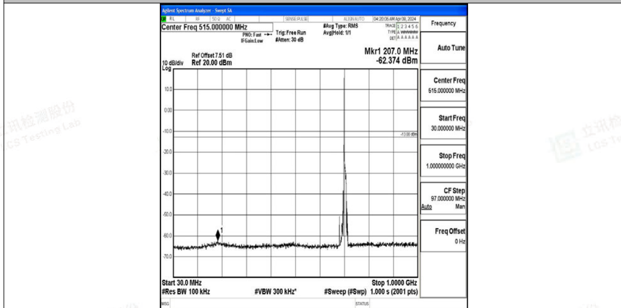
Band12_10MHz_64QAM_23130_1RB#0_30~1000_30~1000
