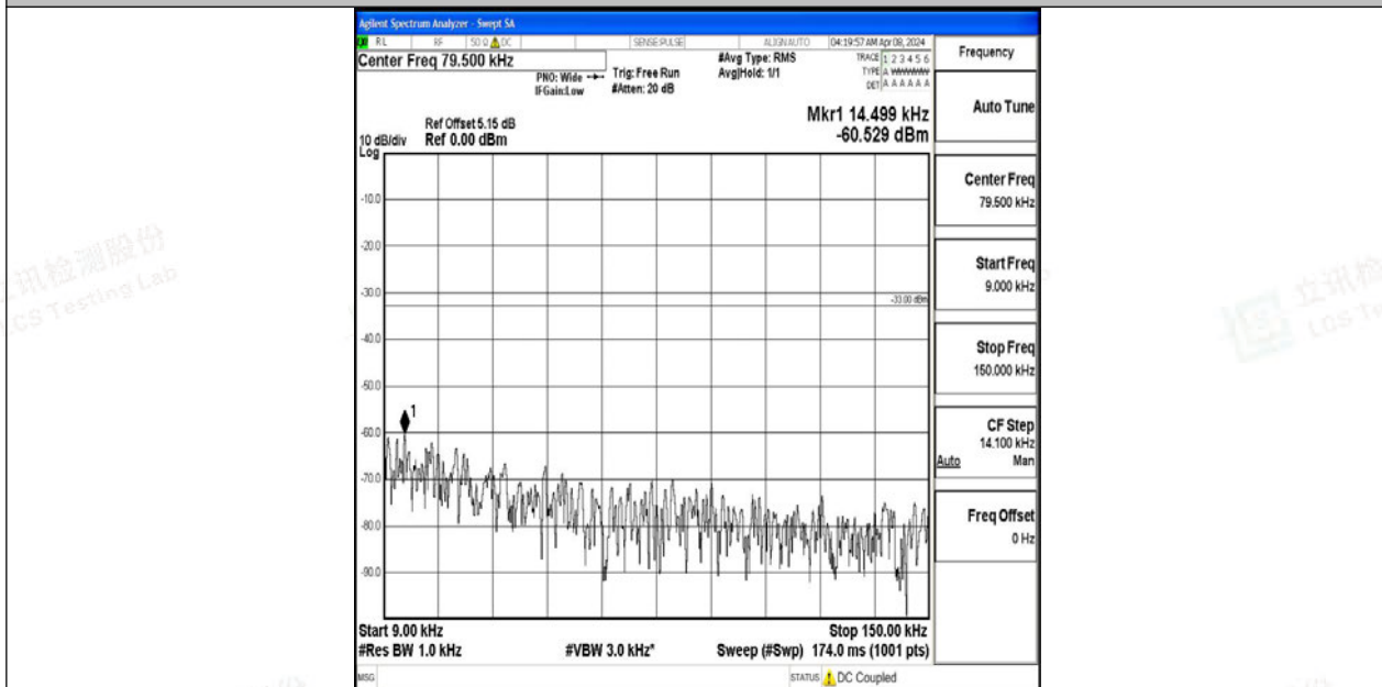
Band12_10MHz_64QAM_23130_1RB#0_0.009~0.15_0.009~0.15
