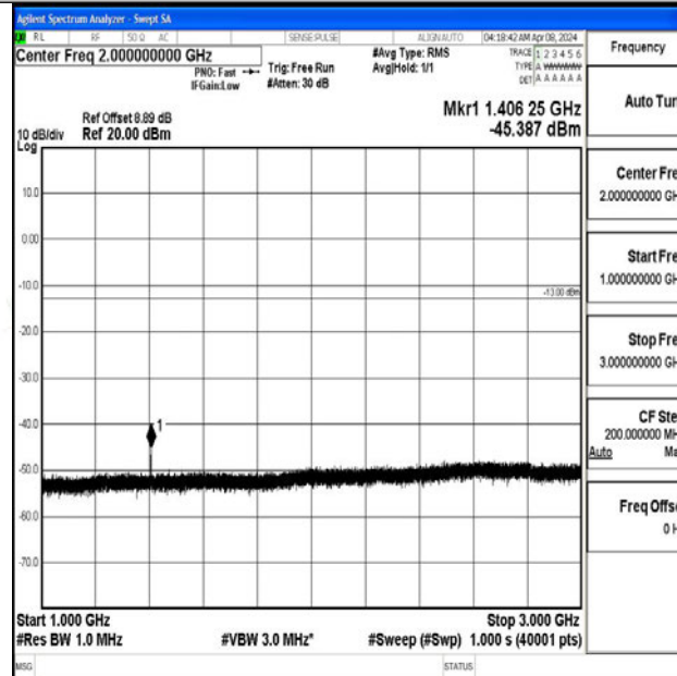
Band12_10MHz_QPSK_23095_1RB#0_1000~3000_1000~3000
