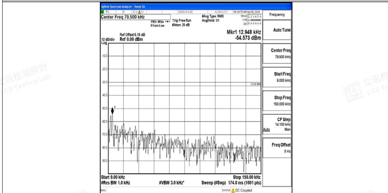
Band12_10MHz_64QAM_23095_1RB#0_0.009~0.15_0.009~0.15
