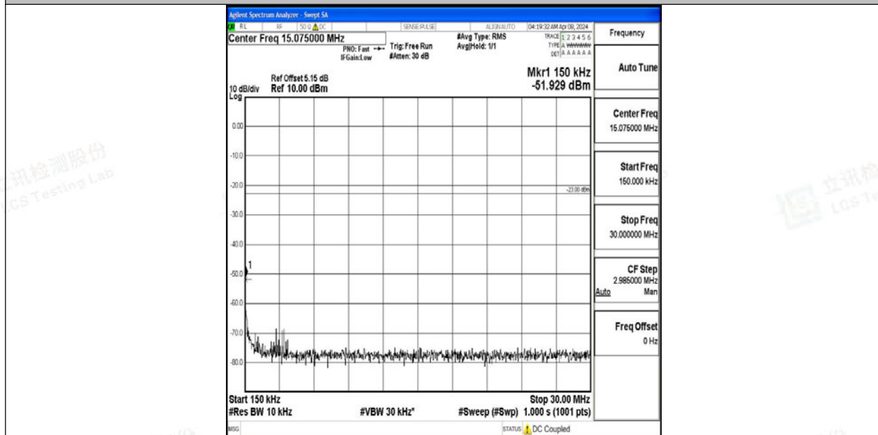
Band12_10MHz_QPSK_23130_1RB#0_0.15~30_0.15~30
