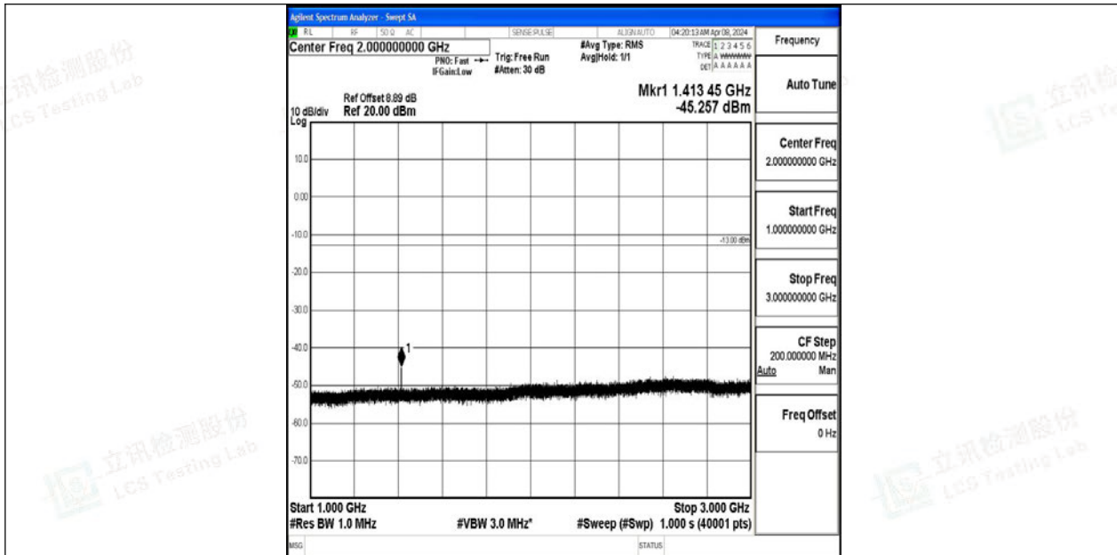
Band12_10MHz_64QAM_23130_1RB#0_1000~3000_1000~3000
