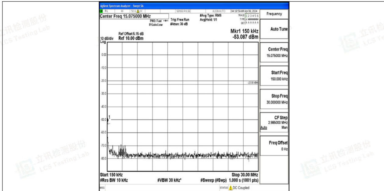
Band12_10MHz_64QAM_23095_1RB#0_0.15~30_0.15~30
