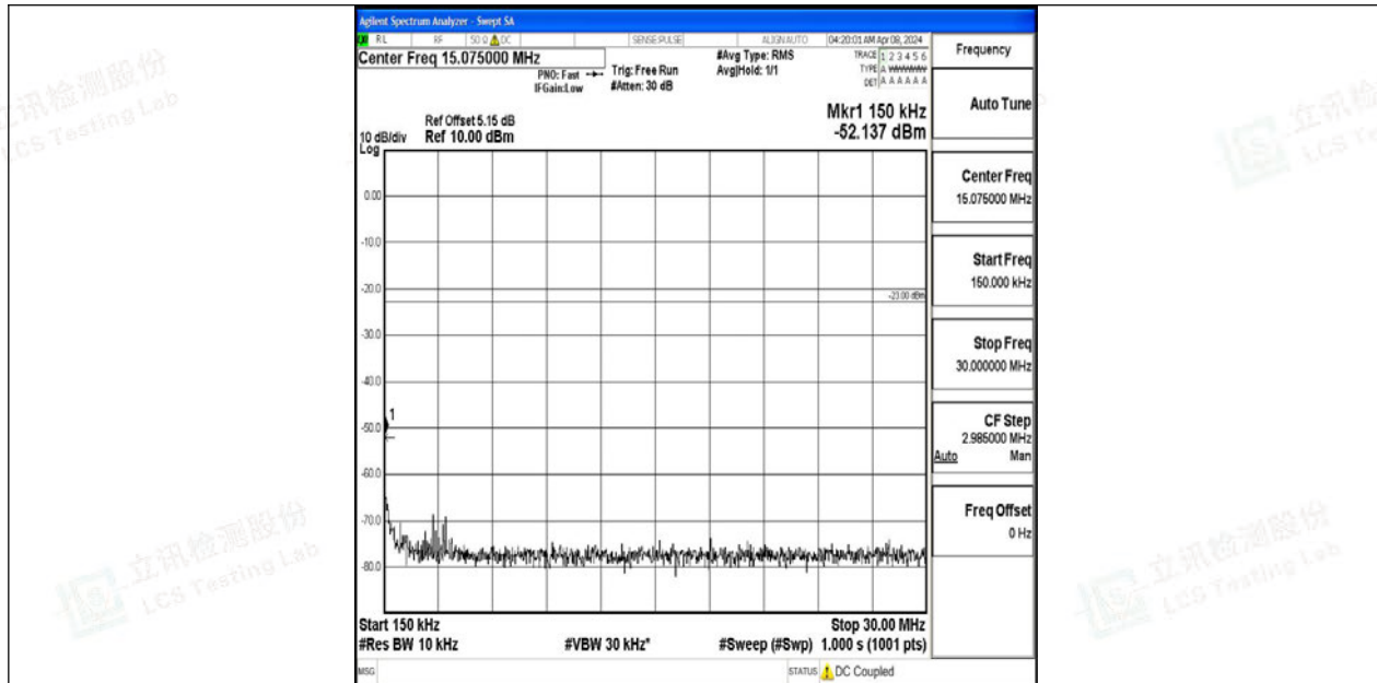
Band12_10MHz_64QAM_23130_1RB#0_0.15~30_0.15~30
