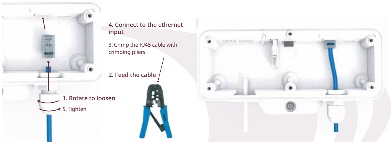
Figure 9 - Network cable installation procedure
