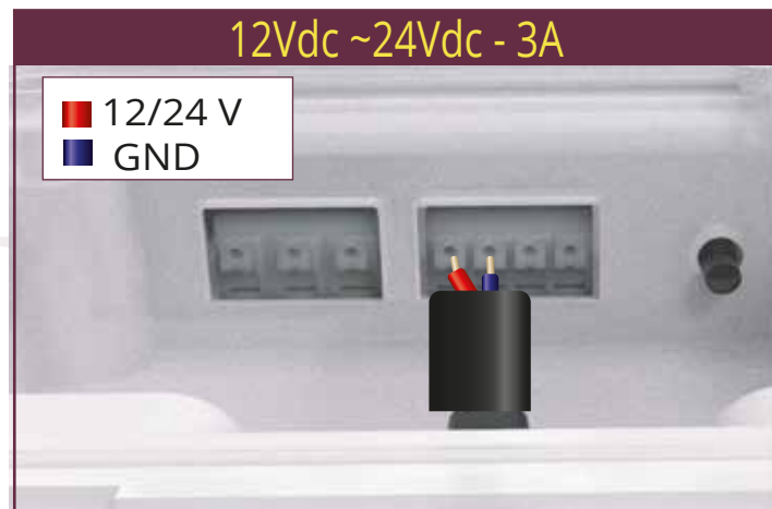
Figure 1 - Connection terminals
