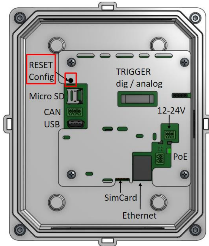
Figure: Reset/Config Button
