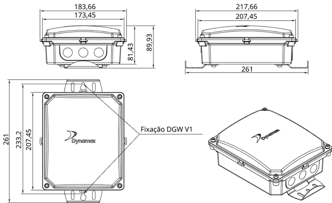
Figure: DynaGateway dimensions and mounting holes
