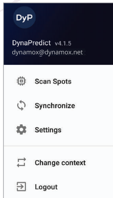
Figure 4 - Side Menu
