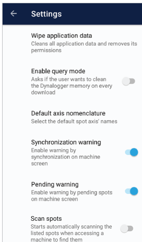
Figure 13 - Settings
