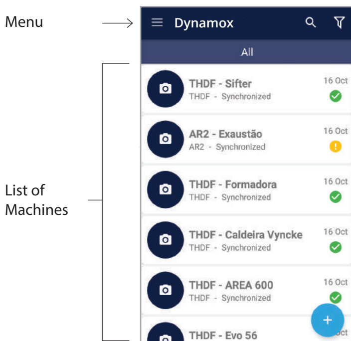
Figure 3 - Initial Screen
