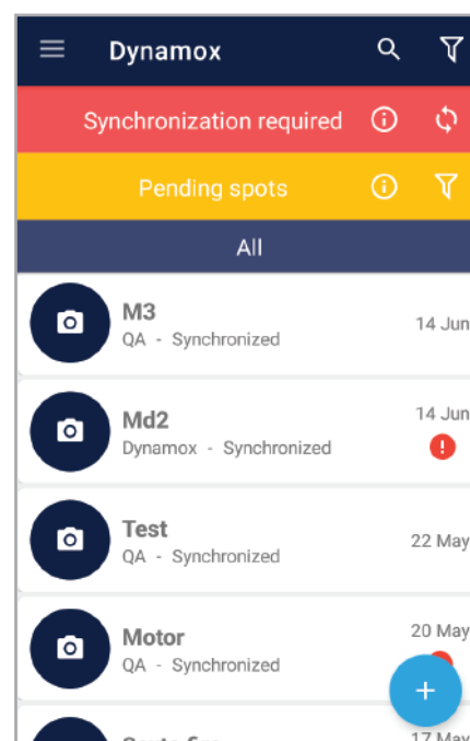
Figure 14 - Warnings
