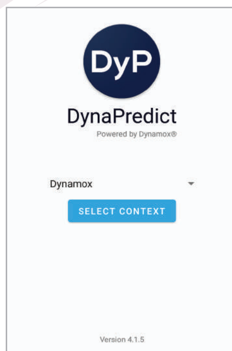
Figure 2 - Workspace selection
