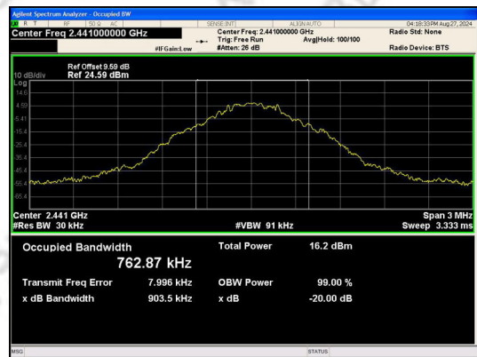
GFSK_DH5_Channel 39
