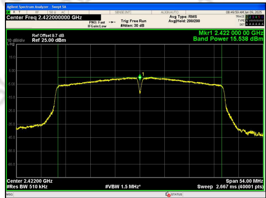
Conducted AVG output power IEEE 802.11n_40_Channel 3_Antenna 0
