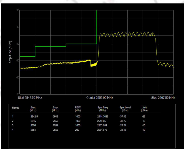
Band41(2555-2655) QPSK BW=10MHz Channel=40290 RB Size=50 Position=#0
