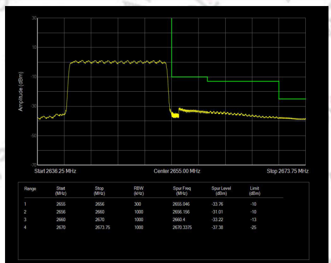
Band41(2555-2655) QAM16 BW=15MHz Channel=41165 RB Size=75 Position=#0
