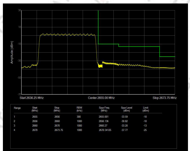
Band41(2555-2655) QPSK BW=15MHz Channel=41165 RB Size=75 Position=#0
