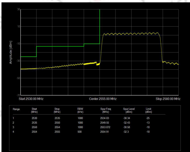
Band41(2555-2655) QAM16 BW=20MHz Channel=40340 RB Size=100 Position=#0
