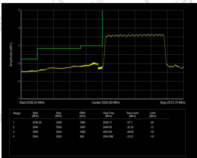
Band41(2555-2655) QPSK BW=15MHz Channel=40315 RB Size=75 Position=#0
