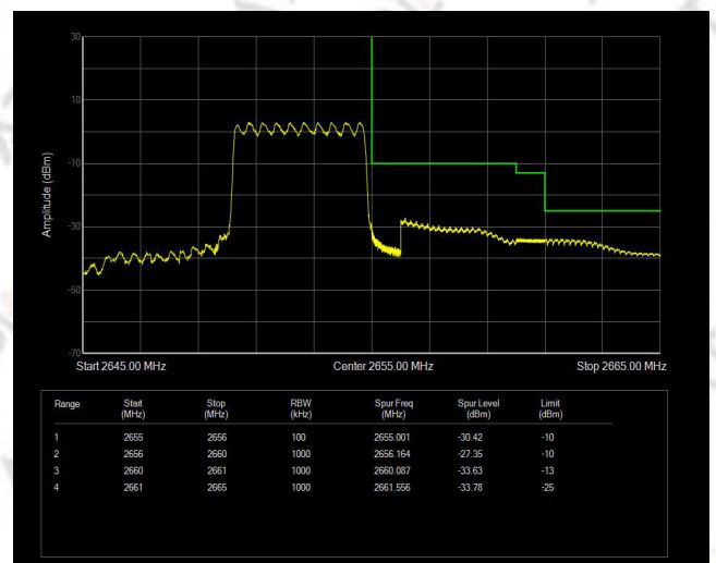
Band41(2555-2655) QPSK BW=5MHz Channel=41215 RB Size=25 Position=#0
