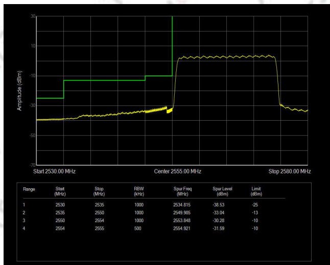
Band41(2555-2655) QPSK BW=20MHz Channel=40340 RB Size=100 Position=#0
