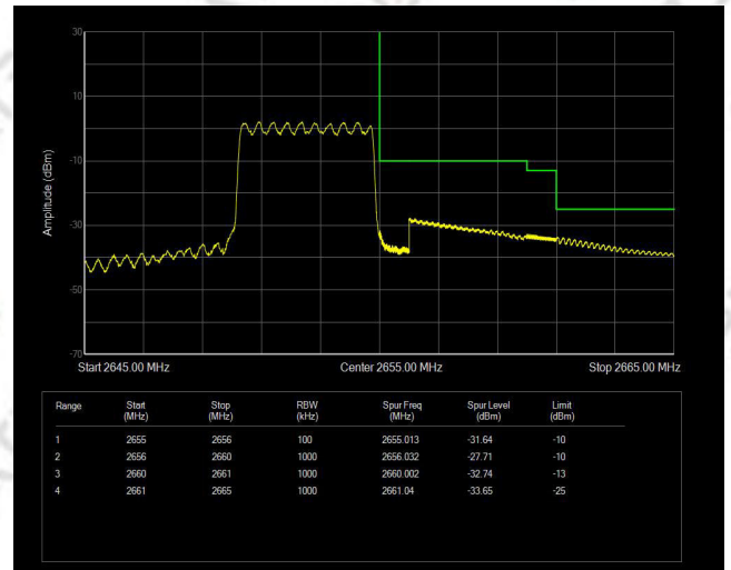
Band41(2555-2655) QAM16 BW=5MHz Channel=41215 RB Size=25 Position=#0
