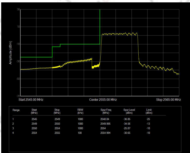
Band41(2555-2655) QPSK BW=5MHz Channel=40265 RB Size=25 Position=#0
