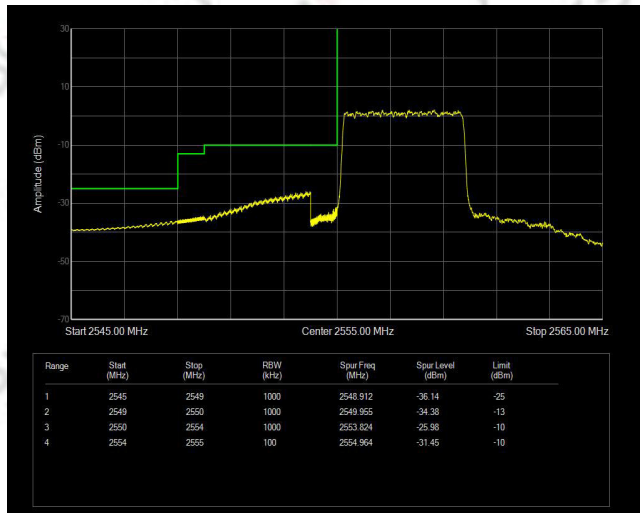
Band41(2555-2655) QAM16 BW=5MHz Channel=40265 RB Size=25 Position=#0
