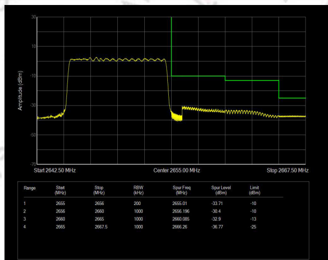
Band41(2555-2655) QPSK BW=10MHz Channel=41190 RB Size=50 Position=#0
