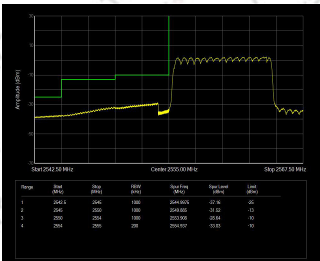
Band41(2555-2655) QAM16 BW=10MHz Channel=40290 RB Size=50 Position=#0
