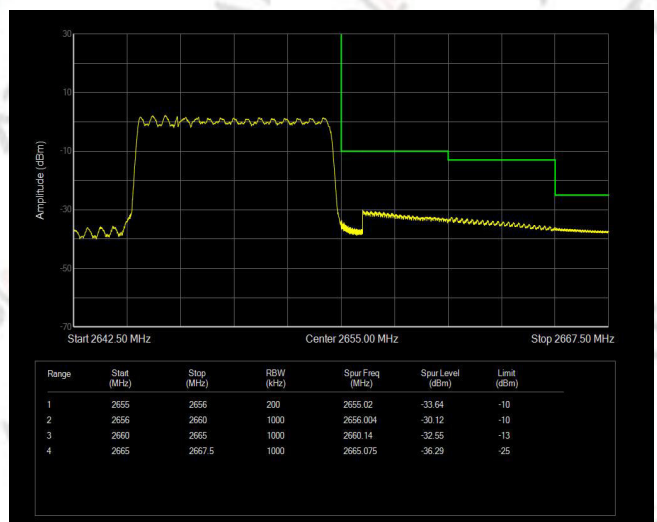
Band41(2555-2655) QAM16 BW=10MHz Channel=41190 RB Size=50 Position=#0
