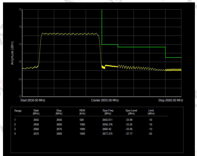
Band41(2555-2655) QPSK BW=20MHz Channel=41140 RB Size=100 Position=#0
