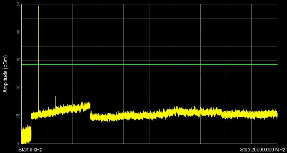
Band66 QAM16 BW=1.4MHz Channel=132322 RB Size=1 Position=#0
