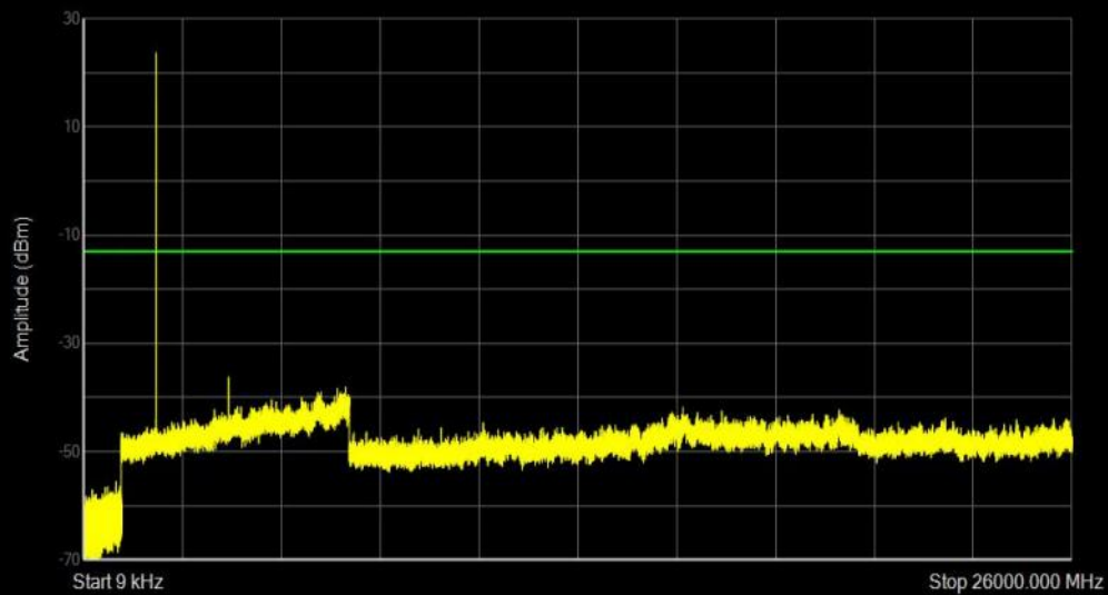
Band25 QPSK BW=1.4MHz Channel=26683 RB Size=1 Position=#0
