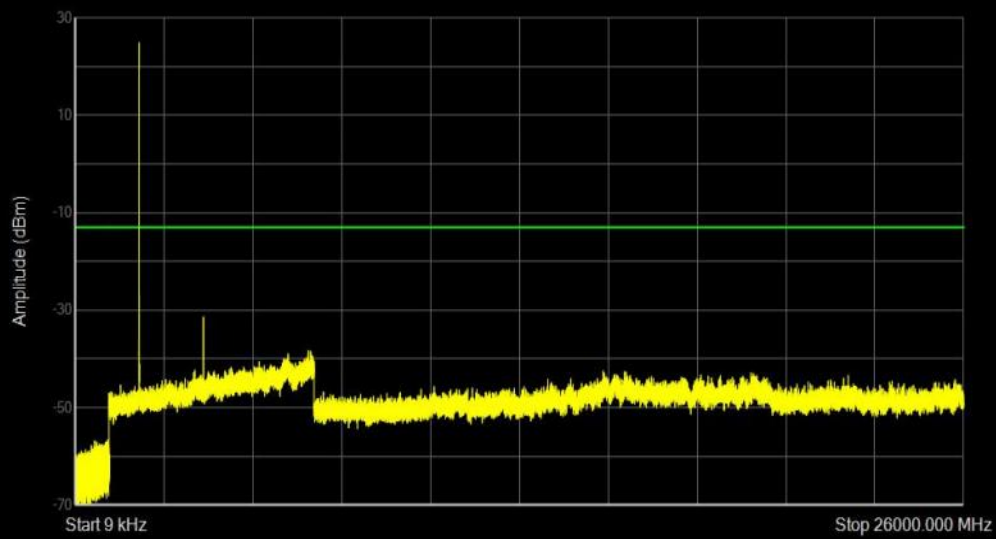
Band25 QPSK BW=1.4MHz Channel=26365 RB Size=1 Position=#0
