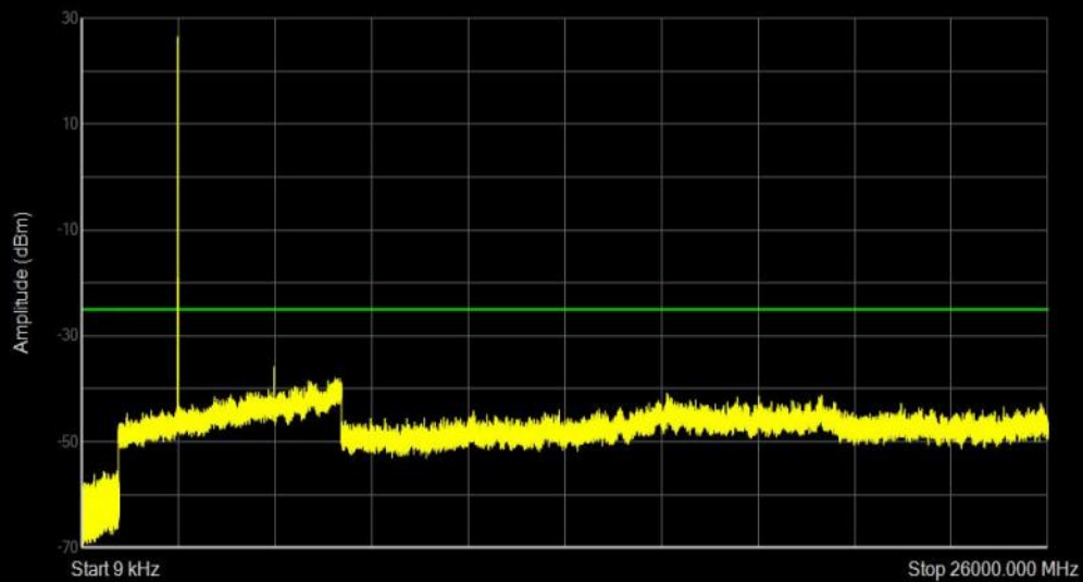
Band38 QPSK BW=5MHz Channel=38000 RB Size=1 Position=#0
