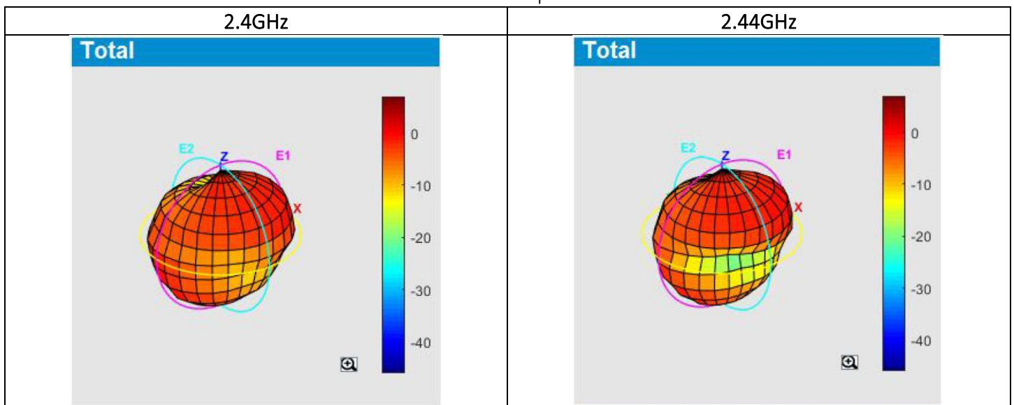
3D radiation pattern
