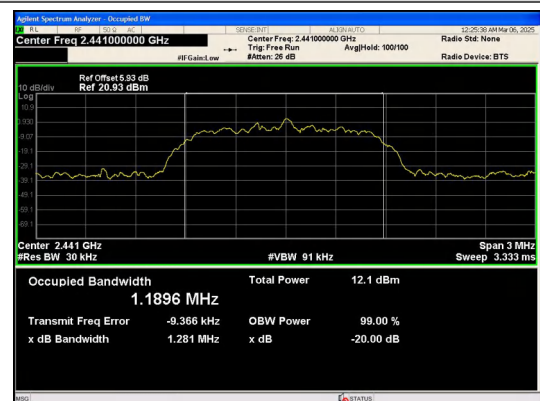
\pi/4 DQPSK_2-DH3_Channel 39
