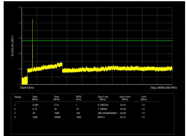
Band2 QPSK BW=15MHz Channel=18675 RB Size=75 Position=#0
