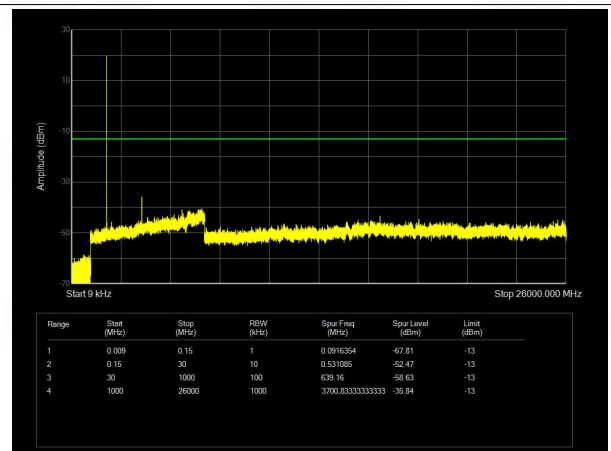
Band2 QAM16 BW=1.4MHz Channel=18607 RB Size=6 Position=#0
