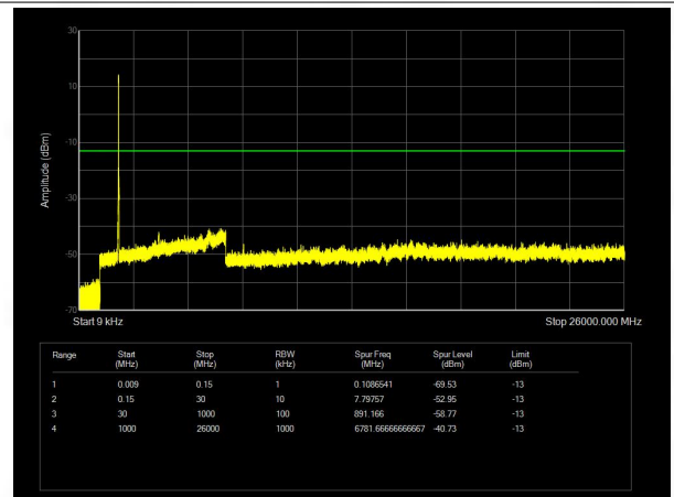
Band2 QPSK BW=15MHz Channel=19125 RB Size=75 Position=#0
