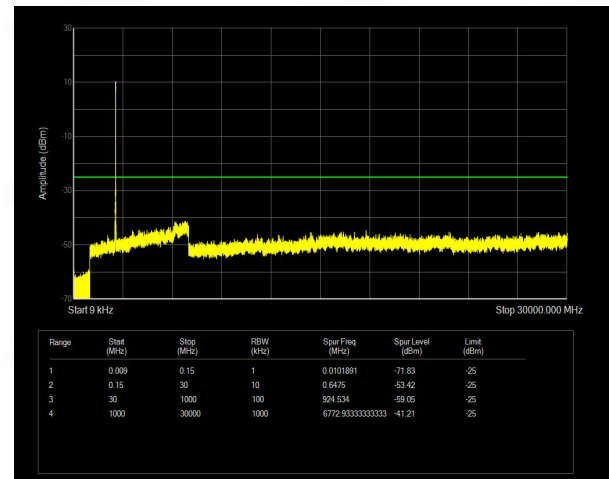
Band41(2555-2655) QAM16 BW=10MHz Channel=40290 RB Size=50 Position=#0
