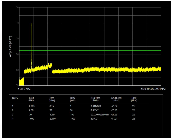
Band41(2555-2655) QPSK BW=15MHz Channel=40315 RB Size=75 Position=#0
