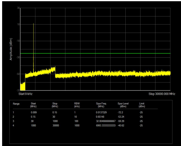
Band41(2555-2655) QPSK BW=5MHz Channel=41215 RB Size=25 Position=#0
