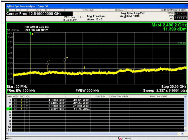
30.0 MHz - 25000.0 MHz GFSK_DH5_Channel 78
