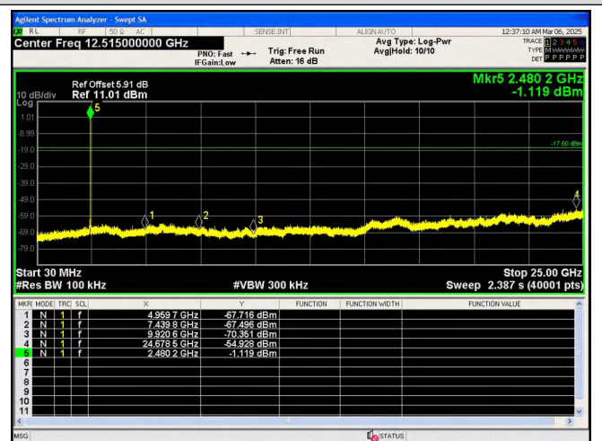
30.0 MHz - 25000.0 MHz \pi/4 DQPSK_2-DH1_Channel 78
