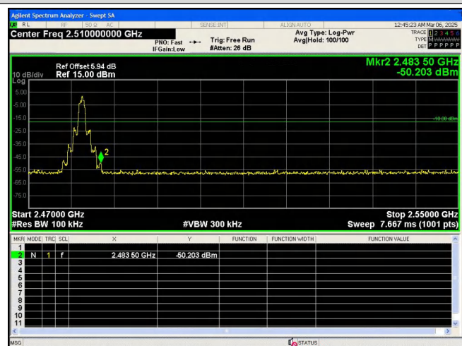
Out Of Band Emission 8DPSK_3-DH3_Channel 78
