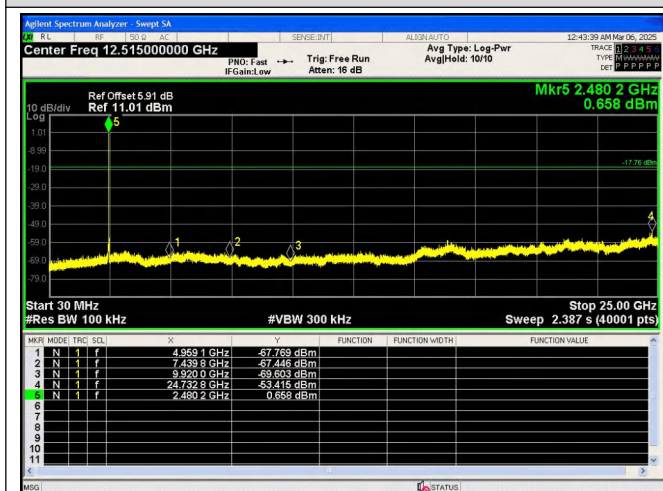
30.0 MHz - 25000.0 MHz 8DPSK_3-DH1_Channel 78
