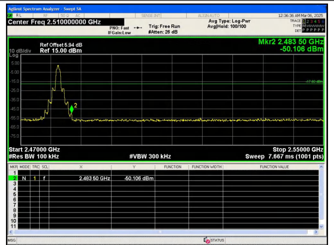
Out Of Band Emission \pi/4 DQPSK_2-DH1_Channel 78
