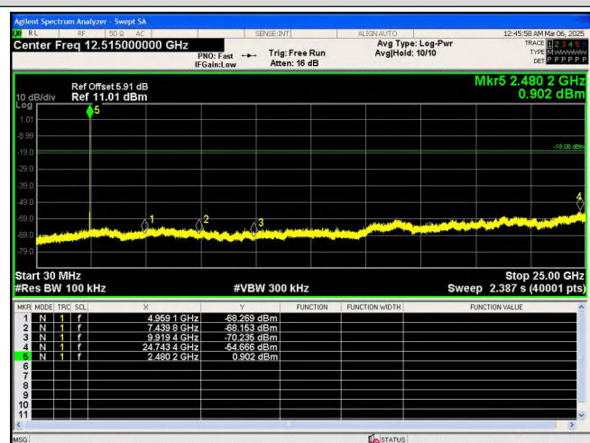
30.0 MHz - 25000.0 MHz 8DPSK_3-DH3_Channel 78
