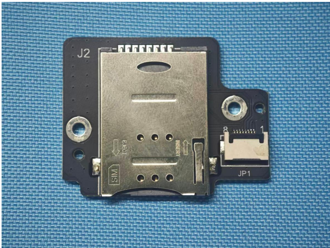
Photo 18 PCB2 SIM-V1.1
