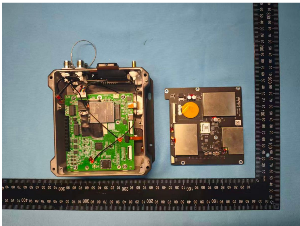
Photo 4 PCB3 Black Adapter Board - V2.320
