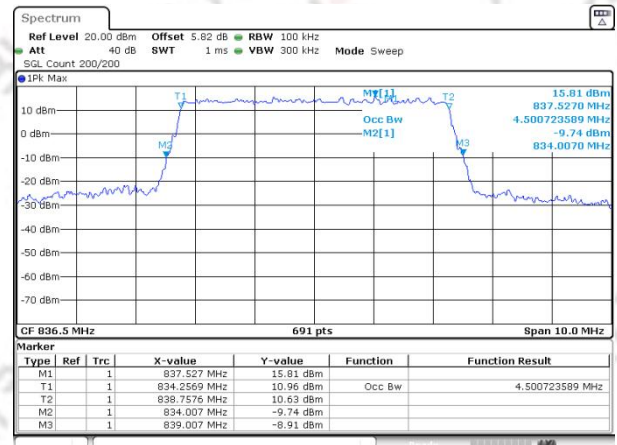
Band26(824-849) QAM16 BW=5MHz Channel=26915 RB Size=25 Position=#0
