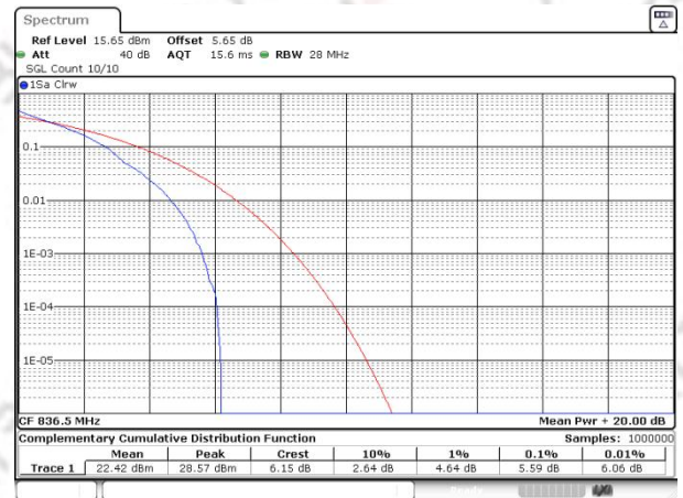
Band26(824-849) QPSK BW=1.4MHz Channel=26915 RB Size=1 Position=#0
