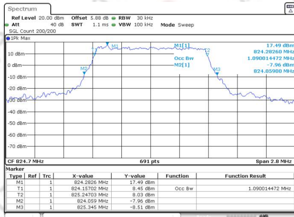
Band26(824-849) QAM16 BW=1.4MHz Channel=26797 RB Size=6 Position=#0
