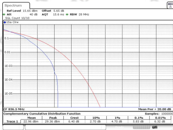
Band26(824-849) QAM16 BW=5MHz Channel=26915 RB Size=1 Position=#0
