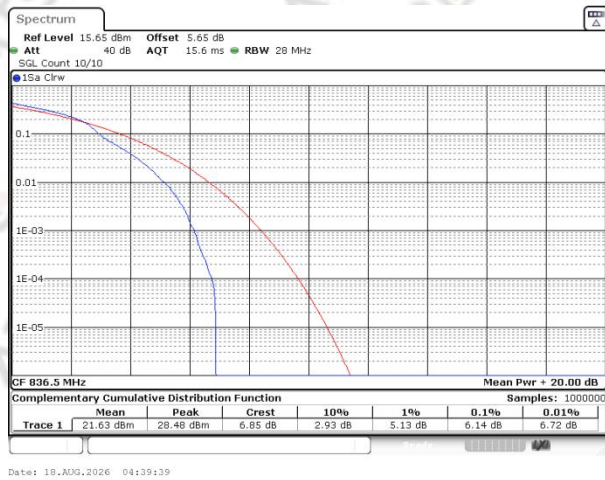
Band26(824-849) QAM16 BW=1.4MHz Channel=26915 RB Size=1 Position=#0
