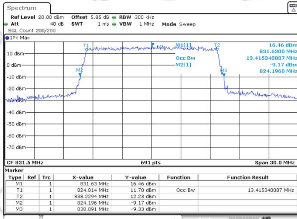
Band26(824-849) QAM16 BW=15MHz Channel=26865 RB Size=75 Position=#0
