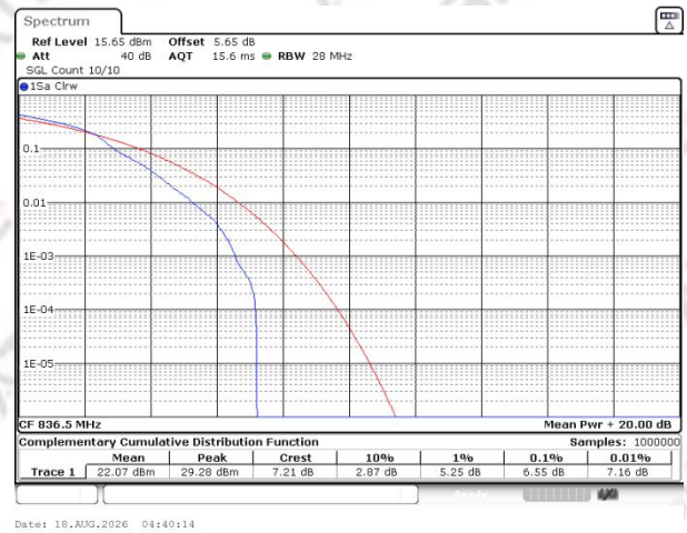
Band26(824-849) QAM16 BW=10MHz Channel=26915 RB Size=1 Position=#0
