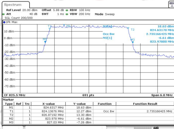
Band26(824-849) QPSK BW=3MHz Channel=26805 RB Size=15 Position=#0
