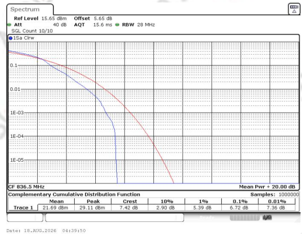
Band26(824-849) QAM16 BW=3MHz Channel=26915 RB Size=1 Position=#0
