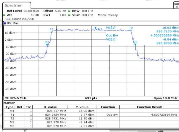
Band26(824-849) QAM16 BW=5MHz Channel=26815 RB Size=25 Position=#0
