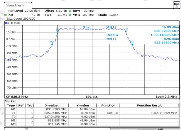
Band26(824-849) QAM16 BW=1.4MHz Channel=26915 RB Size=6 Position=#0
