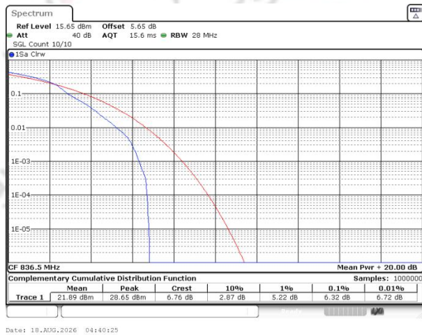
Band26(824-849) QAM16 BW=15MHz Channel=26915 RB Size=1 Position=#0
