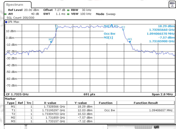
Band4 QPSK BW=1.4MHz Channel=20175 RB Size=6 Position=#0
