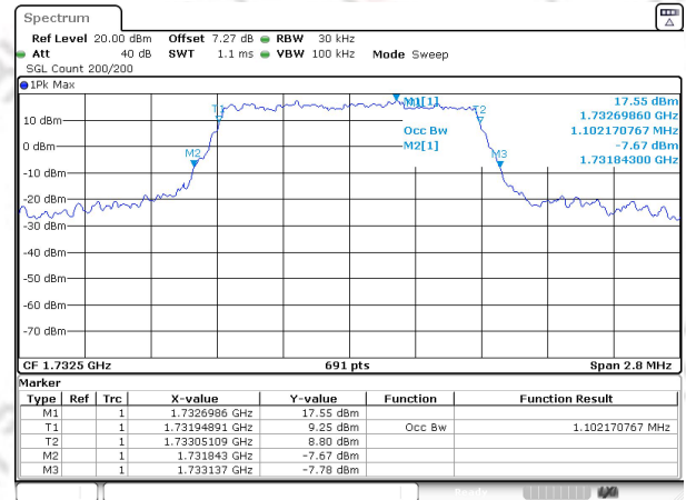
Band4 QAM16 BW=1.4MHz Channel=20175 RB Size=6 Position=#0
