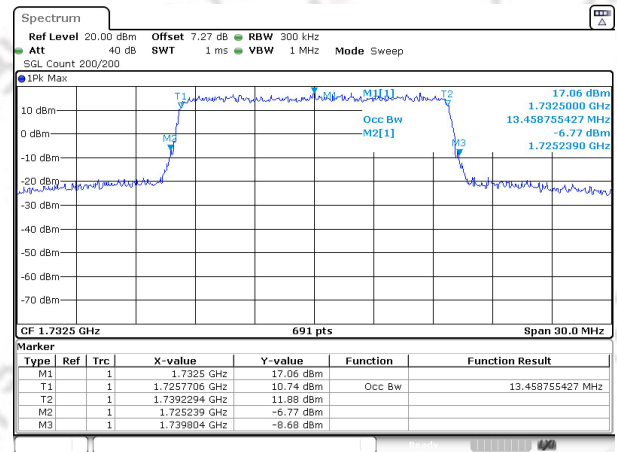
Band4 QAM16 BW=15MHz Channel=20175 RB Size=75 Position=#0
