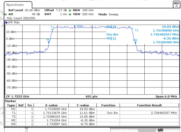
Band4 QAM16 BW=3MHz Channel=20175 RB Size=15 Position=#0
