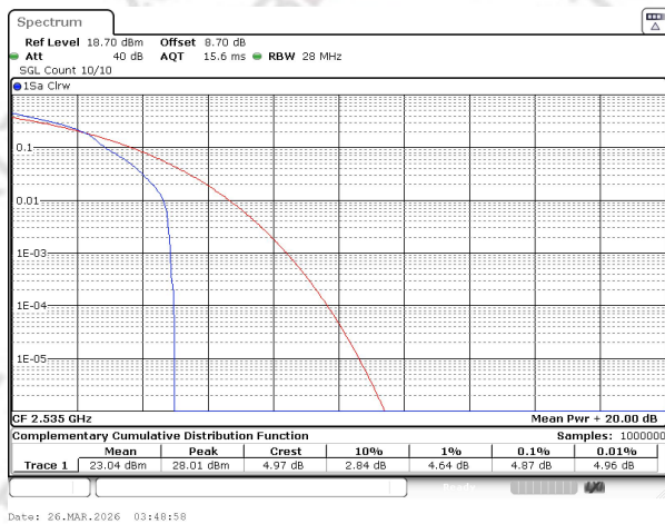
Band7 QAM16 BW=20MHz Channel=21100 RB Size=1 Position=#0 NVNT
