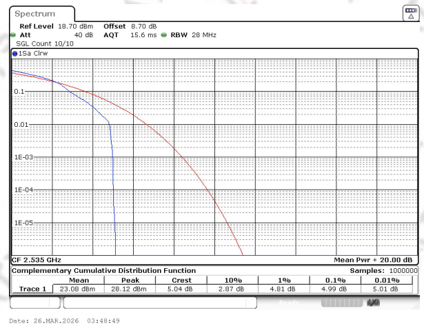
Band7 QAM16 BW=15MHz Channel=21100 RB Size=1 Position=#0 NVNT
