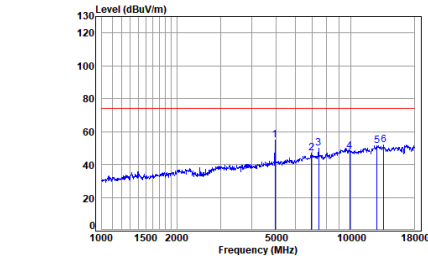
BLE_2M_TX_CH_39_Horizontal-Peak
