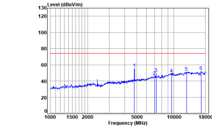
BLE_2M_TX_CH_00_Horizontal-Peak
