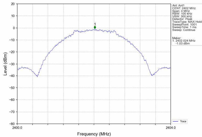
2M_LCH_2402MHz_Ant1_NTNV
