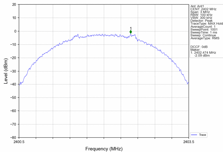
2M_LCH_2402MHz_Ant1_NTNV
