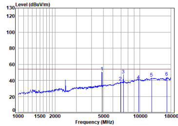
BLE_1M_TX_CH_19_Horizontal-Avg
