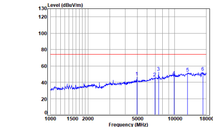
BLE_2M_TX_CH_39_Vertical-Peak
