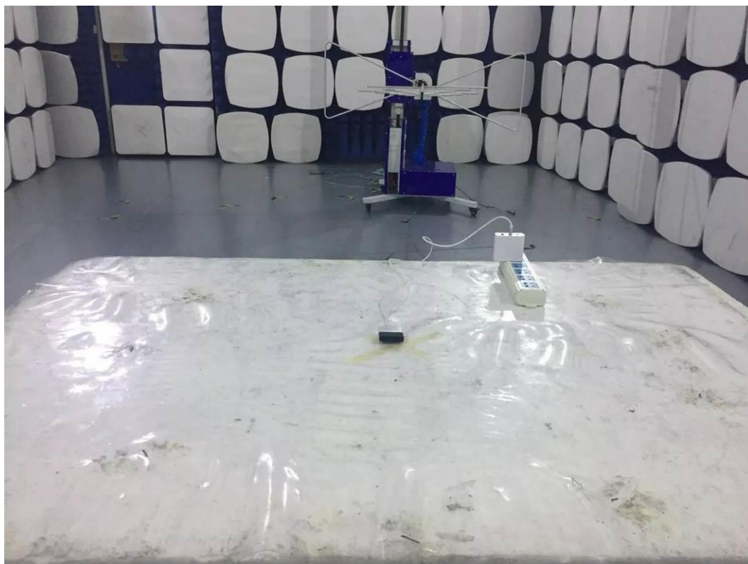
Radiated emission
