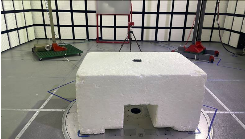
RADIATED PHOTO (BLE <30 MHz)
