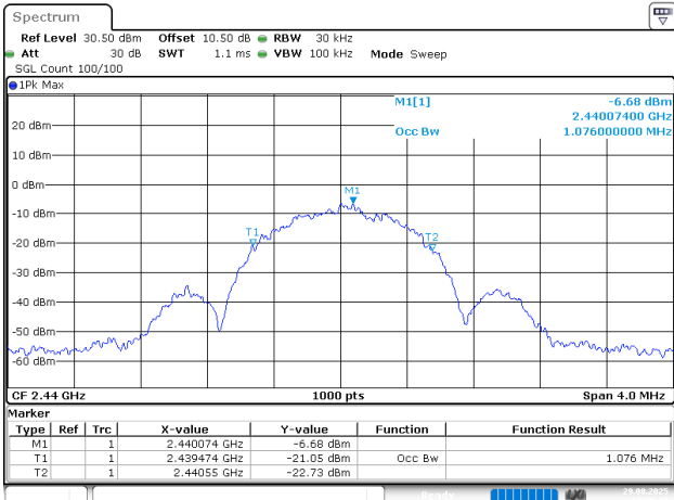
BLE_1M_Middle_Channel
