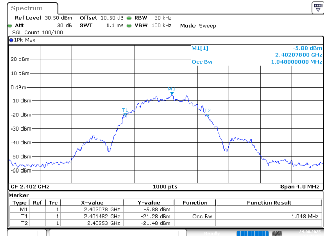
BLE_1M_Low_Channel
