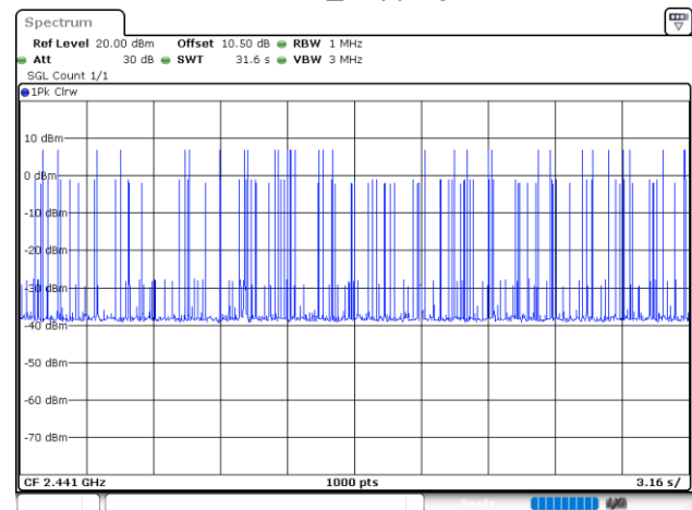
3DH3_Hopping
