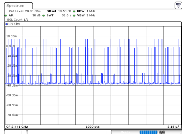
3DH5_Hopping
