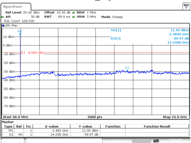
2DH5_High
