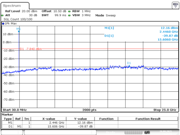
DH5_Middle
