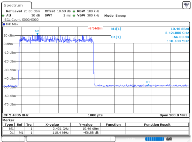
3DH5_Hopping_Upper
