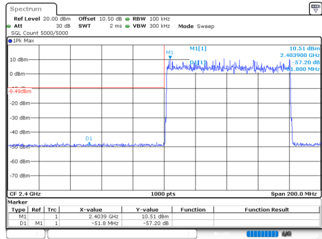
3DH5_Hopping_Lower
