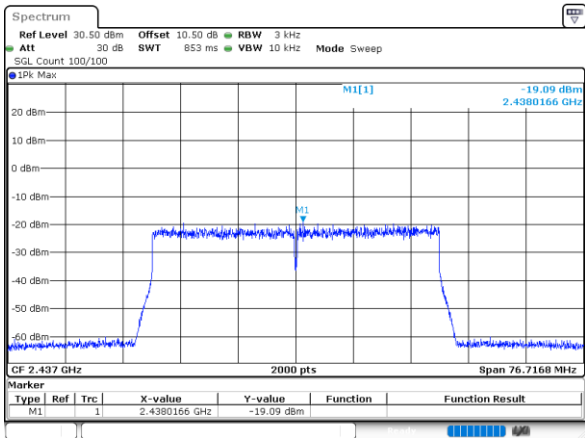
802.11ax40_2437MHz_RU_Full_Chain 1
