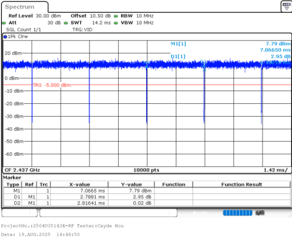
802.11ax20_2437MHz_RU_FULL_Chain 0
