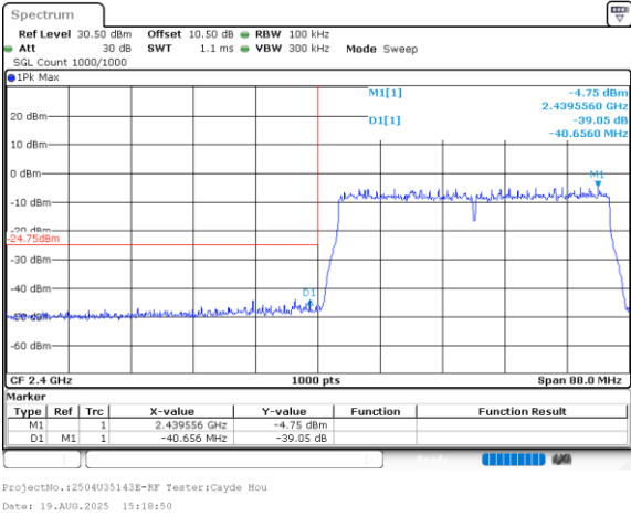
802.11ax40_2422MHz_RU_Full_Chain 1
