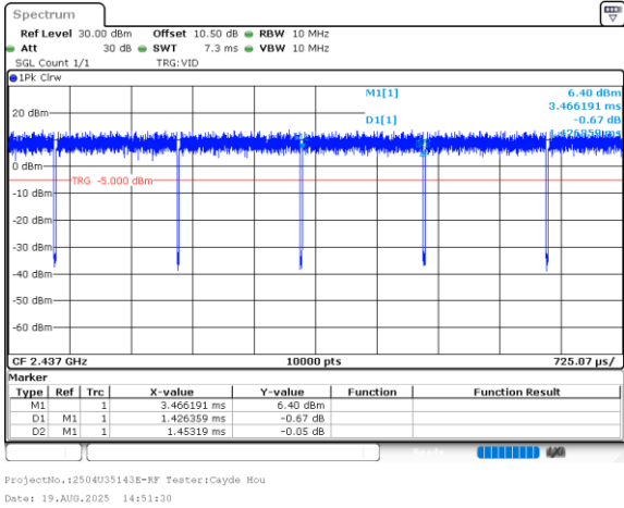
802.11ax40_2437MHz_RU_FULL_Chain 1
