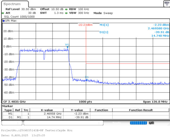
802.11n40_2452MHz_Chain 1
