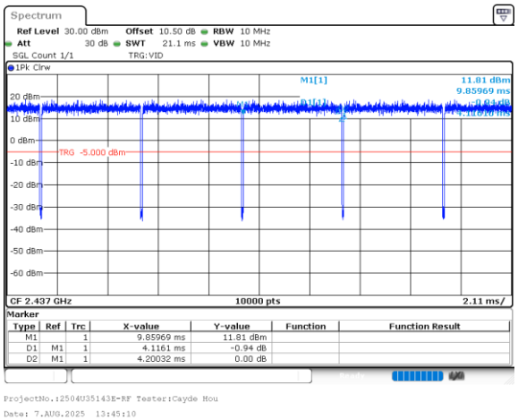
802.11g_2437MHz_Chain 1
