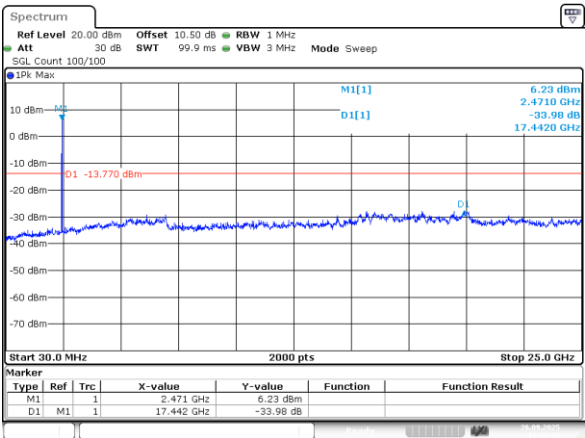
802.11ax20_2462MHz_RU_Full_Chain 1
