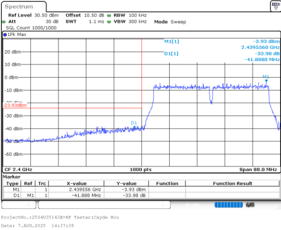
802.11n40_2422MHz_Chain 0
