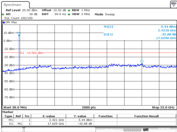
802.11ax20_2412MHz_RU_Full_Chain 0
