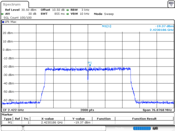
802.11ax40_2422MHz_RU_Full_Chain 1
