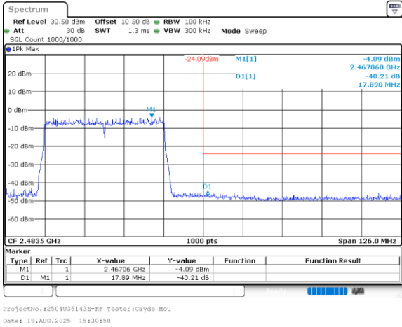
802.11ax40_2452MHz_RU_Full_Chain 1
