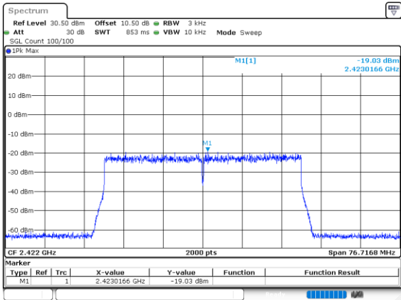
802.11ax40_2422MHz_RU_Full_Chain 0
