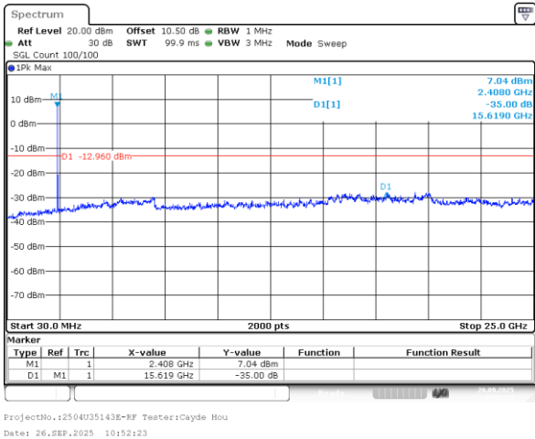
802.11ax40_2422MHz_RU_Full_Chain 0
