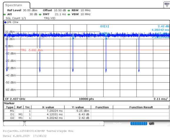
802.11g_2437MHz_Chain 0
