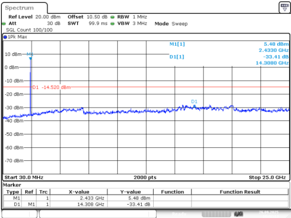
802.11ax20_2437MHz_RU_Full_Chain 0
