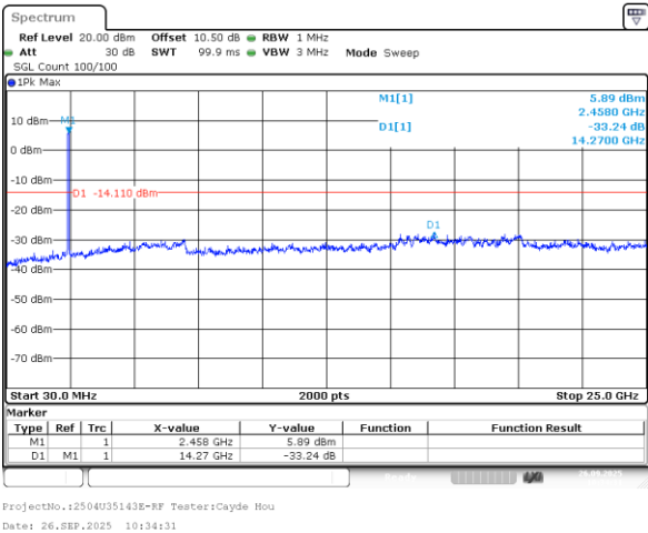
802.11n40_2437MHz_Chain 0
