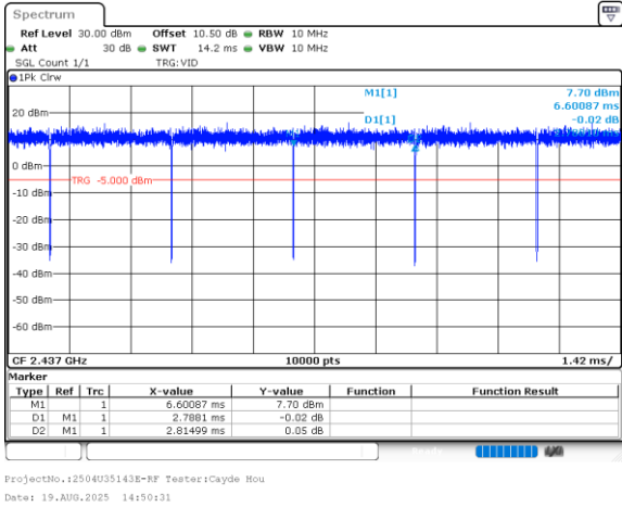
802.11ax20_2437MHz_RU_FULL_Chain 1
