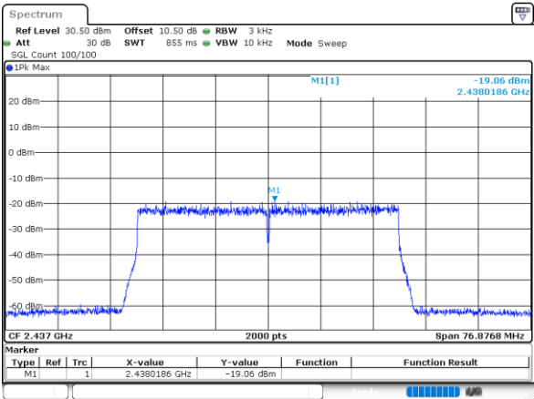
802.11ax40_2437MHz_RU_Full_Chain 0
