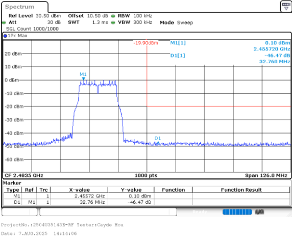
802.11g_2462MHz_Chain 1
