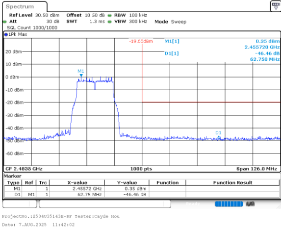
802.11g_2462MHz_Chain 0
