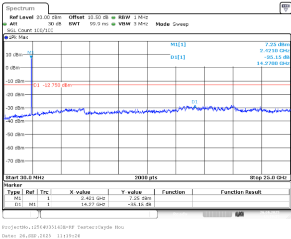
802.11n40_2437MHz_Chain 1
