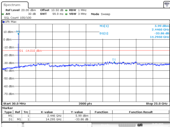
802.11ax20_2437MHz_RU_Full_Chain 1
