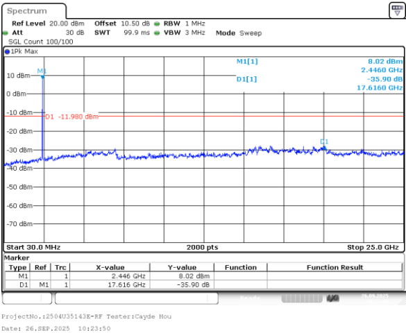
802.11g_2437MHz_Chain 0
