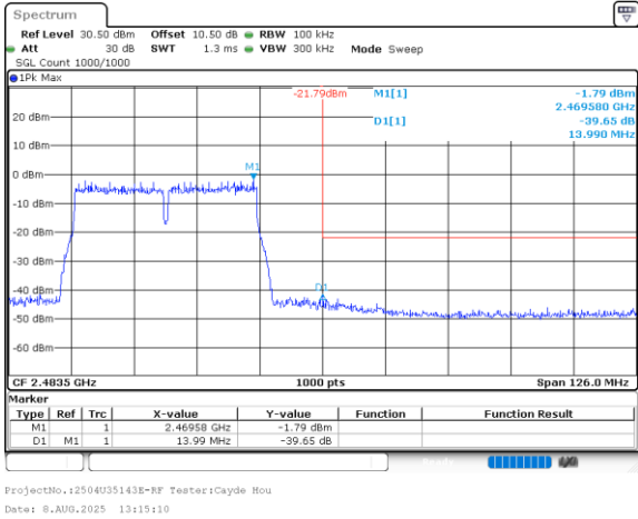
802.11n40_2452MHz_Chain 0
