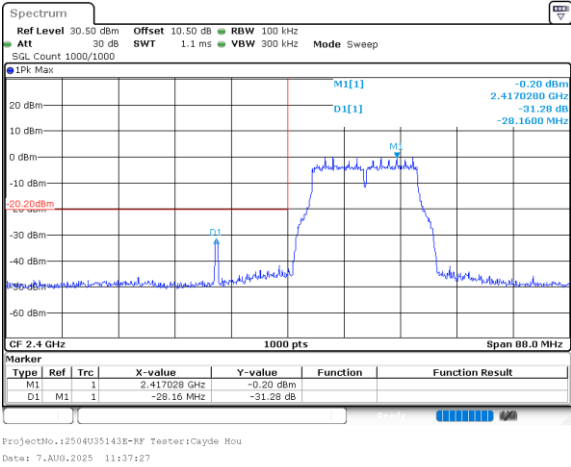
802.11g_2412MHz_Chain 0
