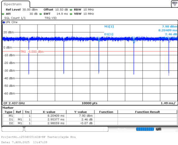
802.11n40_2437MHz_Chain 1
