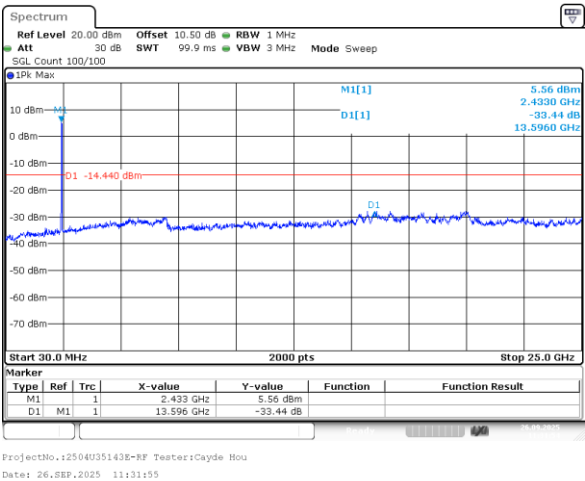
802.11ax40_2452MHz_RU_Full_Chain 1
