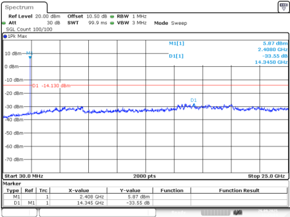
802.11ax20_2412MHz_RU_Full_Chain 1
