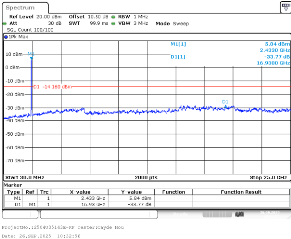
802.11n40_2422MHz_Chain 0
