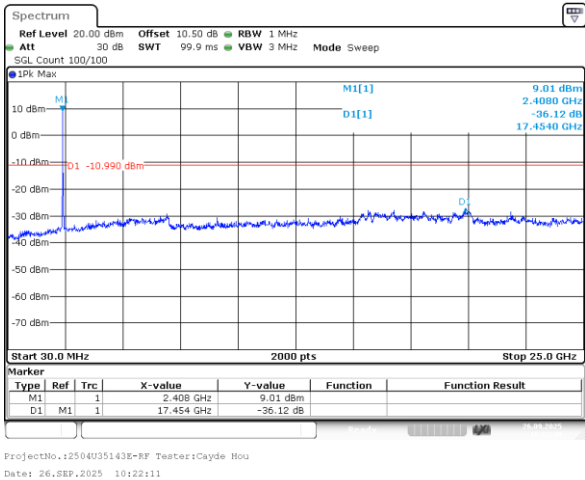
802.11g_2412MHz_Chain 0
