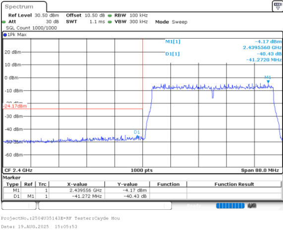
802.11ax40_2422MHz_RU_Full_Chain 0
