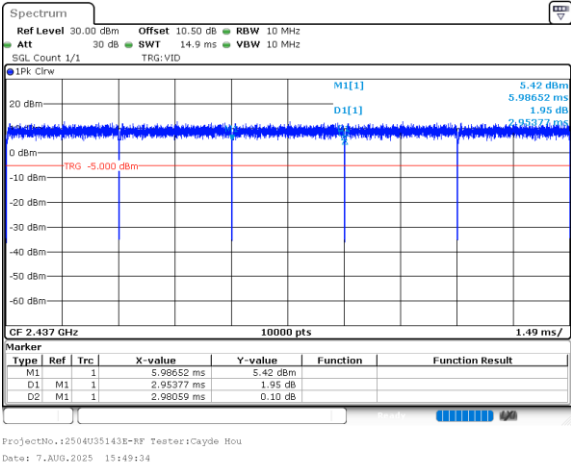
802.11n40_2437MHz_Chain 0
