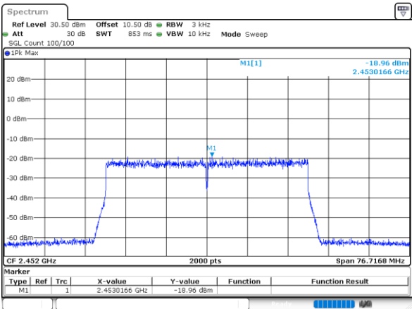
802.11ax40_2452MHz_RU_Full_Chain 1
