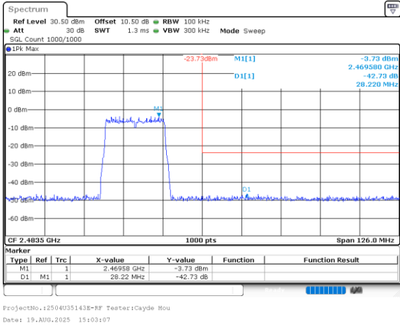
802.11ax20_2462MHz_RU_Full_Chain 0
