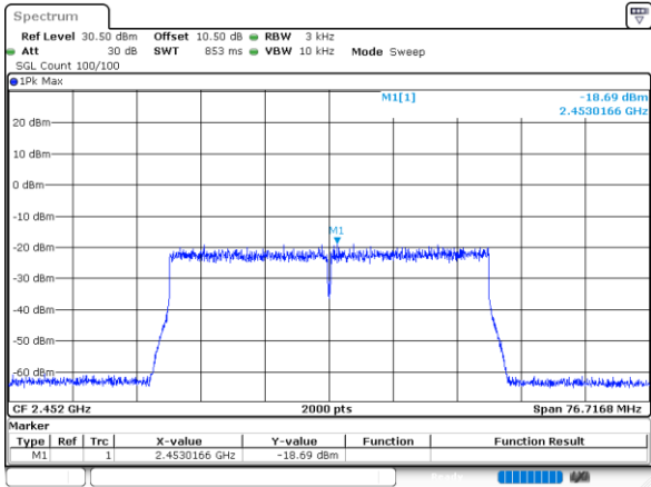
802.11ax40_2452MHz_RU_Full_Chain 0
