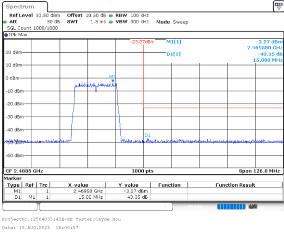
802.11ax20_2462MHz_RU_Full_Chain 1
