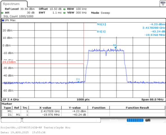
802.11ax20_2412MHz_RU_Full_Chain 1
