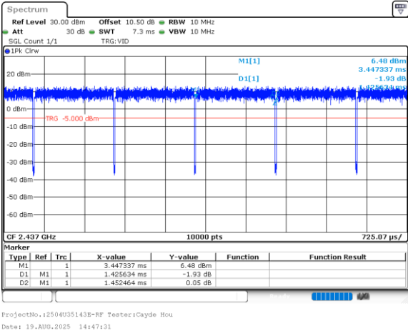
802.11ax40_2437MHz_RU_FULL_Chain 0
