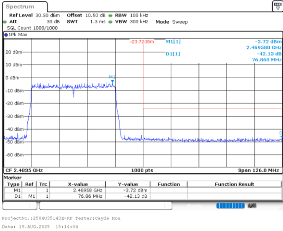
802.11ax40_2452MHz_RU_Full_Chain 0
