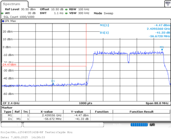
802.11n40_2422MHz_Chain 1
