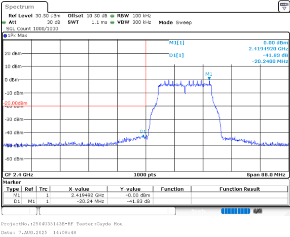
802.11g_2412MHz_Chain 1
