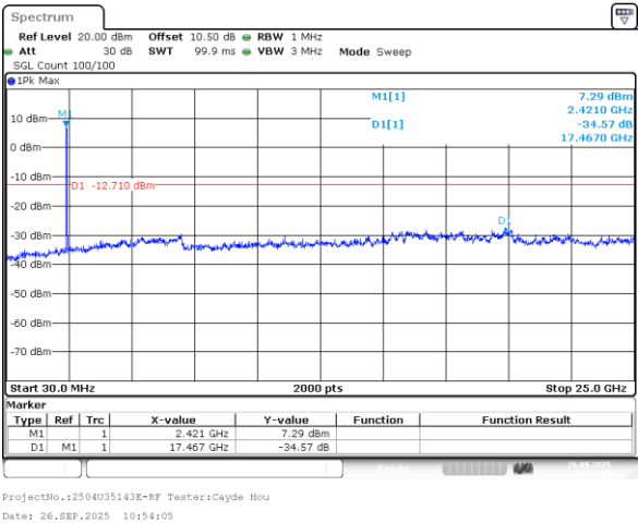
802.11ax40_2437MHz_RU_Full_Chain 0
