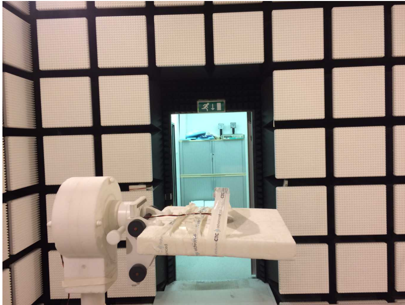
Photo 5 - RSE Setup > 1000 MHz
