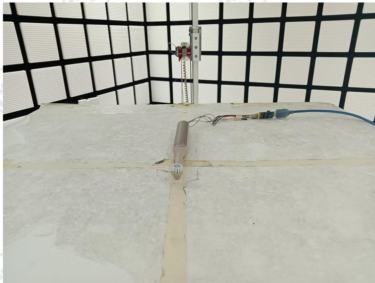
Radiated spurious emission Test Setup-2(Above 1GHz)
