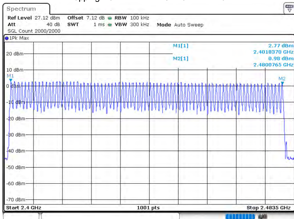
Hopping No. NVNT 1-DH5 2402MHz Ant 2
