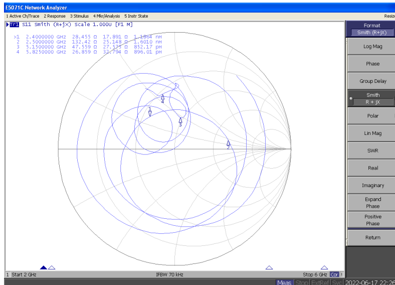
Smith chart
