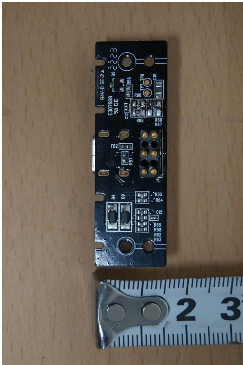
< Charging cradle main board bottom view >
