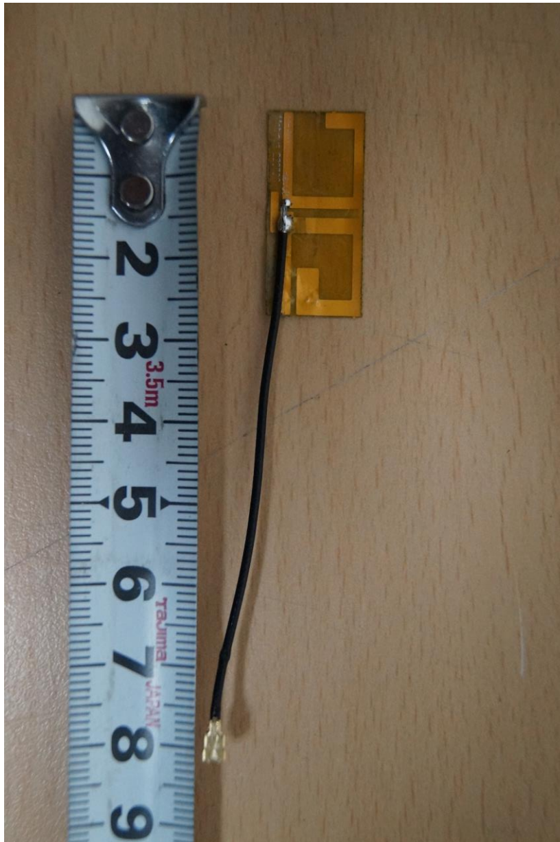
< Antenna Top view >
