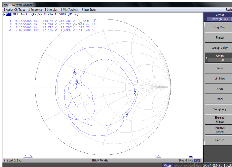
Smith chart
