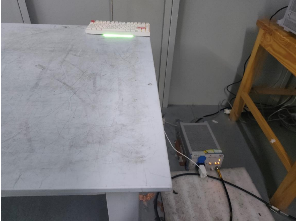
Description: AC Conducted Emissions Test Setup Photo
