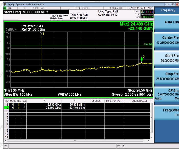
5.8G_Ant1_5790_0~Reference
