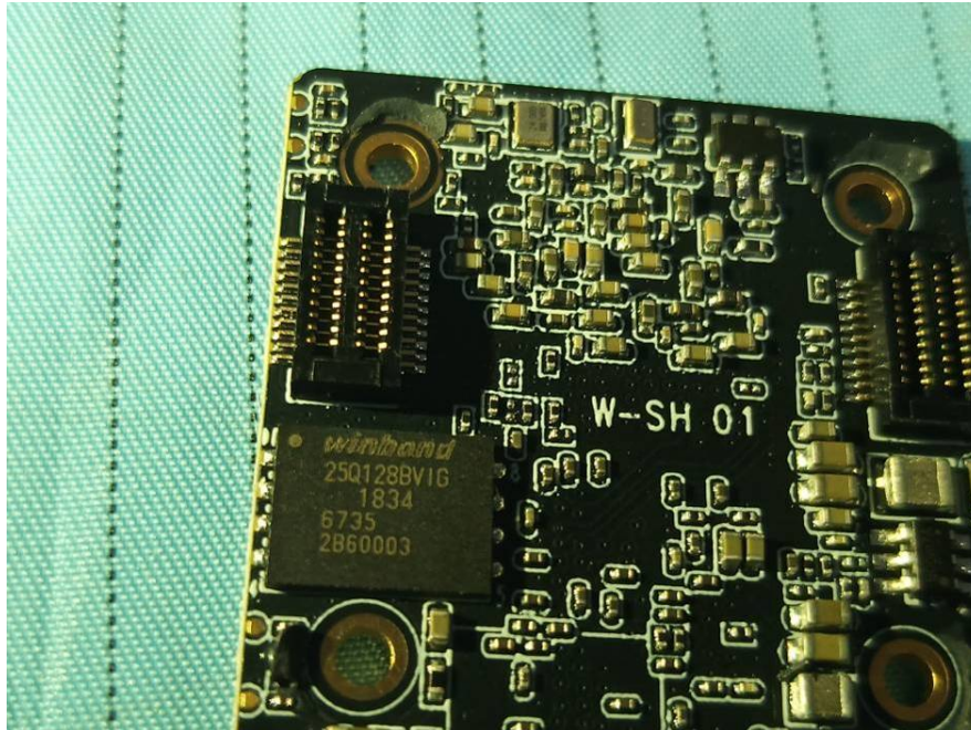
EUT – IC Chip 1 View (for Main Board 3)
