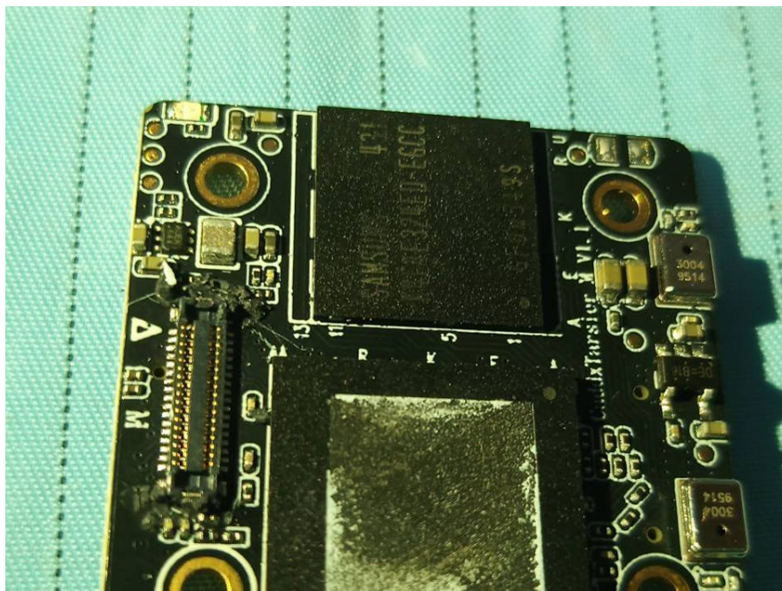
EUT – IC Chip 2 View (for Main Board 3)
