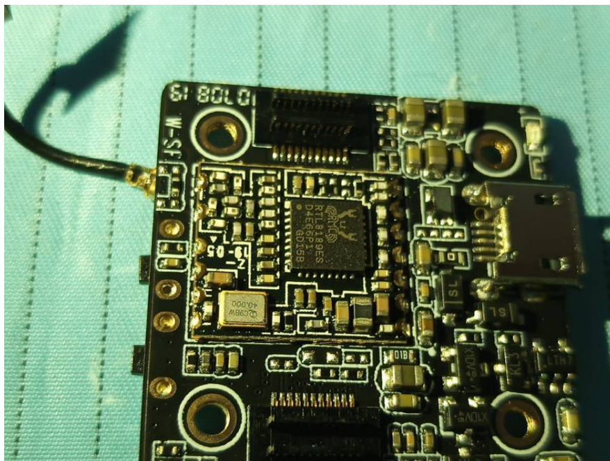
EUT – IC Chip View (for Main Board 2)
