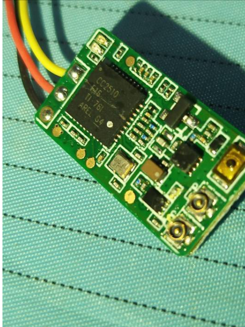
EUT – IC Chip View (for Main Board 5)
