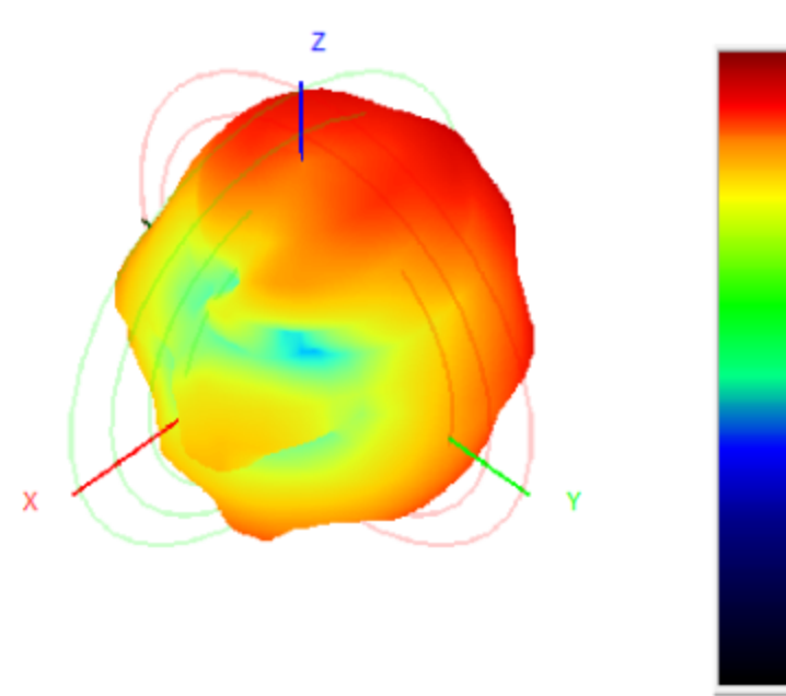
445MHz H+V, Eff: 17.4%
