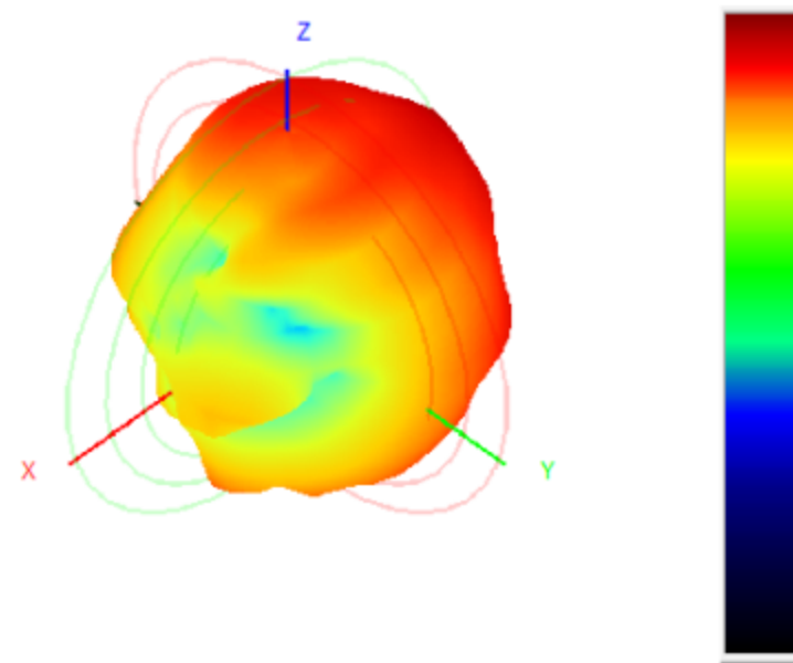
439MHz H+V, Eff: 13.2%
