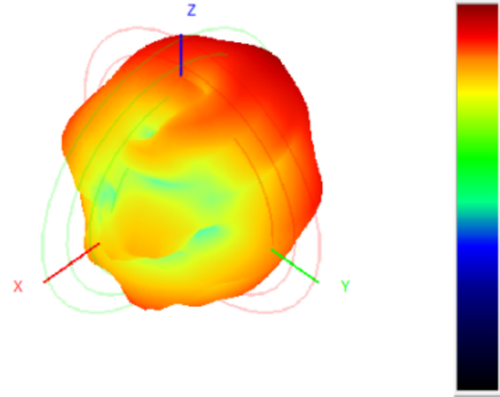
435MHz H+V, Eff: 10.5%
