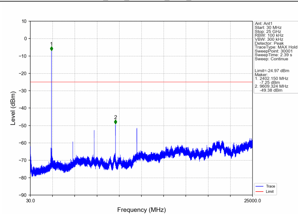
2M_LCH_2402MHz_Ant1_NTNV
