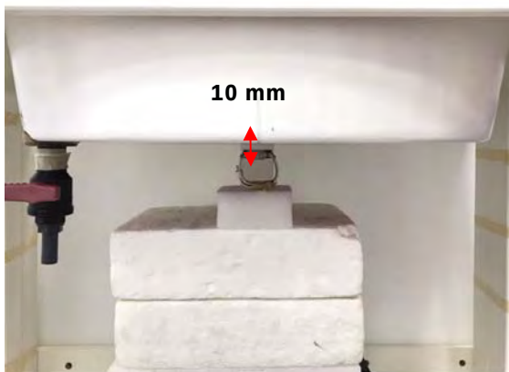
Fig.4 Front side of EUT to flat phantom
