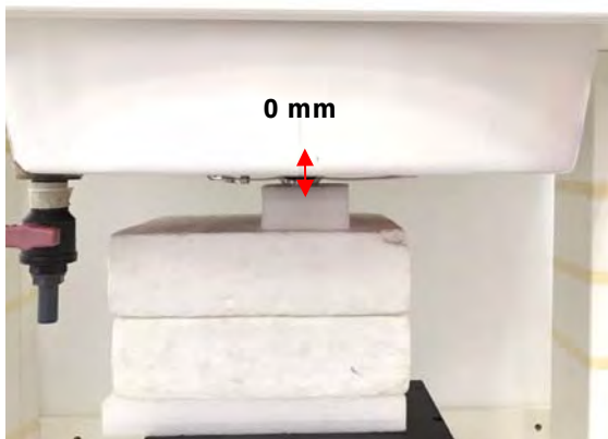
Fig.3 Back side of EUT to flat phantom
