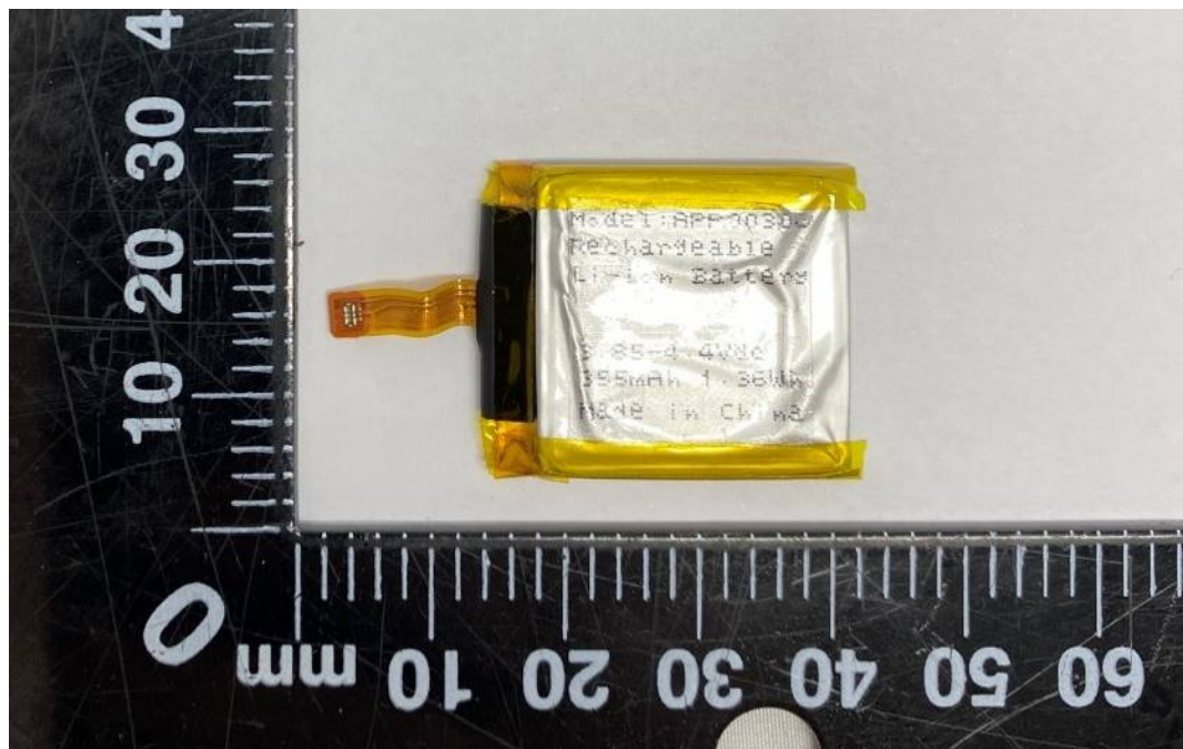
Fig. 6. Battery view-01
