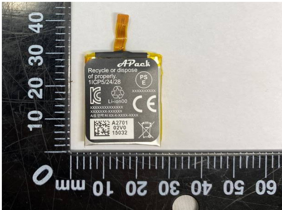
Fig. 7. Battery view-02
