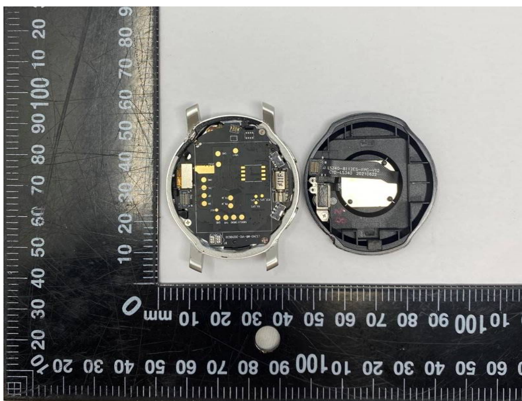
Fig. 2. Internal view-01
