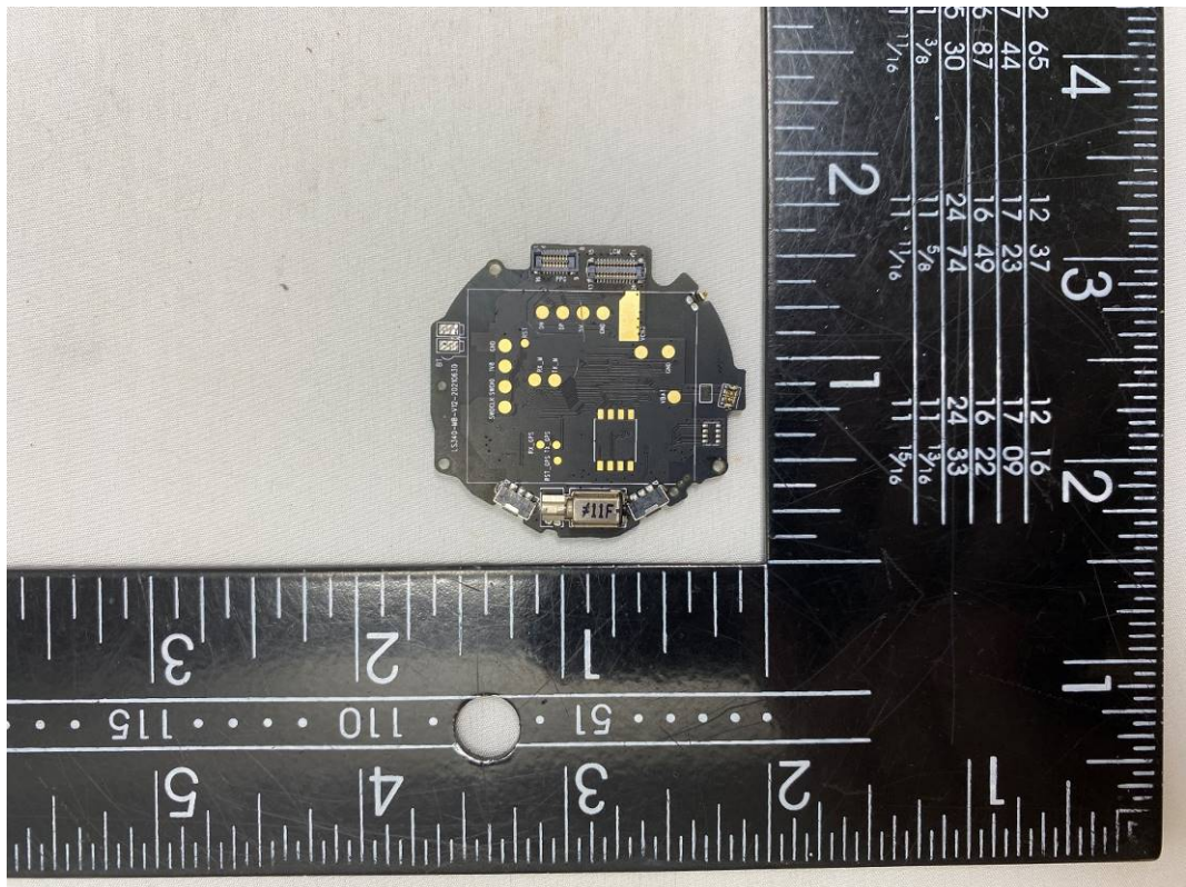
Fig. 3. Internal view-02
