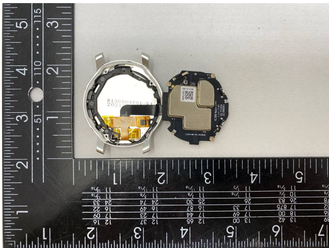
Fig. 4. PCB view-01
