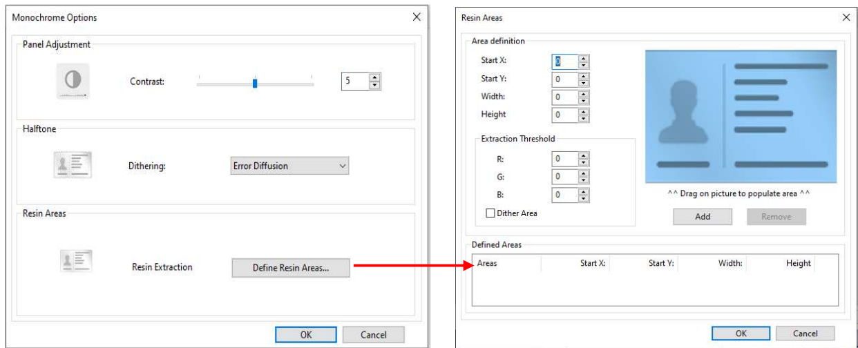
Resin Areas extraction user interface
